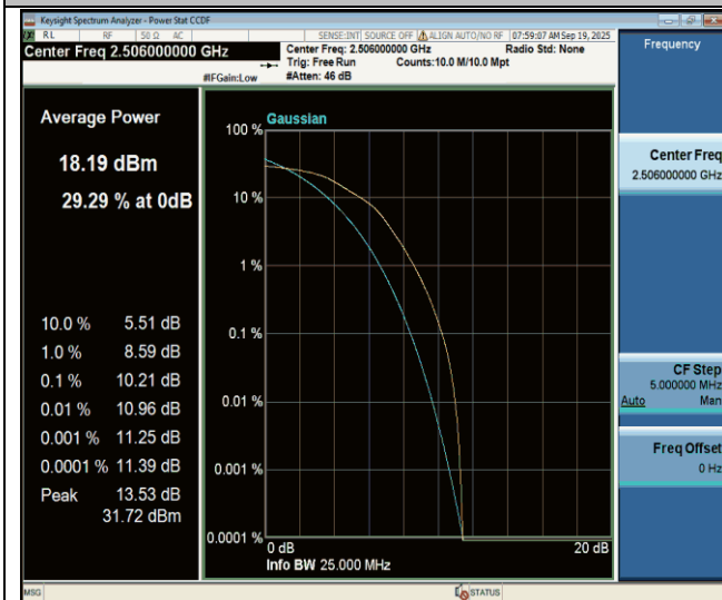
Band41-20MHz-16QAM-39750-100RB#0-PASS
