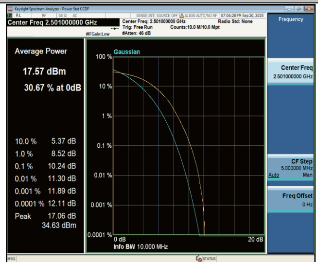
Band41-10MHz-64QAM-39700-50RB#0-PASS
