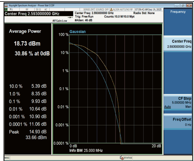
Band41-20MHz-16QAM-40620-100RB#0-PASS
