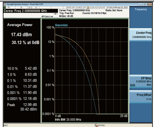
Band41-20MHz-64QAM-39750-100RB#0-PASS
