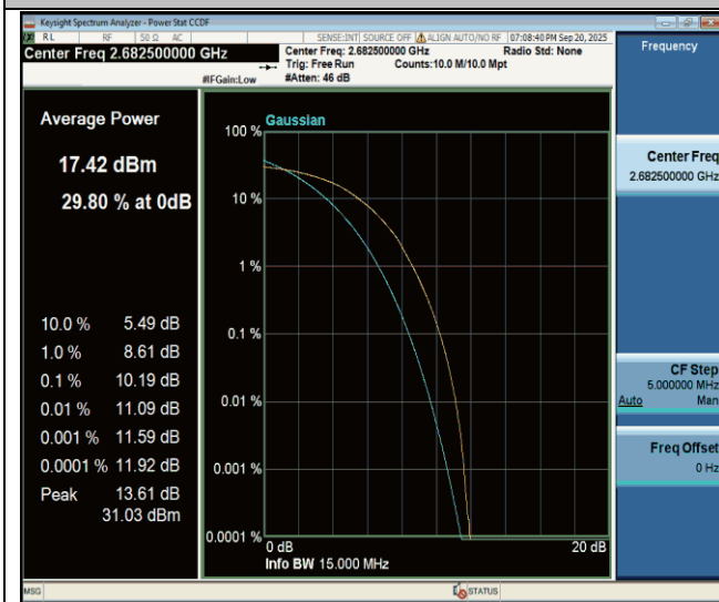
Band41-15MHz-64QAM-41515-75RB#0-PASS
