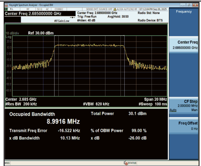
Band41-10MHz-64QAM-41540-50RB#0-PASS
