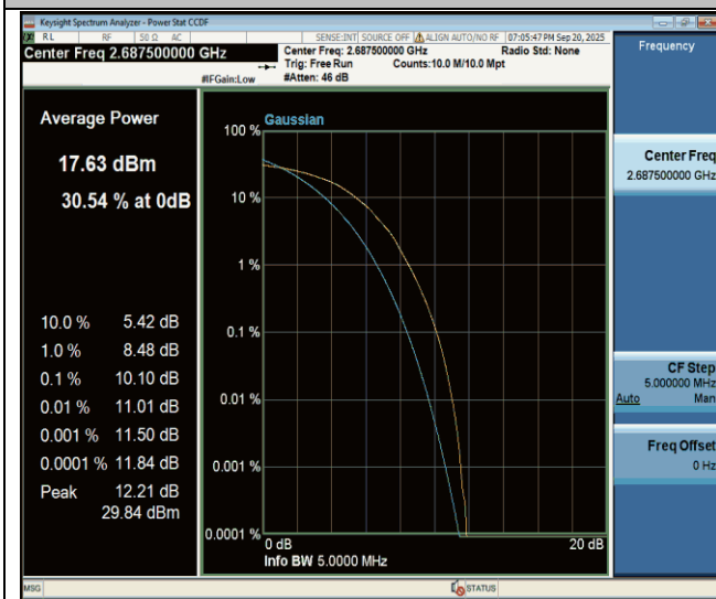
Band41-5MHz-64QAM-41565-25RB#0-PASS
