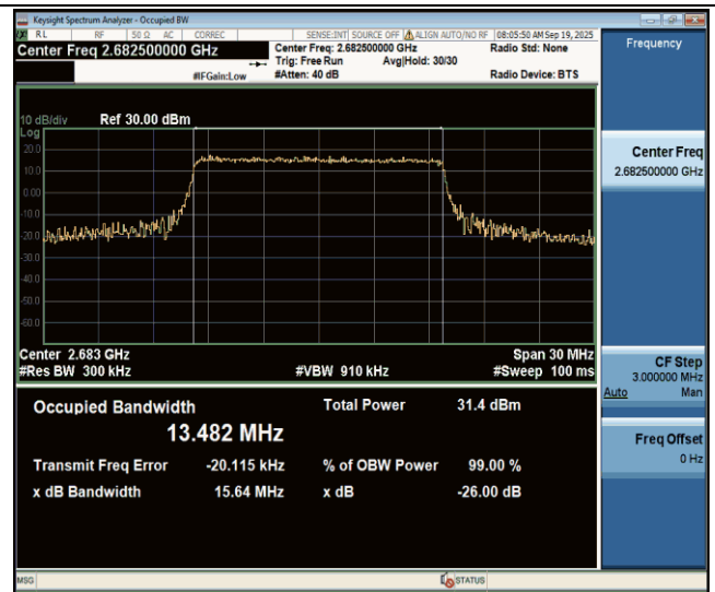
Band41-15MHz-16QAM-41515-75RB#0-PASS
