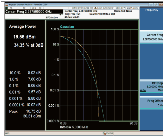
Band41-5MHz-QPSK-41565-25RB#0-PASS
