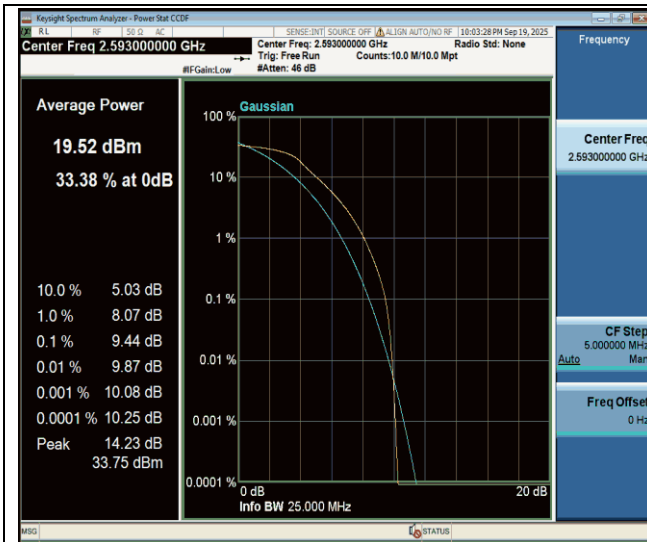
Band41-20MHz-QPSK-40620-100RB#0-PASS
