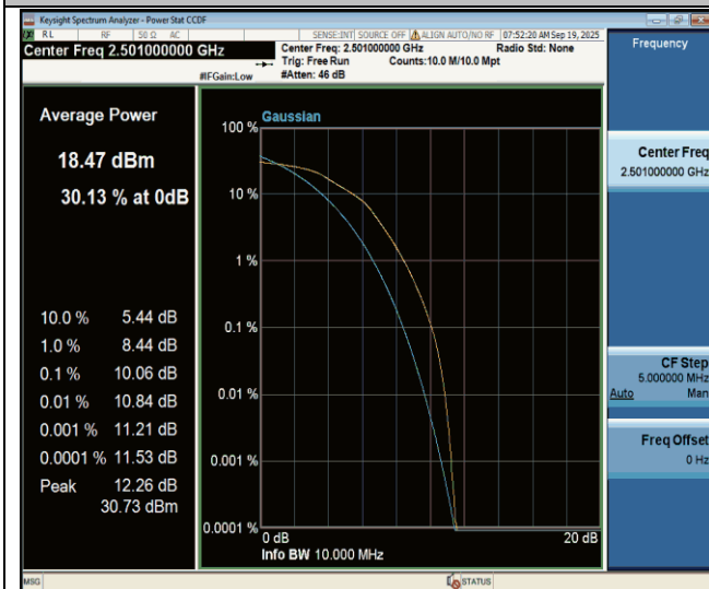
Band41-10MHz-16QAM-39700-50RB#0-PASS
