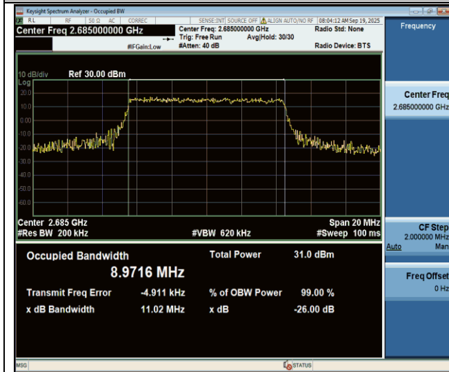
Band41-10MHz-16QAM-41540-50RB#0-PASS
