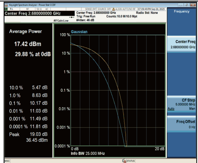
Band41-20MHz-64QAM-41490-100RB#0-PASS
