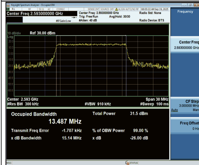
Band41-15MHz-16QAM-40620-75RB#0-PASS
