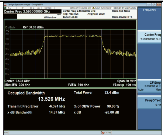
Band41-15MHz-QPSK-40620-75RB#0-PASS
