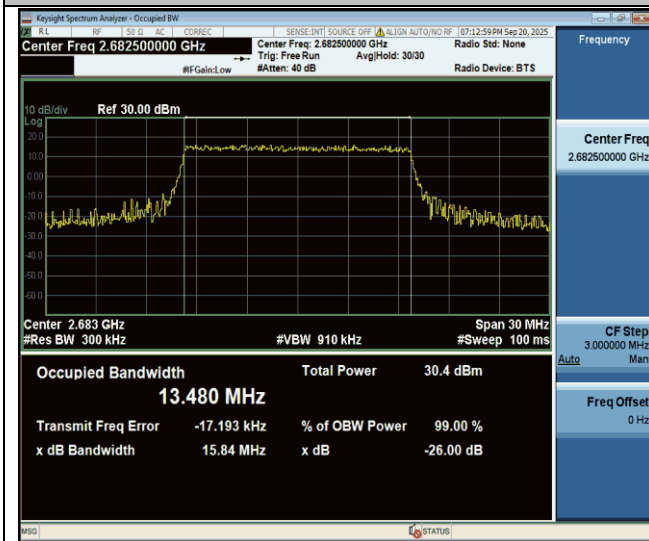
Band41-15MHz-64QAM-41515-75RB#0-PASS
