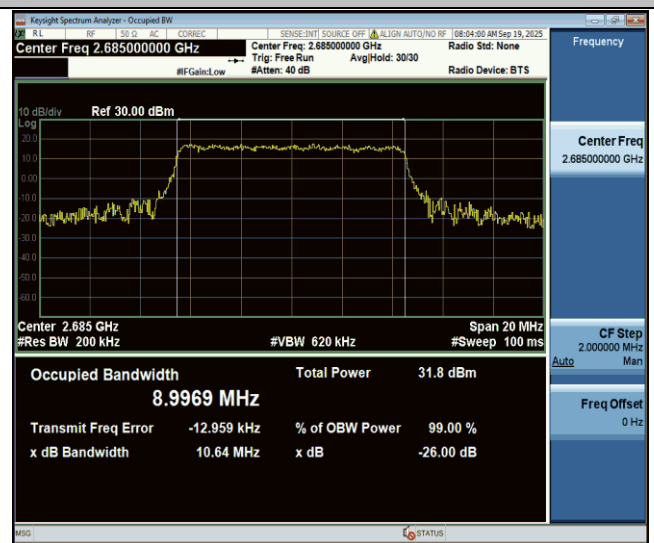
Band41-10MHz-QPSK-41540-50RB#0-PASS
