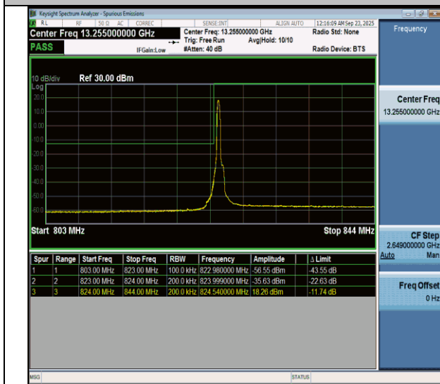
NTNV-n5-PC3-15-20-L-CP-QPSK-Edge_1RB_Left-PASS
