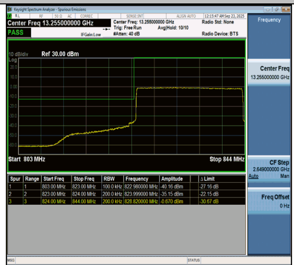
NTNV-n5-PC3-15-20-L-CP-QPSK-Outer_Full-PASS
