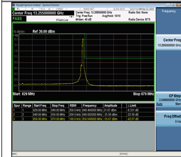
NTNV-n5-PC3-15-20-H-DFT-BPSK-Edge_1RB_Right-PASS
