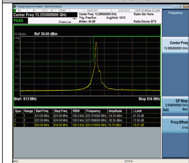
NTNV-n5-PC3-15-10-L-DFT-BPSK-Edge_1RB_Left-PASS
