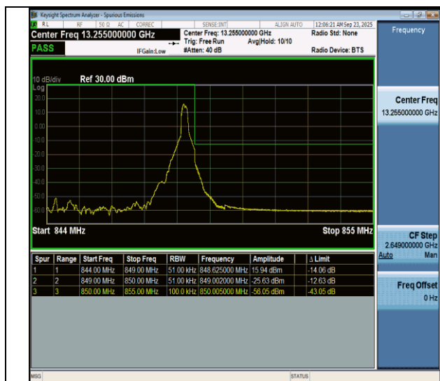
NTNV-n5-PC3-15-5-H-CP-QPSK-Edge_1RB_Right-PASS
