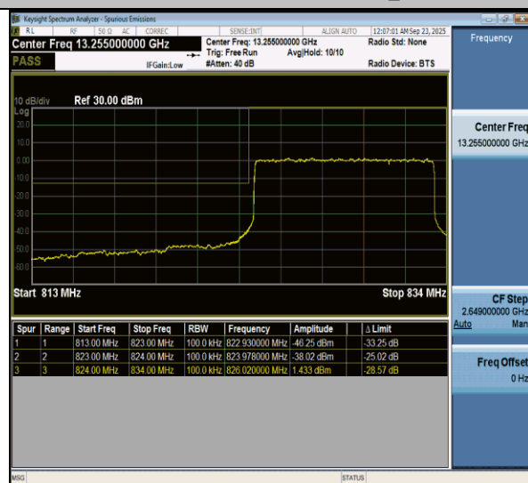
NTNV-n5-PC3-15-10-L-DFT-BPSK-Outer_Full-PASS
