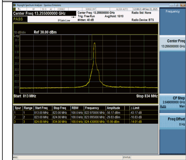
NTNV-n5-PC3-15-10-L-CP-QPSK-Edge_1RB_Left-PASS
