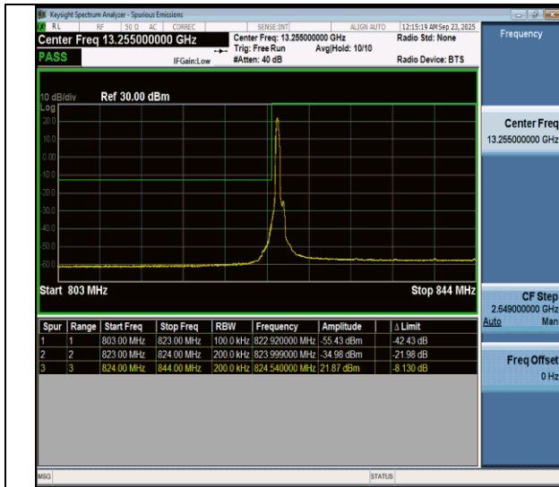
NTNV-n5-PC3-15-20-L-DFT-BPSK-Edge_1RB_Left-PASS
