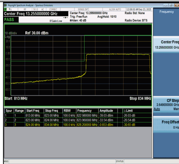
NTNV-n5-PC3-15-10-L-CP-QPSK-Outer_Full-PASS
