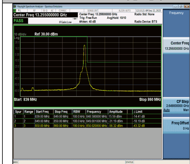
NTNV-n5-PC3-15-10-H-CP-QPSK-Edge_1RB_Right-PASS
