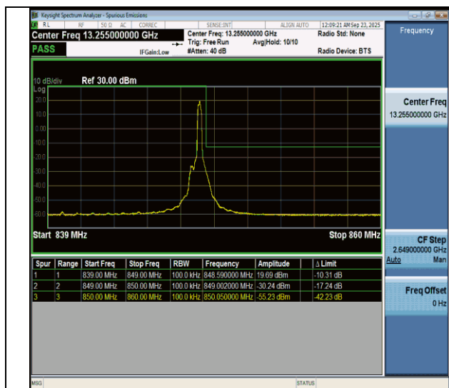
NTNV-n5-PC3-15-10-H-DFT-BPSK-Edge_1RB_Right-PASS
