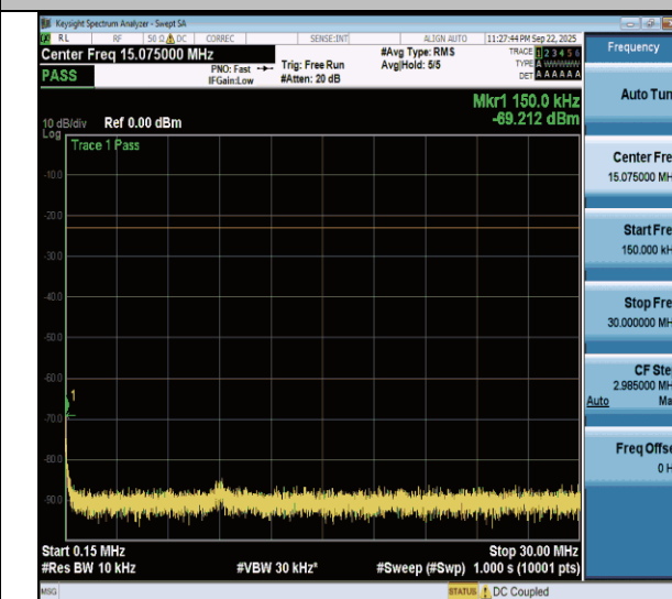
NTNV-n5-PC3-15-20-M-DFT-BPSK-Edge_1RB_Left-12000-20000-PASS
