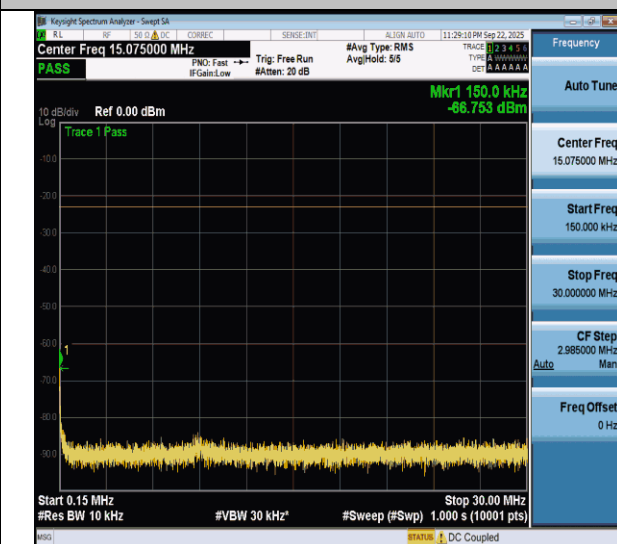
NTNV-n5-PC3-15-20-H-DFT-BPSK-Edge_1RB_Left-0.15-30- PASS
