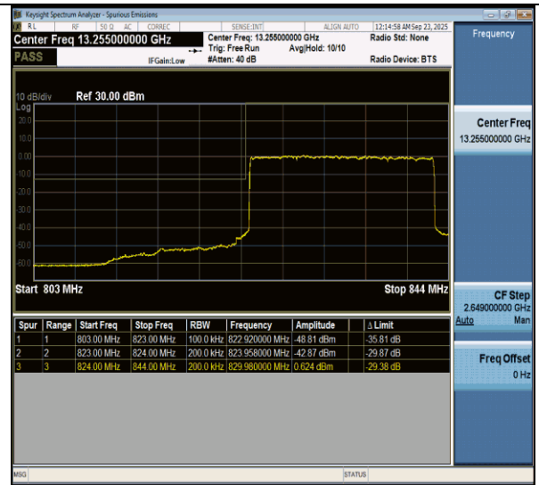
NTNV-n5-PC3-15-20-L-DFT-BPSK-Outer_Full-PASS
