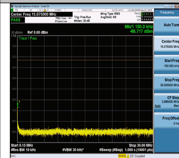
NTNV-n5-PC3-15-20-M-DFT-BPSK-Edge_1RB_Left-0.15-30- PASS
