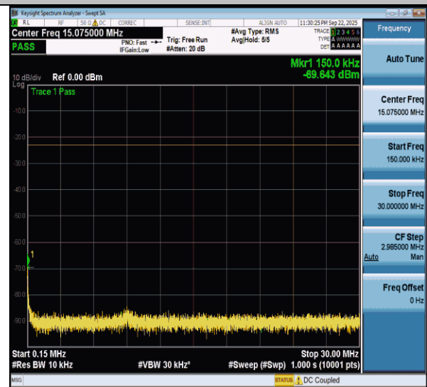
NTNV-n5-PC3-15-20-H-CP-QPSK-Edge_1RB_Left-0.15-30-PASS
