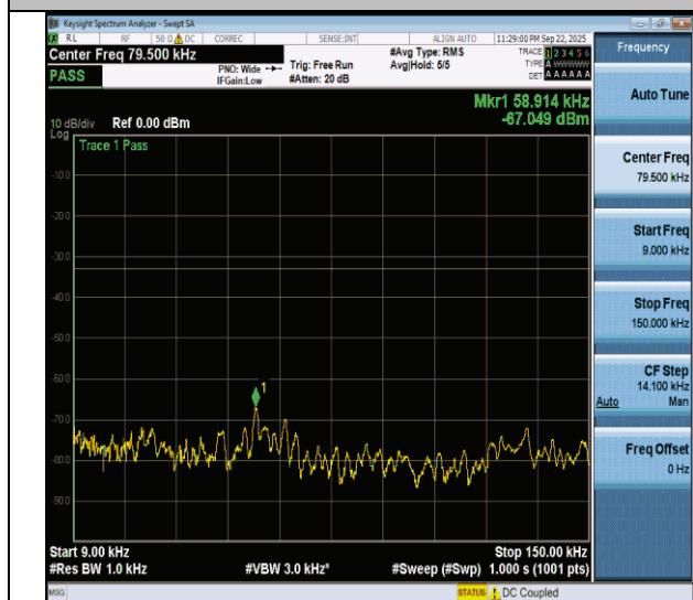
NTNV-n5-PC3-15-20-H-DFT-BPSK-Edge_1RB_Left-0.009-0.15- PASS
