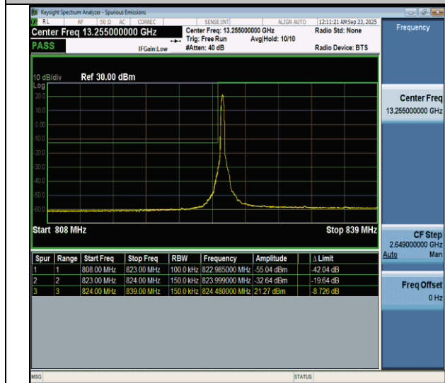
NTNV-n5-PC3-15-15-L-DFT-BPSK-Edge_1RB_Left-PASS
