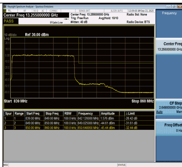
NTNV-n5-PC3-15-10-H-DFT-BPSK-Outer_Full-PASS
