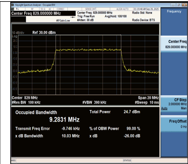
NTNV-n26(824-849)-PC3-15-10-L-CP-256QAM-Outer_Full-Ant1- PASS
