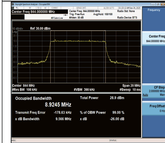
NTNV-n26(824-849)-PC3-15-10-H-DFT-64QAM-Outet_Full-Ant1- PASS
