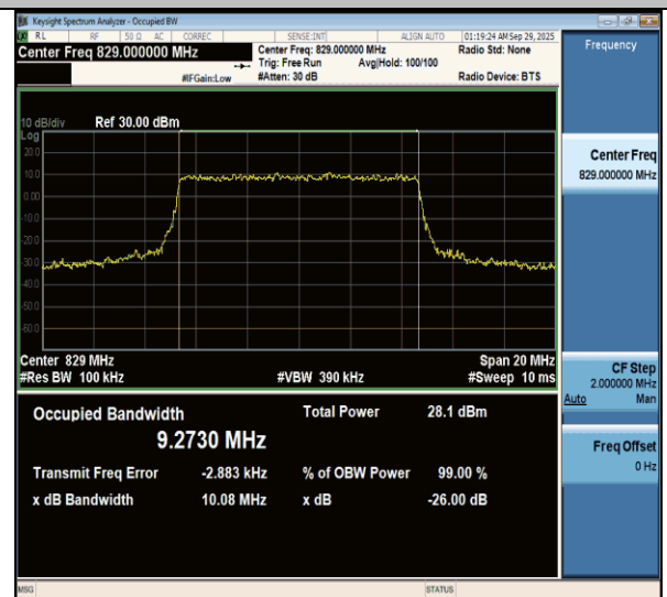
NTNV-n26(824-849)-PC3-15-10-L-CP-16QAM-Outet_Full-Ant1- PASS
