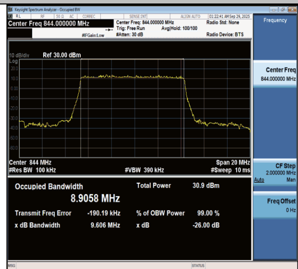
NTVN-n26(824-849)-PC3-15-10-H-DFT-BPSK-Outet_Full-Ant1-PASS
