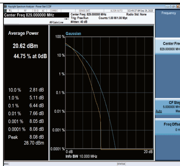
NTNV-n26(824-849)-PC3-15-10-L-DFT-256QAM-Outer_Full-PASS
