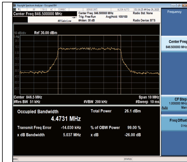
NTNV-n26(824-849)-PC3-15-5-H-DFT-256QAM-Outer_Full-Ant1- PASS
