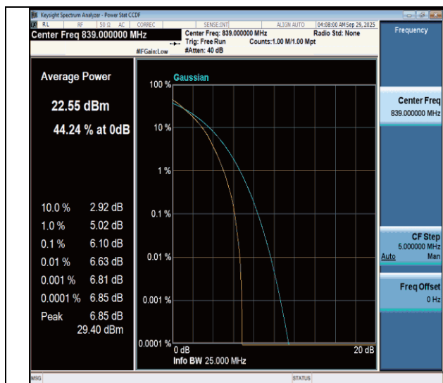
NTNV-n26(824-849)-PC3-15-20-H-DFT-64QAM-Outer_Full-PASS
