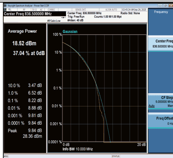
NTNV-n26(824-849)-PC3-15-5-M-CP-256QAM-Outer_Full-PASS
