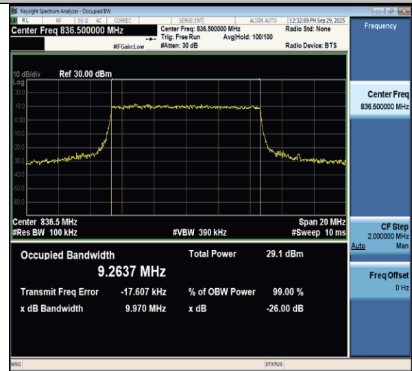
NTVN-n26(824-849)-PC3-15-10-M-CP-64QAM-Outet_Full-Ant1-PASS
