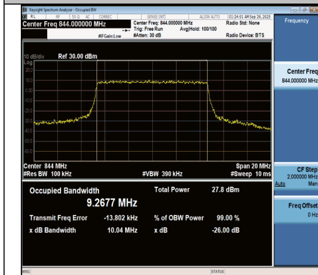
NTNV-n26(824-849)-PC3-15-10-H-CP-QPSK-Outet_Full-Ant1- PASS
