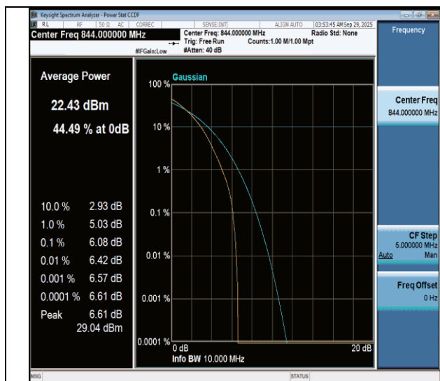
NTNV-n26(824-849)-PC3-15-10-H-DFT-64QAM-Outer_Full-PASS
