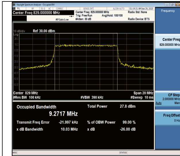
NTNV-n26(824-849)-PC3-15-10-L-CP-64QAM-Outer_Full-Ant1- PASS
