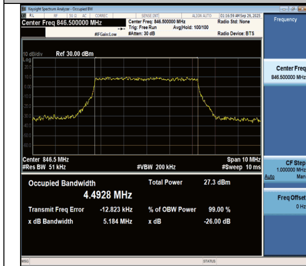
NTNV-n26(824-849)-PC3-15-5-H-CP-16QAM-Outer_Full-Ant1- PASS
