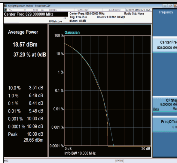
NTNV-n26(824-849)-PC3-15-10-L-CP-256QAM-Outer_Full-PASS
