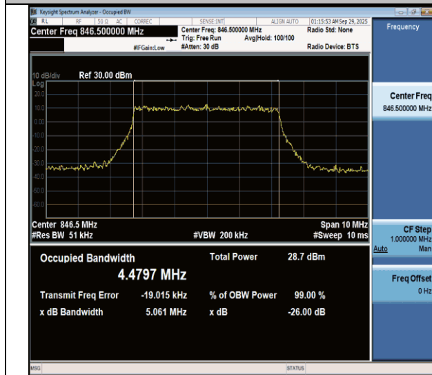
NTNV-n26(824-849)-PC3-15-5-H-DFT-16QAM-Outet_Full-Ant1- PASS
