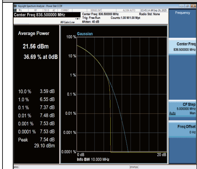
NTNV-n26(824-849)-PC3-15-5-M-CP-64QAM-Outer_Full-PASS
