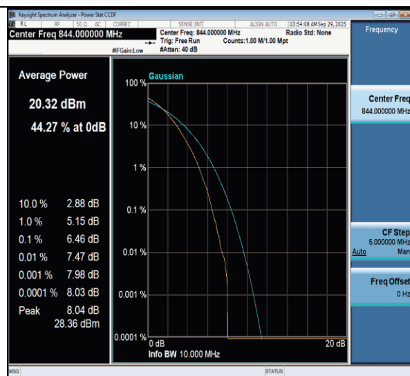
NTNV-n26(824-849)-PC3-15-10-H-DFT-256QAM-Outer_Full-PASS
