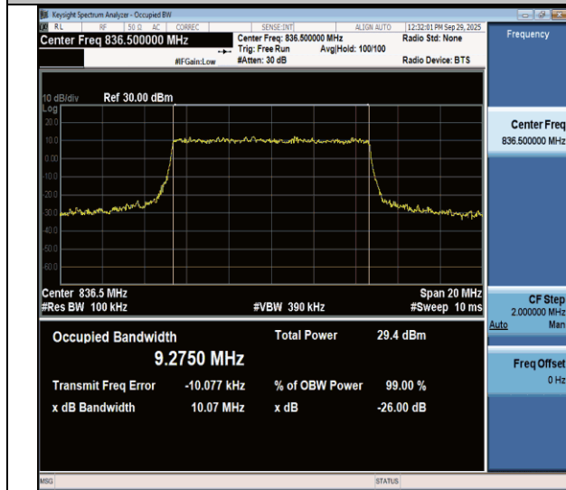
NTVN-n26(824-849)-PC3-15-10-M-CP-16QAM-Outet_Full-Ant1-PASS
