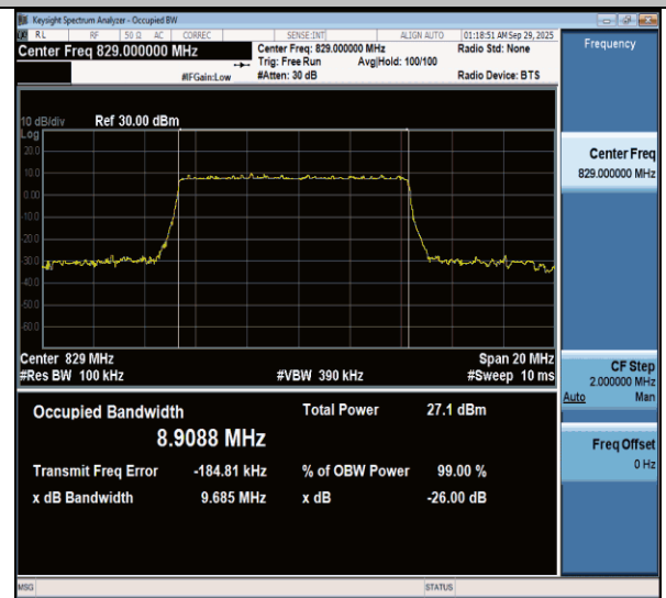
NTNV-n26(824-849)-PC3-15-10-L-DFT-256QAM-Outet_Full-Ant1- PASS
