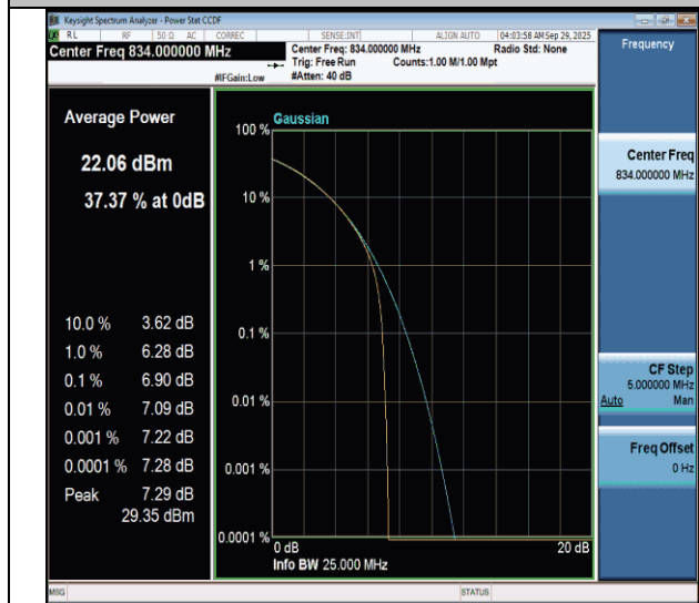
NTVN-n26(824-849)-PC3-15-20-L-CP-QPSK-Outer_Full-PASS
