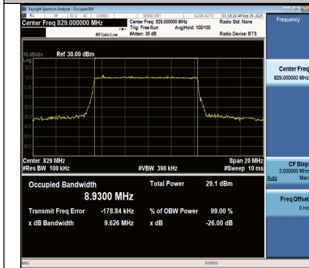
NTNV-n26(824-849)-PC3-15-10-L-DFT-64QAM-Outet_Full-Ant1- PASS
