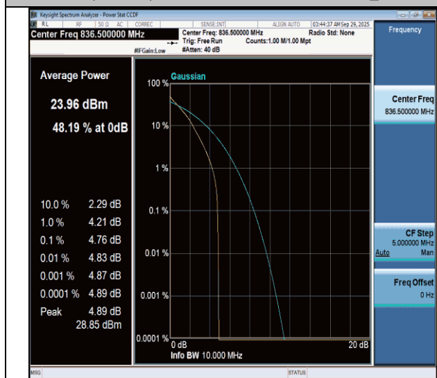
NTNV-n26(824-849)-PC3-15-5-M-CP-QPSK-Outer_Full-PASS
