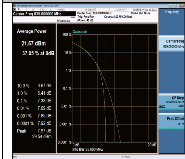
NTNV-n26(824-849)-PC3-15-20-H-CP-64QAM-Outer_Full-PASS
