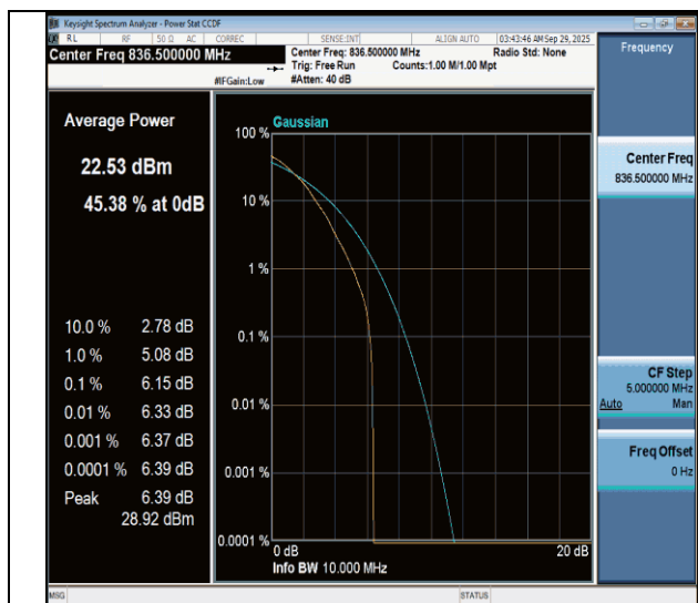
NTNV-n26(824-849)-PC3-15-5-M-DFT-64QAM-Outer_Full-PASS
