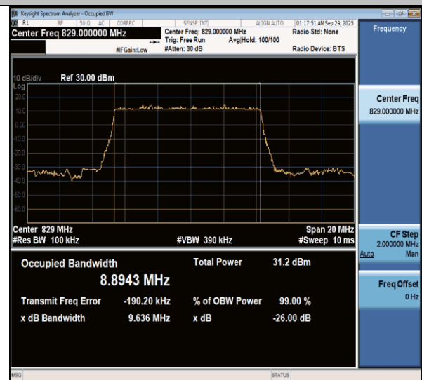
NTNV-n26(824-849)-PC3-15-10-L-DFT-BPSK-Outer_Full-Ant1- PASS
