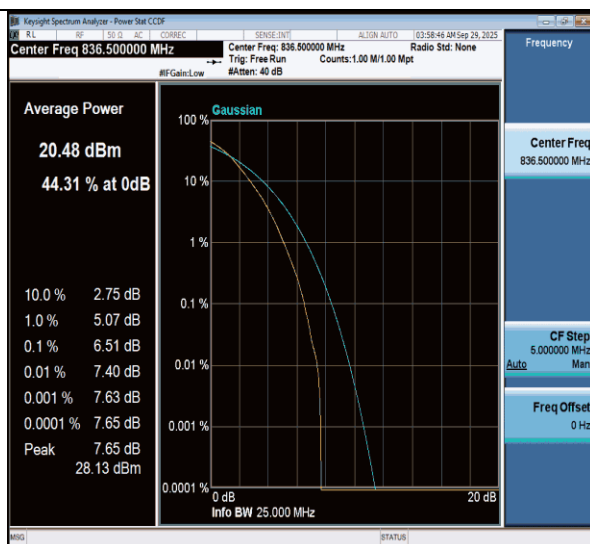
NTNV-n26(824-849)-PC3-15-15-M-DFT-256QAM-Outer_Full-PASS
