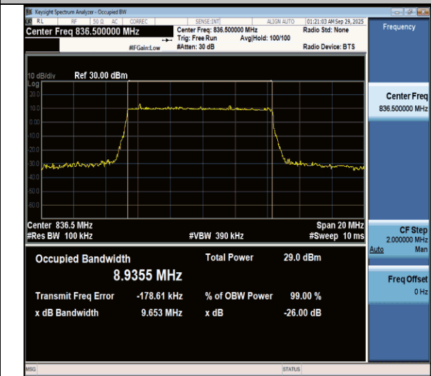
NTNV-n26(824-849)-PC3-15-10-M-DFT-64QAM-Outer_Full-Ant1- PASS
