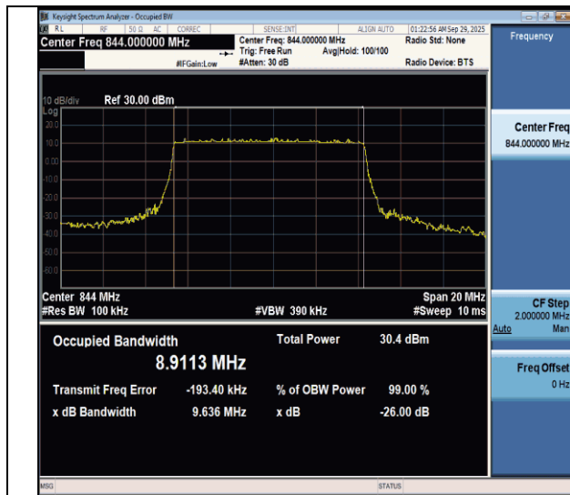
NTNV-n26(824-849)-PC3-15-10-H-DFT-QPSK-Outet_Full-Ant1- PASS
