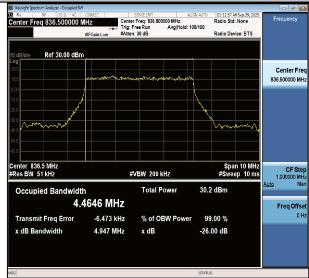
NTNV-n26(824-849)-PC3-15-5-M-DFT-BPSK-Outet_Full-Ant1- PASS
