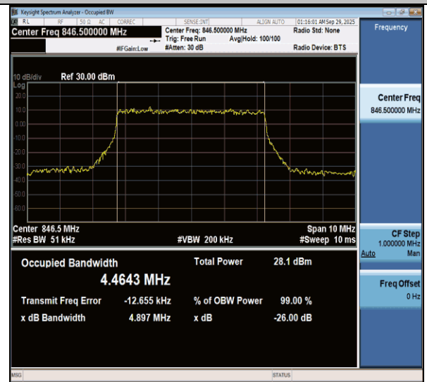
NTNV-n26(824-849)-PC3-15-5-H-DFT-64QAM-Outet_Full-Ant1- PASS
