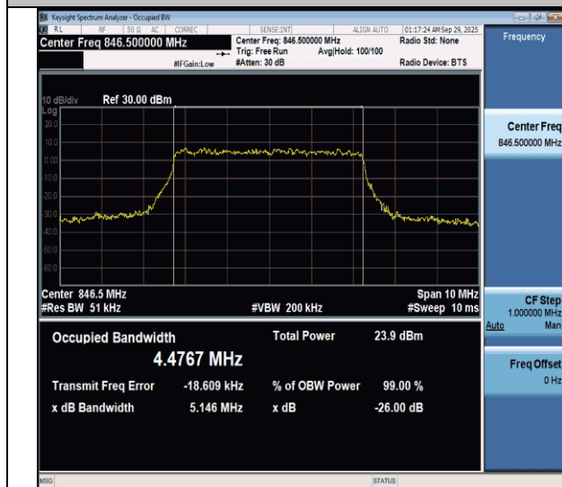
NTNV-n26(824-849)-PC3-15-5-H-CP-256QAM-Outer_Full-Ant1- PASS
