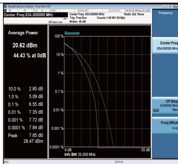
NTVN-n26(824-849)-PC3-15-20-L-DFT-256QAM-Outer_Full-PASS
