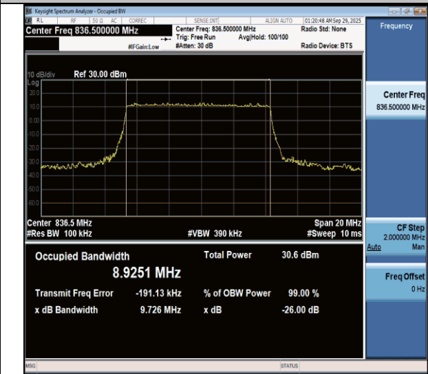
NTNV-n26(824-849)-PC3-15-10-M-DFT-QPSK-Outer_Full-Ant1- PASS
