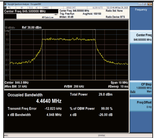
NTNV-n26(824-849)-PC3-15-5-H-DFT-QPSK-Outet_Full-Ant1- PASS
