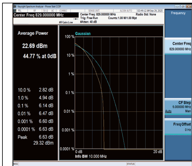
NTNV-n26(824-849)-PC3-15-10-L-DFT-64QAM-Outer_Full-PASS
