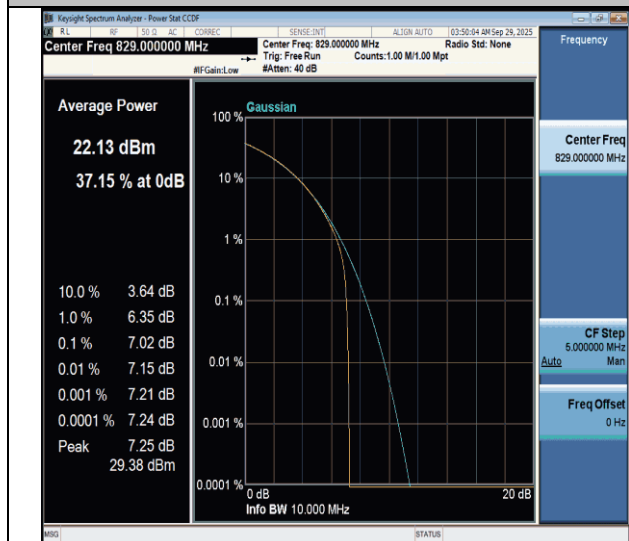
NTNV-n26(824-849)-PC3-15-10-L-CP-QPSK-Outer_Full-PASS
