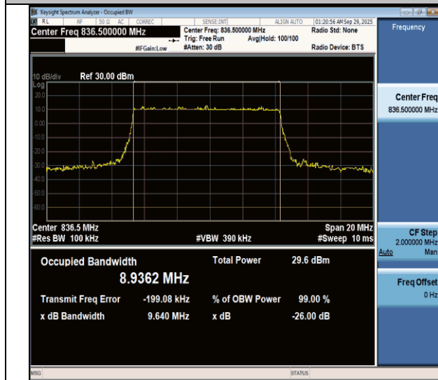
NTNV-n26(824-849)-PC3-15-10-M-DFT-16QAM-Outer_Full-Ant1- PASS
