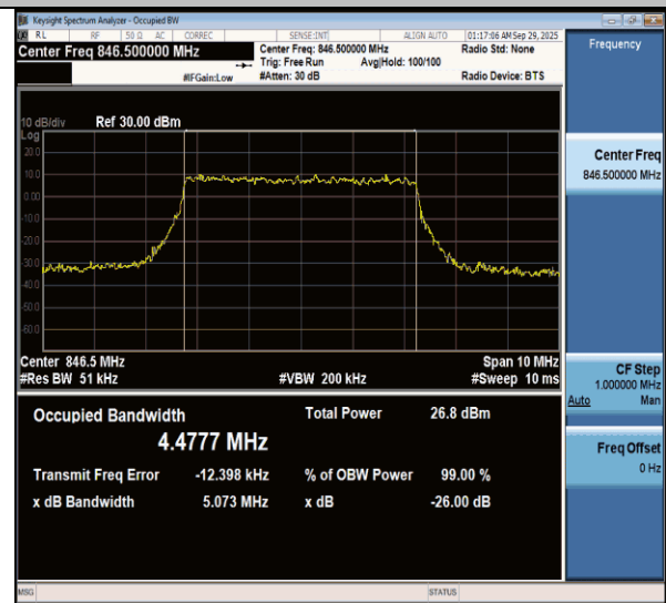
NTNV-n26(824-849)-PC3-15-5-H-CP-64QAM-Outer_Full-Ant1- PASS
