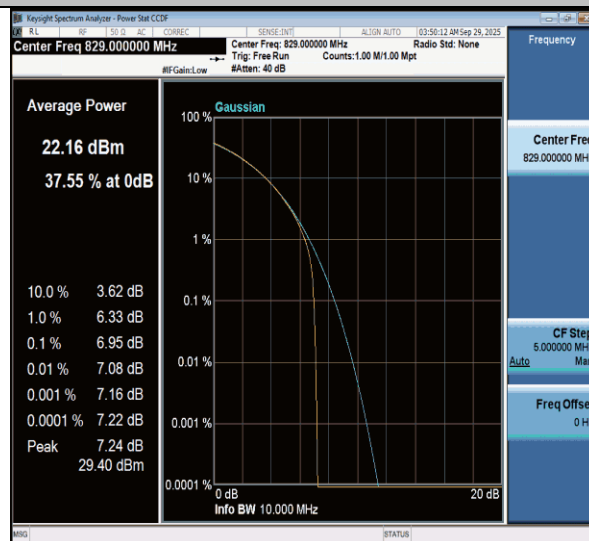
NTNV-n26(824-849)-PC3-15-10-L-CP-16QAM-Outer_Full-PASS
