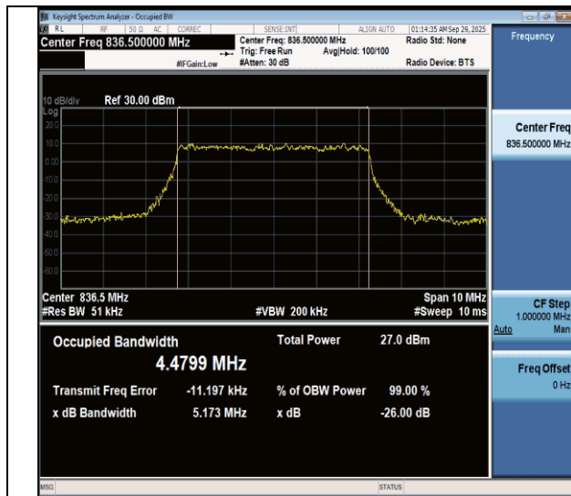
NTNV-n26(824-849)-PC3-15-5-M-CP-64QAM-Outet_Full-Ant1- PASS
