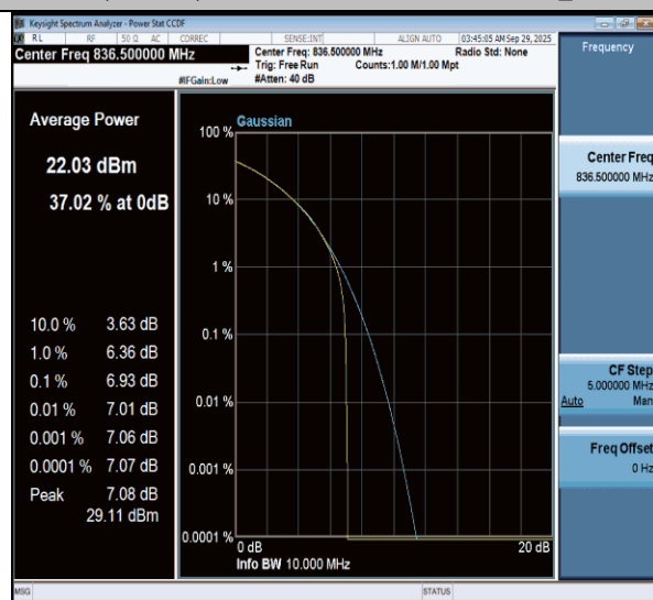
NTNV-n26(824-849)-PC3-15-5-M-CP-16QAM-Outer_Full-PASS
