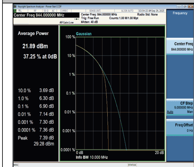
NTNV-n26(824-849)-PC3-15-10-H-CP-QPSK-Outer_Full-PASS
