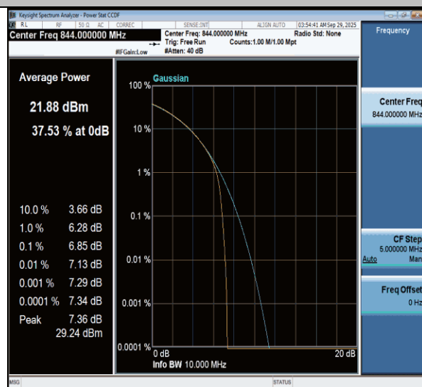
NTNV-n26(824-849)-PC3-15-10-H-CP-16QAM-Outer_Full-PASS
