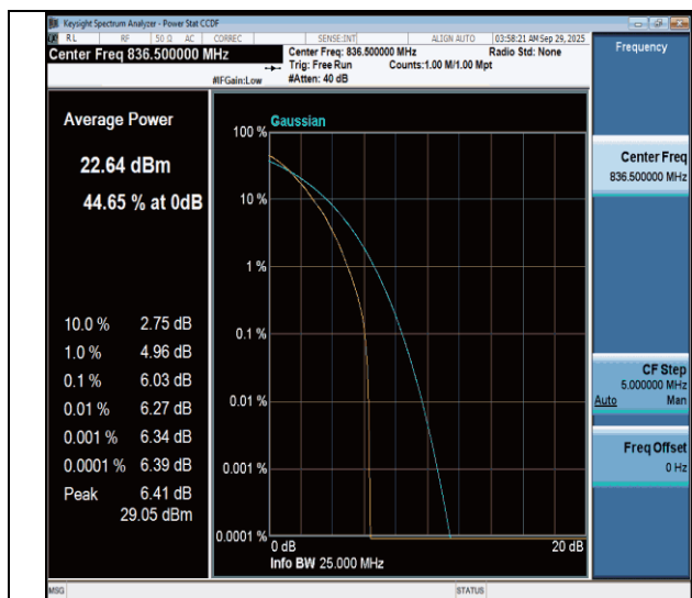
NTNV-n26(824-849)-PC3-15-15-M-DFT-64QAM-Outer_Full-PASS
