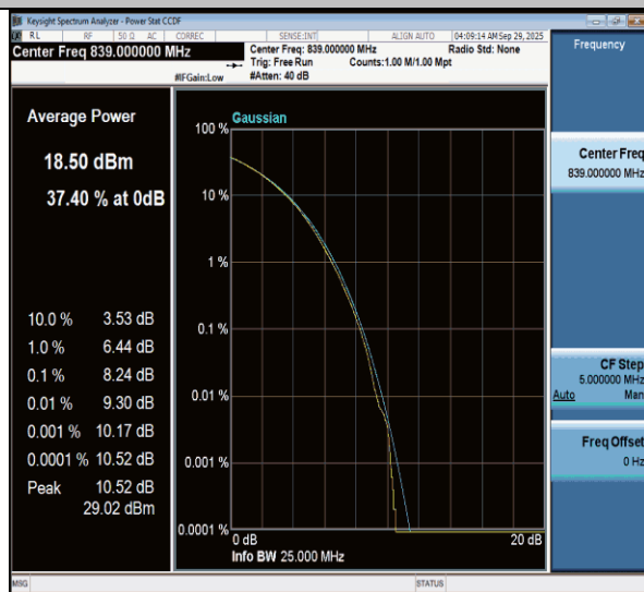
NTNV-n26(824-849)-PC3-15-20-H-CP-256QAM-Outer_Full-PASS
