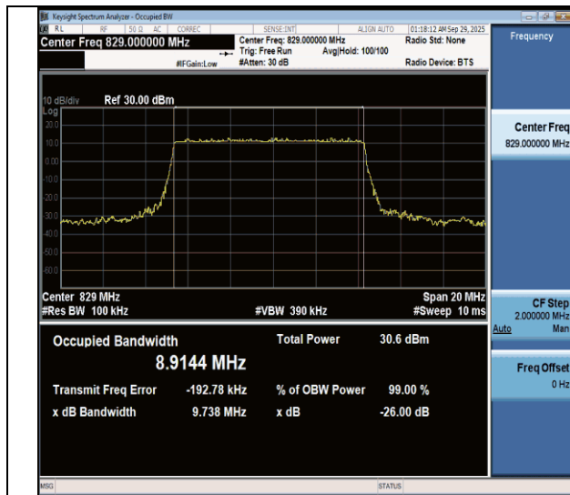
NTNV-n26(824-849)-PC3-15-10-L-DFT-QPSK-Outet_Full-Ant1- PASS
