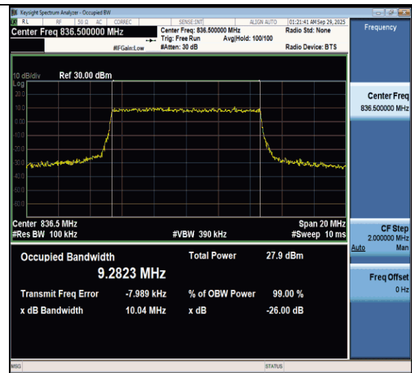
NTVN-n26(824-849)-PC3-15-10-M-CP-QPSK-Outet_Full-Ant1-PASS
