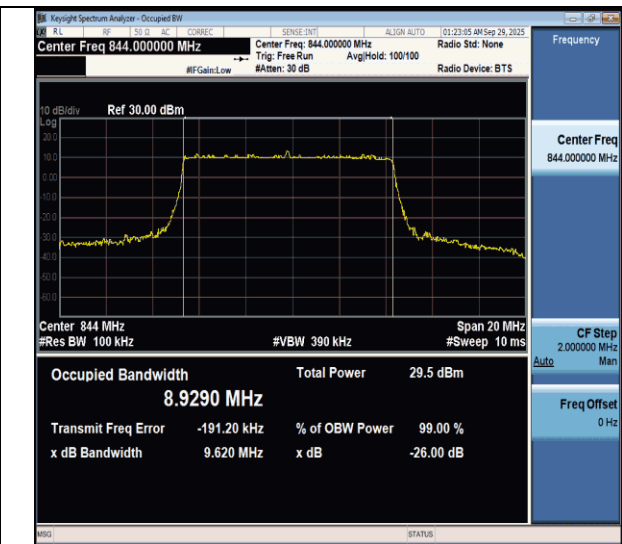
NTNV-n26(824-849)-PC3-15-10-H-DFT-16QAM-Outet_Full-Ant1- PASS
