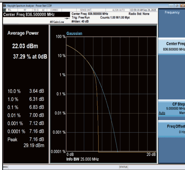
NTNV-n26(824-849)-PC3-15-15-M-CP-16QAM-Outer_Full-PASS
