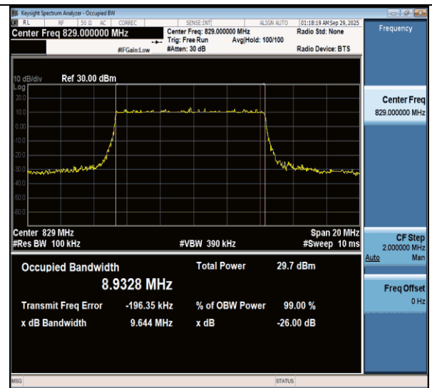
NTNV-n26(824-849)-PC3-15-10-L-DFT-16QAM-Outet_Full-Ant1- PASS
