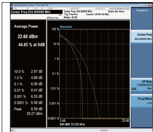
NTVN-n26(824-849)-PC3-15-20-L-DFT-64QAM-Outer_Full-PASS
