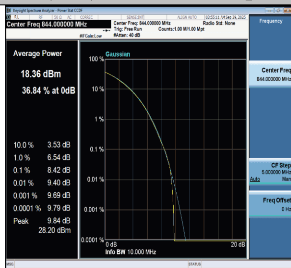
NTNV-n26(824-849)-PC3-15-10-H-CP-256QAM-Outer_Full-PASS
