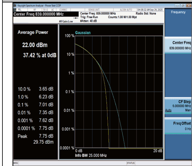
NTNV-n26(824-849)-PC3-15-20-H-CP-QPSK-Outer_Full-PASS
