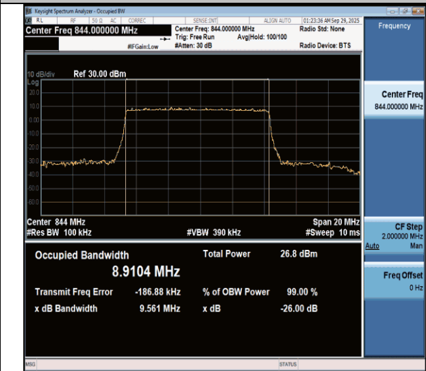
NTNV-n26(824-849)-PC3-15-10-H-DFT-256QAM-Outet_Full-Ant1-PASS
