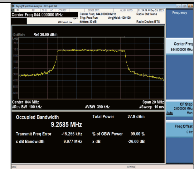
NTNV-n26(824-849)-PC3-15-10-H-CP-16QAM-Outet_Full-Ant1- PASS
