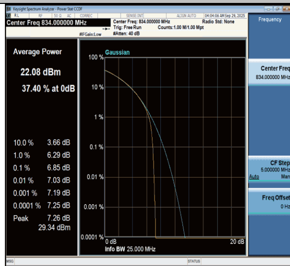
NTVN-n26(824-849)-PC3-15-20-L-CP-16QAM-Outer_Full-PASS
