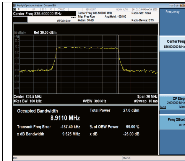
NTVN-n26(824-849)-PC3-15-10-M-DFT-256QAM-Outet_Full-Ant1-PASS
