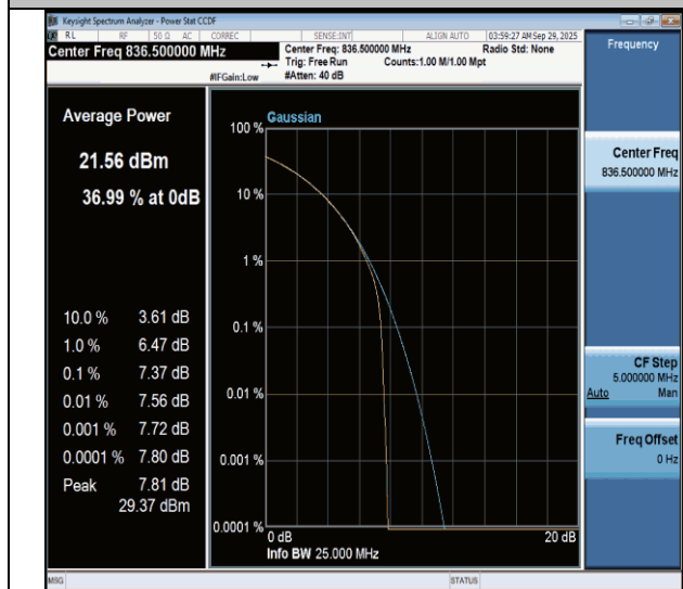
NTNV-n26(824-849)-PC3-15-15-M-CP-64QAM-Outer_Full-PASS
