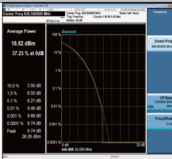
NTNV-n26(824-849)-PC3-15-15-M-CP-256QAM-Outer_Full-PASS
