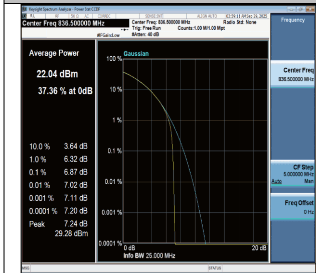
NTNV-n26(824-849)-PC3-15-15-M-CP-QPSK-Outer_Full-PASS
