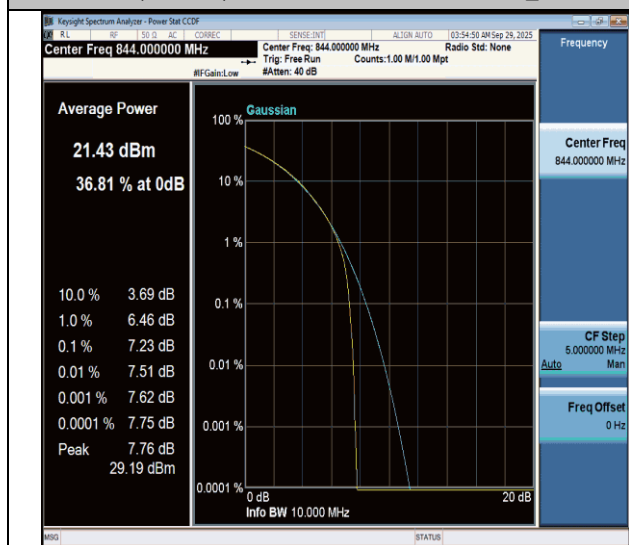
NTNV-n26(824-849)-PC3-15-10-H-CP-64QAM-Outer_Full-PASS
