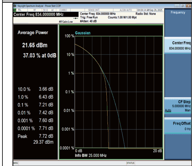
NTVN-n26(824-849)-PC3-15-20-L-CP-64QAM-Outer_Full-PASS
