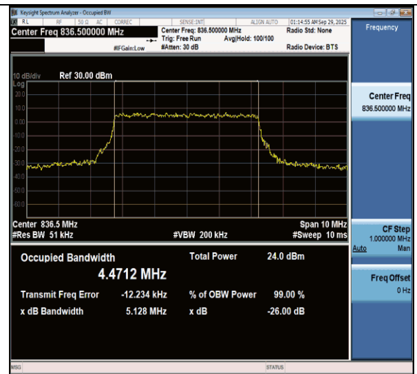
NTNV-n26(824-849)-PC3-15-5-M-CP-256QAM-Outet_Full-Ant1- PASS
