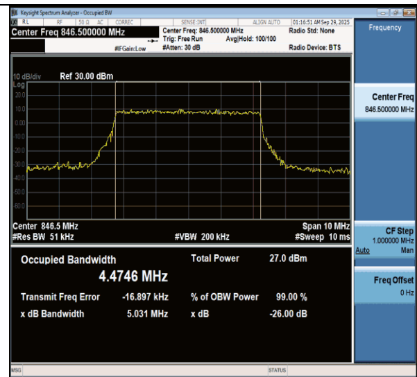
NTNV-n26(824-849)-PC3-15-5-H-CP-QPSK-Outer_Full-Ant1- PASS
