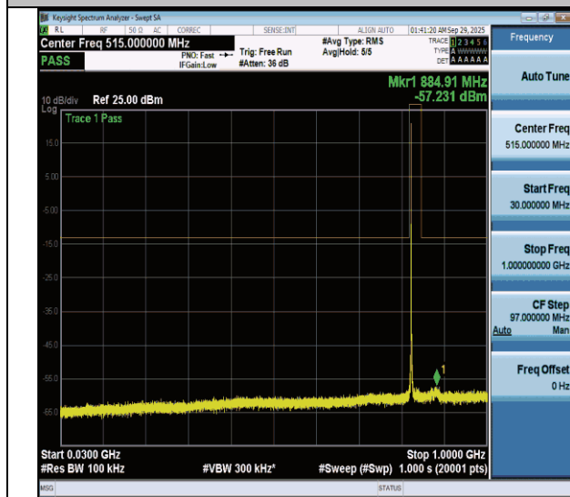
NTNV-n26(824-849)-PC3-15-20-M-DFT-BPSK-Edge_1RB_Left- 30-1000-PASS
