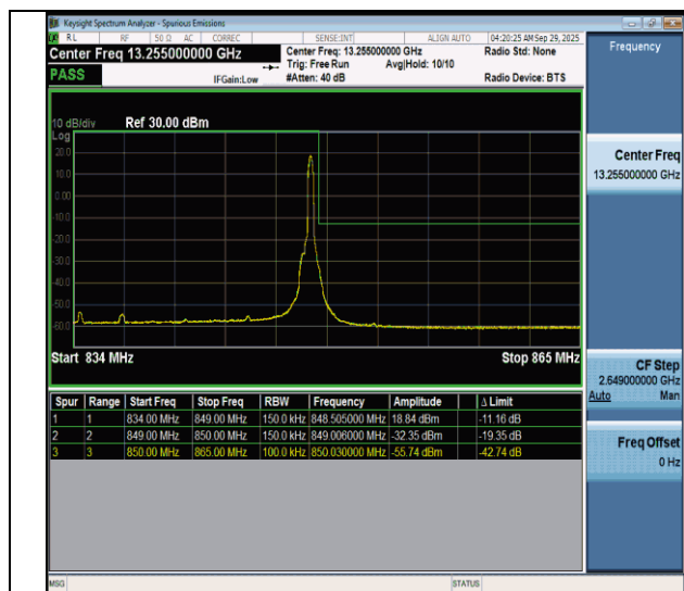
NTNV-n26(824-849)-PC3-15-15-H-CP-QPSK-Edge_1RB_Right-PASS
