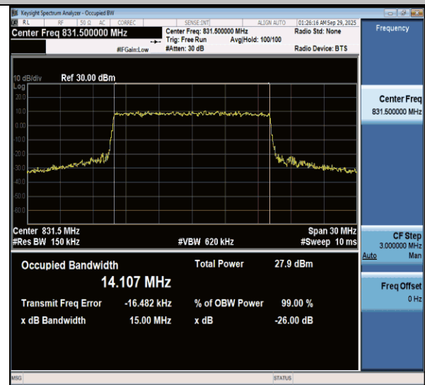
NTNV-n26(824-849)-PC3-15-15-L-CP-64QAM-Outer_Full-Ant1- PASS
