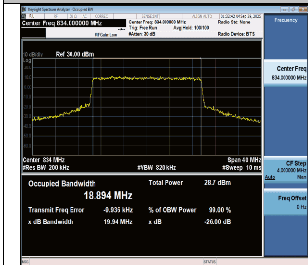
NTNV-n26(824-849)-PC3-15-20-L-CP-QPSK-Outet_Full-Ant1- PASS
