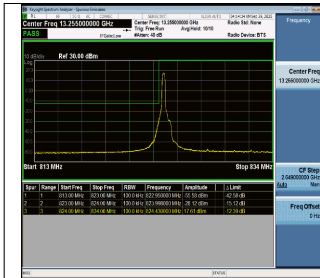
NTNV-n26(824-849)-PC3-15-10-L-CP-QPSK-Edge_1RB_Left-PASS
