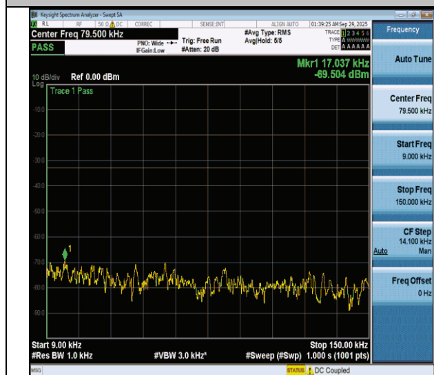
NTNV-n26(824-849)-PC3-15-20-L-CP-QPSK-Edge_1RB_Left- 0.009-0.15-PASS
