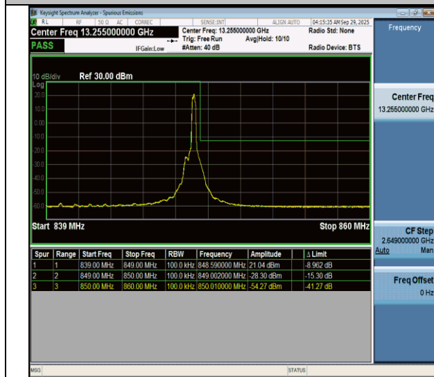
NTNV-n26(824-849)-PC3-15-10-H-DFT-BPSK-Edge_1RB_Right-PASS
