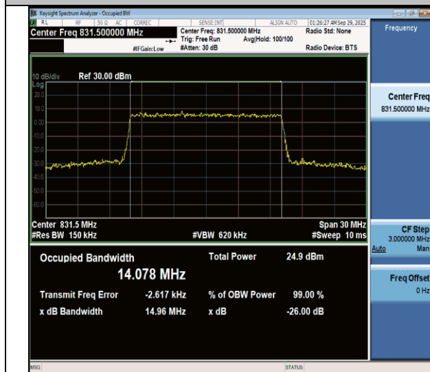
NTNV-n26(824-849)-PC3-15-15-L-CP-256QAM-Outer_Full-Ant1- PASS
