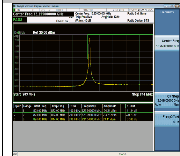
NTNV-n26(824-849)-PC3-15-20-L-DFT-BPSK-Edge_1RB_Left-PASS
