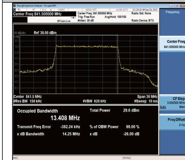
NTNV-n26(824-849)-PC3-15-15-H-DFT-16QAM-Outer_Full-Ant1- PASS
