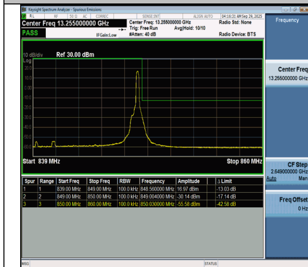
NTNV-n26(824-849)-PC3-15-10-H-CP-QPSK-Edge_1RB_Right-PASS
