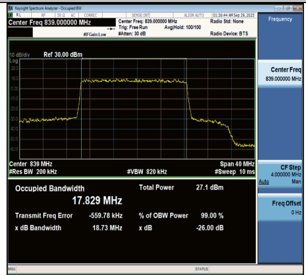
NTNV-n26(824-849)-PC3-15-20-H-DFT-256QAM-Outet_Full-Ant1-PASS
