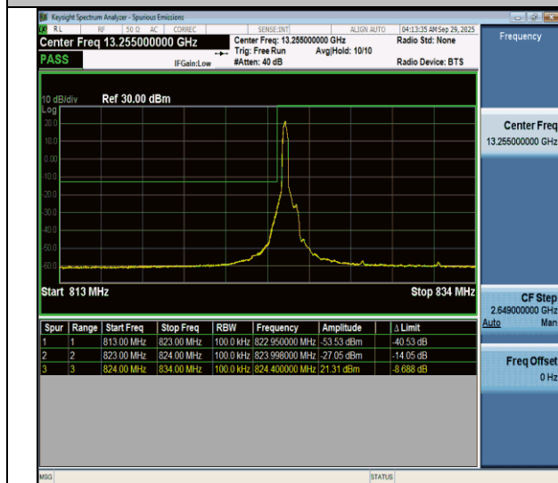
NTVN-n26(824-849)-PC3-15-10-L-DFT-BPSK-Edge_1RB_Left-PASS
