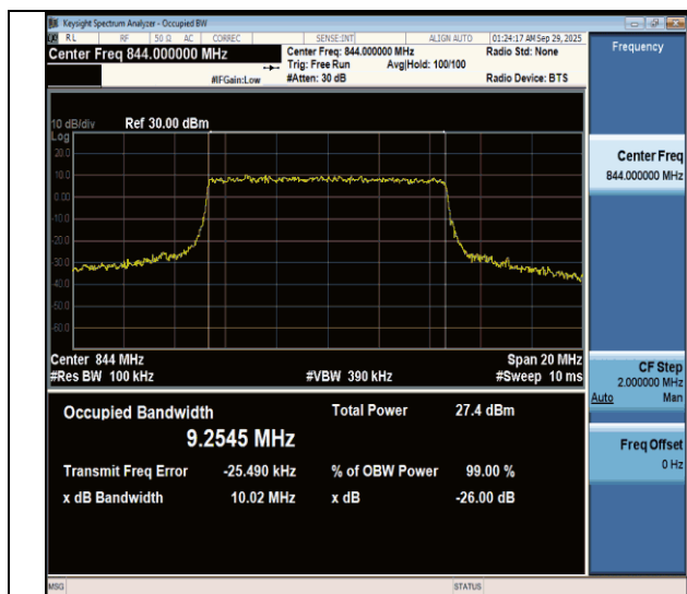
NTNV-n26(824-849)-PC3-15-10-H-CP-64QAM-Outer_Full-Ant1- PASS
