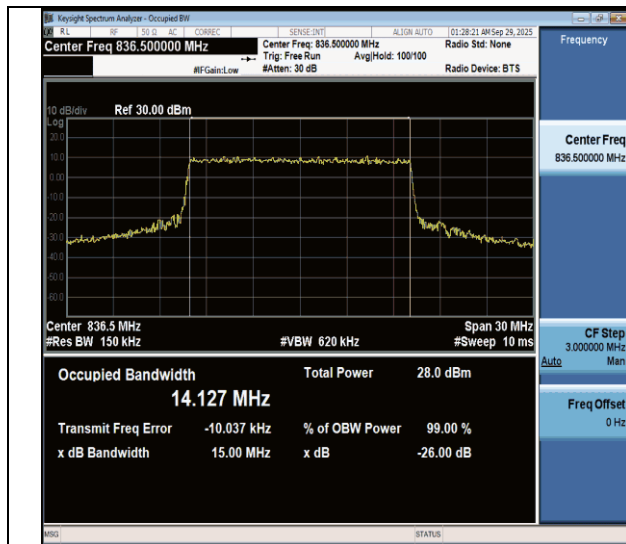
NTNV-n26(824-849)-PC3-15-15-M-CP-64QAM-Outer_Full-Ant1- PASS
