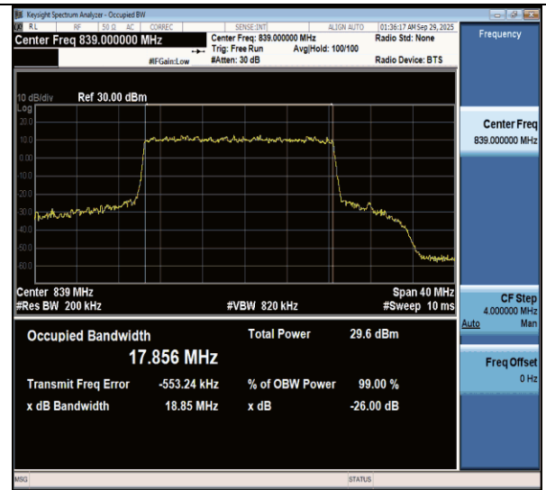
NTNV-n26(824-849)-PC3-15-20-H-DFT-16QAM-Outet_Full-Ant1- PASS
