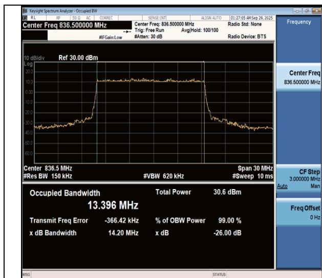
NTNV-n26(824-849)-PC3-15-15-M-DFT-QPSK-Outet_Full-Ant1- PASS
