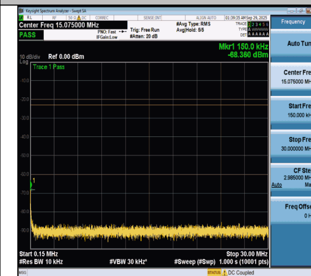
NTNV-n26(824-849)-PC3-15-20-L-CP-QPSK-Edge_1RB_Left- 0.15-30-PASS
