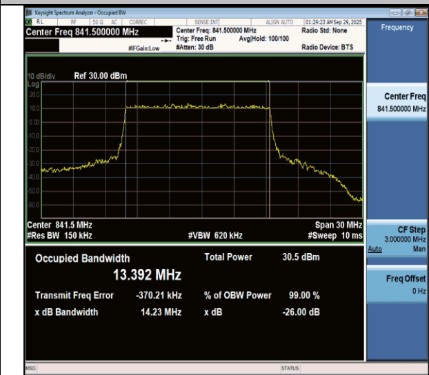
NTNV-n26(824-849)-PC3-15-15-H-DFT-QPSK-Outer_Full-Ant1- PASS
