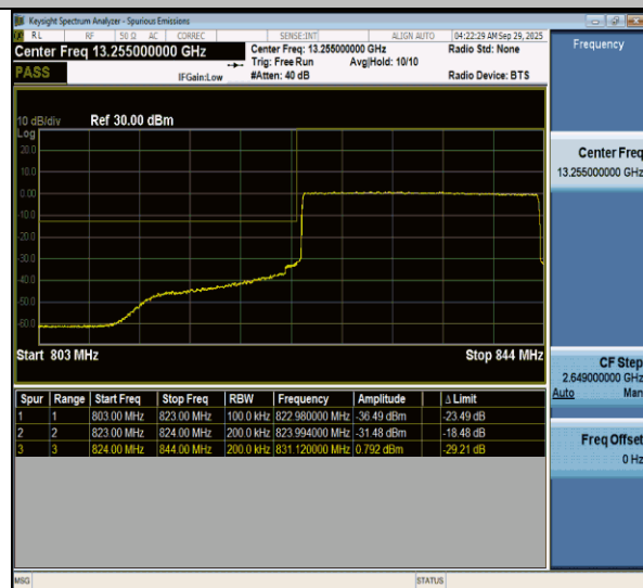
NTNV-n26(824-849)-PC3-15-20-L-CP-QPSK-Outer_Full-PASS
