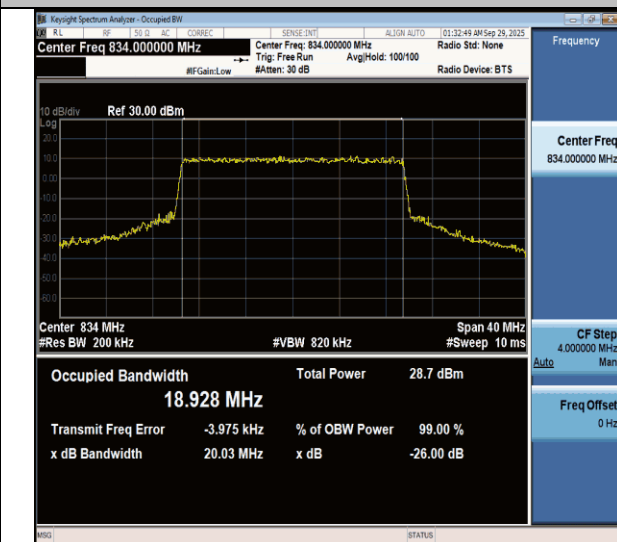
NTNV-n26(824-849)-PC3-15-20-L-CP-16QAM-Outet_Full-Ant1- PASS
