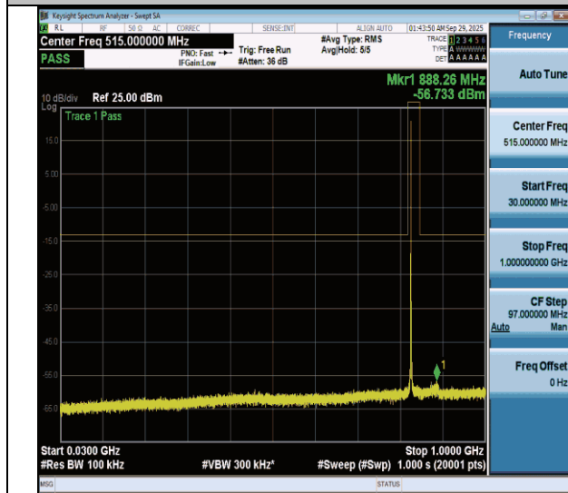
NTNV-n26(824-849)-PC3-15-20-H-DFT-BPSK-Edge_1RB_Left- 30-1000-PASS
