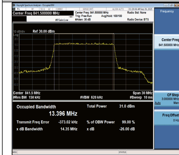
NTNV-n26(824-849)-PC3-15-15-H-DFT-BPSK-Outer_Full-Ant1- PASS
