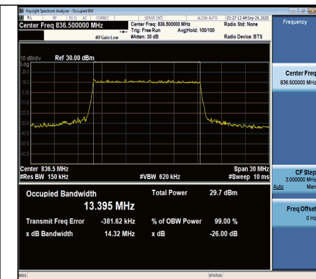
NTNV-n26(824-849)-PC3-15-15-M-DFT-16QAM-Outet_Full-Ant1- PASS
