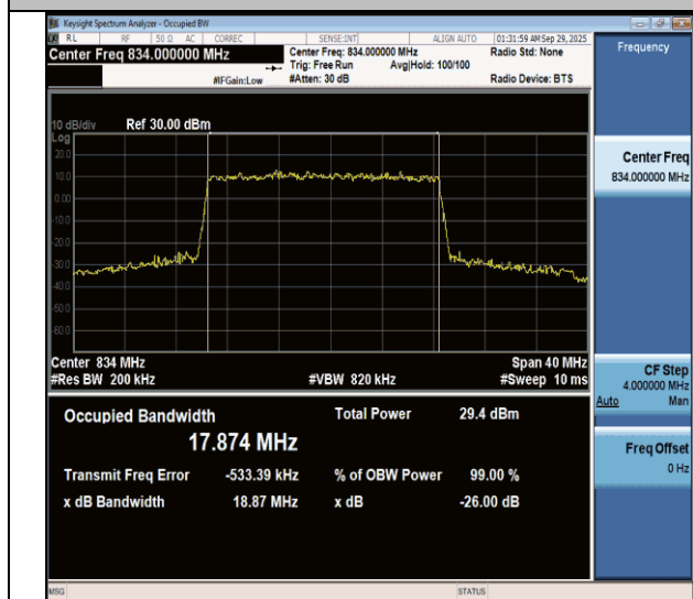
NTNV-n26(824-849)-PC3-15-20-L-DFT-64QAM-Outet_Full-Ant1- PASS
