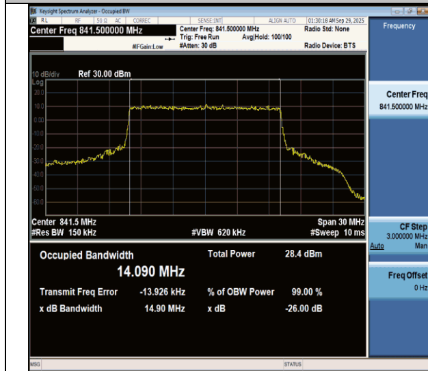
NTVN-n26(824-849)-PC3-15-15-H-CP-16QAM-Outet_Full-Ant1-PASS
