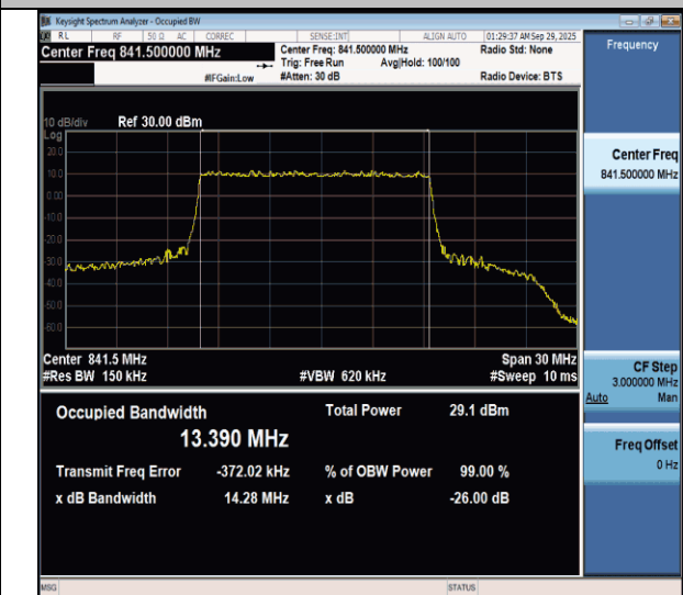
NTNV-n26(824-849)-PC3-15-15-H-DFT-64QAM-Outer_Full-Ant1- PASS
