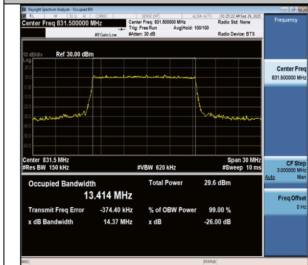
NTNV-n26(824-849)-PC3-15-15-L-DFT-16QAM-Outer_Full-Ant1- PASS
