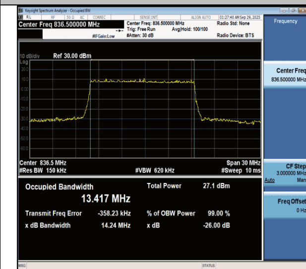
NTNV-n26(824-849)-PC3-15-15-M-DFT-256QAM-Outet_Full-Ant1-PASS
