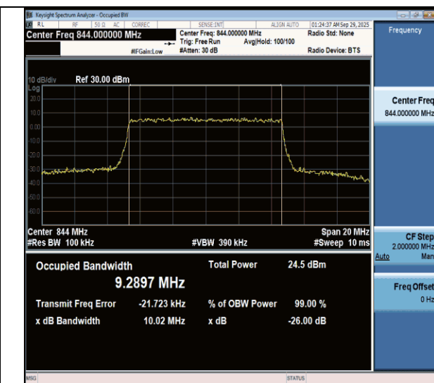
NTNV-n26(824-849)-PC3-15-10-H-CP-256QAM-Outer_Full-Ant1- PASS
