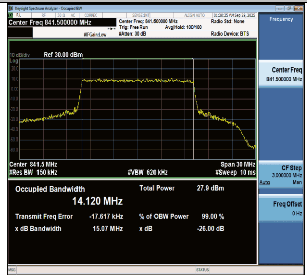
NTVN-n26(824-849)-PC3-15-15-H-CP-64QAM-Outet_Full-Ant1-PASS
