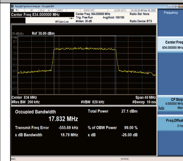
NTNV-n26(824-849)-PC3-15-20-L-DFT-256QAM-Outet_Full-Ant1- PASS
