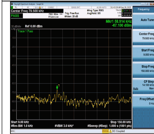
NTNV-n26(824-849)-PC3-15-20-H-DFT-BPSK-Edge_1RB_Left- 0.009-0.15-PASS
