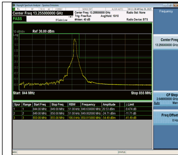
NTVN-n26(824-849)-PC3-15-5-H-DFT-BPSK-Edge_1RB_Right-PASS
