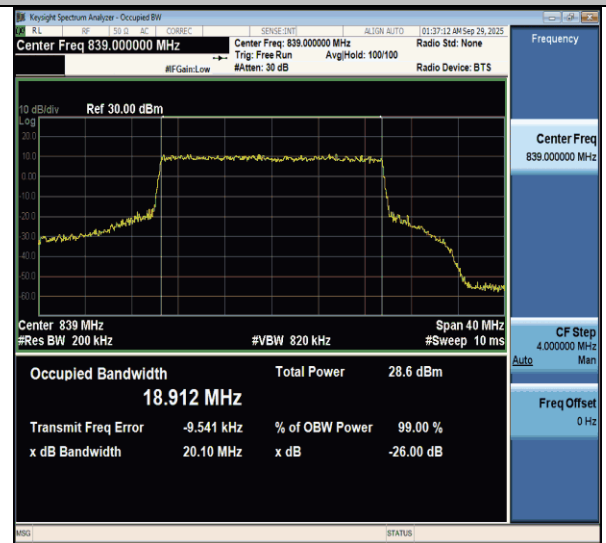
NTNV-n26(824-849)-PC3-15-20-H-CP-16QAM-Outet_Full-Ant1- PASS
