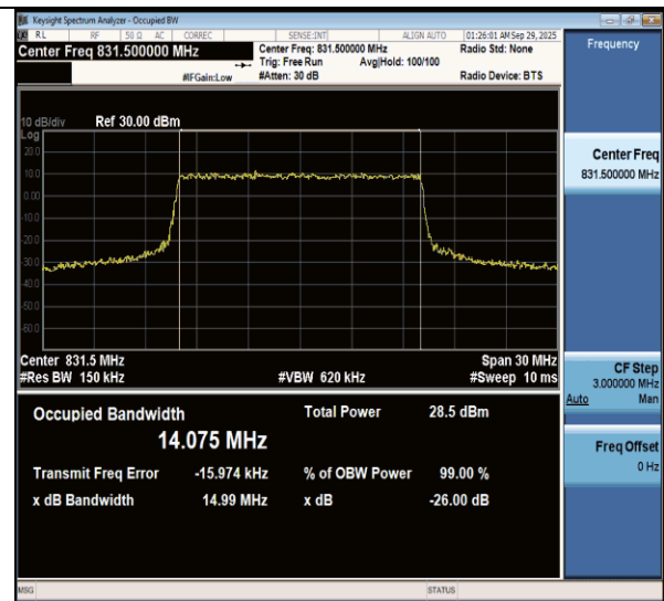
NTNV-n26(824-849)-PC3-15-15-L-CP-QPSK-Outer_Full-Ant1- PASS
