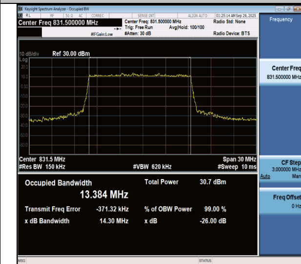
NTNV-n26(824-849)-PC3-15-15-L-DFT-QPSK-Outer_Full-Ant1- PASS
