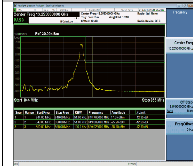
NTVN-n26(824-849)-PC3-15-5-H-CP-QPSK-Edge_1RB_Right-PASS
