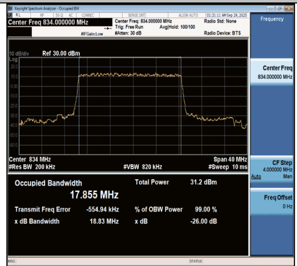
NTVN-n26(824-849)-PC3-15-20-L-DFT-BPSK-Outet_Full-Ant1-PASS
