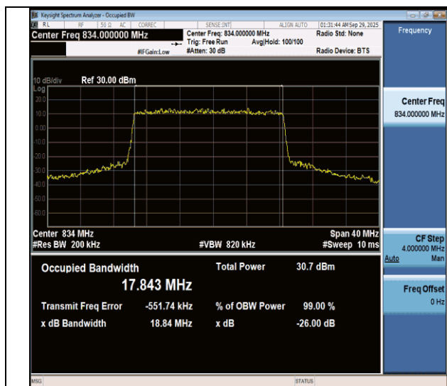
NTNV-n26(824-849)-PC3-15-20-L-DFT-QPSK-Outet_Full-Ant1- PASS
