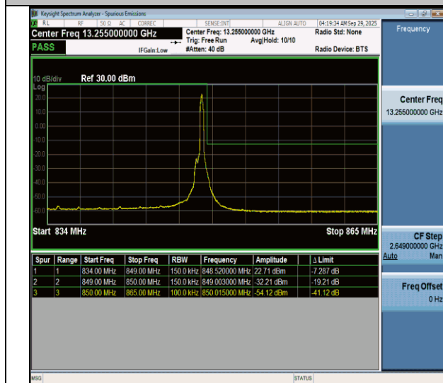
NTNV-n26(824-849)-PC3-15-15-H-DFT-BPSK-Edge_1RB_Right-PASS
