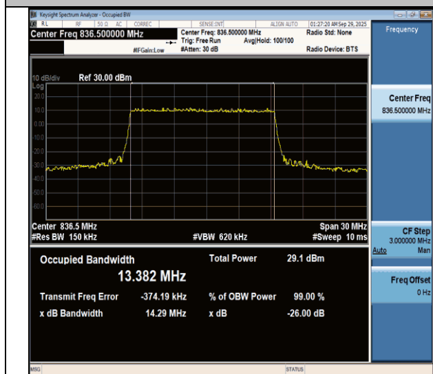
NTNV-n26(824-849)-PC3-15-15-M-DFT-64QAM-Outet_Full-Ant1- PASS
