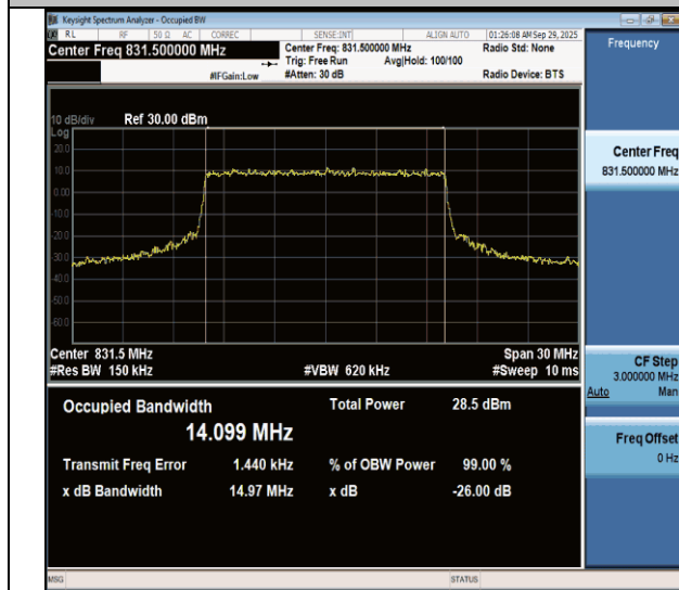
NTNV-n26(824-849)-PC3-15-15-L-CP-16QAM-Outer_Full-Ant1- PASS
