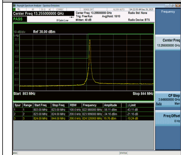
NTNV-n26(824-849)-PC3-15-20-L-CP-QPSK-Edge_1RB_Left-PASS
