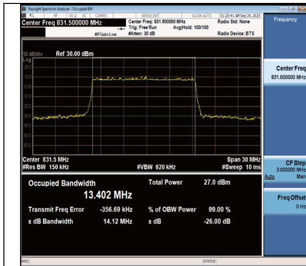
NTNV-n26(824-849)-PC3-15-15-L-DFT-256QAM-Outer_Full-Ant1- PASS
