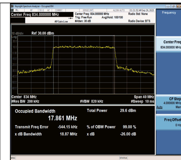
NTNV-n26(824-849)-PC3-15-20-L-DFT-16QAM-Outet_Full-Ant1- PASS
