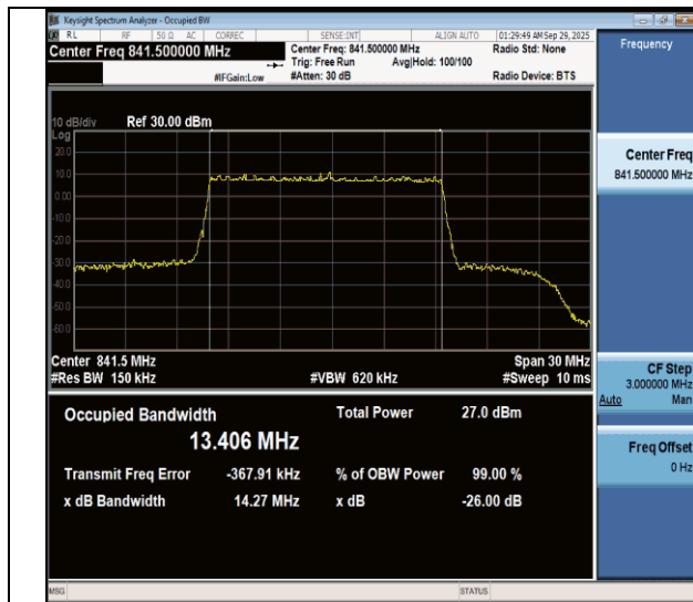
NTVN-n26(824-849)-PC3-15-15-H-DFT-256QAM-Outet_Full-Ant1-PASS
