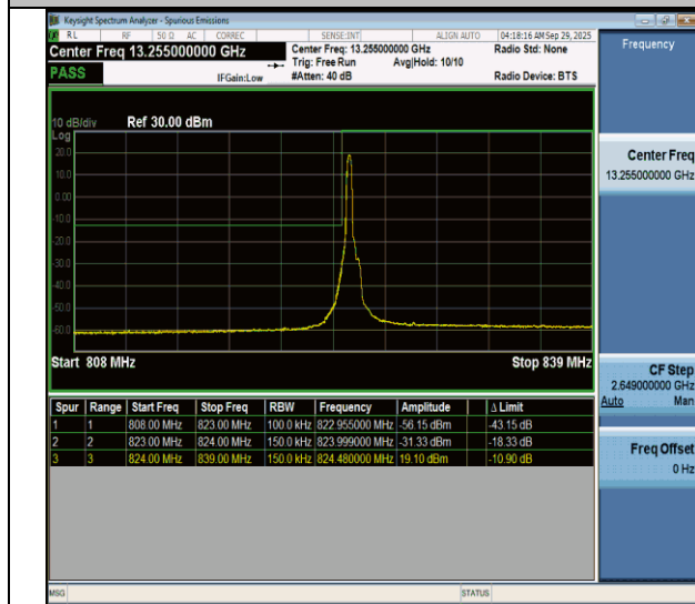
NTNV-n26(824-849)-PC3-15-15-L-CP-QPSK-Edge_1RB_Left-PASS
