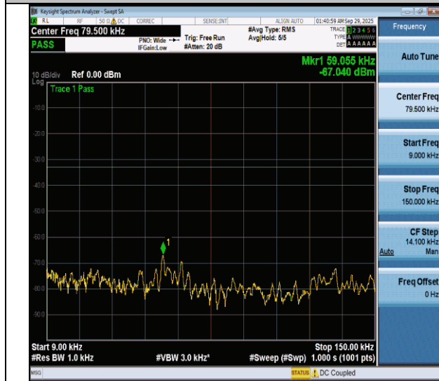
NTNV-n26(824-849)-PC3-15-20-M-DFT-BPSK-Edge_1RB_Left- 0.009-0.15-PASS
