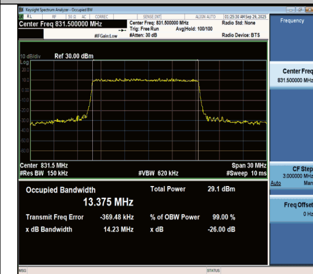
NTNV-n26(824-849)-PC3-15-15-L-DFT-64QAM-Outer_Full-Ant1- PASS
