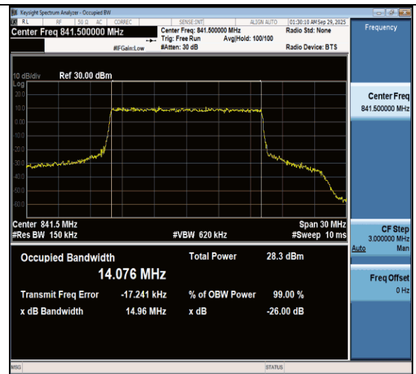
NTVN-n26(824-849)-PC3-15-15-H-CP-QPSK-Outet_Full-Ant1-PASS
