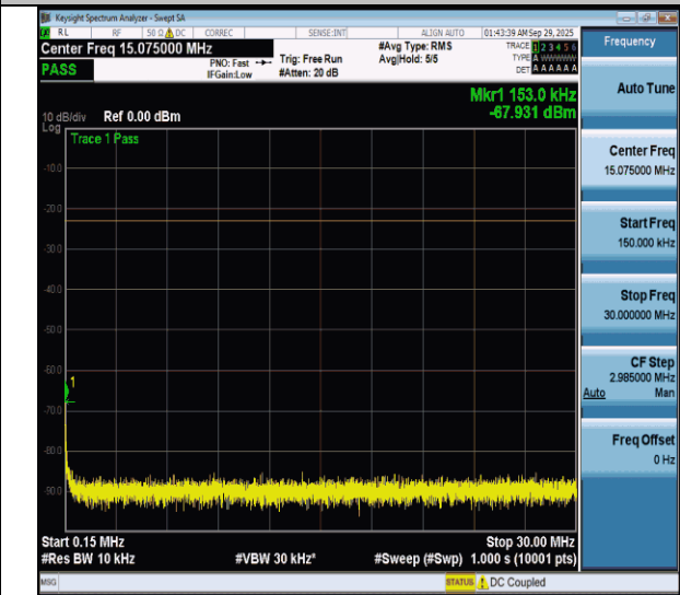
NTNV-n26(824-849)-PC3-15-20-H-DFT-BPSK-Edge_1RB_Left- 0.15-30-PASS
