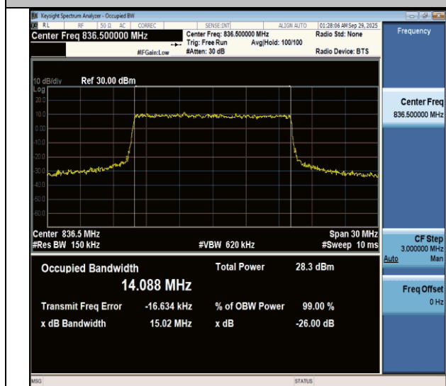
NTNV-n26(824-849)-PC3-15-15-M-CP-QPSK-Outet_Full-Ant1- PASS
