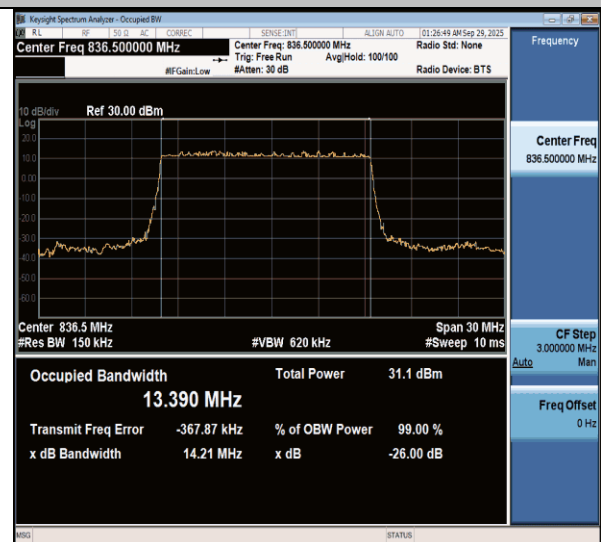
NTNV-n26(824-849)-PC3-15-15-M-DFT-BPSK-Outer_Full-Ant1- PASS
