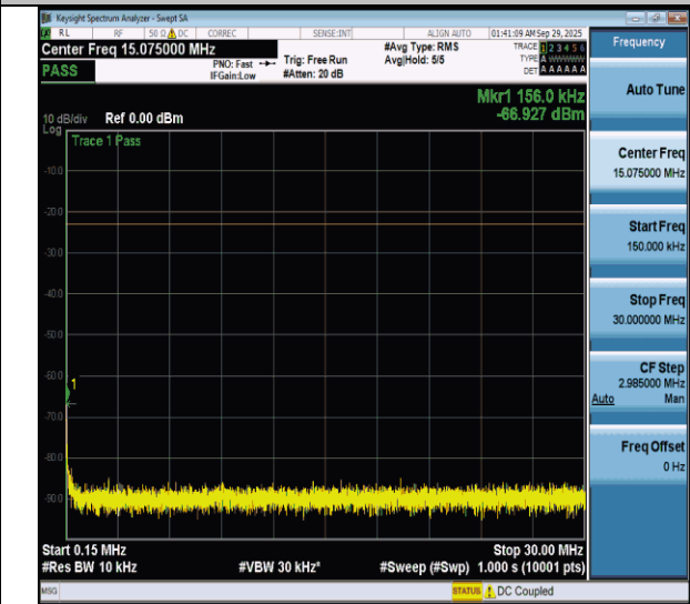
NTNV-n26(824-849)-PC3-15-20-M-DFT-BPSK-Edge_1RB_Left- 0.15-30-PASS
