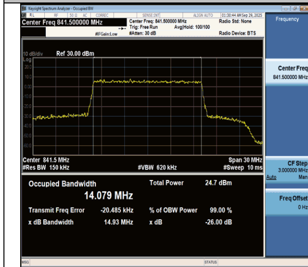
NTVN-n26(824-849)-PC3-15-15-H-CP-256QAM-Outet_Full-Ant1-PASS
