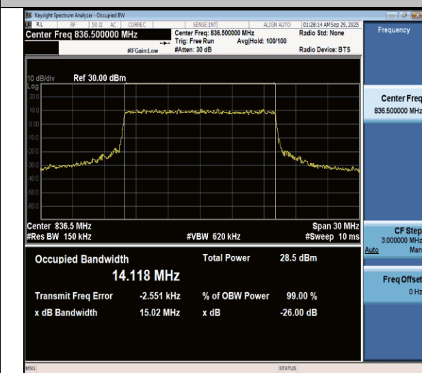
NTNV-n26(824-849)-PC3-15-15-M-CP-16QAM-Outet_Full-Ant1- PASS
