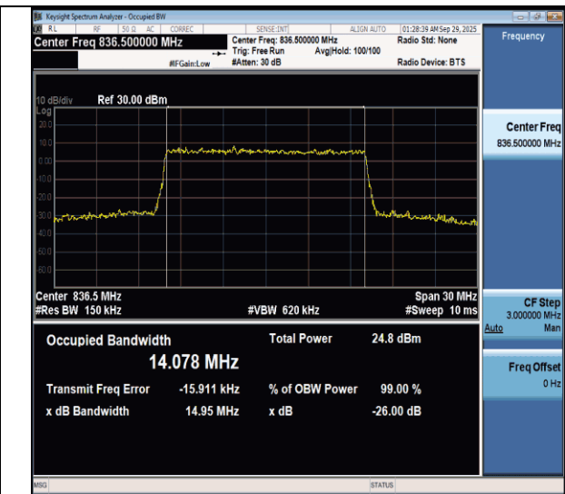
NTNV-n26(824-849)-PC3-15-15-M-CP-256QAM-Outer_Full-Ant1- PASS
