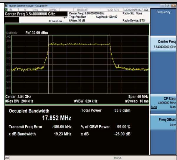
NTNV-n77(3450-3550)-PC3-30-20-H-DFT-64QAM-Outer_Full-Ant1-PASS
