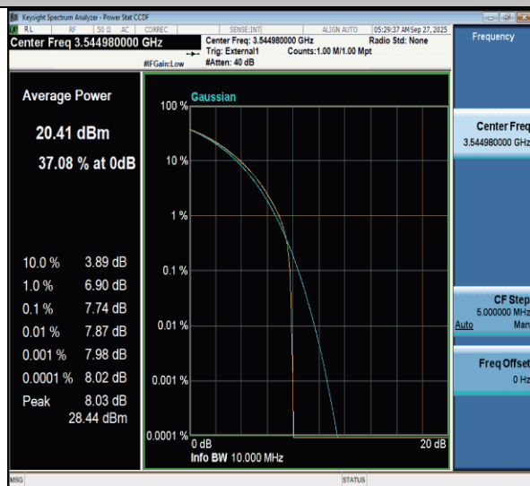
NTNV-n77(3450-3550)-PC3-30-10-H-CP-QPSK-Outter_Full-PASS
