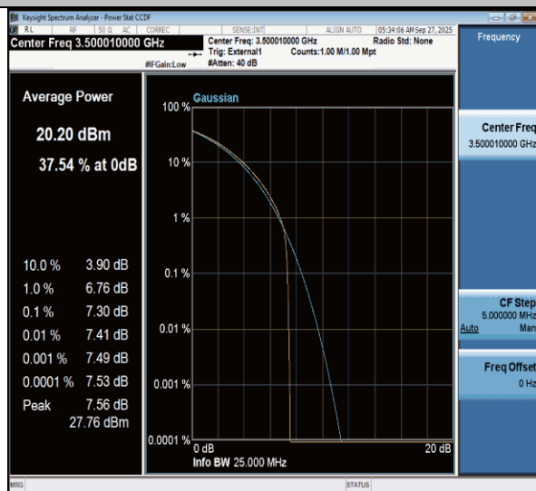
NTNV-n77(3450-3550)-PC3-30-15-M-CP-QPSK-Outter_Full-PASS
