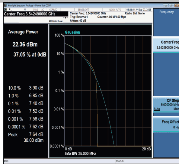
NTNV-n77(3450-3550)-PC3-30-15-H-CP-16QAM-Outter_Full-PASS
