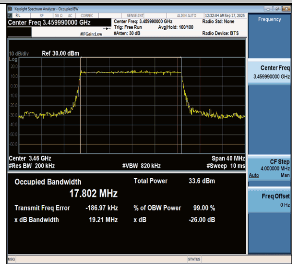
NTNV-n77(3450-3550)-PC3-30-20-L-DFT-QPSK-Outer_Full-Ant1-PASS
