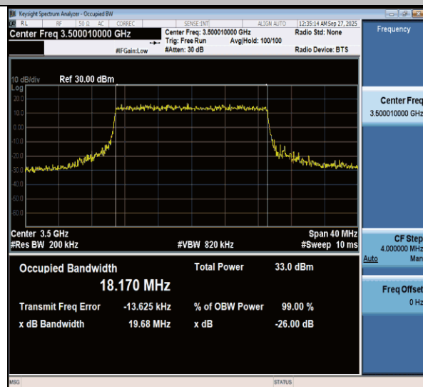
NTVN-n77(3450-3550)-PC3-30-20-M-CP-16QAM-Outter_Full-Ant1-PASS
