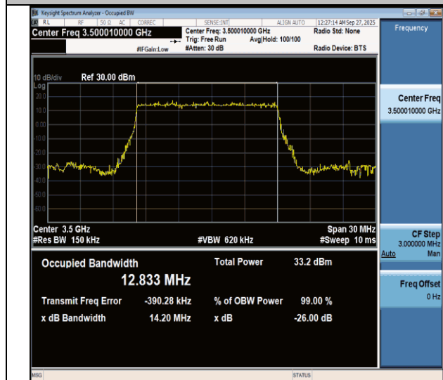
NTNV-n77(3450-3550)-PC3-30-15-M-DFT-BPSK-Outer_Full-Ant1- PASS
