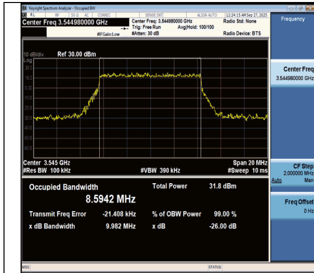
NTNV-n77(3450-3550)-PC3-30-10-H-DFT-256QAM-Outer_Full-Ant1-PASS
