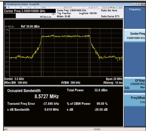
NTNV-n77(3450-3550)-PC3-30-10-M-DFT-BPSK-Outer_Full-Ant1-PASS
