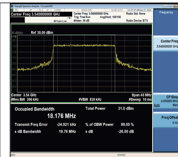
NTNV-n77(3450-3550)-PC3-30-20-H-CP-QPSK-Outer_Full-Ant1-PASS
