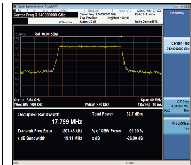
NTNV-n77(3450-3550)-PC3-30-20-H-DFT-256QAM-Outer_Full-Ant1-PASS
