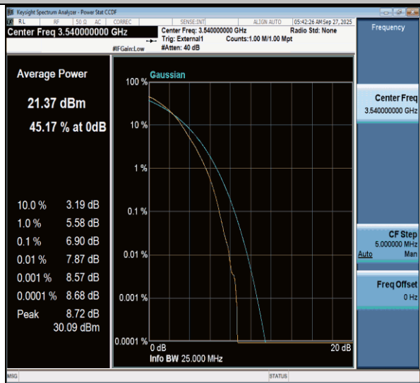
NTNV-n77(3450-3550)-PC3-30-20-H-DFT-256QAM-Outter_Full-PASS
