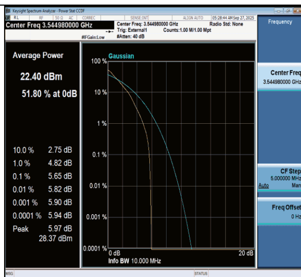
NTNV-n77(3450-3550)-PC3-30-10-H-DFT-QPSK-Outter_Full-PASS
