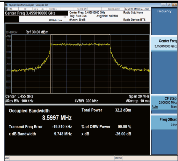
NTNV-n77(3450-3550)-PC3-30-10-L-CP-64QAM-Outer_Full-Ant1-PASS
