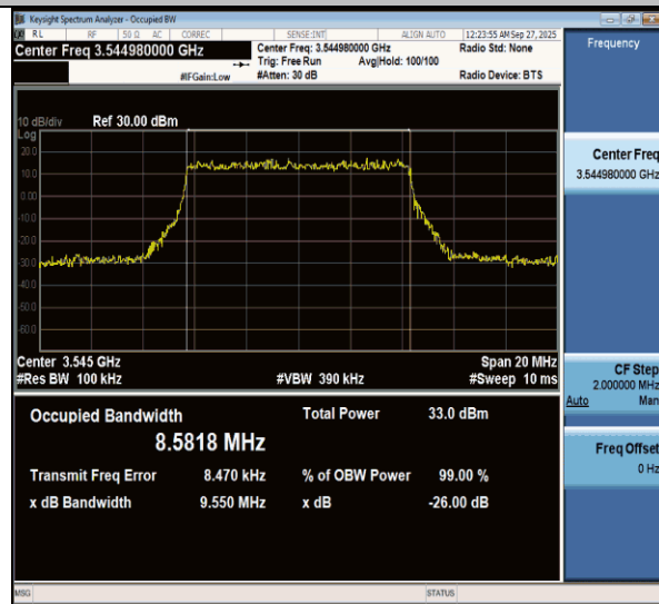
NTNV-n77(3450-3550)-PC3-30-10-H-DFT-64QAM-Outer_Full-Ant1-PASS
