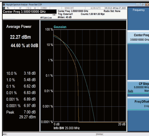
NTNV-n77(3450-3550)-PC3-30-15-M-DFT-64QAM-Outter_Full-PASS
