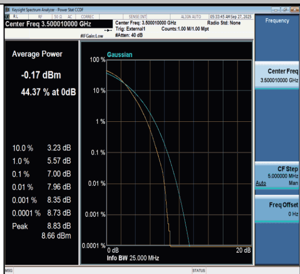
NTNV-n77(3450-3550)-PC3-30-15-M-DFT-256QAM-Outter_Full-PASS
