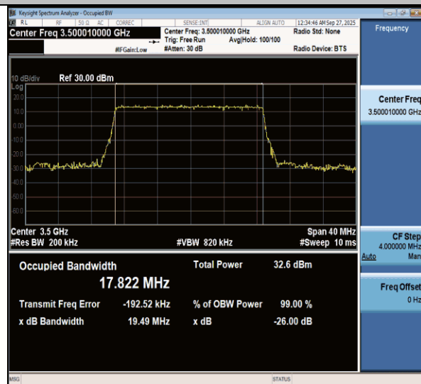
NTVN-n77(3450-3550)-PC3-30-20-M-DFT-256QAM-Outter_Full-Ant1-PASS
