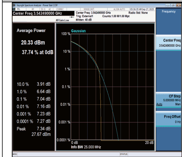
NTNV-n77(3450-3550)-PC3-30-15-H-CP-QPSK-Outter_Full-PASS
