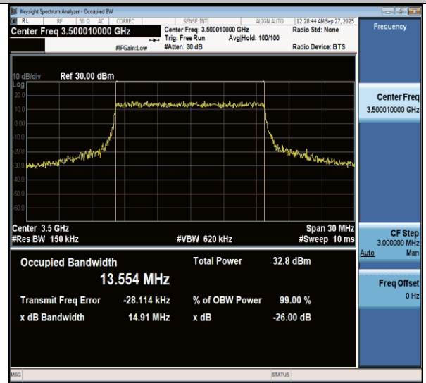
NTNV-n77(3450-3550)-PC3-30-15-M-CP-64QAM-Outet_Full-Ant1-PASS
