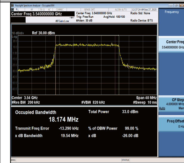
NTNV-n77(3450-3550)-PC3-30-20-H-CP-64QAM-Outer_Full-Ant1-PASS
