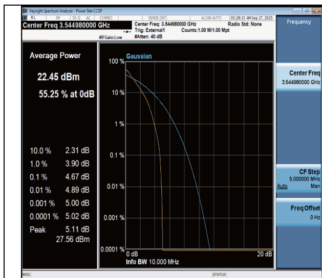
NTNV-n77(3450-3550)-PC3-30-10-H-DFT-BPSK-Outter_Full-PASS
