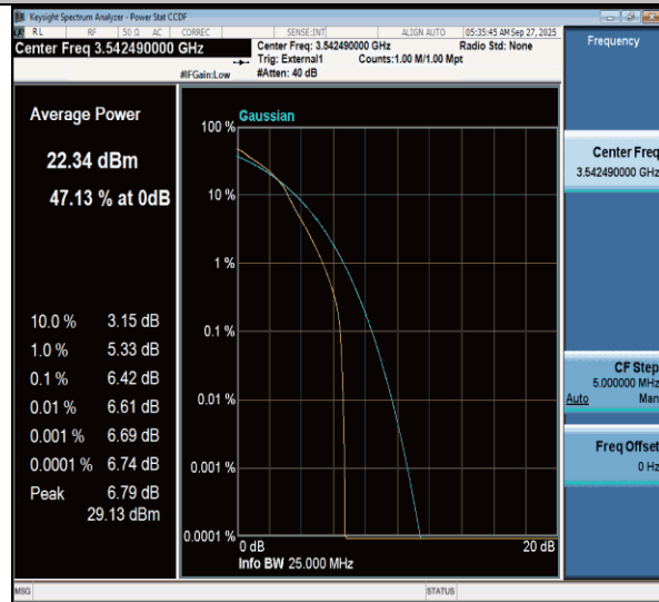
NTNV-n77(3450-3550)-PC3-30-15-H-DFT-16QAM-Outer_Full-PASS
