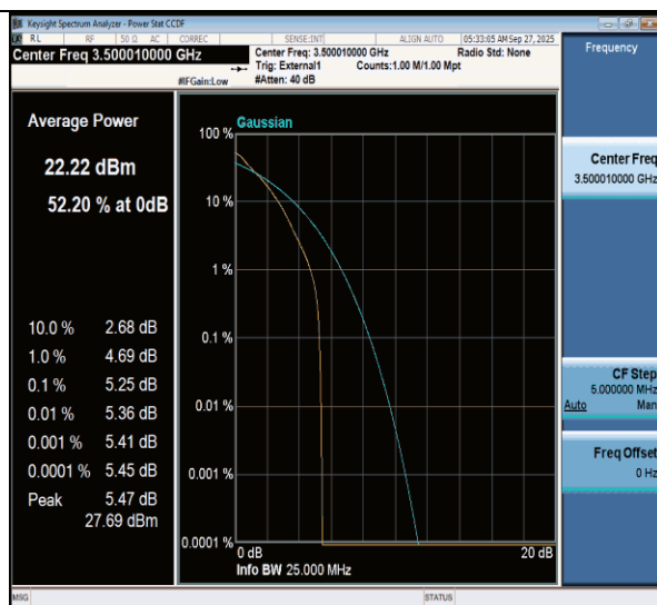
NTNV-n77(3450-3550)-PC3-30-15-M-DFT-QPSK-Outter_Full-PASS
