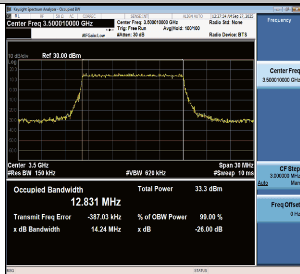
NTNV-n77(3450-3550)-PC3-30-15-M-DFT-QPSK-Outer_Full- Ant1-PASS
