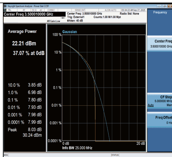
NTNV-n77(3450-3550)-PC3-30-15-M-CP-64QAM-Outer_Full-PASS
