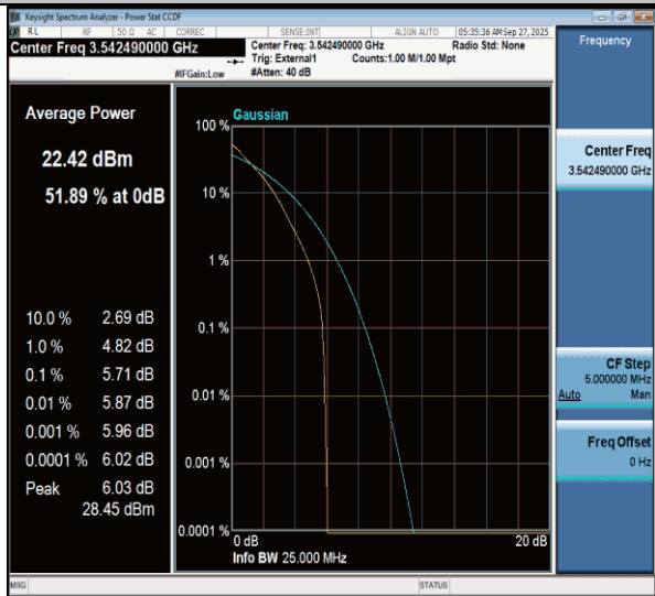
NTNV-n77(3450-3550)-PC3-30-15-H-DFT-QPSK-Outer_Full-PASS
