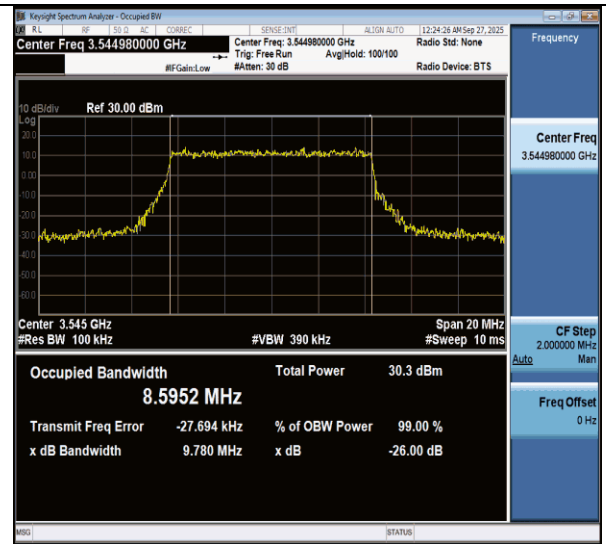
NTNV-n77(3450-3550)-PC3-30-10-H-CP-QPSK-Outer_Full-Ant1-PASS
