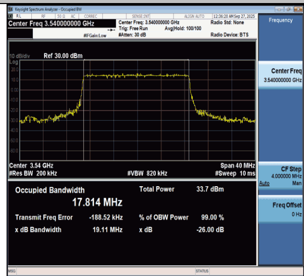
NTNV-n77(3450-3550)-PC3-30-20-H-DFT-QPSK-Outer_Full-Ant1-PASS
