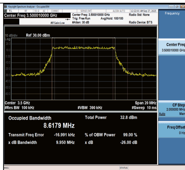
NTVN-n77(3450-3550)-PC3-30-10-M-DFT-16QAM-Outter_Full-Ant1-PASS
