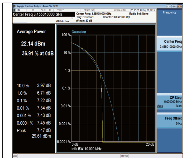
NTNV-n77(3450-3550)-PC3-30-10-L-CP-16QAM-Outter_Full-PASS
