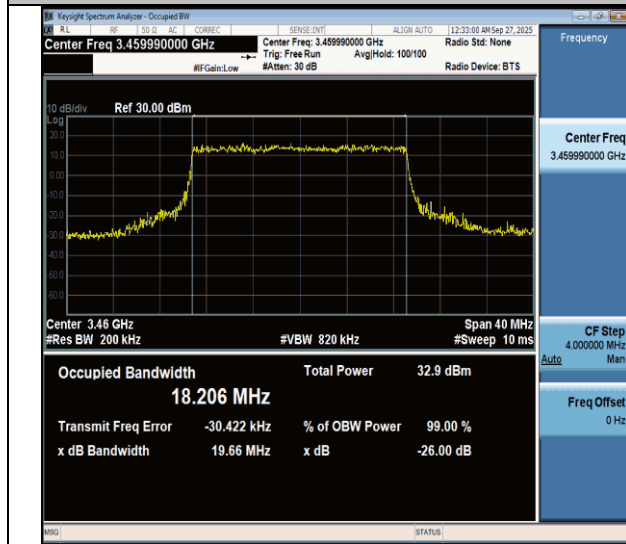
NTNV-n77(3450-3550)-PC3-30-20-L-CP-16QAM-Outer_Full-Ant1-PASS
