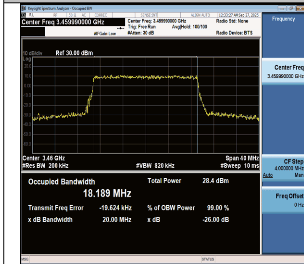
NTNV-n77(3450-3550)-PC3-30-20-L-CP-256QAM-Outer_Full-Ant1-PASS
