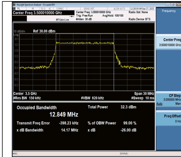
NTNV-n77(3450-3550)-PC3-30-15-M-DFT-256QAM-Outet_Full-Ant1-PASS
