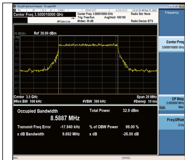
NTVN-n77(3450-3550)-PC3-30-10-M-DFT-QPSK-Outter_Full-Ant1-PASS
