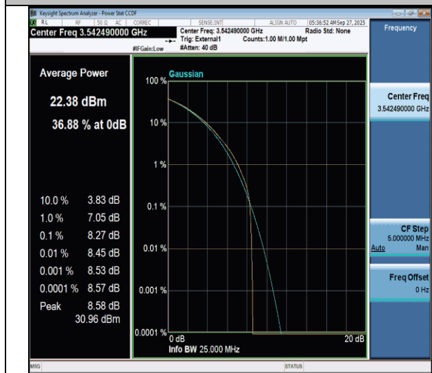
NTNV-n77(3450-3550)-PC3-30-15-H-CP-64QAM-Outter_Full-PASS
