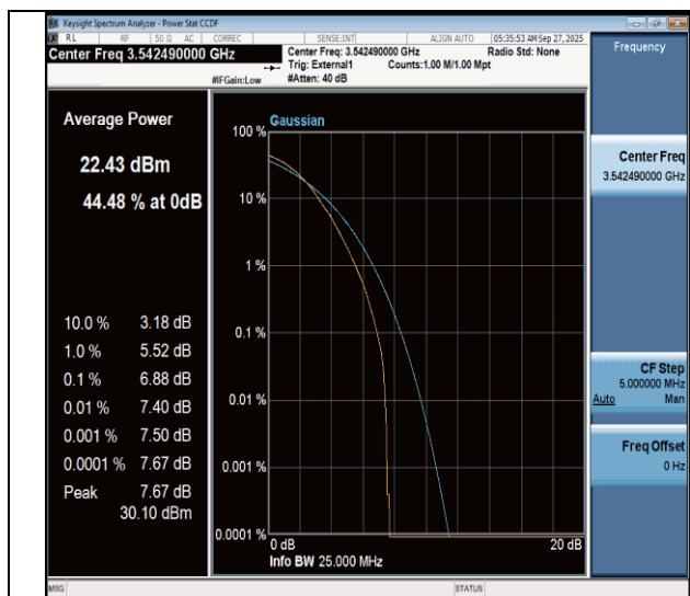
NTNV-n77(3450-3550)-PC3-30-15-H-DFT-64QAM-Outter_Full-PASS
