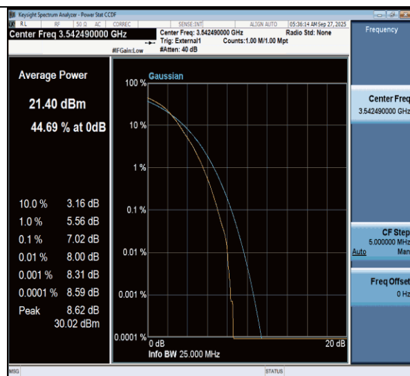
NTNV-n77(3450-3550)-PC3-30-15-H-DFT-256QAM-Outter_Full-PASS
