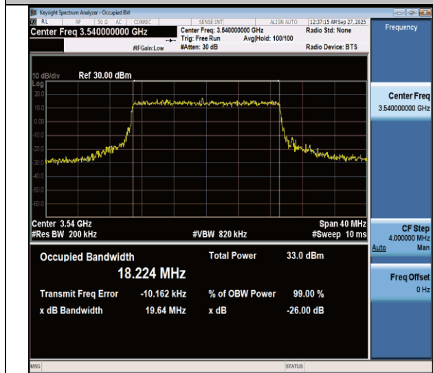
NTNV-n77(3450-3550)-PC3-30-20-H-CP-16QAM-Outer_Full-Ant1-PASS
