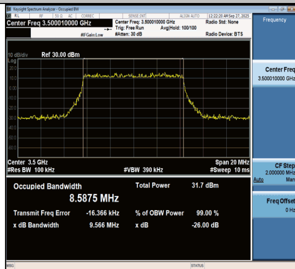
NTVN-n77(3450-3550)-PC3-30-10-M-DFT-256QAM-Outter_Full-Ant1-PASS
