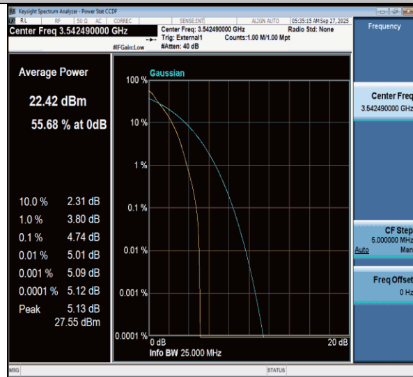
NTNV-n77(3450-3550)-PC3-30-15-H-DFT-BPSK-Outer_Full-PASS
