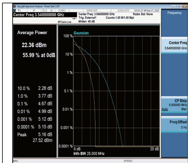
NTNV-n77(3450-3550)-PC3-30-20-H-DFT-BPSK-Outter_Full-PASS
