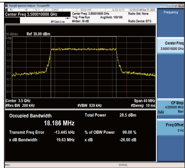
NTNV-n77(3450-3550)-PC3-30-20-M-CP-256QAM-Outer_Full-Ant1-PASS
