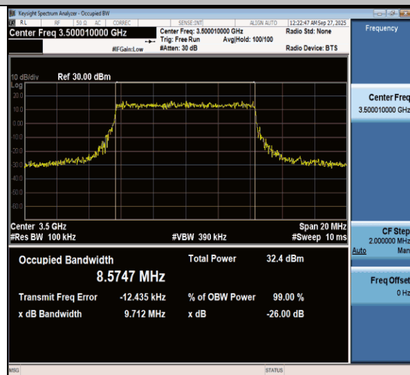
NTVN-n77(3450-3550)-PC3-30-10-M-CP-16QAM-Outter_Full-Ant1-PASS
