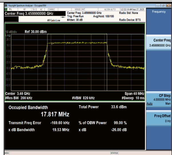
NTNV-n77(3450-3550)-PC3-30-20-L-DFT-64QAM-Outer_Full-Ant1-PASS
