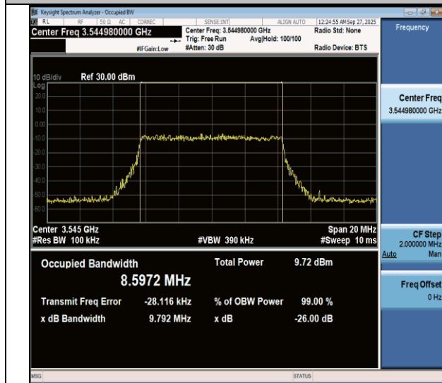
NTNV-n77(3450-3550)-PC3-30-10-H-CP-256QAM-Outer_Full-Ant1-PASS
