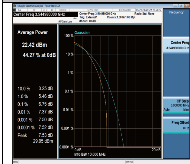
NTNV-n77(3450-3550)-PC3-30-10-H-DFT-256QAM-Outter_Full-PASS
