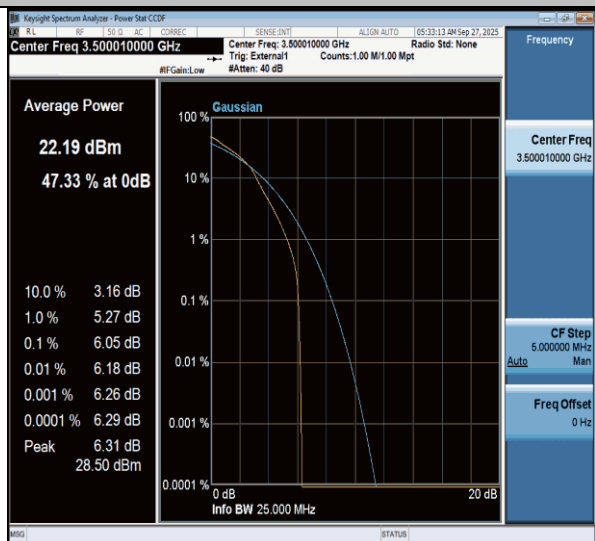
NTNV-n77(3450-3550)-PC3-30-15-M-DFT-16QAM-Outter_Full-PASS
