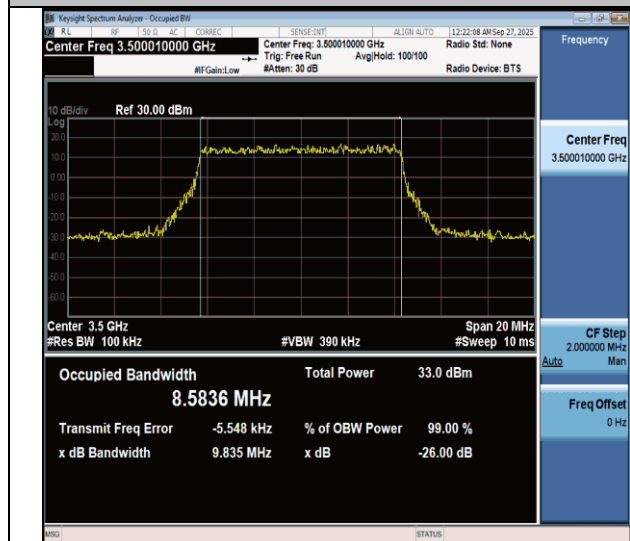
NTVN-n77(3450-3550)-PC3-30-10-M-DFT-64QAM-Outter_Full-Ant1-PASS
