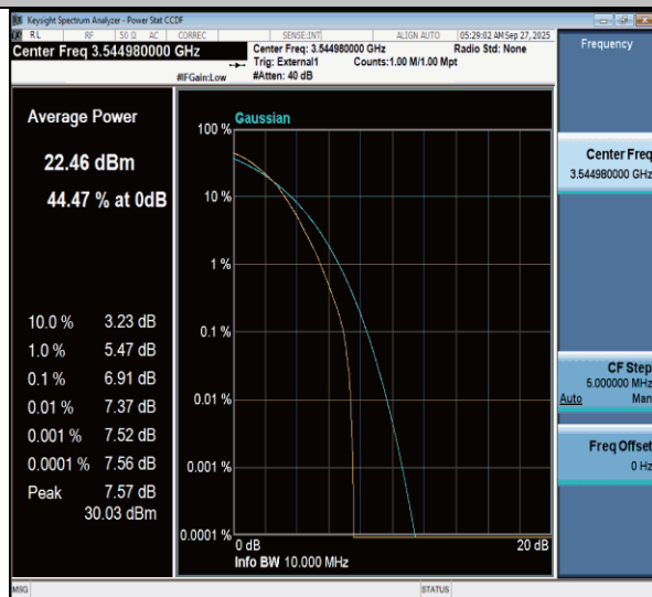
NTNV-n77(3450-3550)-PC3-30-10-H-DFT-64QAM-Outter_Full-PASS
