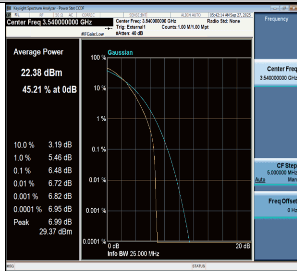
NTNV-n77(3450-3550)-PC3-30-20-H-DFT-64QAM-Outter_Full-PASS
