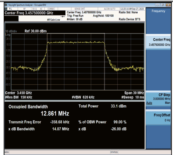
NTNV-n77(3450-3550)-PC3-30-15-L-DFT-BPSK-Outer_Full-Ant1-PASS
