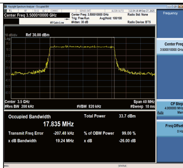
NTVN-n77(3450-3550)-PC3-30-20-M-DFT-16QAM-Outter_Full-Ant1-PASS
