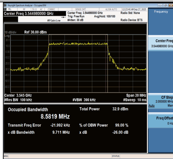
NTNV-n77(3450-3550)-PC3-30-10-H-DFT-QPSK-Outer_Full-Ant1-PASS
