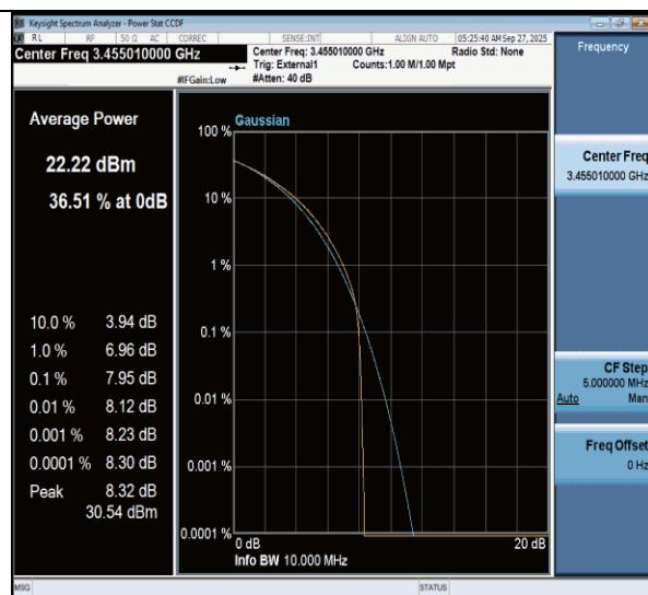
NTNV-n77(3450-3550)-PC3-30-10-L-CP-64QAM-Outter_Full-PASS
