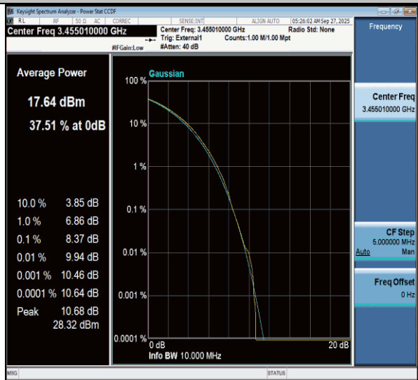
NTNV-n77(3450-3550)-PC3-30-10-L-CP-256QAM-Outter_Full-PASS
