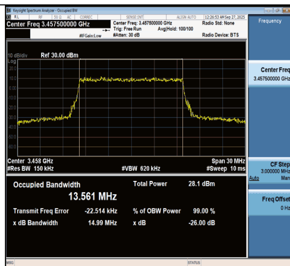
NTNV-n77(3450-3550)-PC3-30-15-L-CP-256QAM-Outer_Full- Ant1-PASS
