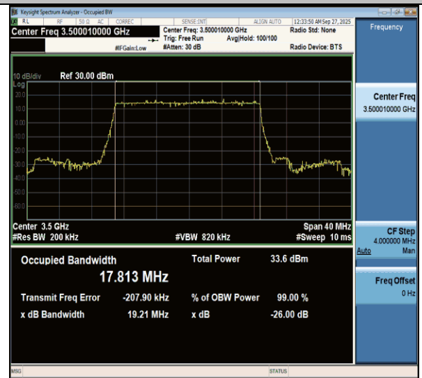
NTNV-n77(3450-3550)-PC3-30-20-M-DFT-BPSK-Outer_Full-Ant1-PASS
