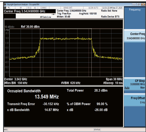
NTNV-n77(3450-3550)-PC3-30-15-H-CP-256QAM-Outer_Full-Ant1-PASS
