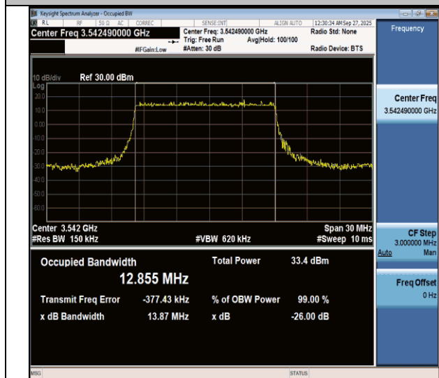
NTNV-n77(3450-3550)-PC3-30-15-H-CP-QPSK-Outet_Full-Ant1- PASS
