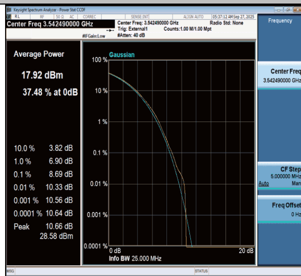
NTNV-n77(3450-3550)-PC3-30-15-H-CP-256QAM-Outter_Full-PASS
