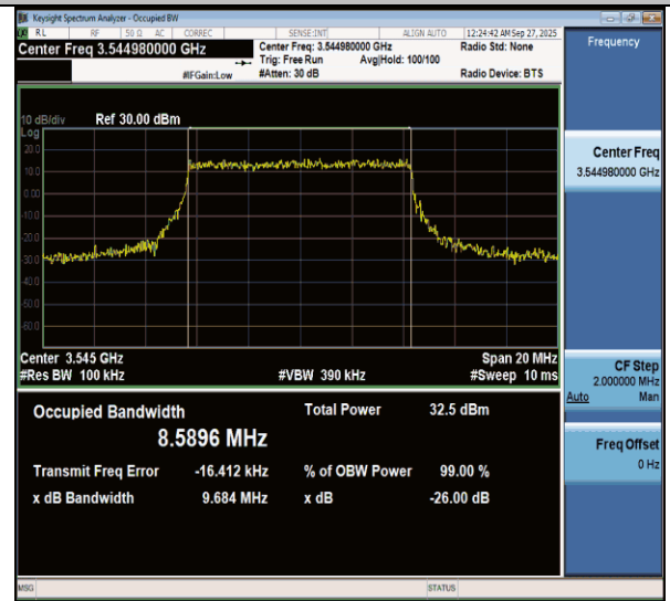
NTNV-n77(3450-3550)-PC3-30-10-H-CP-64QAM-Outer_Full-Ant1-PASS
