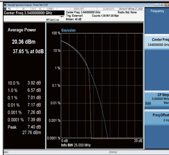
NTNV-n77(3450-3550)-PC3-30-20-H-CP-QPSK-Outter_Full-PASS
