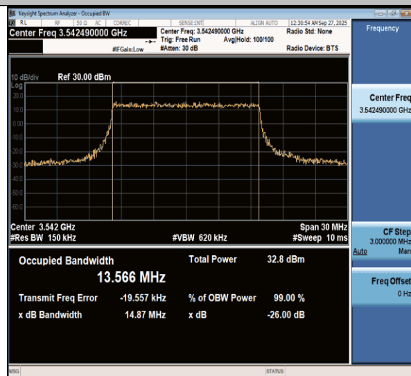
NTNV-n77(3450-3550)-PC3-30-15-H-CP-16QAM-Outet_Full- Ant1-PASS
