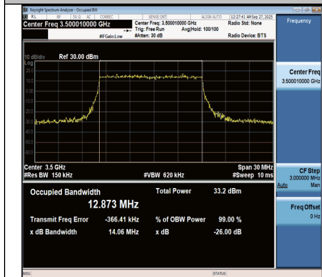
NTNV-n77(3450-3550)-PC3-30-15-M-DFT-16QAM-Outer_Full- Ant1-PASS
