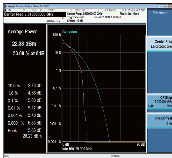
NTNV-n77(3450-3550)-PC3-30-20-H-DFT-QPSK-Outter_Full-PASS
