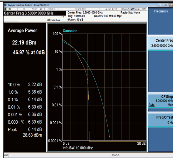
NTNV-n77(3450-3550)-PC3-30-10-M-DFT-16QAM-Outter_Full-PASS
