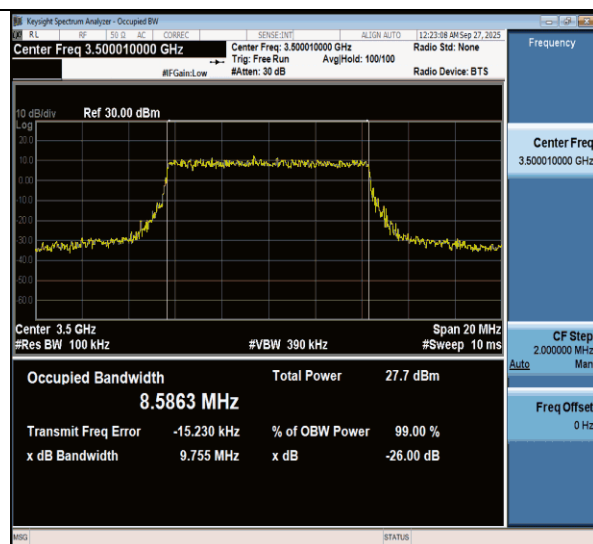
NTNV-n77(3450-3550)-PC3-30-10-M-CP-256QAM-Outer_Full-Ant1-PASS
