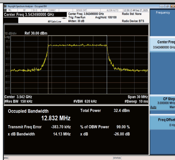
NTNV-n77(3450-3550)-PC3-30-15-H-DFT-256QAM-Outet_Full- Ant1-PASS
