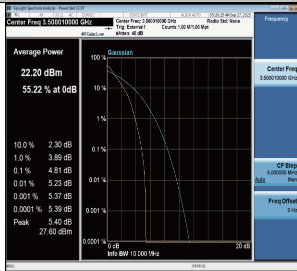
NTNV-n77(3450-3550)-PC3-30-10-M-DFT-BPSK-Outter_Full-PASS
