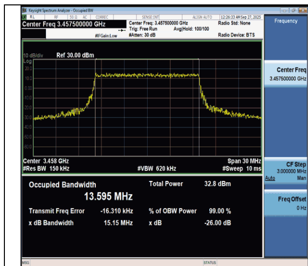
NTNV-n77(3450-3550)-PC3-30-15-L-CP-64QAM-Outer_Full-Ant1- PASS
