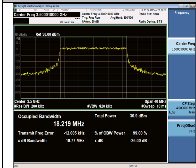
NTVN-n77(3450-3550)-PC3-30-20-M-CP-QPSK-Outter_Full-Ant1-PASS
