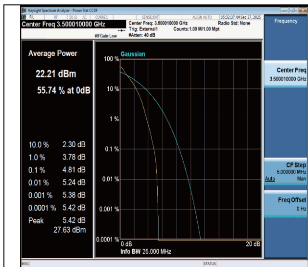
NTNV-n77(3450-3550)-PC3-30-15-M-DFT-BPSK-Outter_Full-PASS
