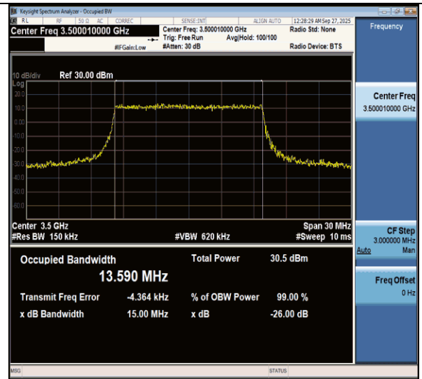
NTNV-n77(3450-3550)-PC3-30-15-M-CP-QPSK-Outet_Full-Ant1-PASS
