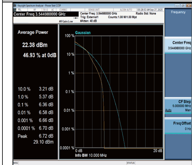
NTNV-n77(3450-3550)-PC3-30-10-H-DFT-16QAM-Outter_Full-PASS
