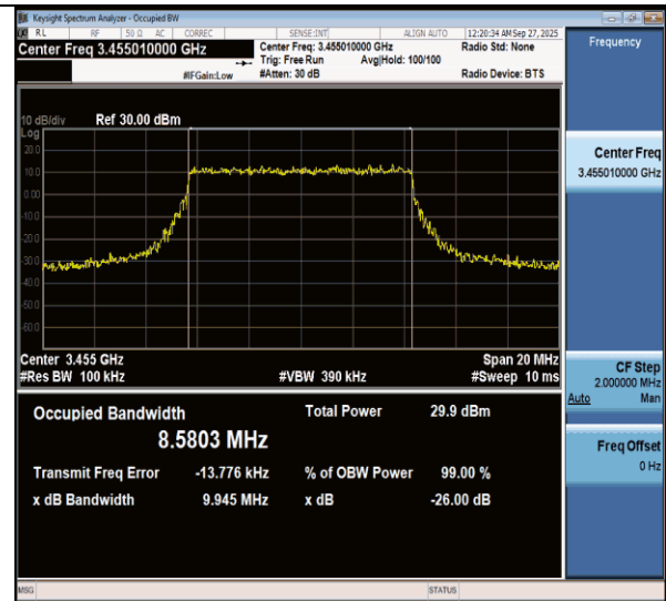
NTNV-n77(3450-3550)-PC3-30-10-L-CP-QPSK-Outer_Full-Ant1-PASS
