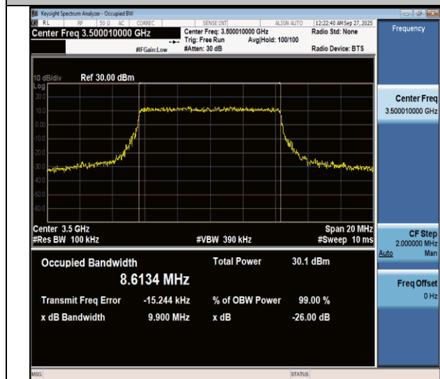
NTVN-n77(3450-3550)-PC3-30-10-M-CP-QPSK-Outter_Full-Ant1-PASS
