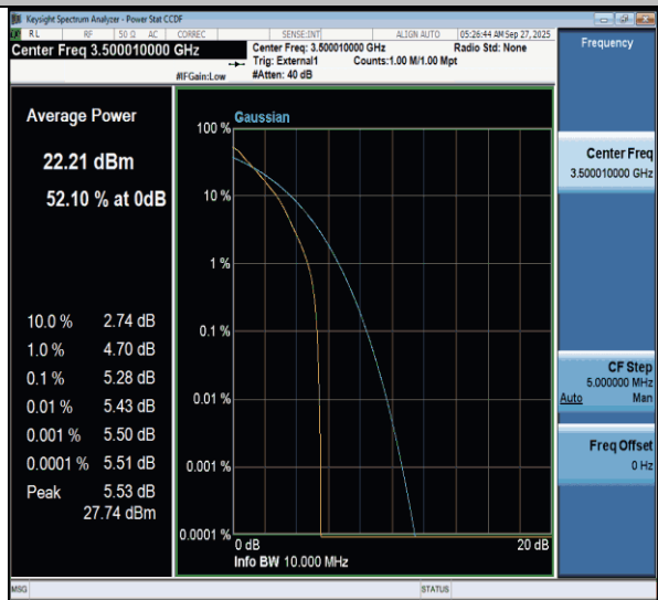
NTNV-n77(3450-3550)-PC3-30-10-M-DFT-QPSK-Outter_Full-PASS
