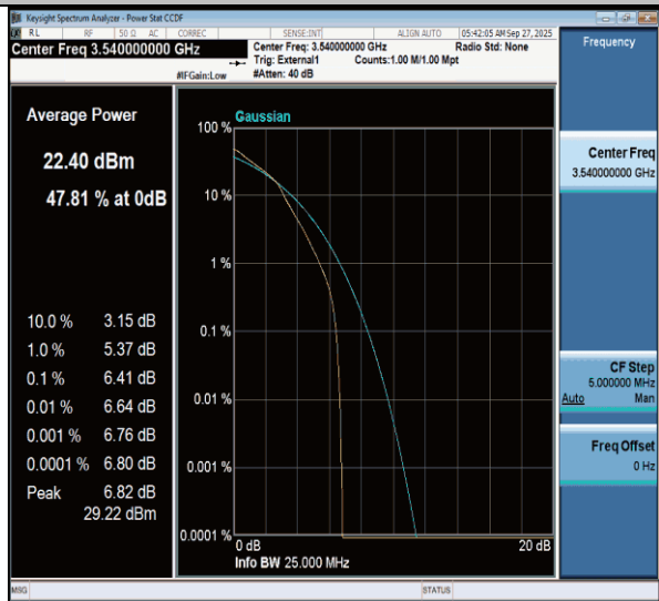
NTNV-n77(3450-3550)-PC3-30-20-H-DFT-16QAM-Outter_Full-PASS
