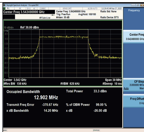
NTNV-n77(3450-3550)-PC3-30-15-H-DFT-16QAM-Outet_Full- Ant1-PASS
