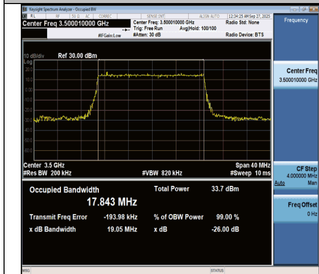
NTVN-n77(3450-3550)-PC3-30-20-M-DFT-64QAM-Outter_Full-Ant1-PASS
