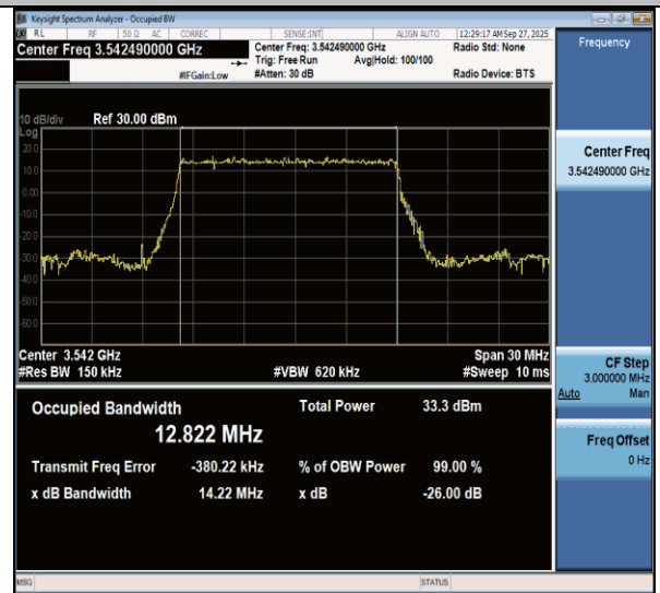
NTNV-n77(3450-3550)-PC3-30-15-H-DFT-BPSK-Outet_Full-Ant1-PASS
