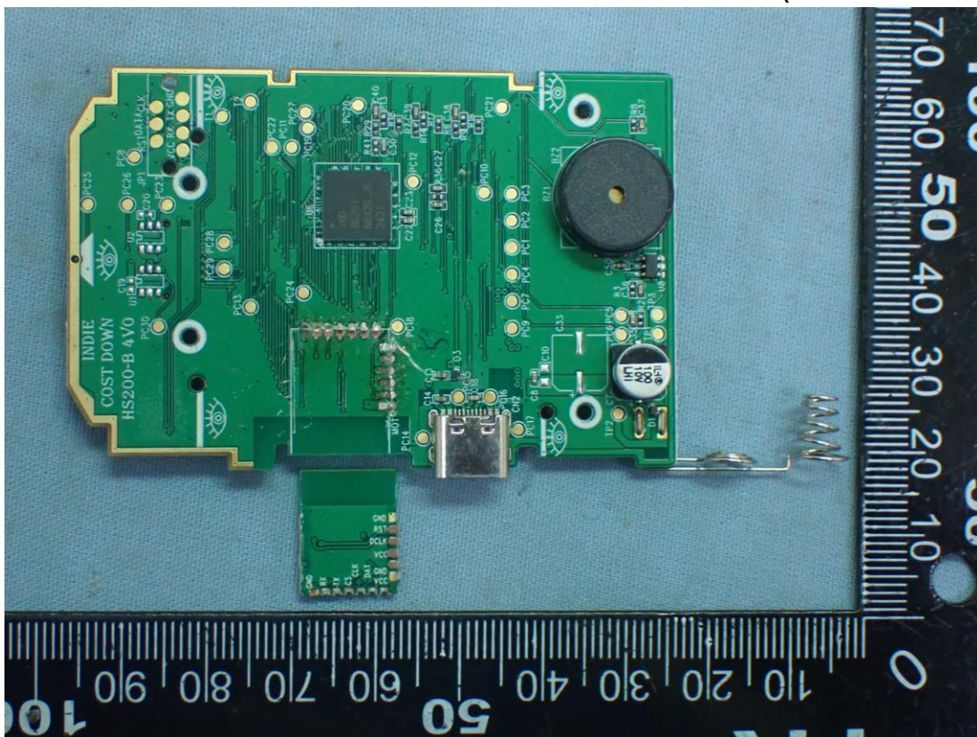
Figure 10 Internal View (Removed RF Module)
