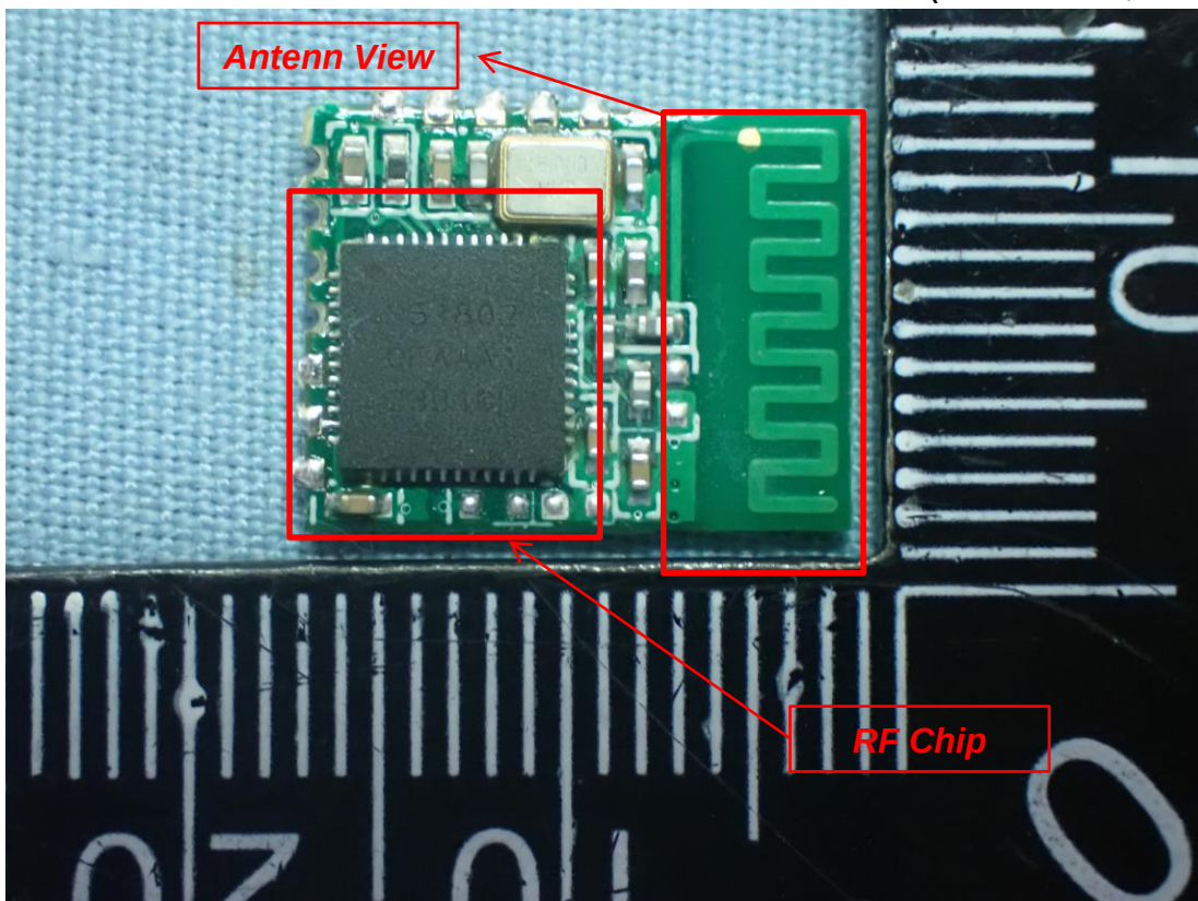
Figure 12 Internal View (RF Module, Front View)
