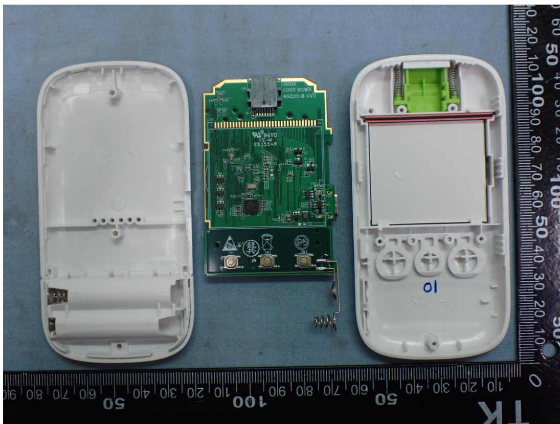
Figure 7 Internal View
