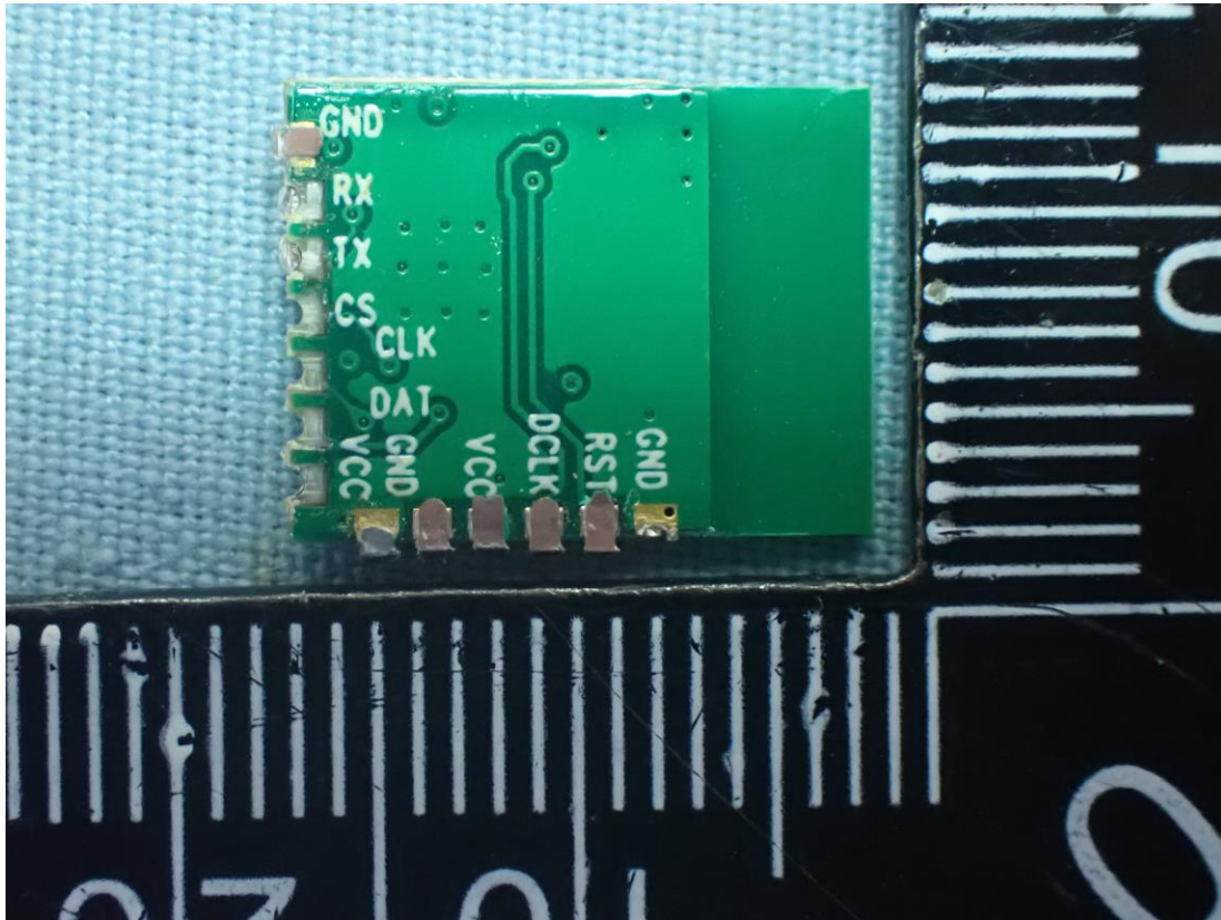
Figure 11 Internal View (RF Module, Back View)
