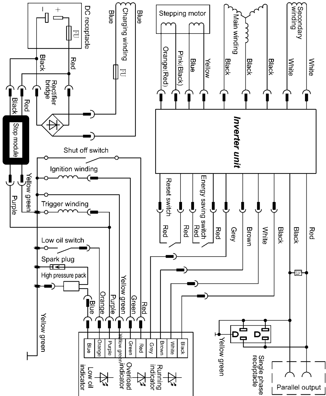
IG2000i Wiring Diagram
