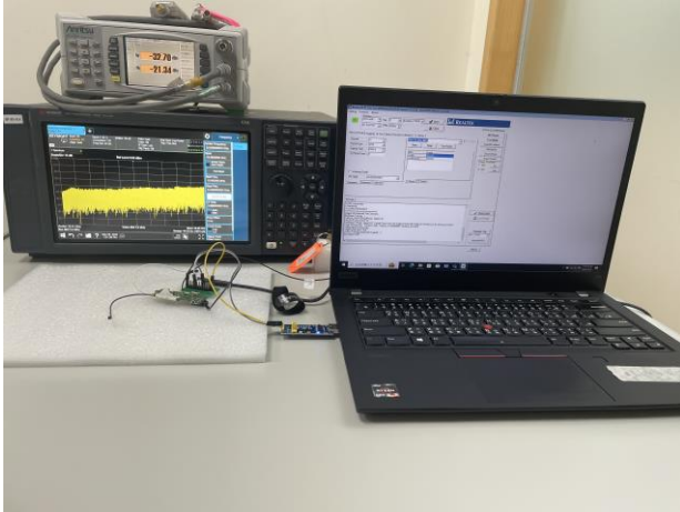
Part_15_247_BT_Radiated_966 (1).JPGSetup
