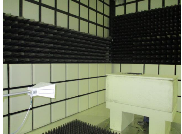
Part_15_247_BT_Radiated_966 (3).JPGSetup
