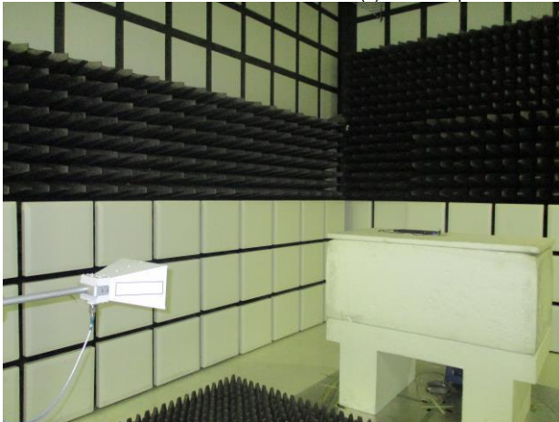
Part_15_247_LE_Radiated_966 (3).JPGSetup
