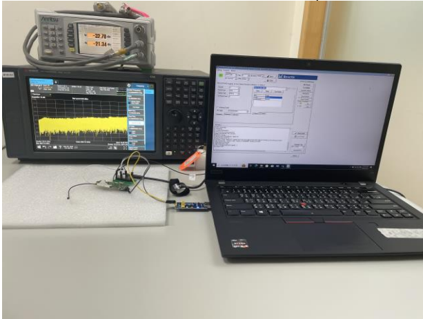
Part_15_247_LE_Conducted_Setup
