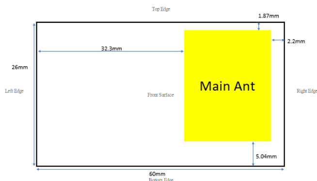
Photograph 13. Antenna position of EUT
