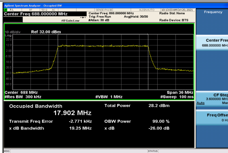
Band71-20MHz-QPSK-133372-100RB#0-17.902
