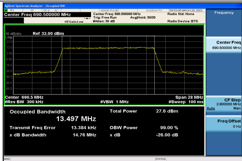
Band71-15MHz-16QAM-133397-75RB#0-13.497
