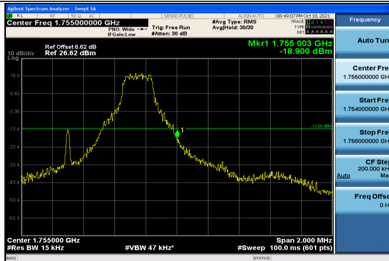
Band4-1.4MHz-16QAM-20393-1RB#5
