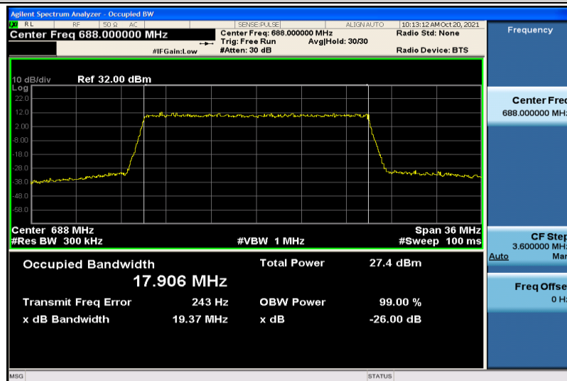
Band71-20MHz-16QAM-133372-100RB#0-17.906
