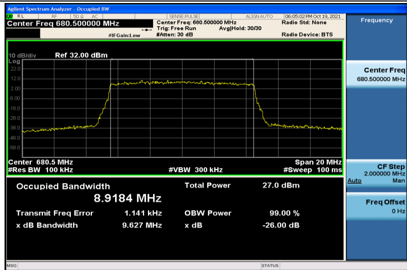
Band71-10MHz-16QAM-133297-50RB#0-8.9184
