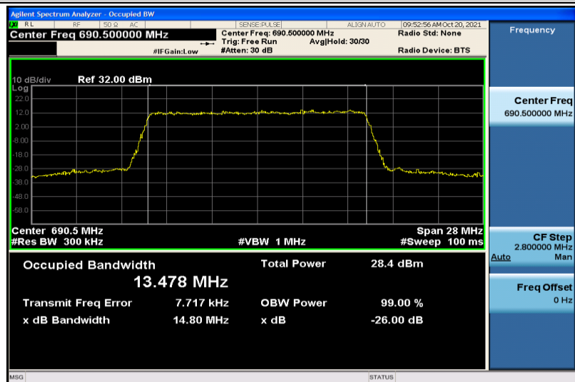
Band71-15MHz-QPSK-133397-75RB#0-13.478
