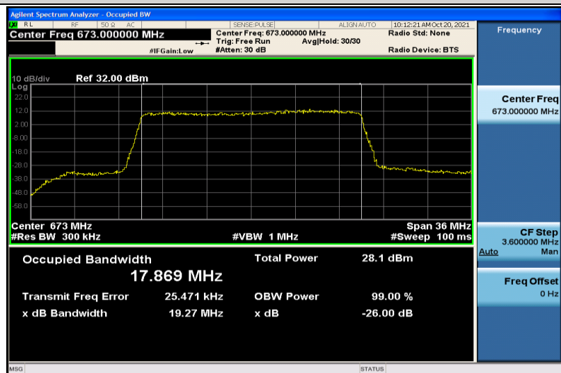
Band71-20MHz-QPSK-133222-100RB#0-17.869
