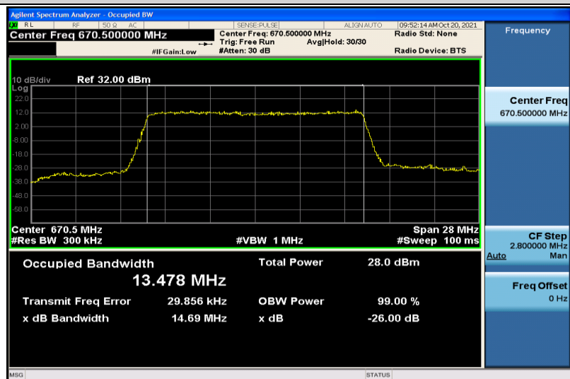
Band71-15MHz-QPSK-133197-75RB#0-13.478
