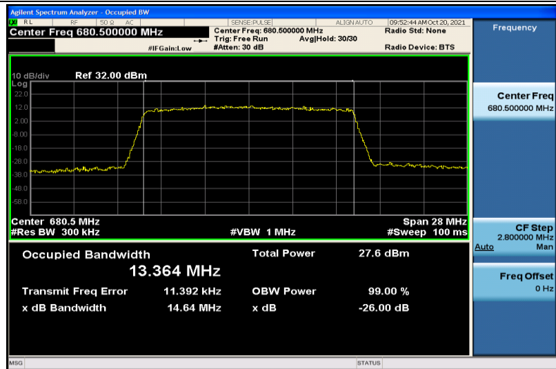
Band71-15MHz-16QAM-133297-75RB#0-13.364
