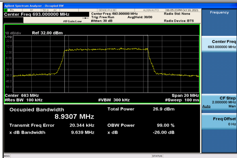
Band71-10MHz-16QAM-133422-50RB#0-8.9307
