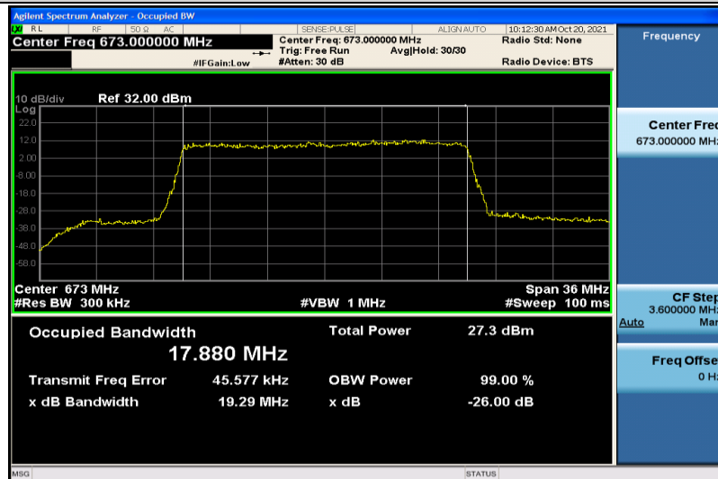
Band71-20MHz-16QAM-133222-100RB#0-17.880
