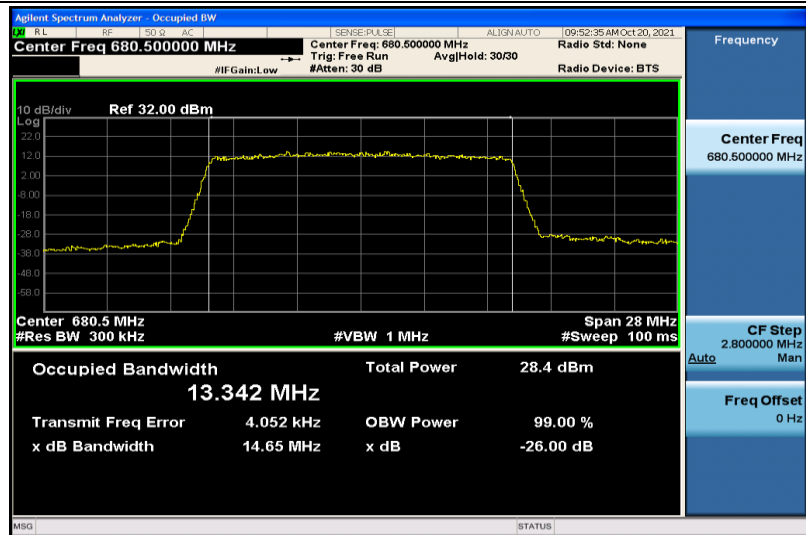
Band71-15MHz-QPSK-133297-75RB#0-13.342
