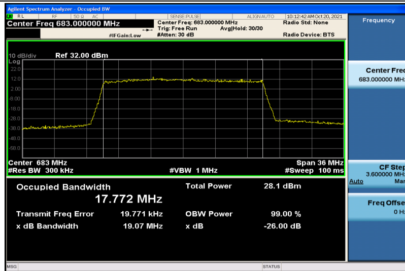
Band71-20MHz-QPSK-133322-100RB#0-17.772
