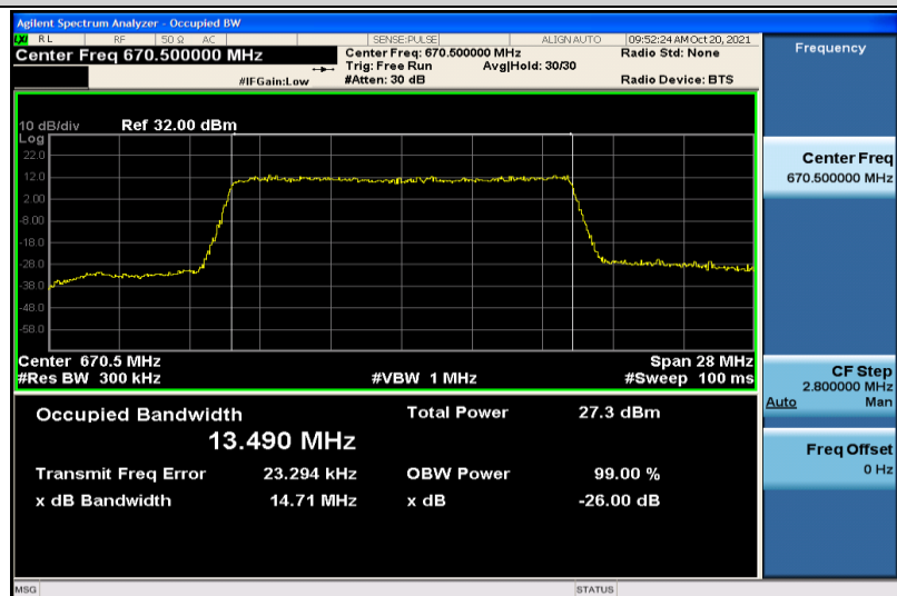
Band71-15MHz-16QAM-133197-75RB#0-13.490
