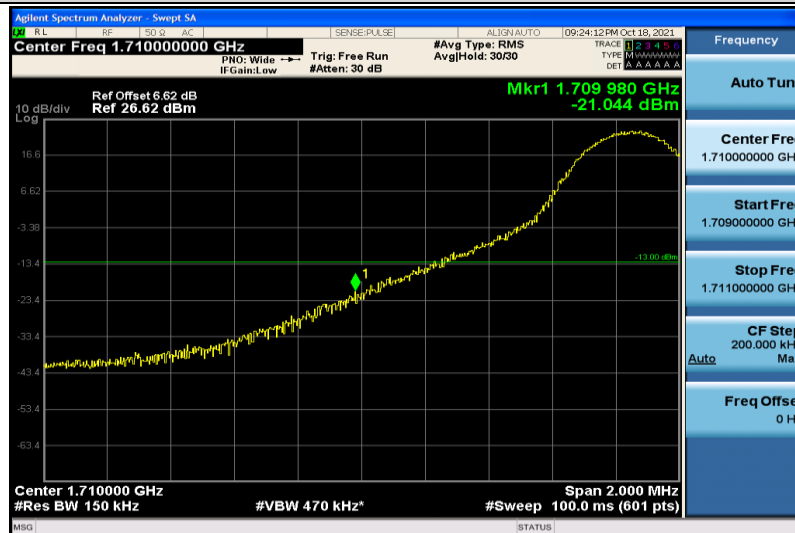
Band4-15MHz-16QAM-20025-1RB#0
