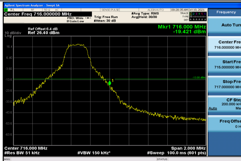
Band12-5MHz-16QAM-23155-1RB#24
