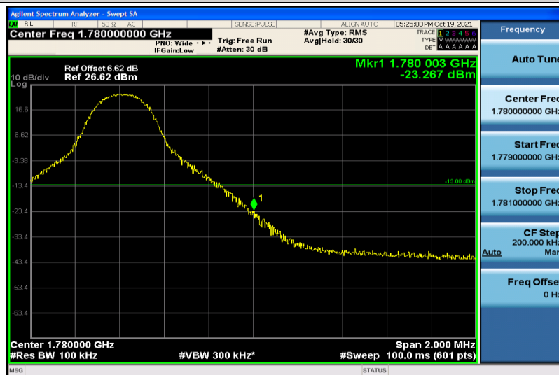
Band66-10MHz-QPSK-132622-1RB#49
