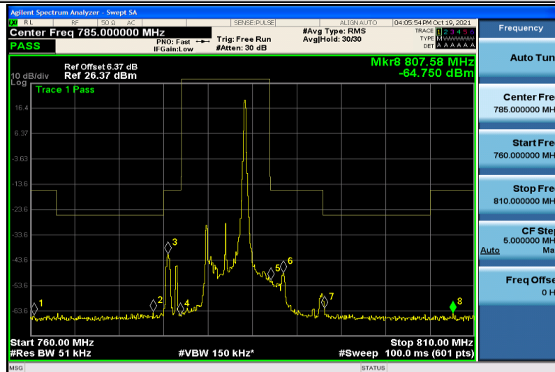
Band13-5MHz-16QAM-23230-1RB#24
