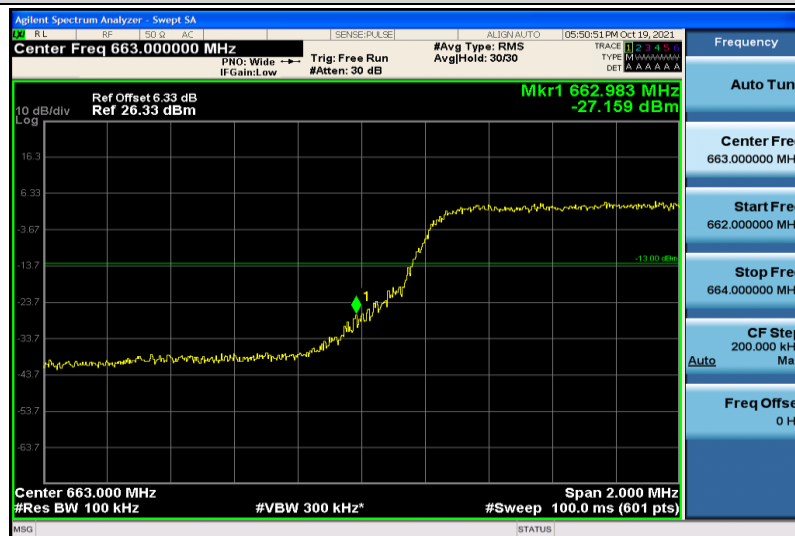
Band71-5MHz-16QAM-133147-25RB#0
