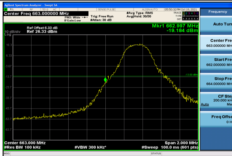
Band71-5MHz-16QAM-133147-1RB#0
