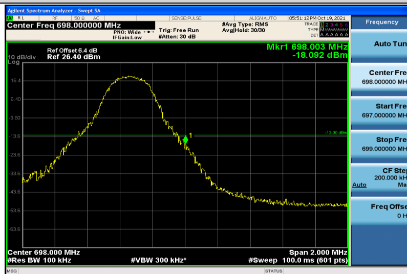
Band71-5MHz-16QAM-133447-1RB#24
