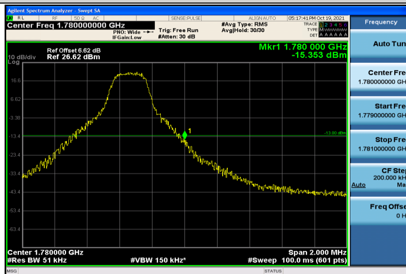
Band66-5MHz-QPSK-132647-1RB#24
