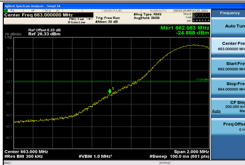
Band71-15MHz-16QAM-133197-1RB#0
