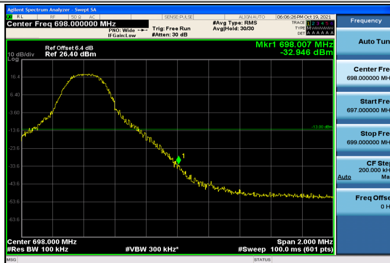
Band71-10MHz-16QAM-133422-1RB#49
