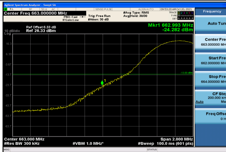
Band71-15MHz-QPSK-133197-1RB#0
