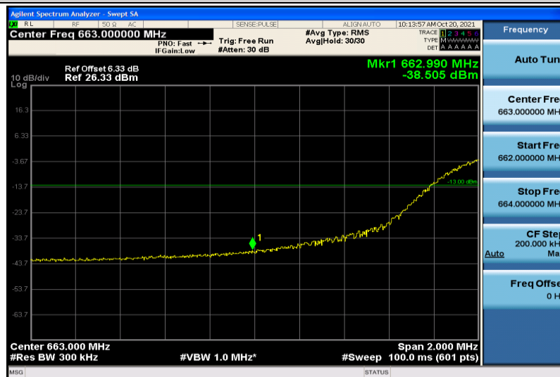
Band71-20MHz-16QAM-133222-100RB#0
