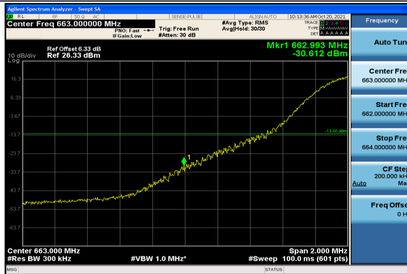
Band71-20MHz-16QAM-133222-1RB#0
