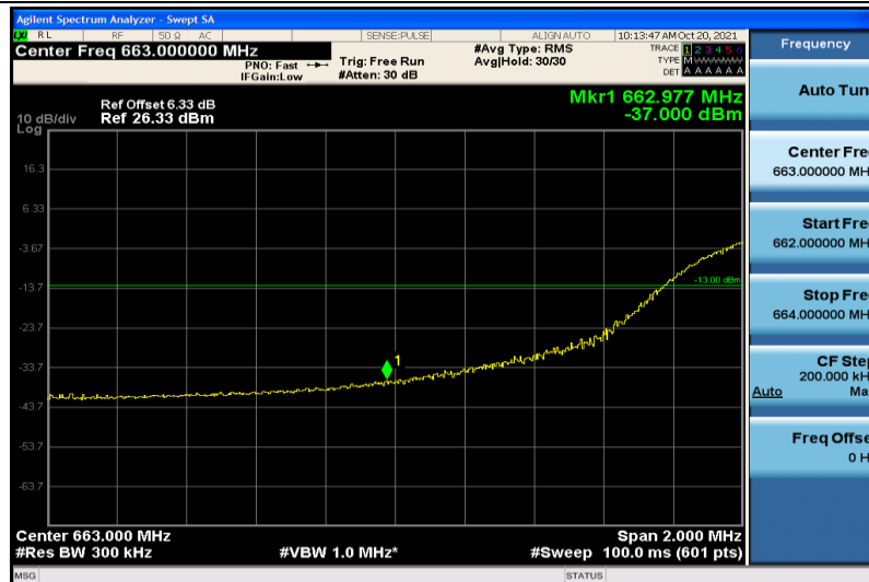
Band71-20MHz-QPSK-133222-100RB#0
