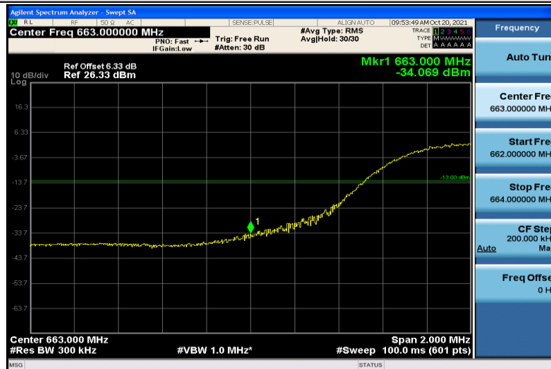
Band71-15MHz-16QAM-133197-75RB#0
