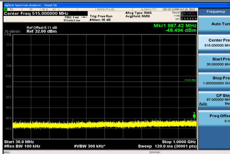
Band4-10MHz-QPSK-20350-1RB#0-30~1000MHz
