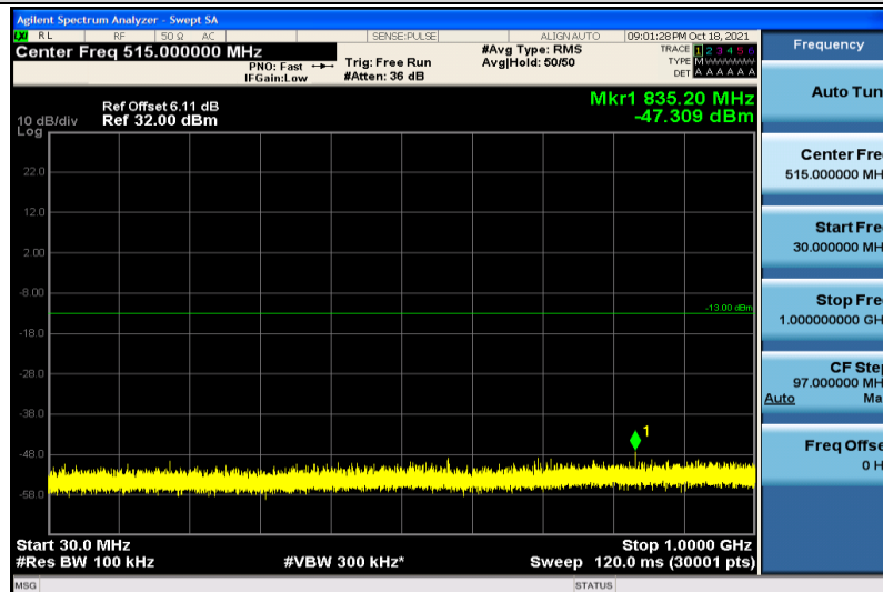
Band4-3MHz-16QAM-20385-1RB#0-30~1000MHz
