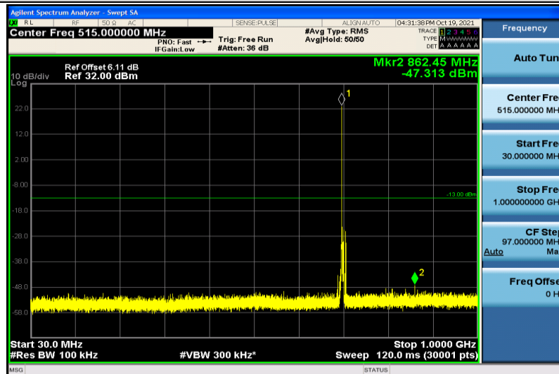
Band17-5MHz-QPSK-23755-1RB#0-30~1000MHz
