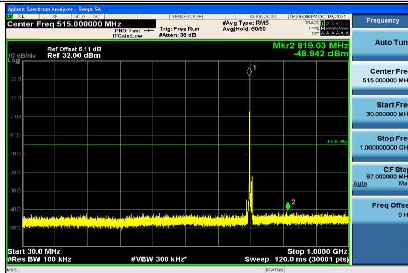
Band17-10MHz-16QAM-23780-1RB#0-30~1000MHz
