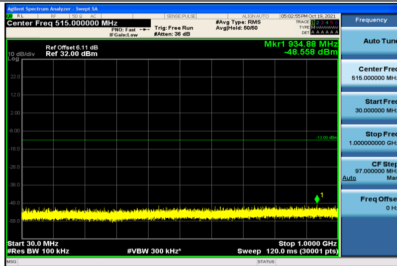
Band66-1.4MHz-QPSK-132665-1RB#0-30~1000MHz
