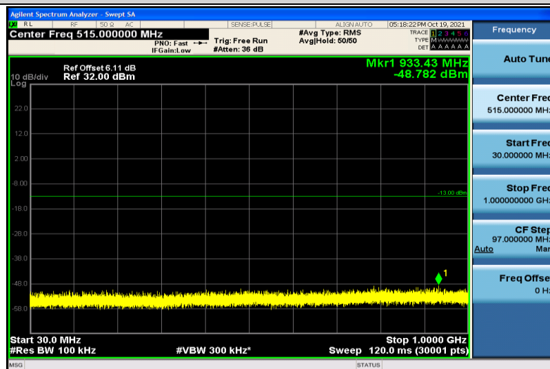
Band66-5MHz-QPSK-131997-1RB#0-30~1000MHz
