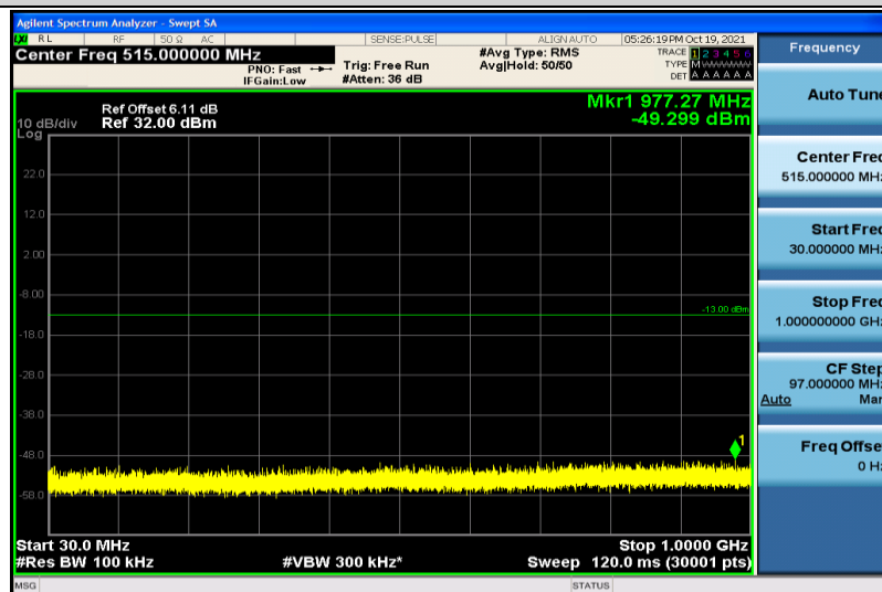
Band66-10MHz-16QAM-132022-1RB#0-30~1000MHz
