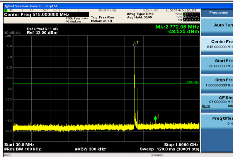
Band71-15MHz-16QAM-133197-1RB#0-30~1000MHz
