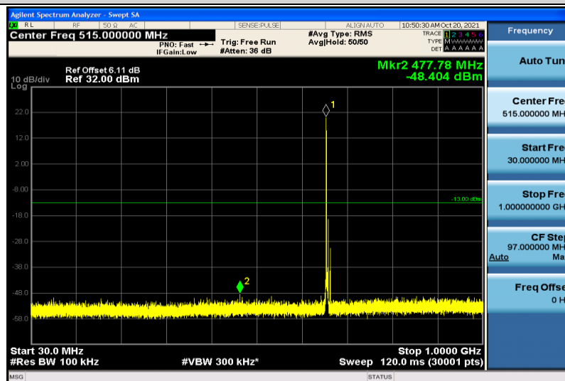
Band71-5MHz-16QAM-133147-1RB#0-30~1000MHz
