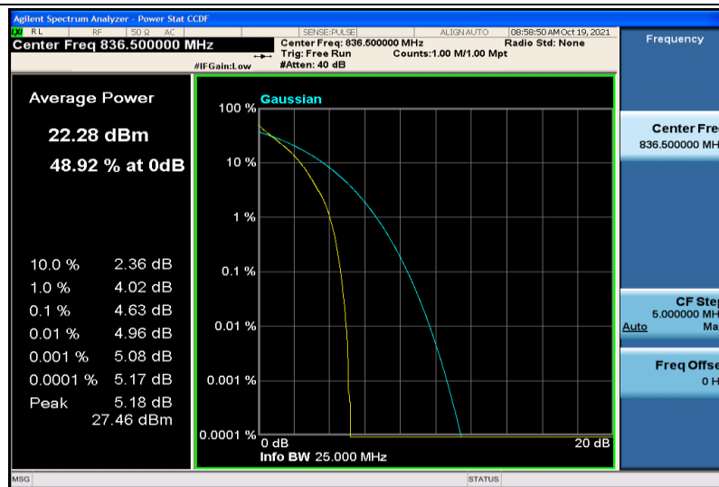
Band5-5MHz-QPSK-20525-25RB#0
