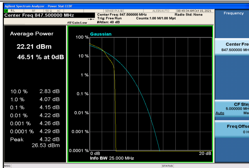
Band5-3MHz-16QAM-20635-1RB#0
