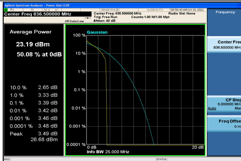
Band5-5MHz-QPSK-20525-1RB#0
