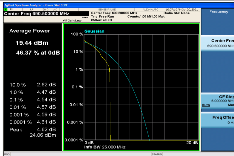
Band71-15MHz-QPSK-133397-1RB#0
