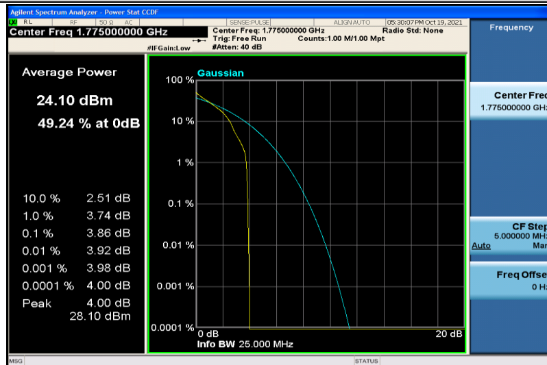
Band66-10MHz-QPSK-132622-1RB#0
