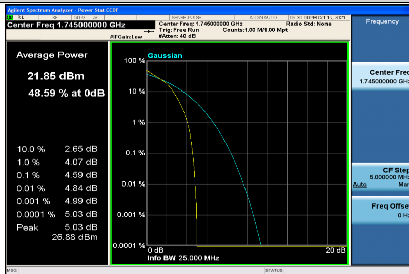
Band66-10MHz-16QAM-132322-50RB#0
