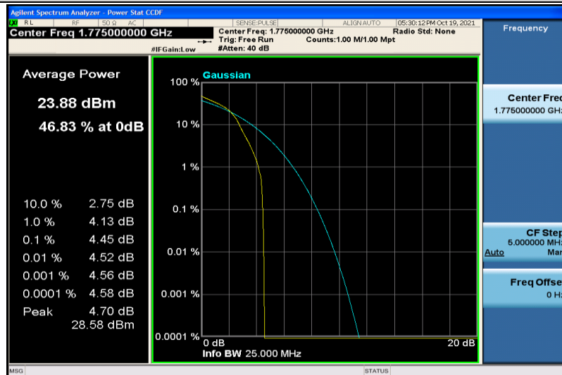
Band66-10MHz-16QAM-132622-1RB#0
