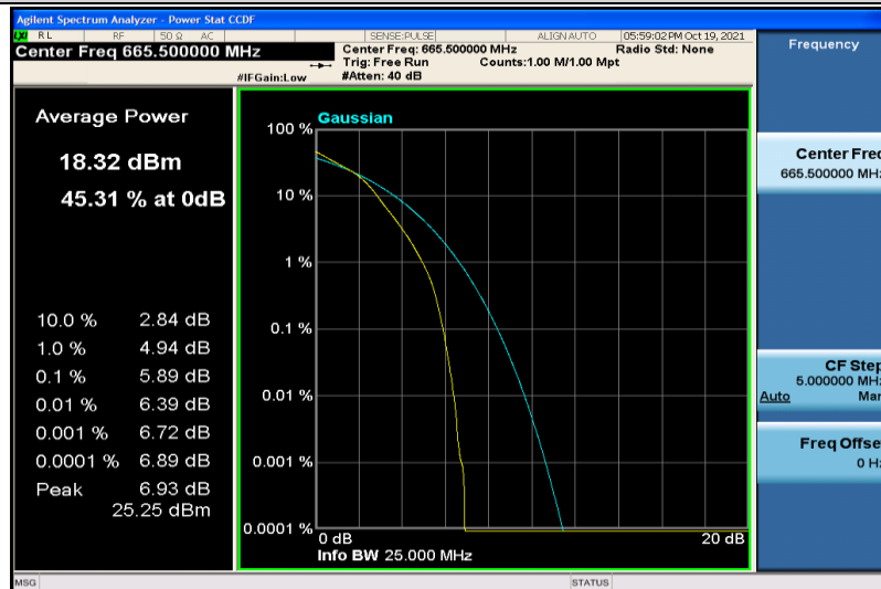
Band71-5MHz-16QAM-133147-25RB#0
