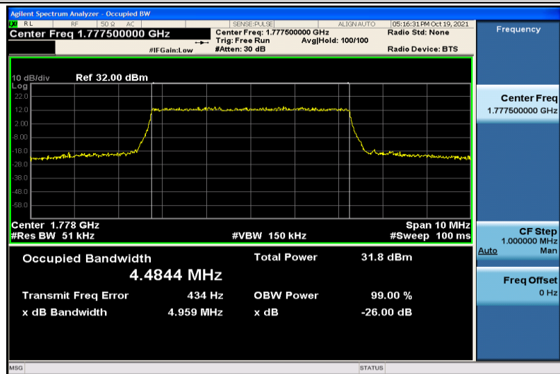
Band66-5MHz-QPSK-132647-25RB#0-4.4844
