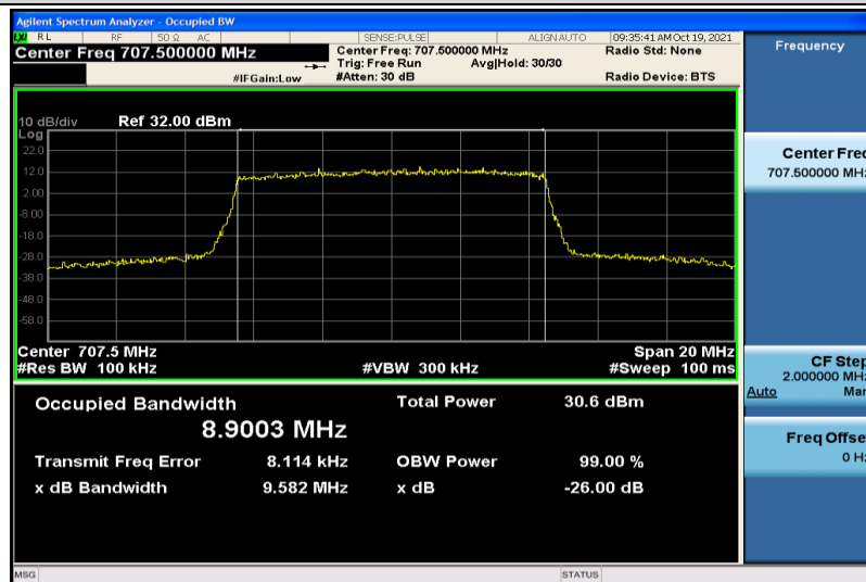
Band12-10MHz-QPSK-23095-50RB#0-8.9003
