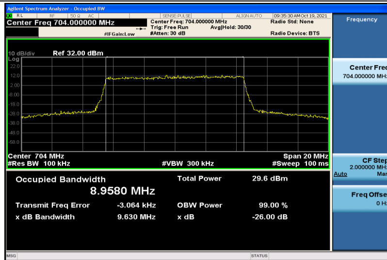
Band12-10MHz-16QAM-23060-50RB#0-8.9580
