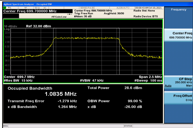
Band12-1.4MHz-16QAM-23017-6RB#0-1.0835
