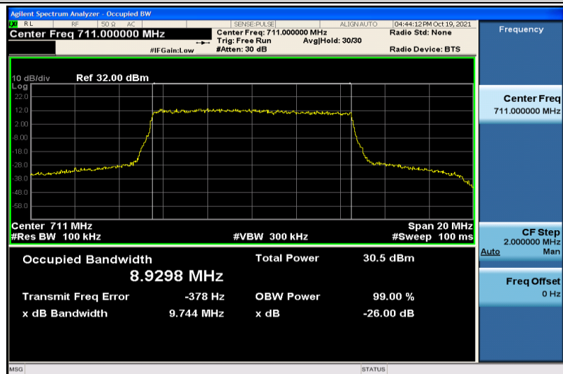
Band17-10MHz-QPSK-23800-50RB#0-8.9298
