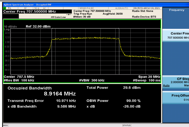
Band12-10MHz-16QAM-23095-50RB#0-8.9164
