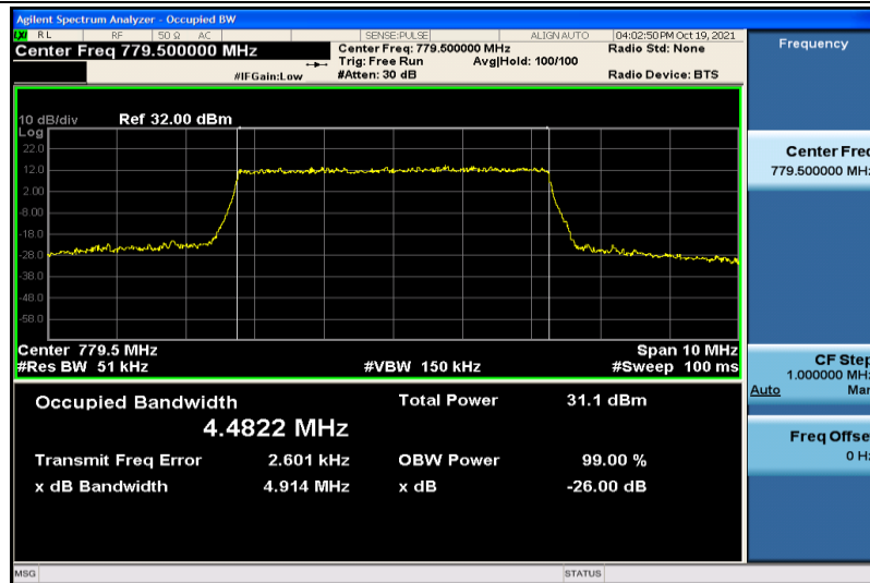
Band13-5MHz-QPSK-23205-25RB#0-4.4822
