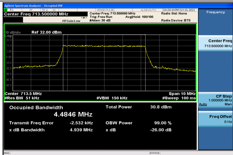
Band17-5MHz-QPSK-23825-25RB#0-4.4846
