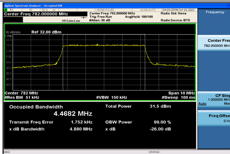
Band13-5MHz-QPSK-23230-25RB#0-4.4682
