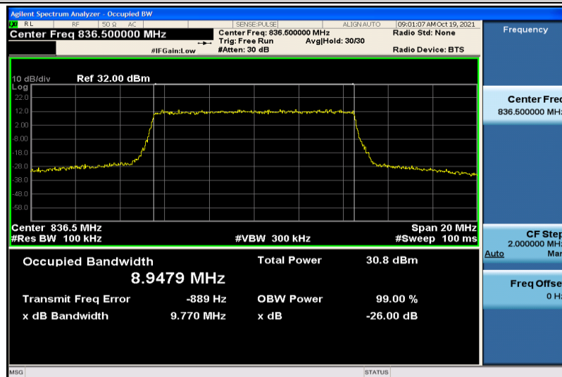
Band5-10MHz-QPSK-20525-50RB#0-8.9479
