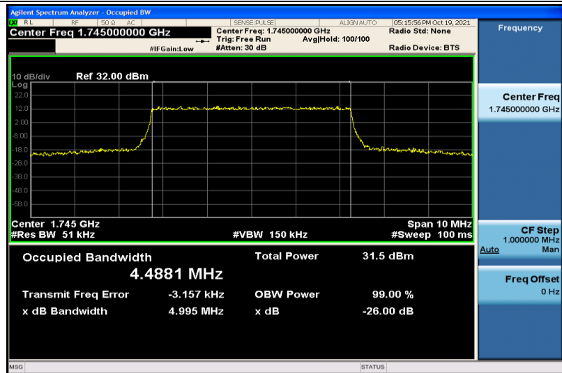
Band66-5MHz-QPSK-132322-25RB#0-4.4881
