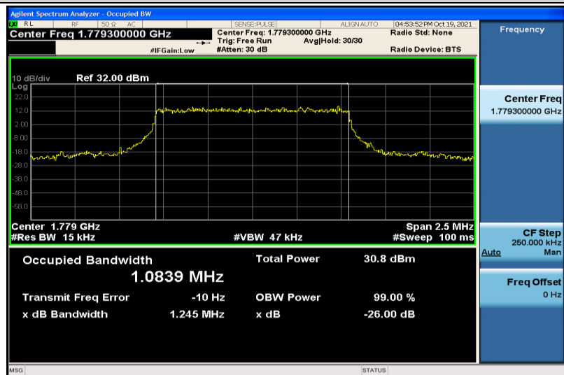
Band66-1.4MHz-QPSK-132665-6RB#0-1.0839
