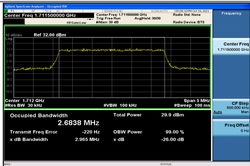
Band66-3MHz-16QAM-131987-15RB#0-2.6838
