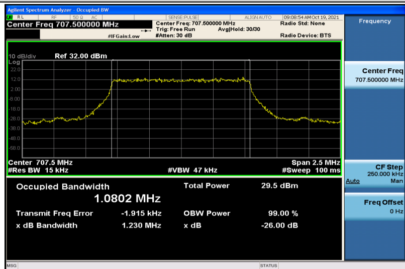
Band12-1.4MHz-QPSK-23095-6RB#0-1.0802
