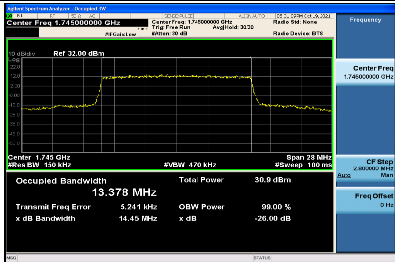
Band66-15MHz-16QAM-132322-75RB#0-13.378
