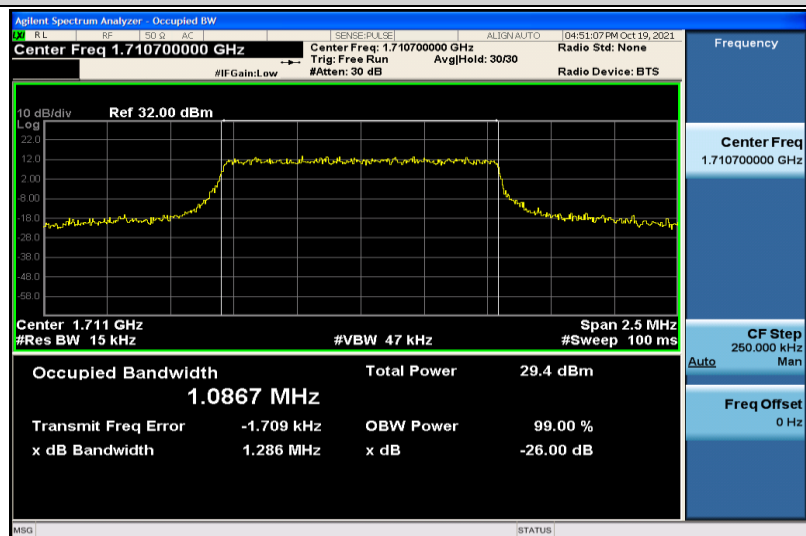
Band66-1.4MHz-16QAM-131979-6RB#0-1.0867
