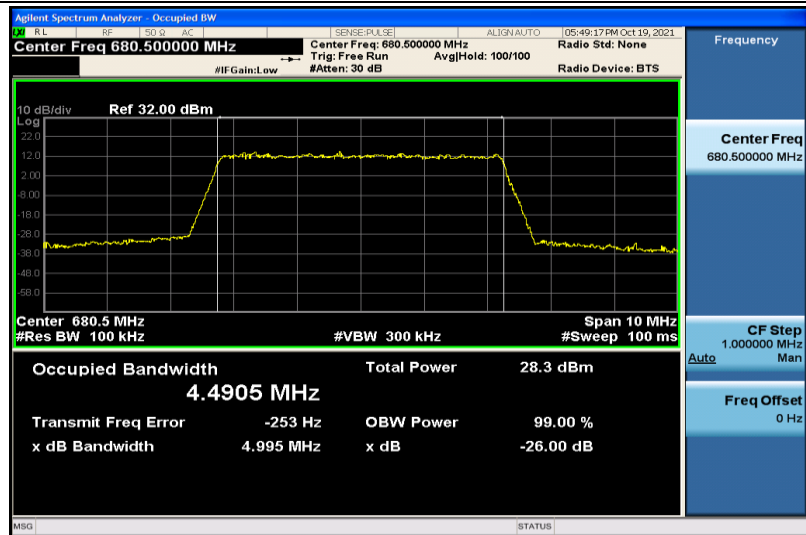
Band71-5MHz-QPSK-133297-25RB#0-4.4905
