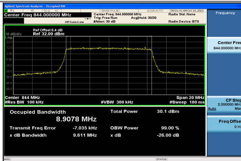
Band5-10MHz-16QAM-20600-50RB#0-8.9078
