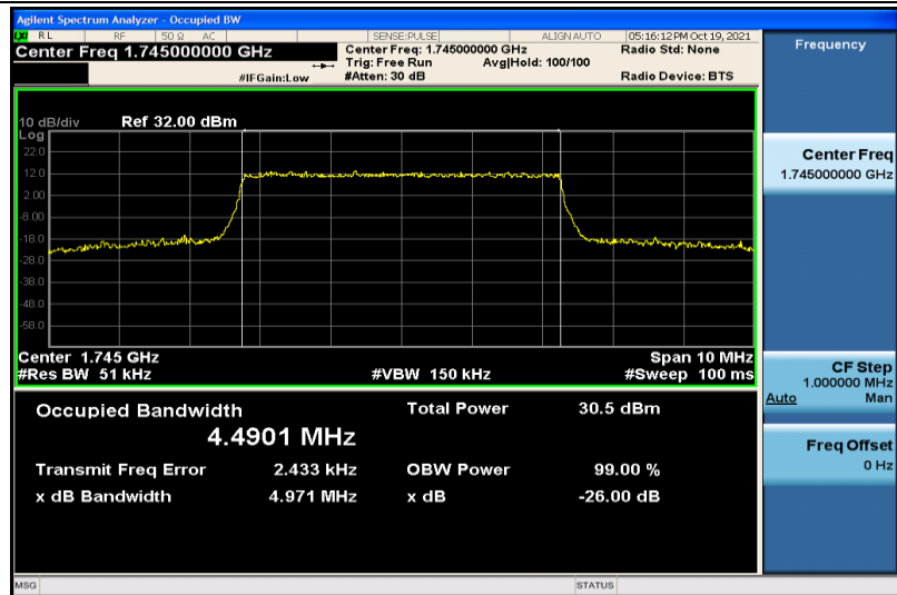
Band66-5MHz-16QAM-132322-25RB#0-4.4901
