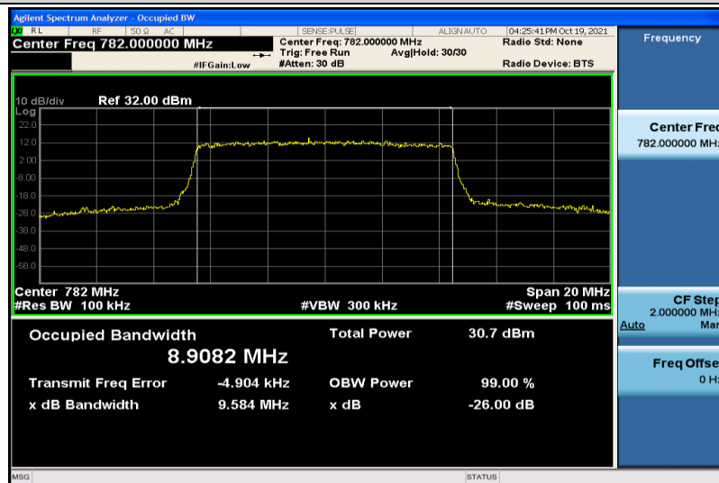
Band13-10MHz-16QAM-23230-50RB#0-8.9082
