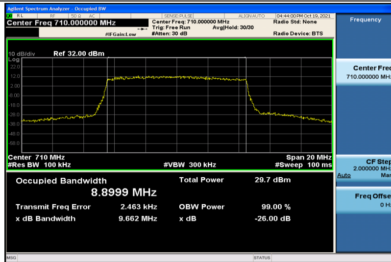
Band17-10MHz-16QAM-23790-50RB#0-8.8999
