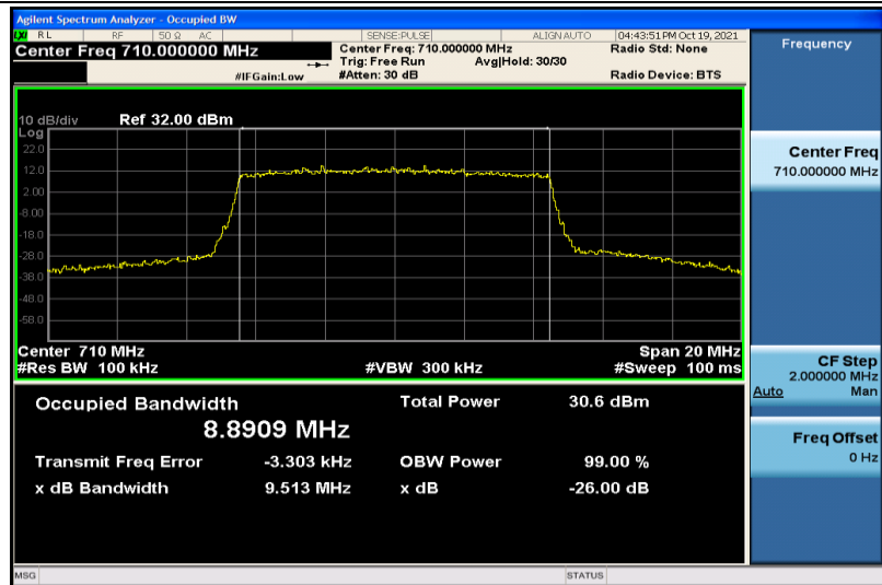
Band17-10MHz-QPSK-23790-50RB#0-8.8909
