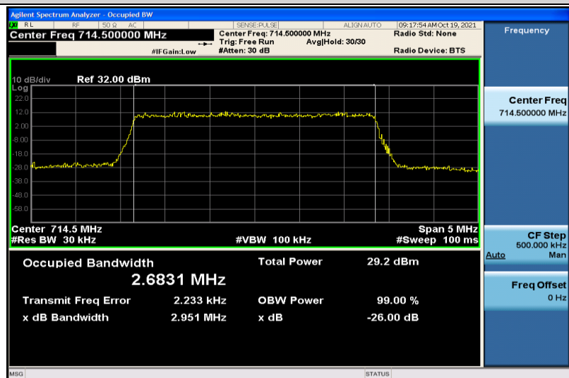
Band12-3MHz-16QAM-23165-15RB#0-2.6831
