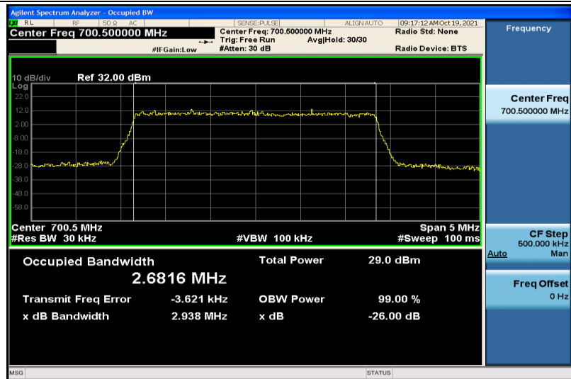
Band12-3MHz-16QAM-23025-15RB#0-2.6816
