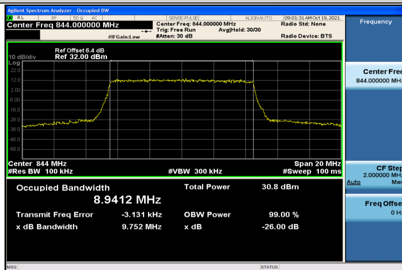
Band5-10MHz-QPSK-20600-50RB#0-8.9412
