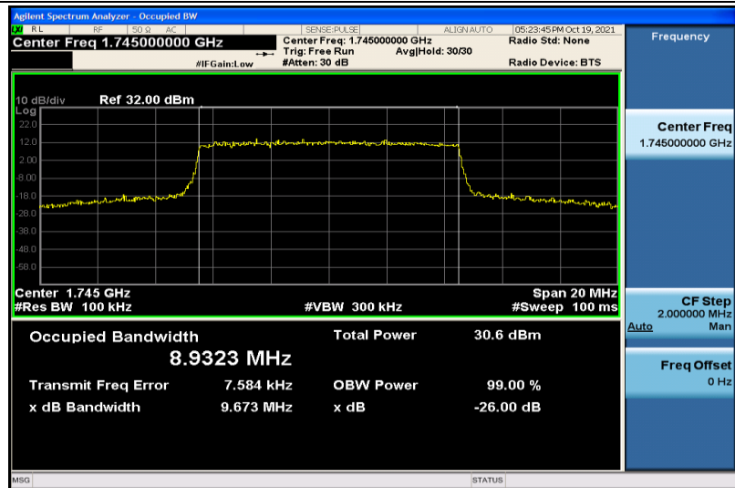
Band66-10MHz-16QAM-132322-50RB#0-8.9323
