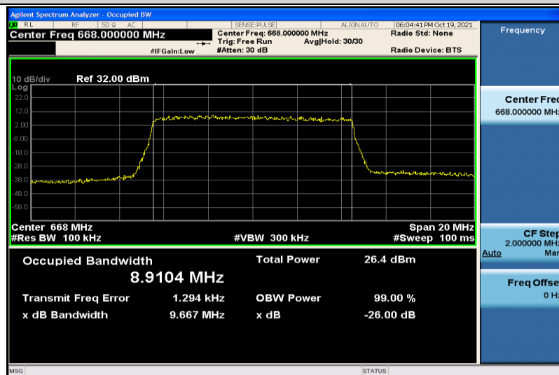
Band71-10MHz-16QAM-133172-50RB#0-8.9104
