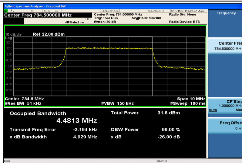
Band13-5MHz-QPSK-23255-25RB#0-4.4813
