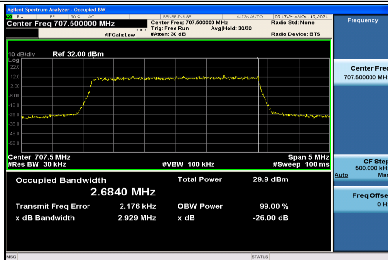
Band12-3MHz-QPSK-23095-15RB#0-2.6840
