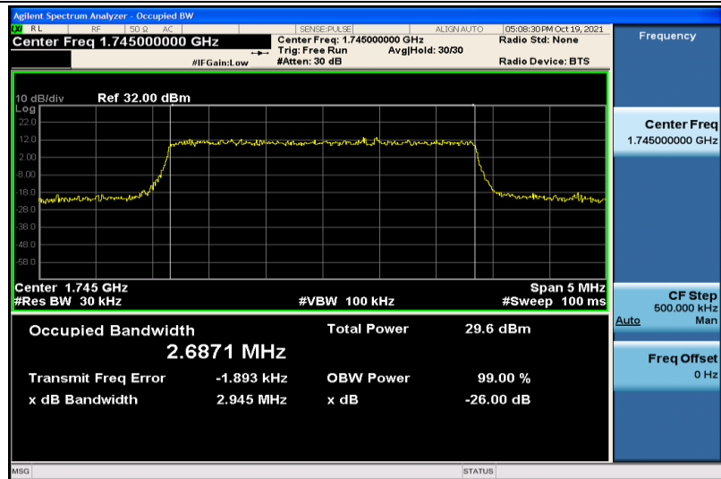
Band66-3MHz-16QAM-132322-15RB#0-2.6871
