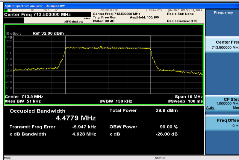
Band17-5MHz-16QAM-23825-25RB#0-4.4779
