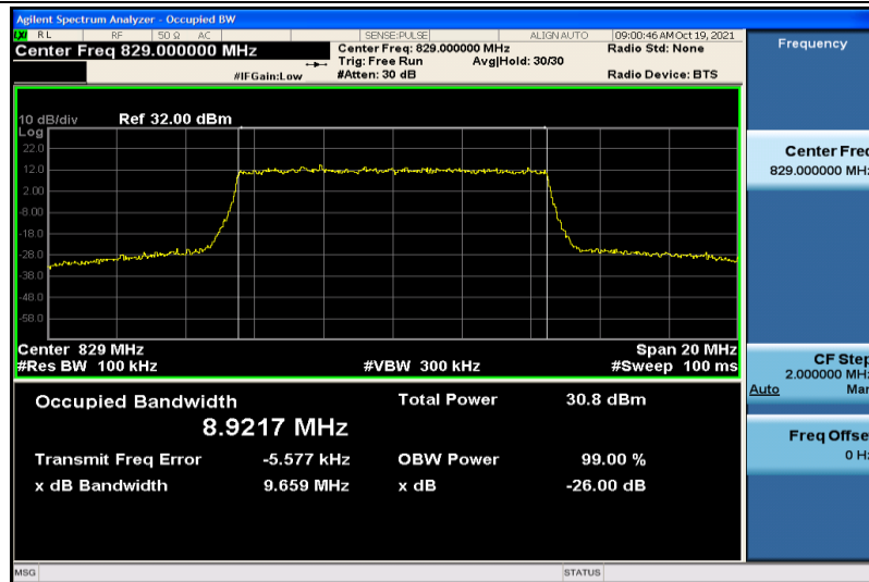
Band5-10MHz-QPSK-20450-50RB#0-8.9217
