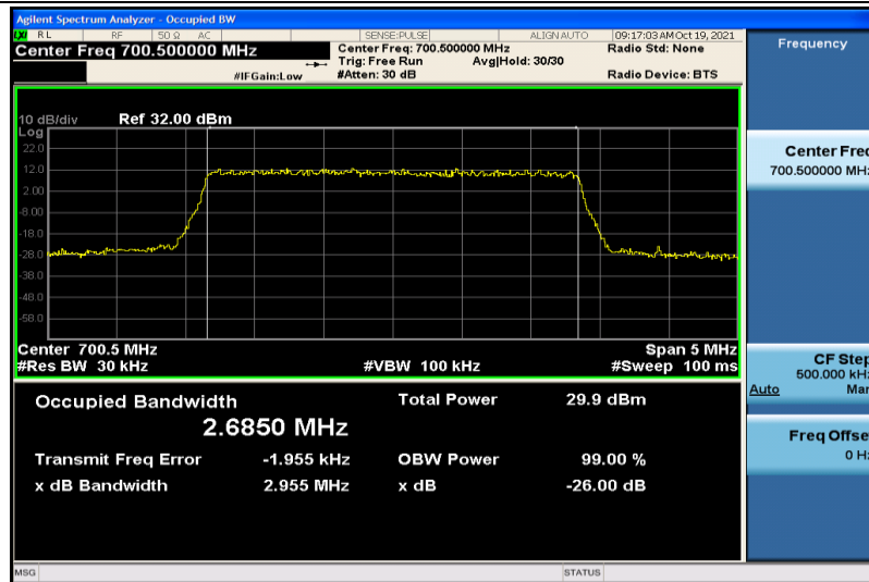
Band12-3MHz-QPSK-23025-15RB#0-2.6850
