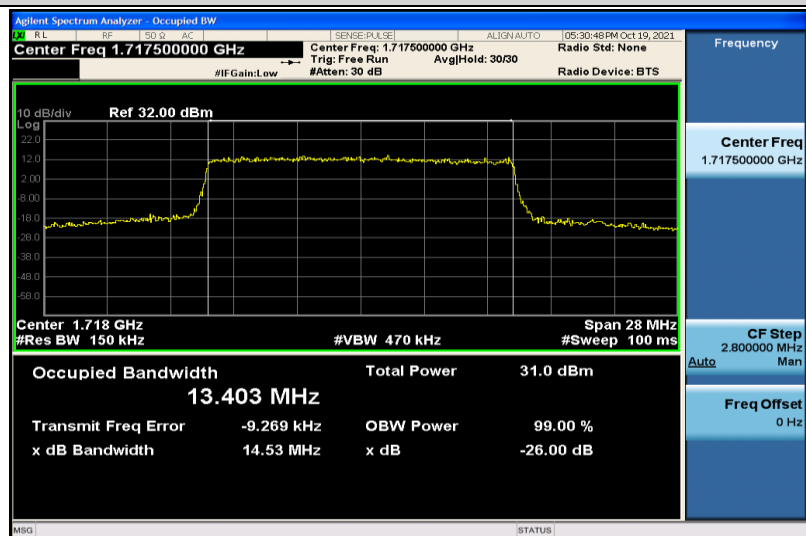
Band66-15MHz-16QAM-132047-75RB#0-13.403
