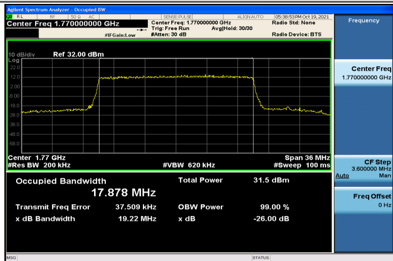
Band66-20MHz-16QAM-132572-100RB#0-17.878
