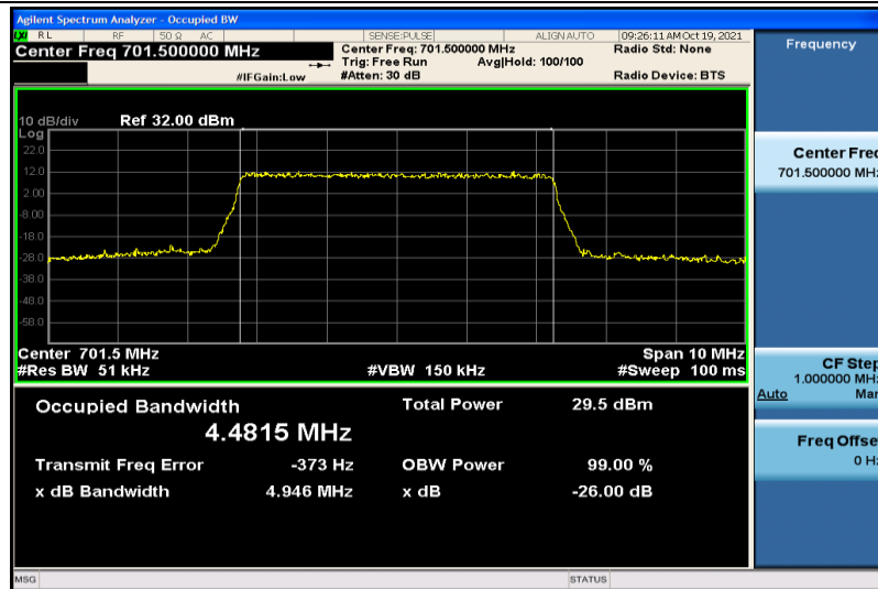
Band12-5MHz-16QAM-23035-25RB#0-4.4815
