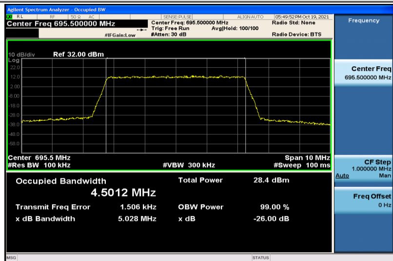
Band71-5MHz-QPSK-133447-25RB#0-4.5012
