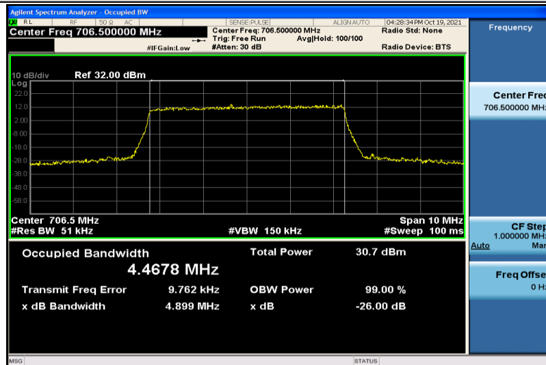
Band17-5MHz-QPSK-23755-25RB#0-4.4678
