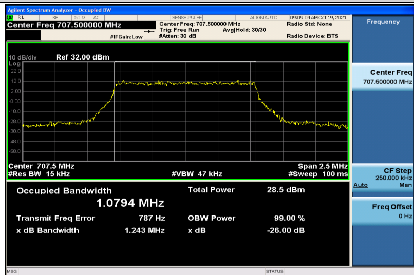
Band12-1.4MHz-16QAM-23095-6RB#0-1.0794
