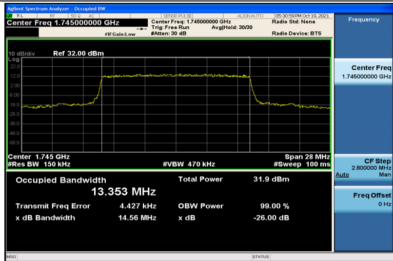
Band66-15MHz-QPSK-132322-75RB#0-13.353
