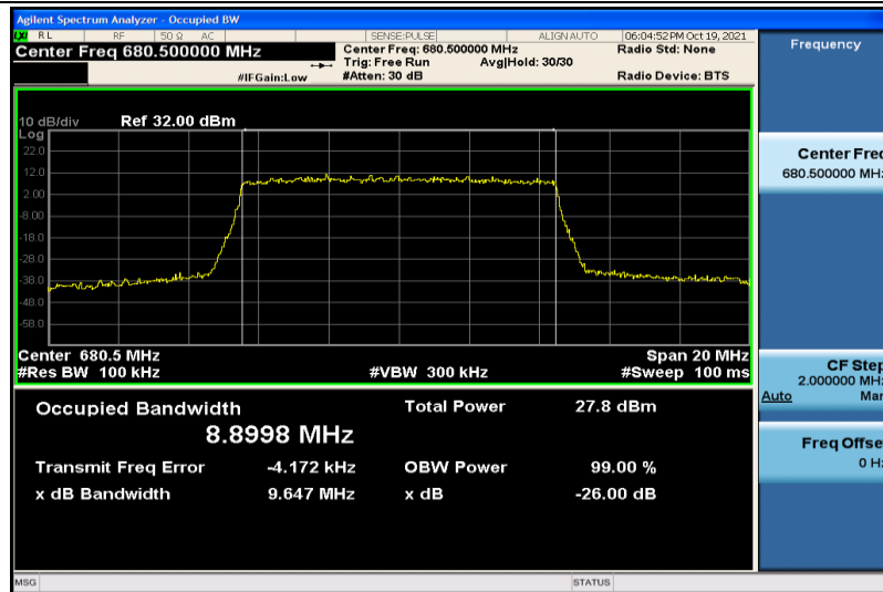
Band71-10MHz-QPSK-133297-50RB#0-8.8998
