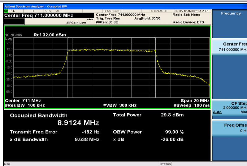
Band12-10MHz-16QAM-23130-50RB#0-8.9124
