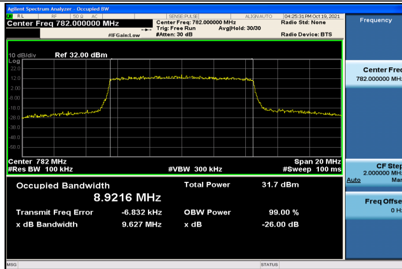
Band13-10MHz-QPSK-23230-50RB#0-8.9216
