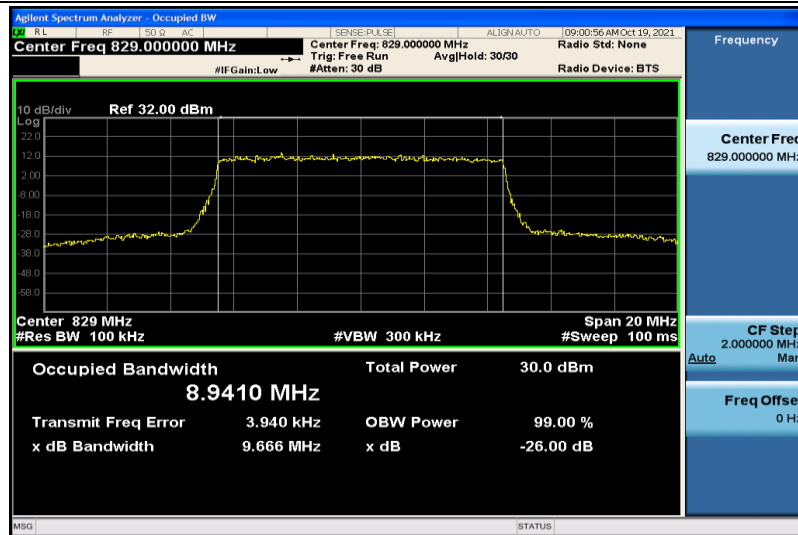
Band5-10MHz-16QAM-20450-50RB#0-8.9410
