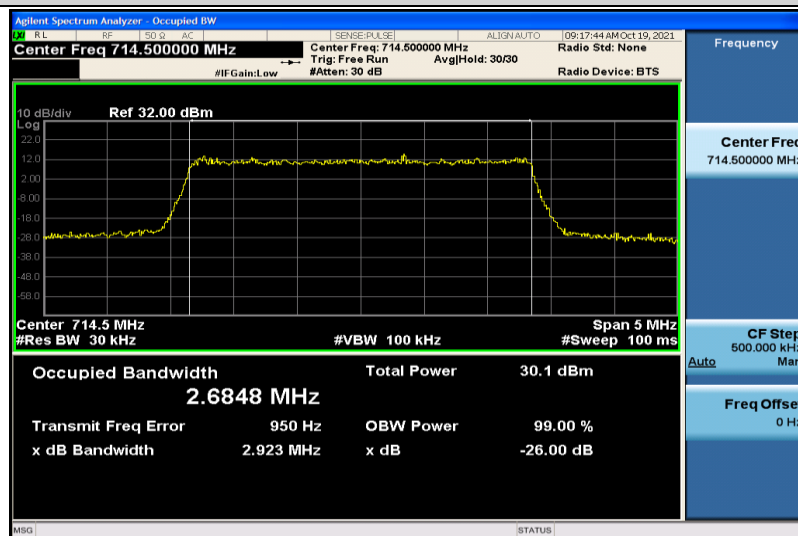
Band12-3MHz-QPSK-23165-15RB#0-2.6848
