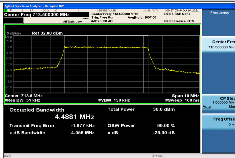
Band12-5MHz-QPSK-23155-25RB#0-4.4881
