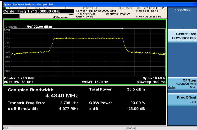
Band66-5MHz-16QAM-131997-25RB#0-4.4840
