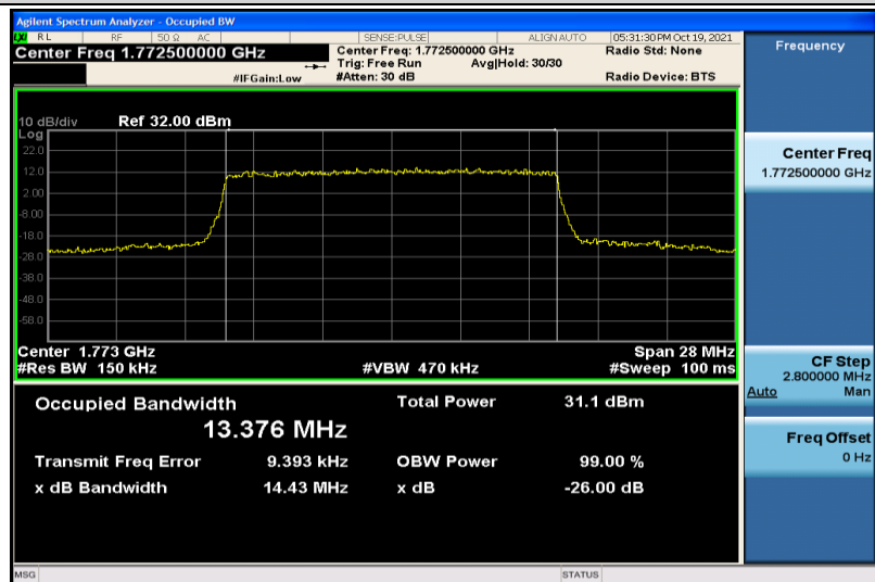
Band66-15MHz-16QAM-132597-75RB#0-13.376
