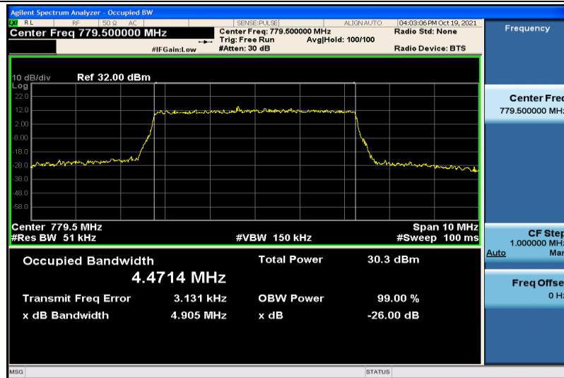
Band13-5MHz-16QAM-23205-25RB#0-4.4714
