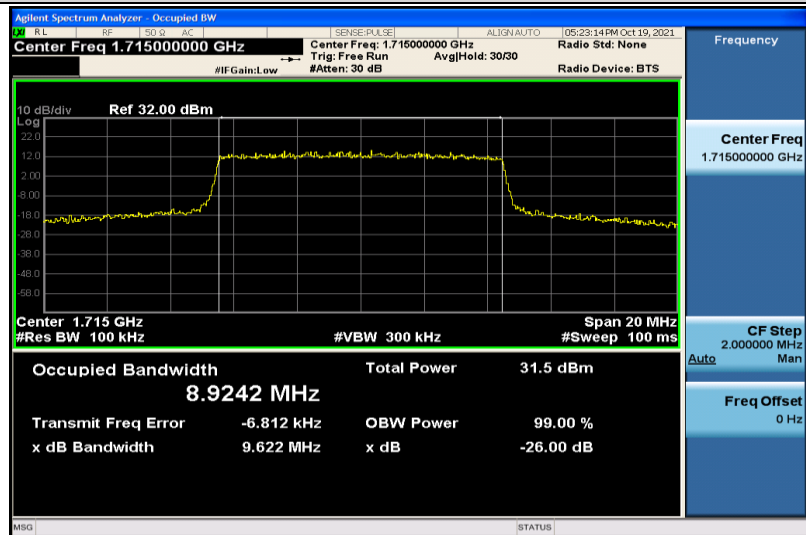
Band66-10MHz-QPSK-132022-50RB#0-8.9242
