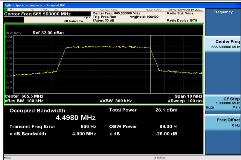
Band71-5MHz-QPSK-133147-25RB#0-4.4980
