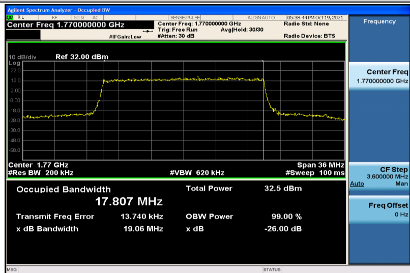
Band66-20MHz-QPSK-132572-100RB#0-17.807
