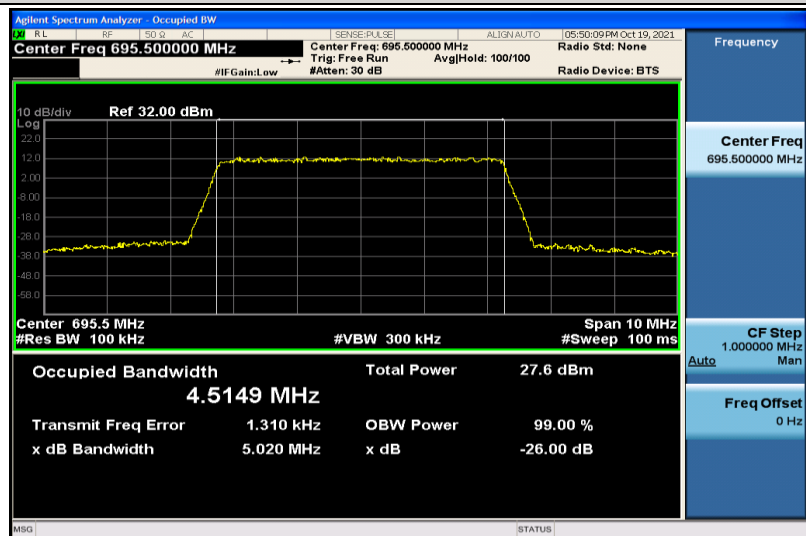
Band71-5MHz-16QAM-133447-25RB#0-4.5149
