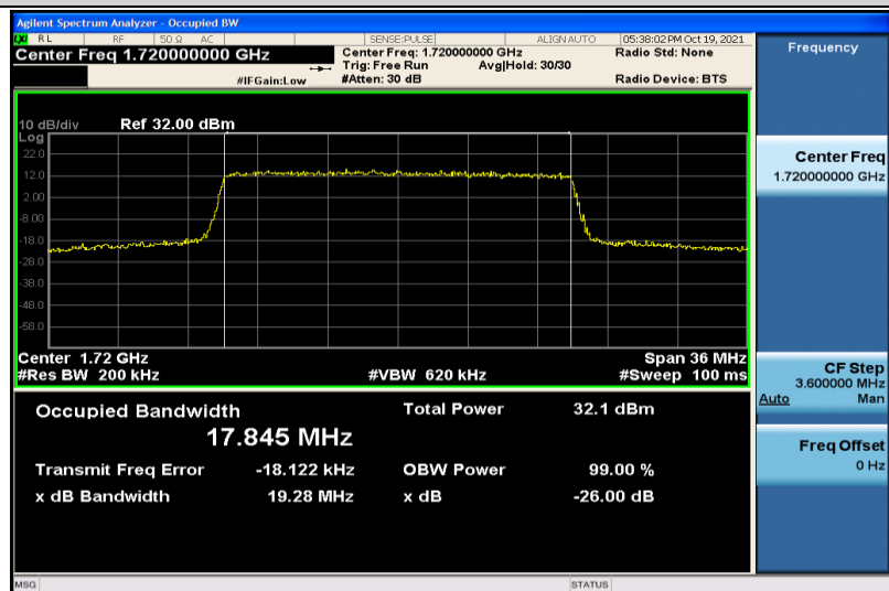
Band66-20MHz-QPSK-132072-100RB#0-17.845
