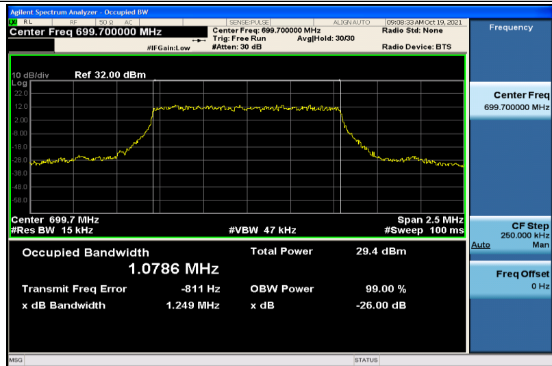
Band12-1.4MHz-QPSK-23017-6RB#0-1.0786
