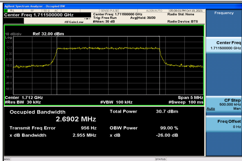
Band66-3MHz-QPSK-131987-15RB#0-2.6902
