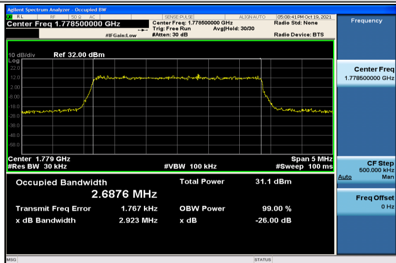
Band66-3MHz-QPSK-132657-15RB#0-2.6876
