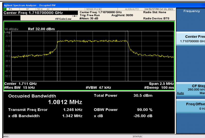
Band66-1.4MHz-QPSK-131979-6RB#0-1.0812
