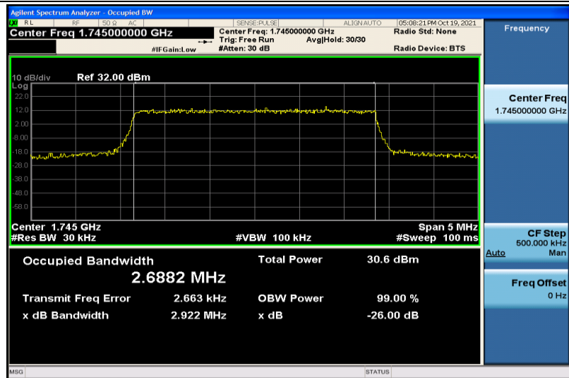
Band66-3MHz-QPSK-132322-15RB#0-2.6882
