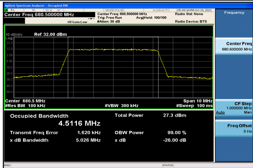
Band71-5MHz-16QAM-133297-25RB#0-4.5116
