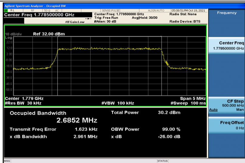
Band66-3MHz-16QAM-132657-15RB#0-2.6852
