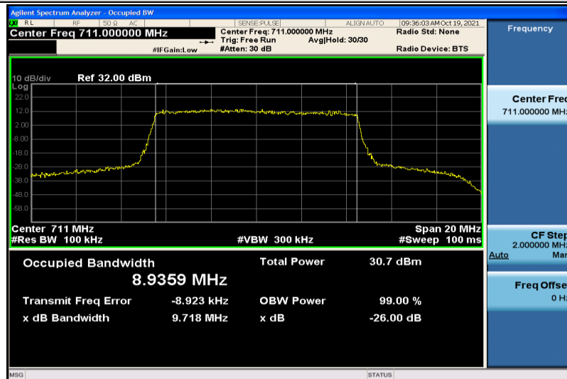
Band12-10MHz-QPSK-23130-50RB#0-8.9359
