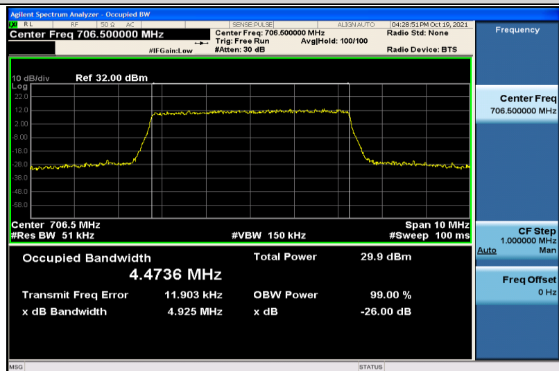
Band17-5MHz-16QAM-23755-25RB#0-4.4736
