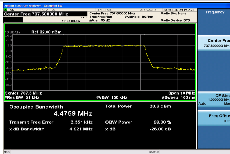
Band12-5MHz-QPSK-23095-25RB#0-4.4759
