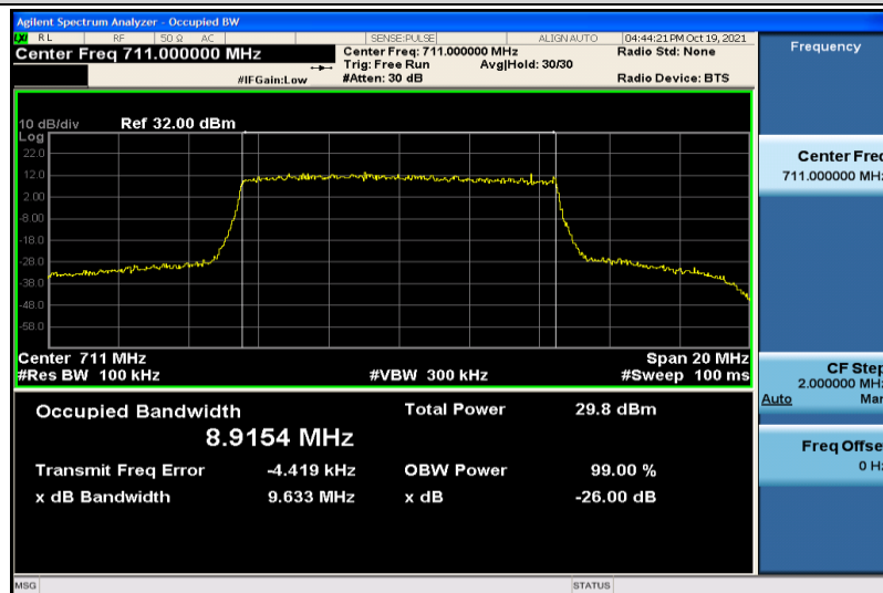
Band17-10MHz-16QAM-23800-50RB#0-8.9154
