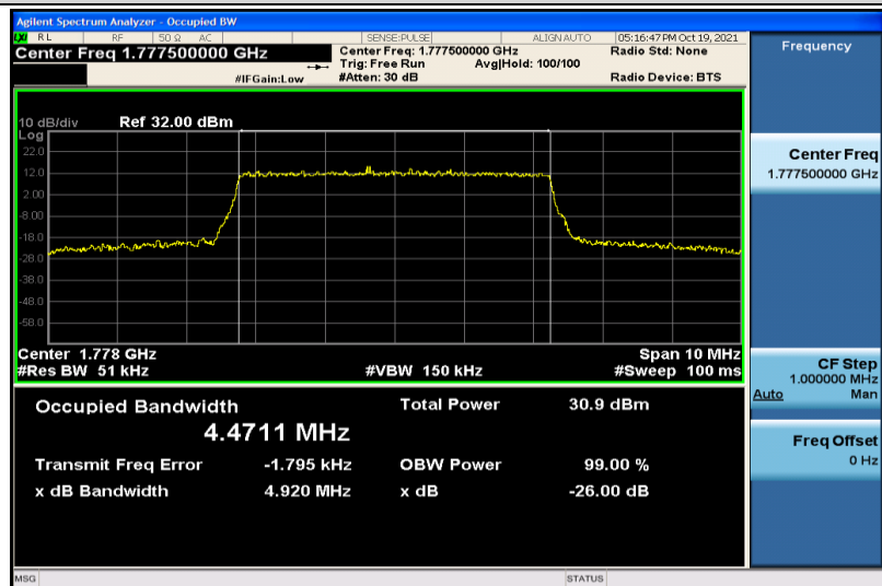
Band66-5MHz-16QAM-132647-25RB#0-4.4711
