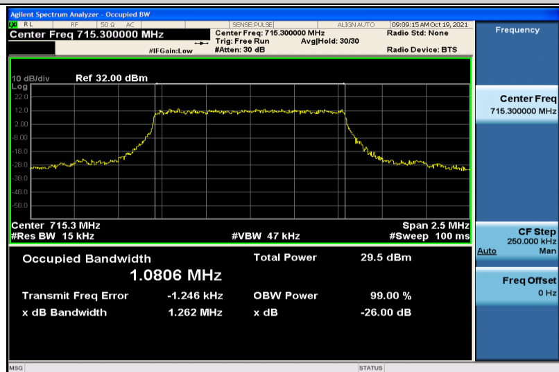
Band12-1.4MHz-QPSK-23173-6RB#0-1.0806
