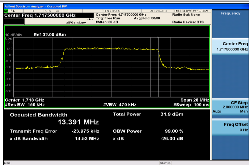
Band66-15MHz-QPSK-132047-75RB#0-13.391
