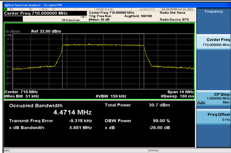
Band17-5MHz-QPSK-23790-25RB#0-4.4714
