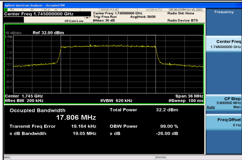
Band66-20MHz-QPSK-132322-100RB#0-17.806
