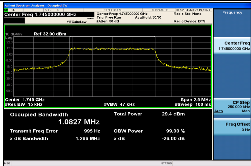
Band66-1.4MHz-16QAM-132322-6RB#0-1.0827
