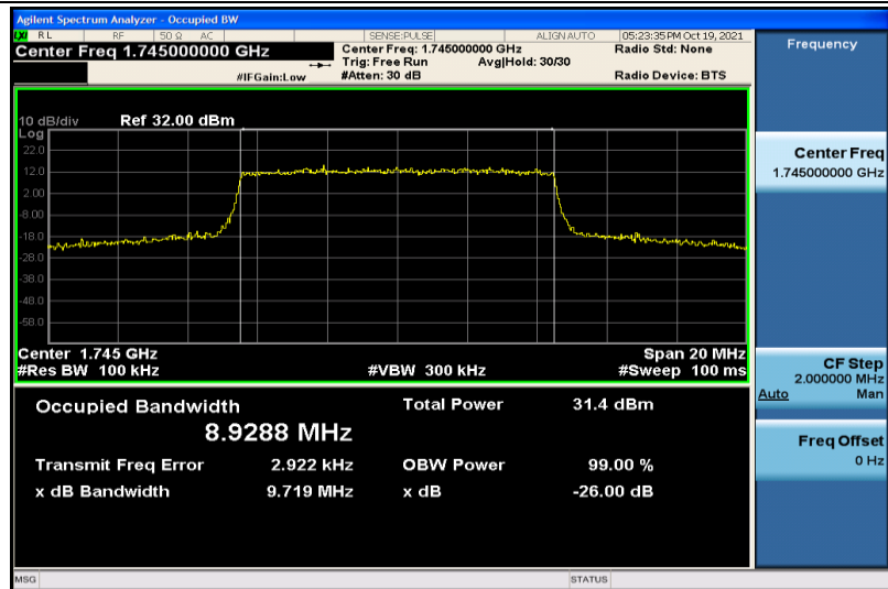
Band66-10MHz-QPSK-132322-50RB#0-8.9288
