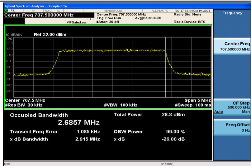
Band12-3MHz-16QAM-23095-15RB#0-2.6857
