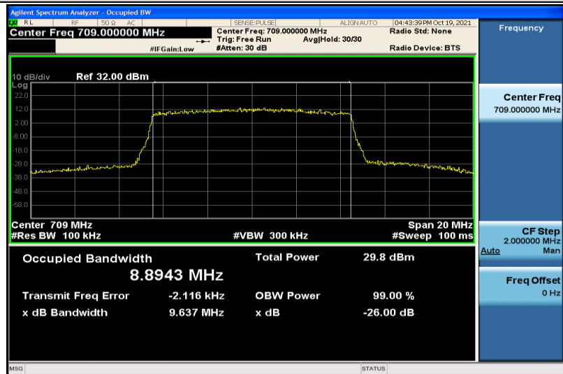
Band17-10MHz-16QAM-23780-50RB#0-8.8943
