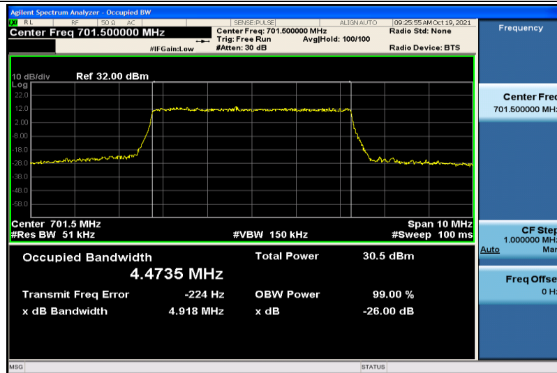
Band12-5MHz-QPSK-23035-25RB#0-4.4735
