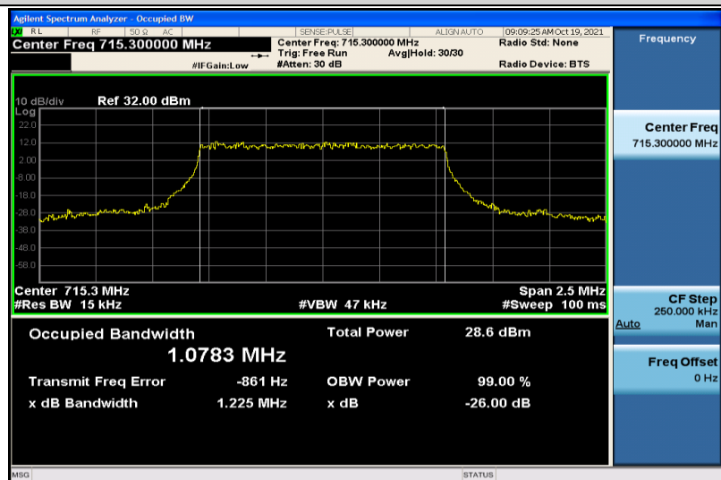
Band12-1.4MHz-16QAM-23173-6RB#0-1.0783
