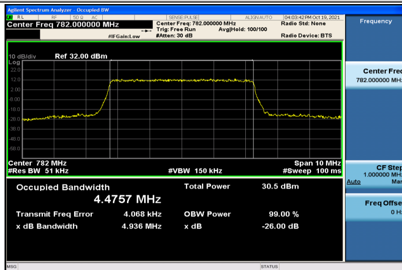
Band13-5MHz-16QAM-23230-25RB#0-4.4757
