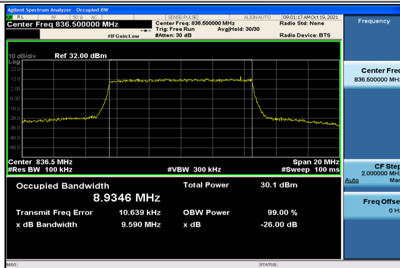
Band5-10MHz-16QAM-20525-50RB#0-8.9346
