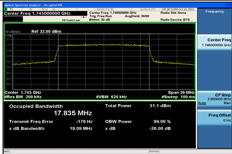
Band66-20MHz-16QAM-132322-100RB#0-17.835
