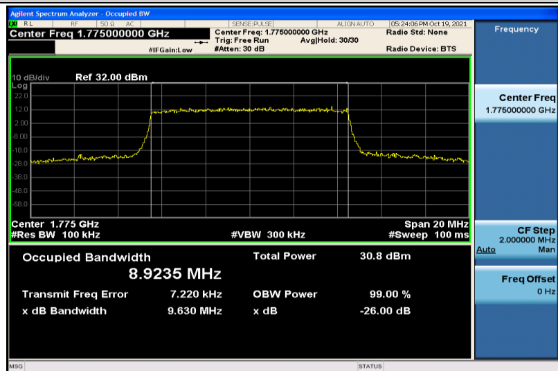
Band66-10MHz-16QAM-132622-50RB#0-8.9235
