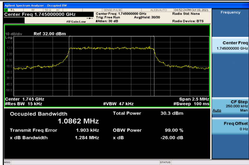
Band66-1.4MHz-QPSK-132322-6RB#0-1.0862
