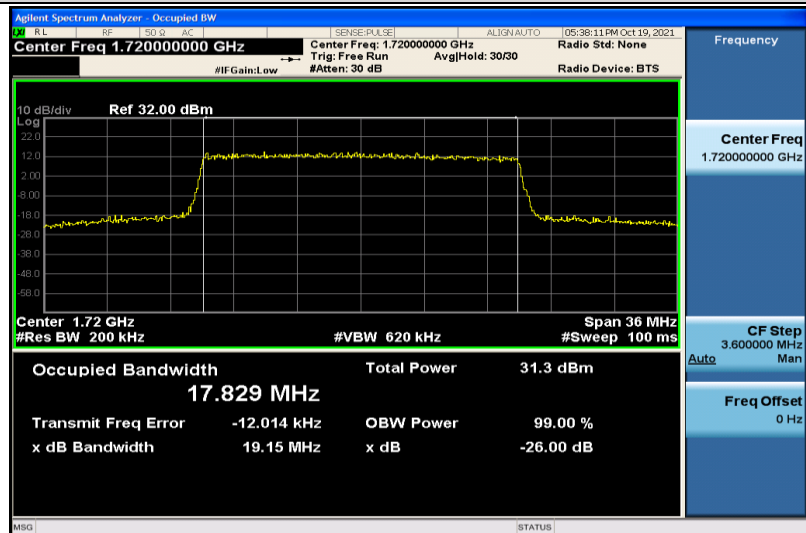
Band66-20MHz-16QAM-132072-100RB#0-17.829
