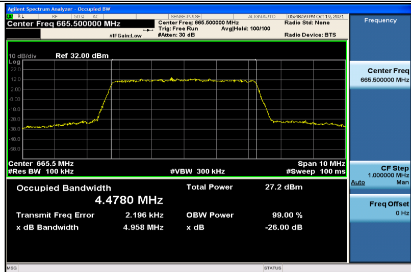
Band71-5MHz-16QAM-133147-25RB#0-4.4780
