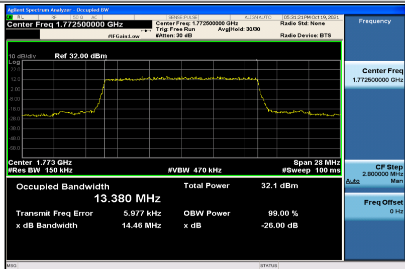
Band66-15MHz-QPSK-132597-75RB#0-13.380
