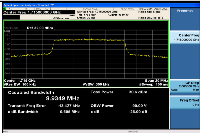
Band66-10MHz-16QAM-132022-50RB#0-8.9349
