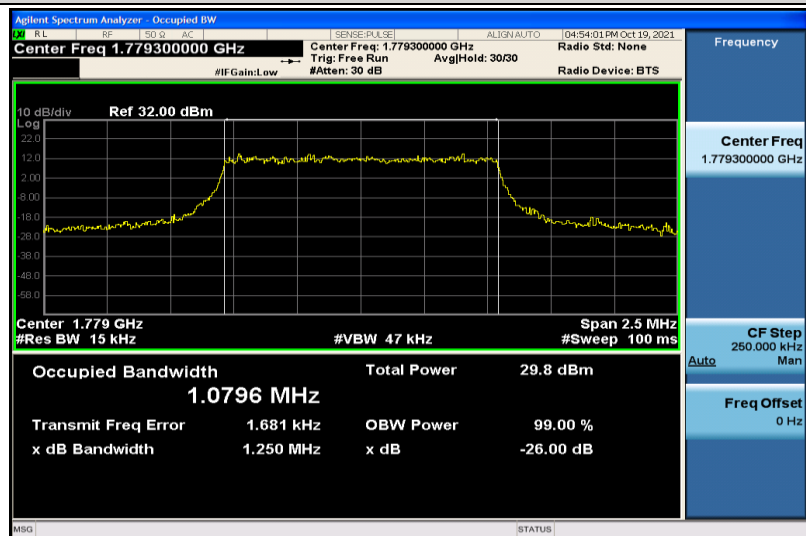
Band66-1.4MHz-16QAM-132665-6RB#0-1.0796
