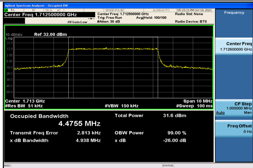
Band66-5MHz-QPSK-131997-25RB#0-4.4755
