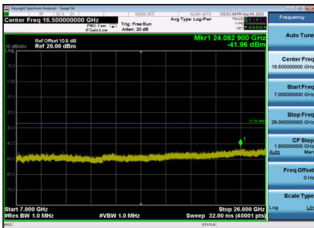
U-NII-2c ,Plot 4,7000MHz~26000MHz-802 .11a(20MHz),5600MHz,Ant1
