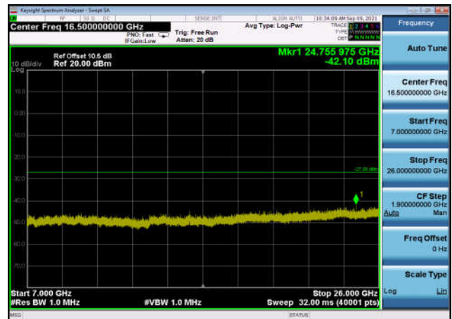
U-NII-2a ,Plot 4,7000MHz~26000MHz-802 .11a(20MHz),5320MHz,Ant1
