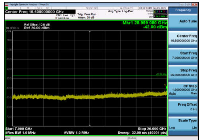
U-NII-2a ,Plot 4,7000MHz~26000MHz-802 .11ac(80MHz),5290MHz,Ant1
