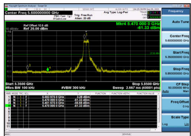
U-NII-2c ,Plot 1,Band Edge-802.11n(20 MHz),5600MHz,Ant1
