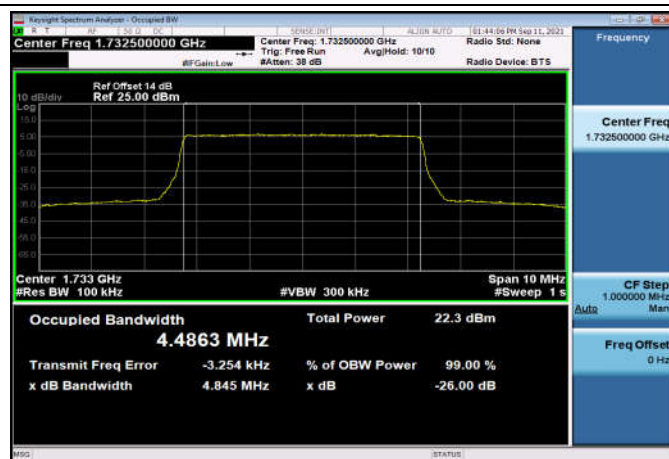
FDD04_MidRange_5_1732.5_Q16
