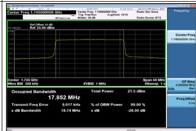
FDD66_MidRange_20_1745_Q16
