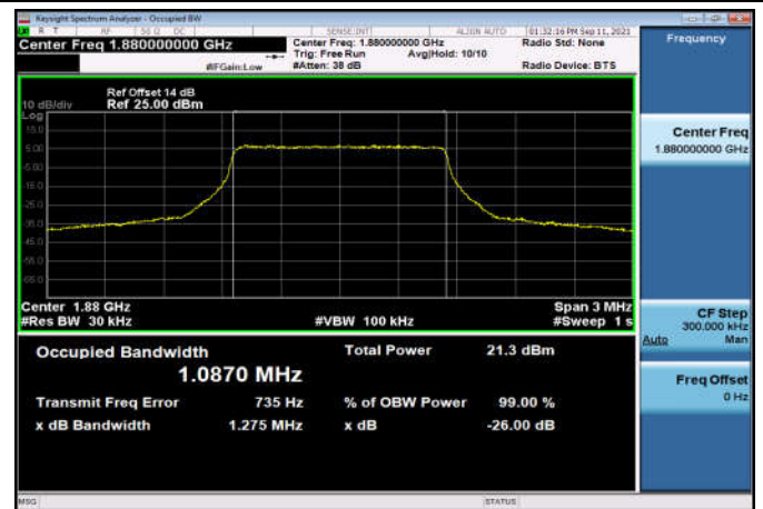
FDD02_MidRange_3_1880_Q16
