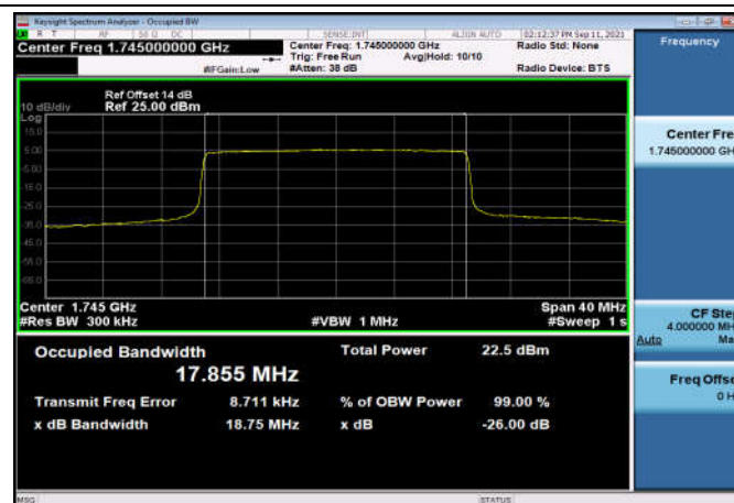
FDD66_MidRange_20_1745_QPSK
