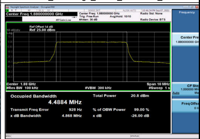
FDD02_MidRange_5MHz_1880MHz_Q16
