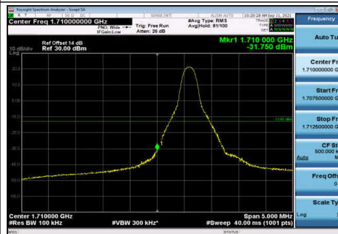
LowRange_FDD04_10MHz_1715_fullIRB _Low_QPSK
