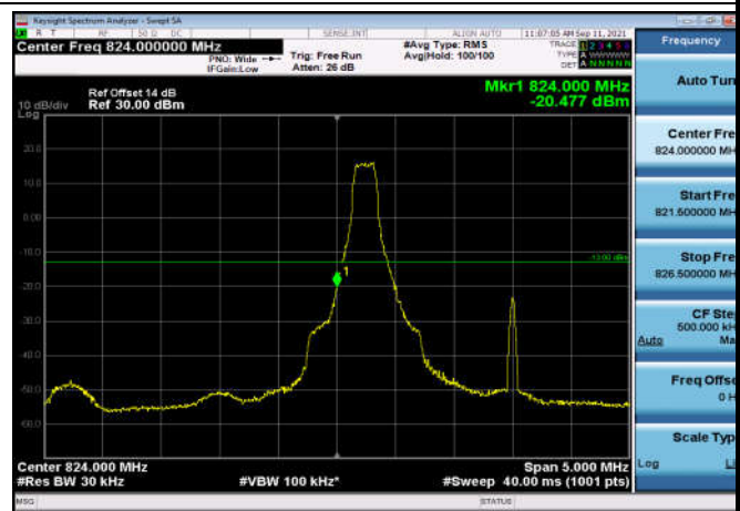
LowRange_FDD05_3MHz_825.5_OneRB _low_Q16
