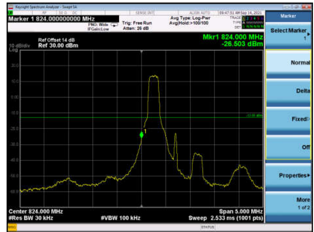
LowRange_FDD05_1.4MHz_824.7_fullIRB _Low_Q16
