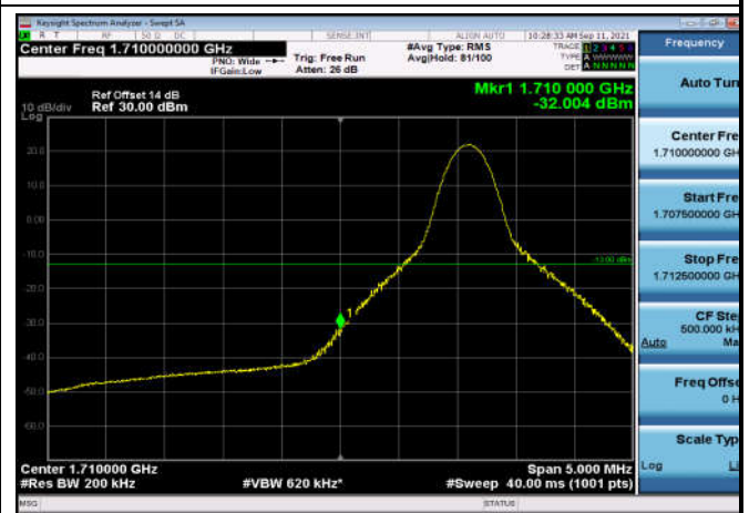
LowRange_FDD04_20MHz_1720_OneRB _low_Q16
