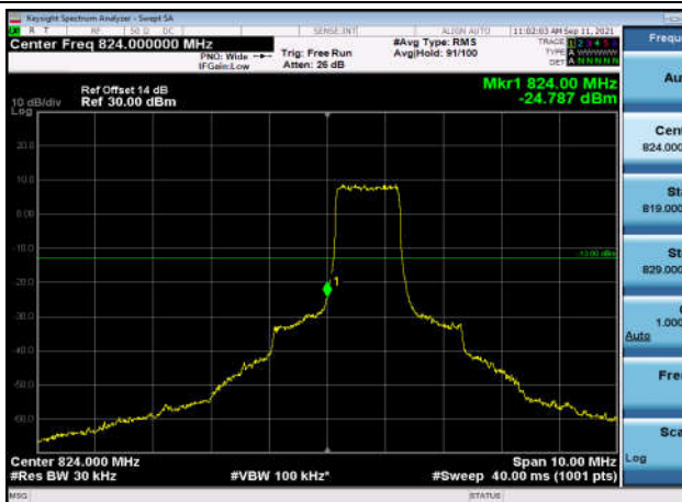
LowRange_FDD05_3MHz_825.5_OneRB _low_QPSK
