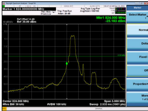
LowRange_FDD05_1.4MHz_824.7_fullIRB _Low_QPSK
