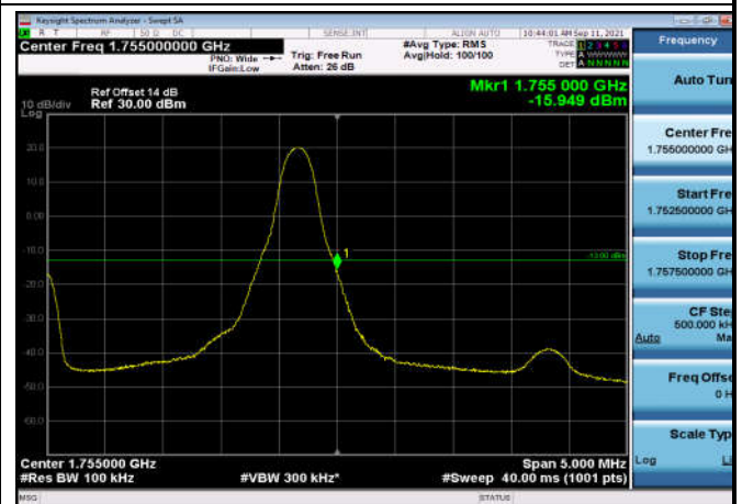
HighRange_FDD04_5MHz_1752.5_fullIRB _High_Q16
