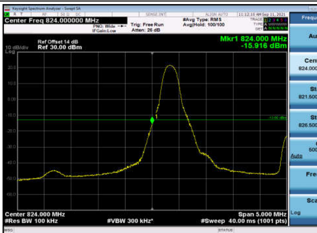
LowRange_FDD05_5MHz_826.5_fullIRB _Low_QPSK
