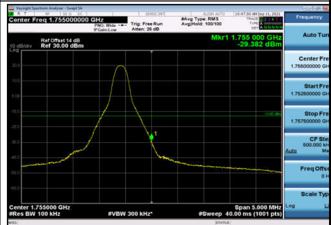
HighRange_FDD04_10MHz_1750_fullIRB _High_Q16
