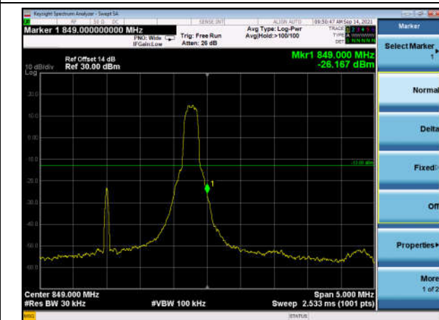
HighRange_ FDD05_3MHz_847.5_fullIRB _High_QPSK
