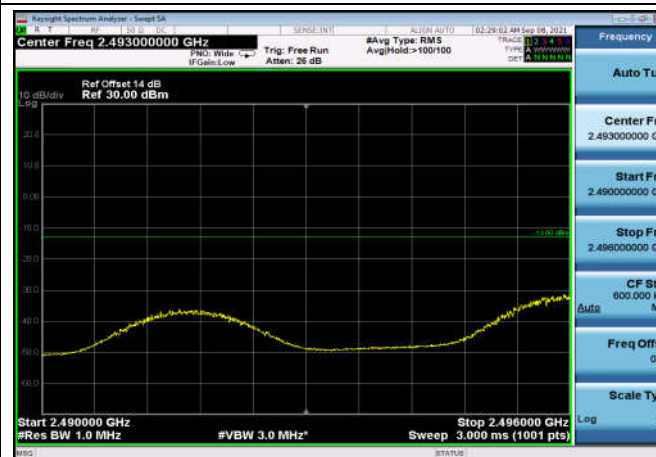
LowRange_FDD07_5MHz_2502.5_fullRB_Low_Q16
