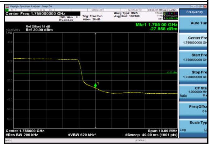
HighRange_FDD04_20MHz_1745_fullRB _High_Q16
