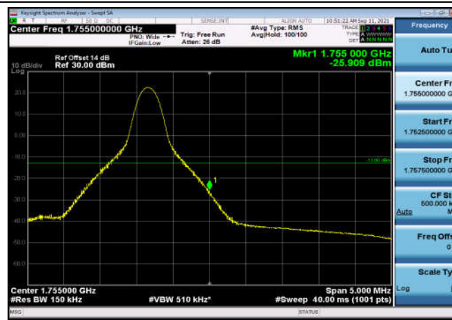
HighRange_FDD04_15MHz_1747.5_OneRB _high_QPSK
