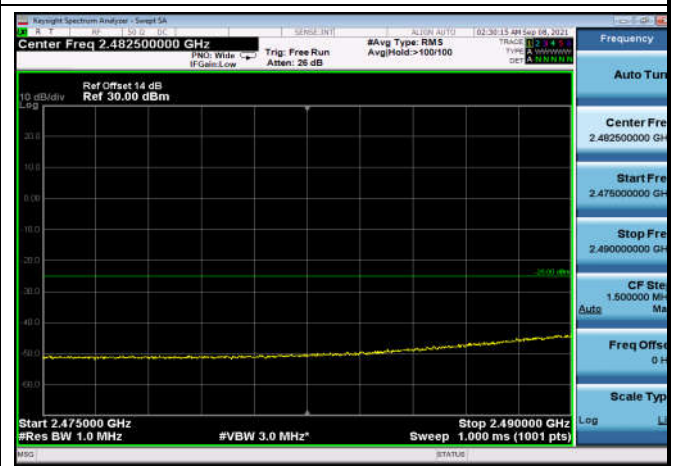
FDD07_5MHz_2502.5_Q16_fullRB_ExtraBands_Range_2475~2490
