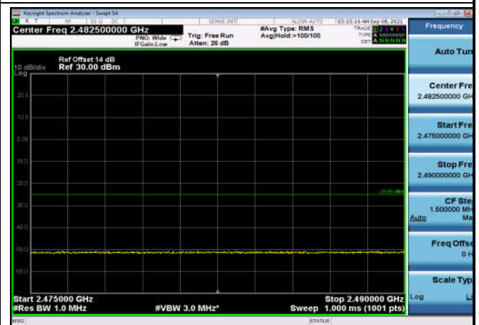
FDD07_15MHz_2562.5_QPSK_fullRB _ExtraBands_Range_2475~2490
