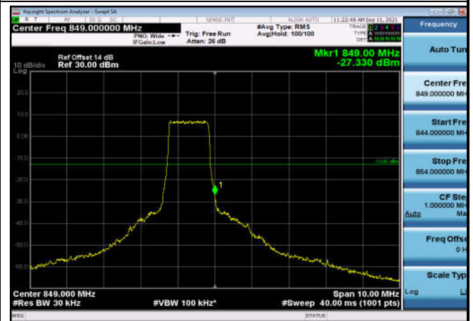
HighRange_ FDD05_3MHz_847.5_OneRB _high_Q16
