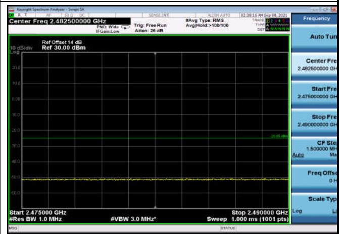
FDD07_10MHz_2505_Q16_fullRB_ExtraBand s_Range_2475~2490
