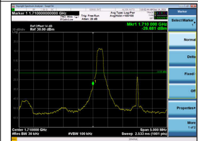
LowRange_FDD66_5MHz_1712.5_OneRB _low_Q16
