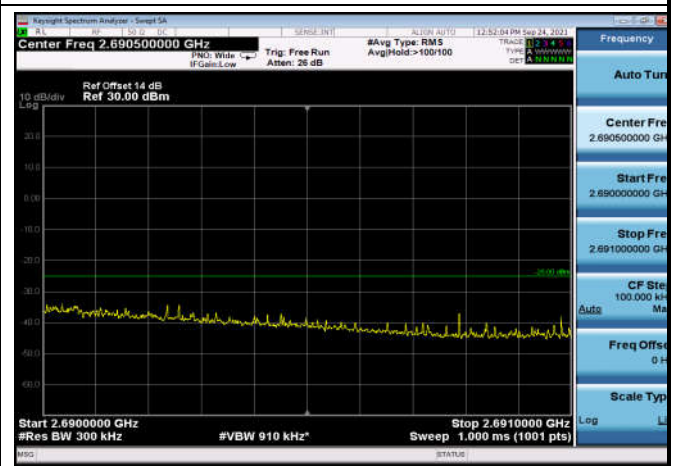
TDD41_15MHz_2682.5_Q16_FullRB_High _ExtraBands_Range_2690~2691
