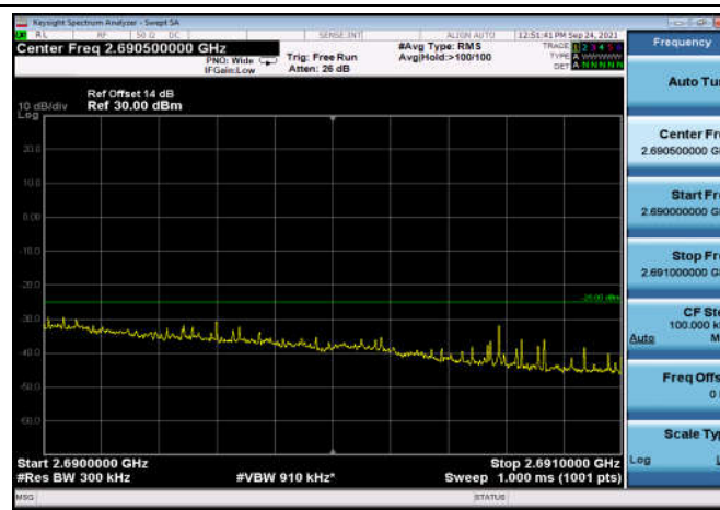
TDD41_15MHz_2682.5_QPSK_FullRB _High_ExtraBands_Range_2690~2691
