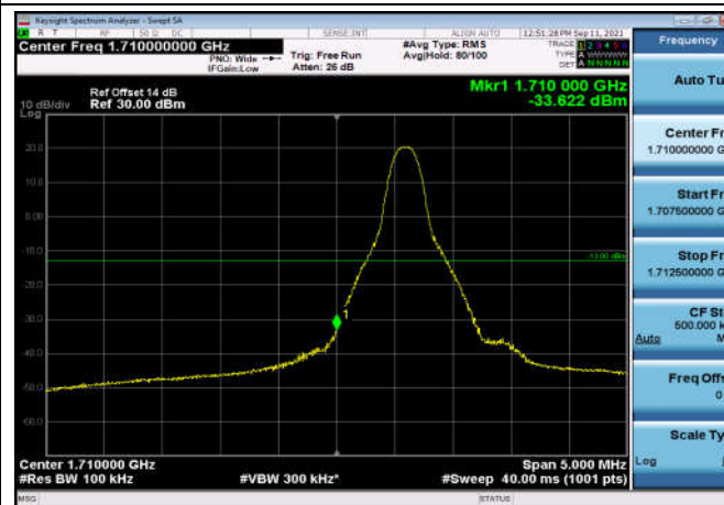
LowRange_FDD66_10MHz_1715_fullIRB _Low_QPSK
