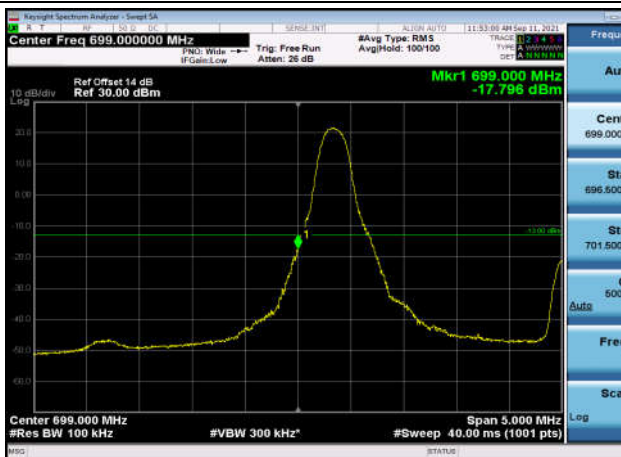
LowRange_FDD12_5MHz_701.5_fullIRB _Low_QPSK
