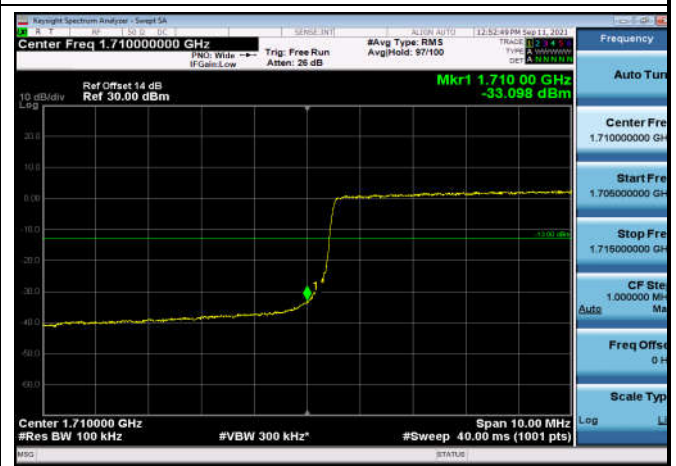
LowRange_FDD66_10MHz_1715_fullIRB _Low_Q16
