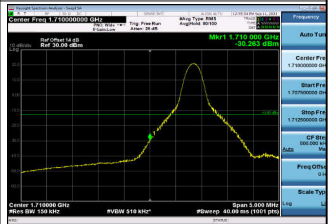
LowRange_FDD66_15MHz_1717.5_fullIRB _Low_Q16
