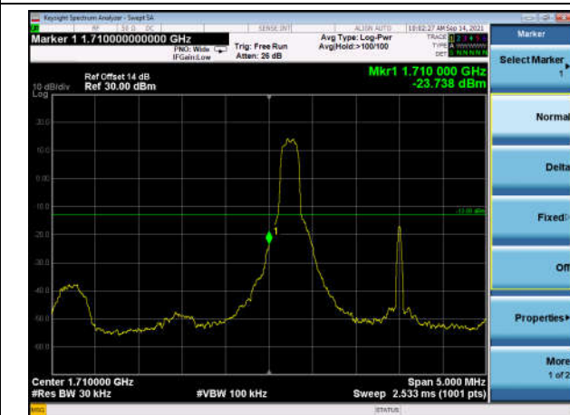
LowRange_FDD66_5MHz_1712.5_OneRB _low_QPSK
