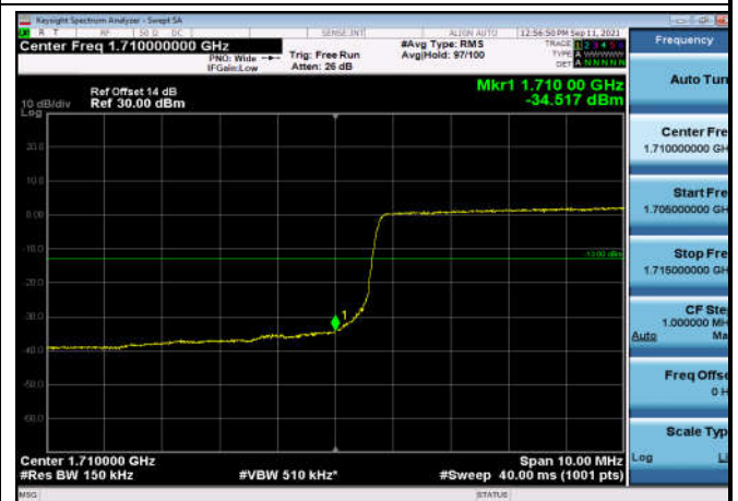
LowRange_FDD66_20MHz_1720_OneRB _low_Q16
