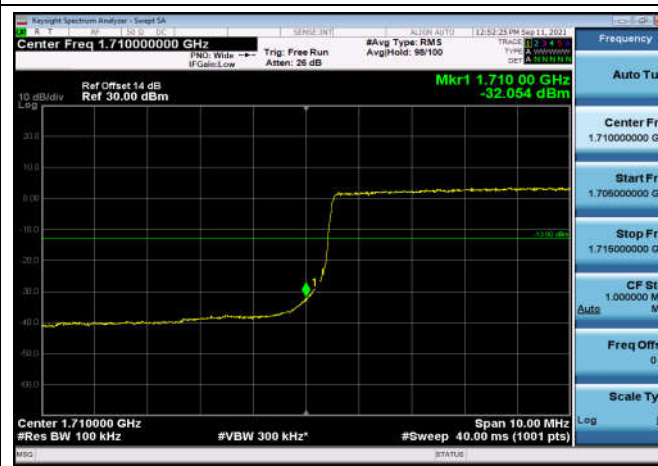
LowRange_FDD66_10MHz_1715_fullIRB _Low_QPSK
