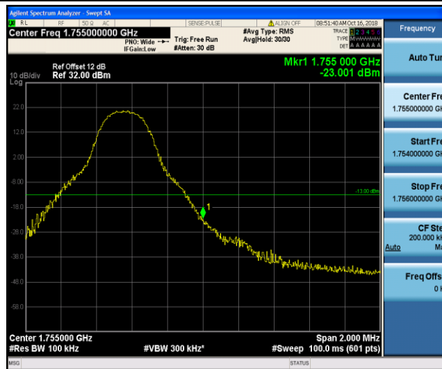
Band4_5MHz_QPSK_20375_1RB#24
