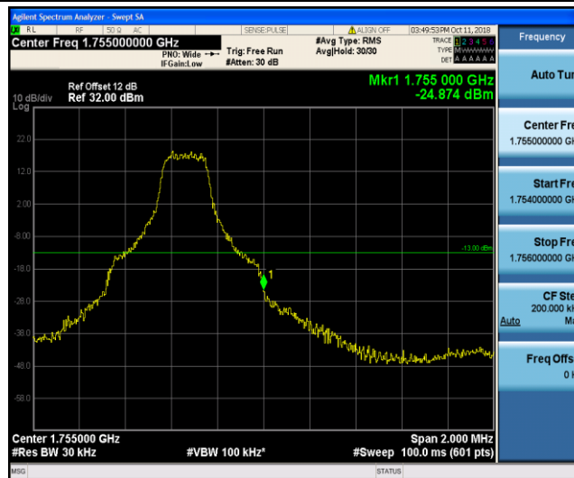
Band4_3MHz_QPSK_20385_1RB#14
