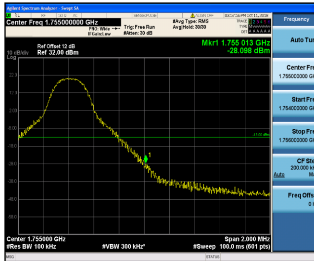
Band4_10MHz_16QAM_20350_1RB#49
