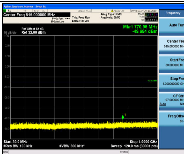
Band2 5MHz 16QAM 18625 1RB#0
