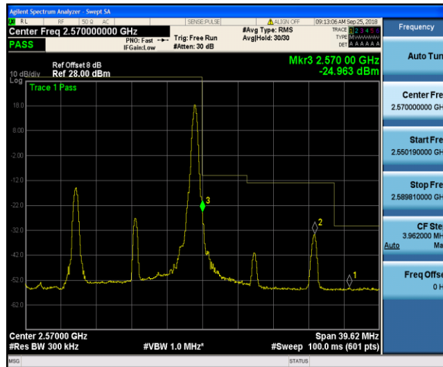
Band7_15MHz_16QAM_21375_1RB#74
