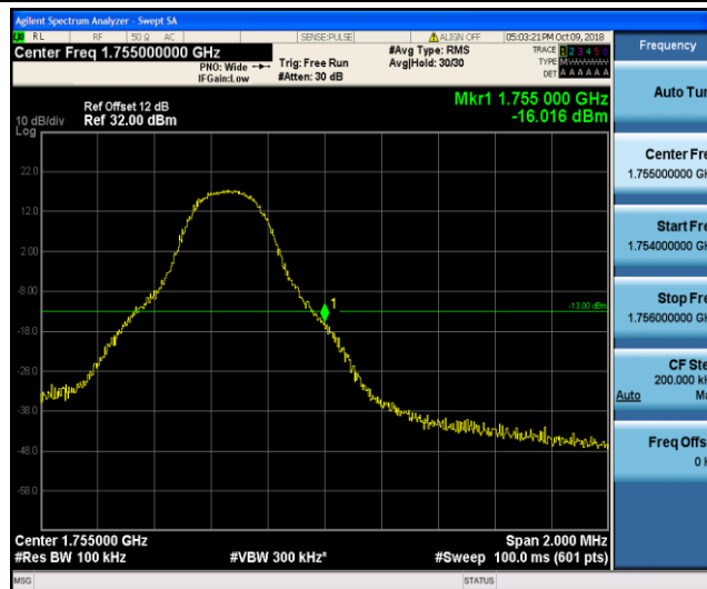
Band4_5MHz_16QAM_20375_1RB#24
