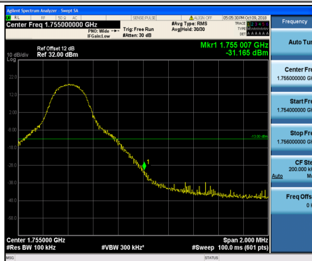
Band4_10MHz_QPSK_20350_1RB#49
