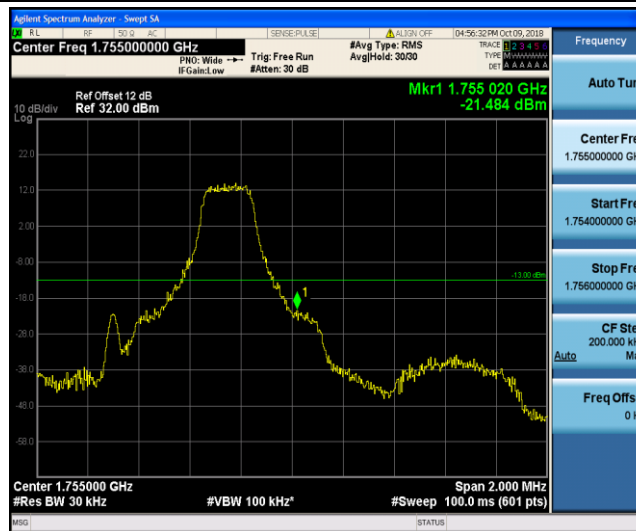
Band4_1.4MHz_16QAM_20393_1RB#5
