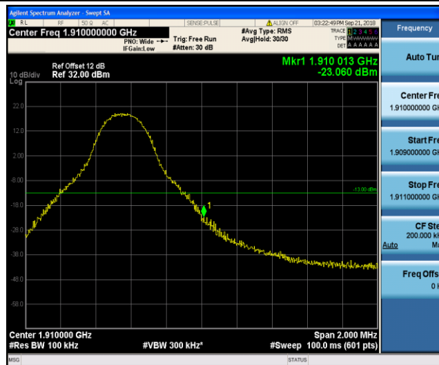
Band2_5MHz_16QAM_19175_1RB#24
