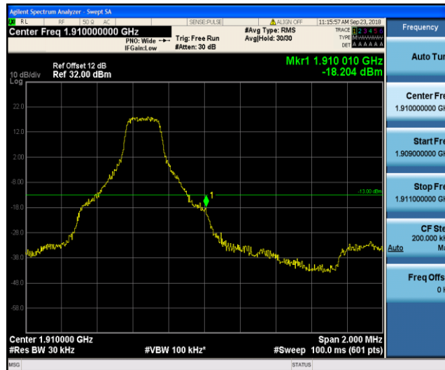
Band2_3MHz_QPSK_19185_1RB#14
