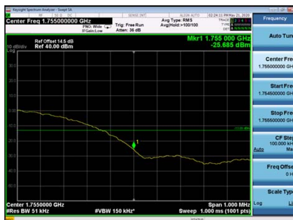
(Plot N: WCDMA 1700 Channel = 1513)
