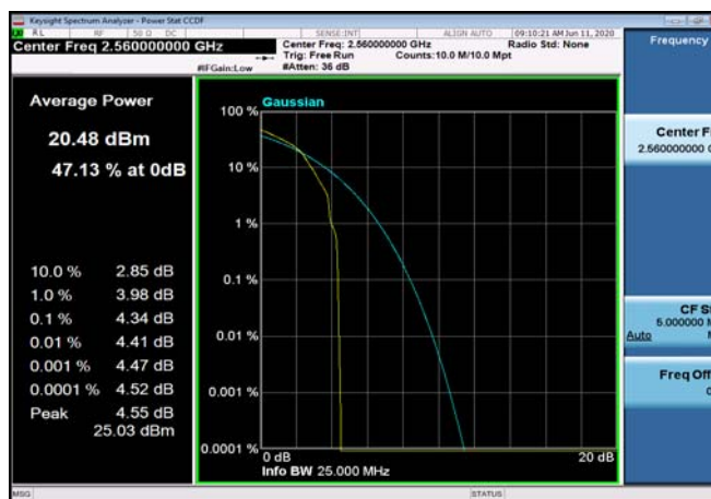
FDD07_HighRange_20MHz_2560_OneRB _high_Q16
