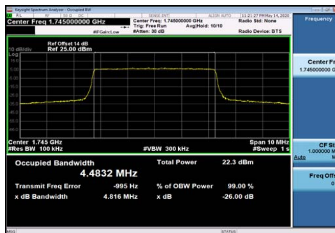
FDD66_MidRange_5_1745_Q16
