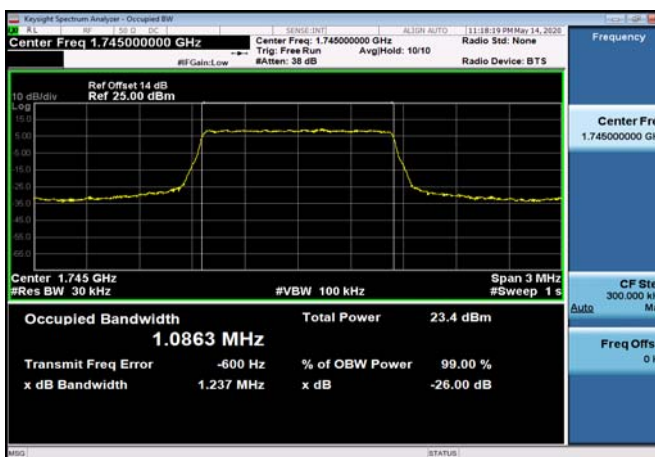
FDD66_MidRange_3_1745_QPSK
