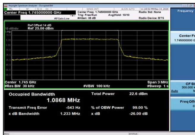
FDD66_MidRange_3_1745_Q16
