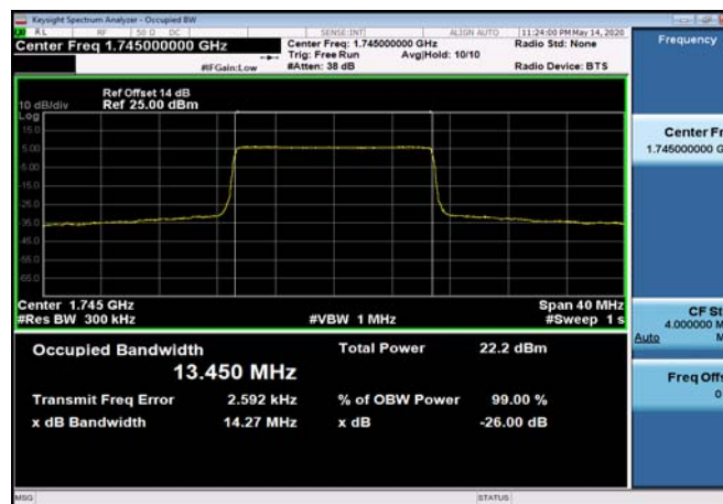
FDD66_MidRange_20_1745_Q16
