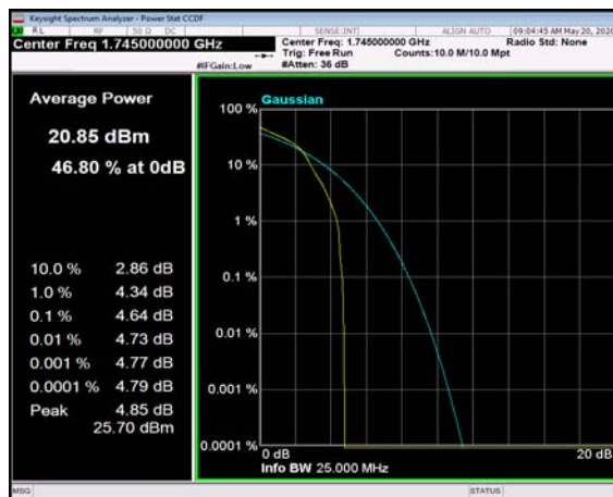
FDD04_HighRange_20MHz_1745_OneRB _high_Q16
