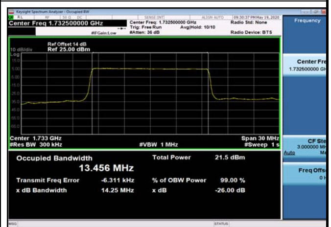
FDD04_MidRange_15MHz_1732.5MHz_Q16
