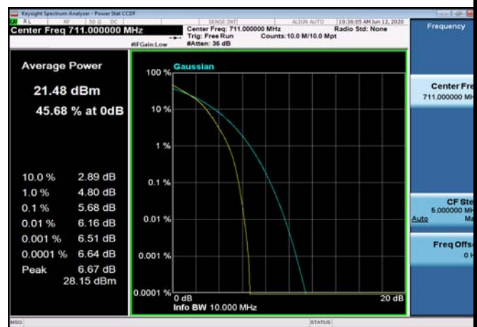
FDD12_HighRange_10MHz_711_fullRB _Q16
