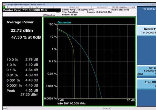
FDD12_HighRange_10MHz_711_OneRB _high_Q16
