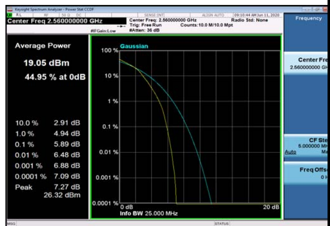
FDD07_HighRange_20MHz_2560_fullRB _Q16
