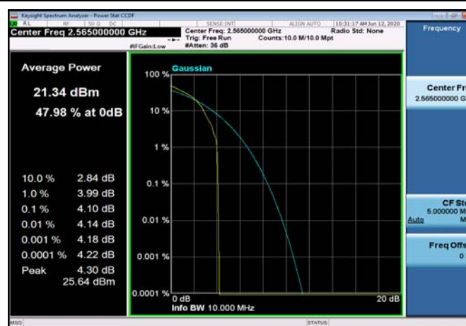
FDD07_HighRange_10MHz_2565_OneRB _high_Q16
