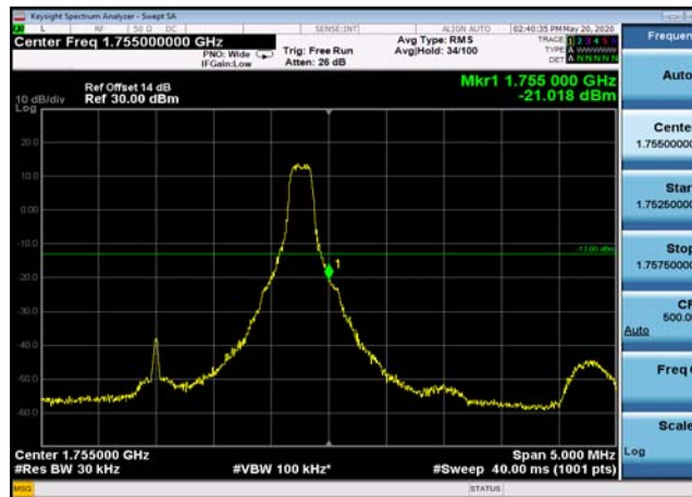
HighRange_FDD04_3MHz_1753.5_fullRB _High_QPSK
