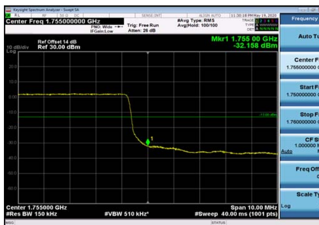
HighRange_FDD04_20MHz_1745_OneRB _high_QPSK
