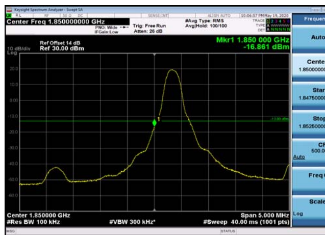
LowRange_FDD02_5MHz_1852.5_OneRB _low_QPSK
