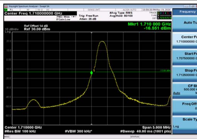
LowRange_FDD04_5MHz_1712.5_OneRB _low_QPSK
