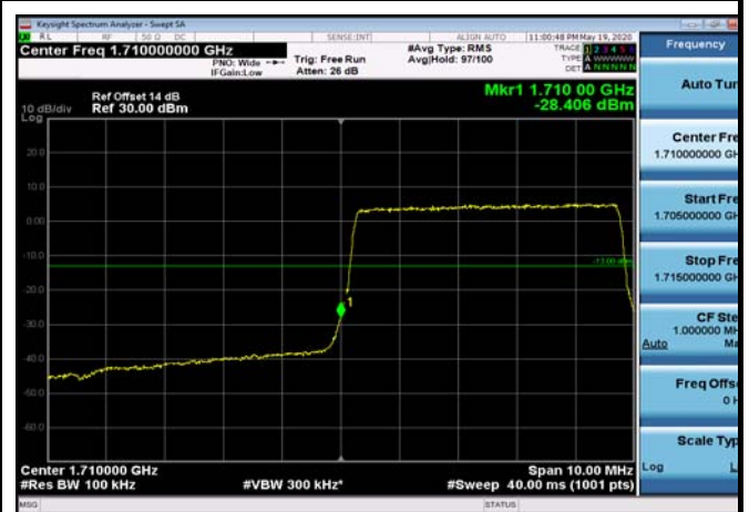
LowRange_FDD04_10MHz_1715_OneRB _low_Q16
