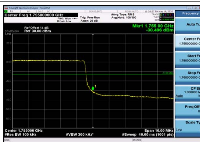
HighRange_FDD04_10MHz_1750_fullRB _High_QPSK
