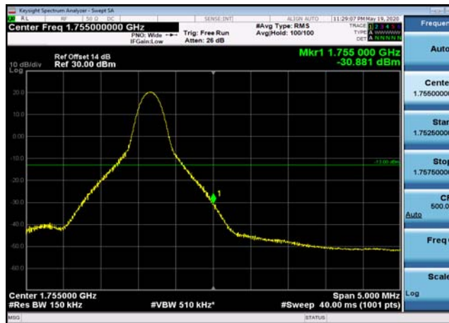
HighRange_FDD04_15MHz_1747.5_fullRB _High_QPSK
