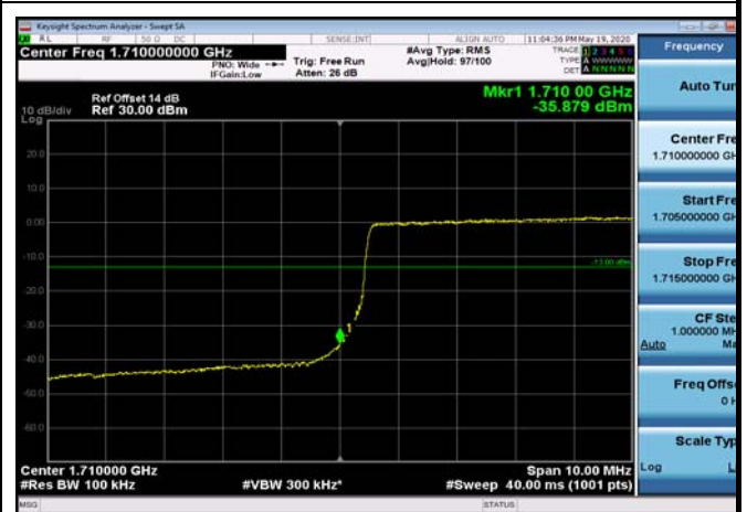
LowRange_FDD04_10MHz_1715_fullIRB _Low_Q16
