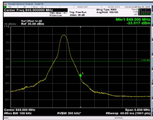
HighRange_FDD05_10MHz_844_fullRB _High_QPSK
