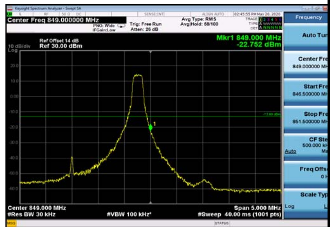
HighRange_FDD05_3MHz_847.5_OneRB _high_Q16
