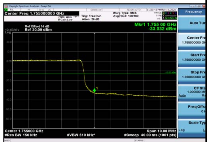
HighRange_FDD04_20MHz_1745_OneRB _high_Q16
