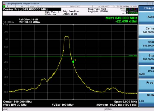
HighRange_FDD05_1.4MHz_848.3_fullRB _High_QPSK
