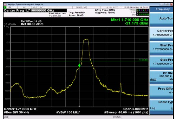
LowRange_FDD04_3MHz_1711.5_fullRB _Low_Q16
