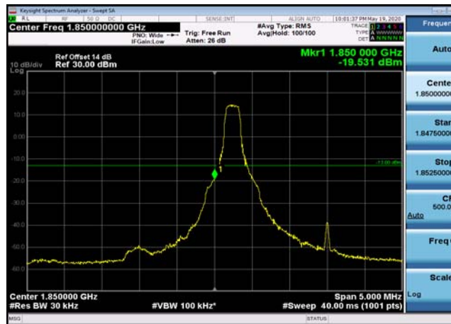
LowRange_FDD02_3MHz_1851.5_fullIRB _Low_QPSK
