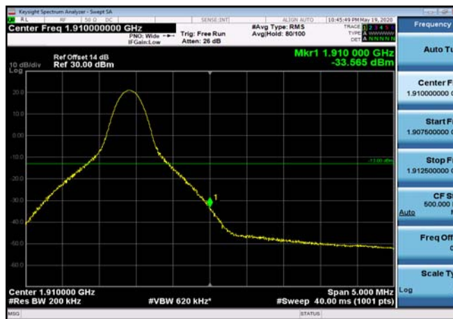
HighRange_FDD02_20MHz_1900_OneRB _high_QPSK
