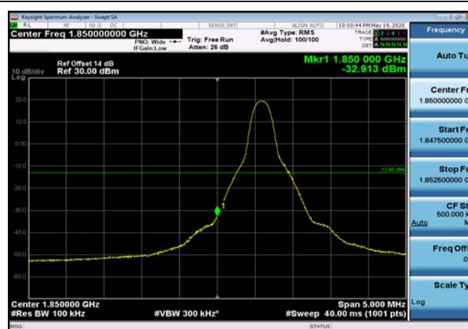
LowRange_FDD02_10MHz_1855_fullRB _Low_QPSK
