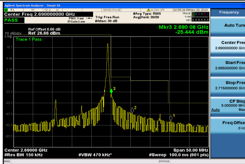
Band41-15MHz-QPSK-41515-1RB#74
