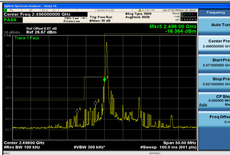
Band41-10MHz-QPSK-39700-1RB#0
