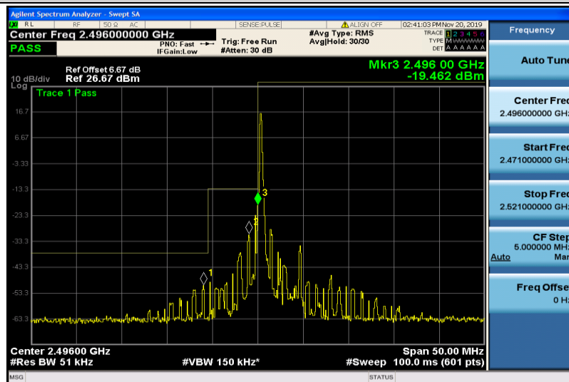
Band41-5MHz-16QAM-39675-1RB#0
