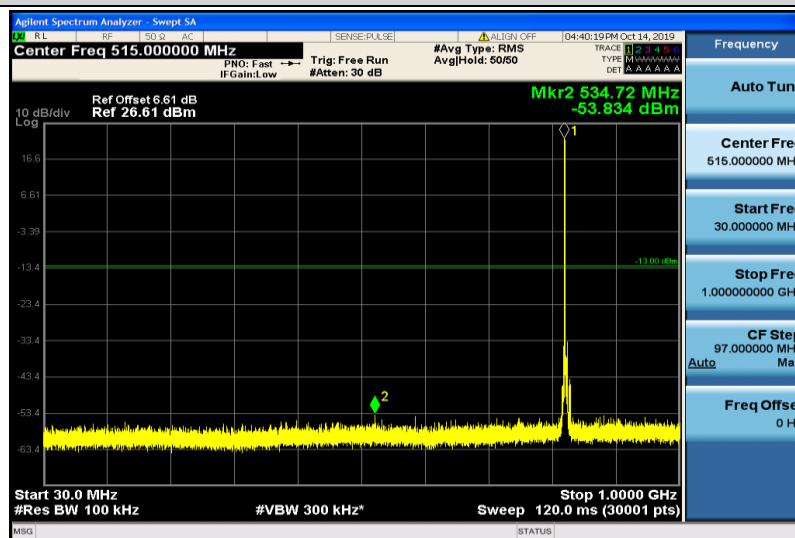
Band5-5MHz-16QAM-20425-1RB#0-30~1000MHz
