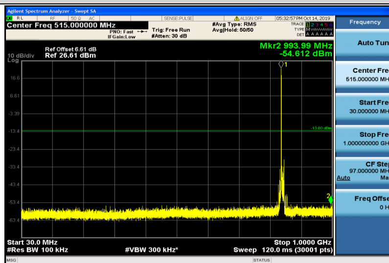
Band5-10MHz-QPSK-20600-1RB#0-30~1000MHz
