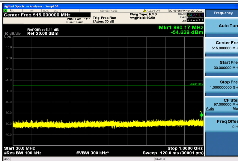
Band41-5MHz-16QAM-41565-1RB#0-30~1000MHz
