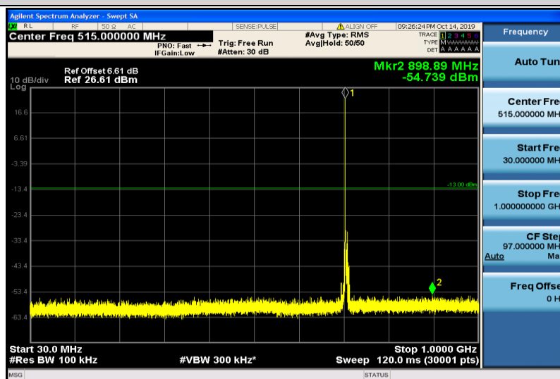
Band12-5MHz-16QAM-23155-1RB#0-30~1000MHz
