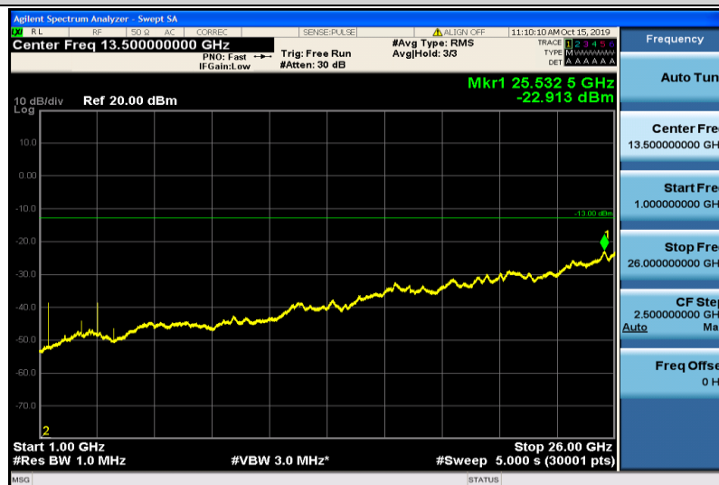
Band17-5MHz-QPSK-23755-1RB#0-1000~26000MHz
