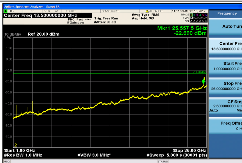
Band17-5MHz-QPSK-23790-1RB#0-1000~26000MHz
