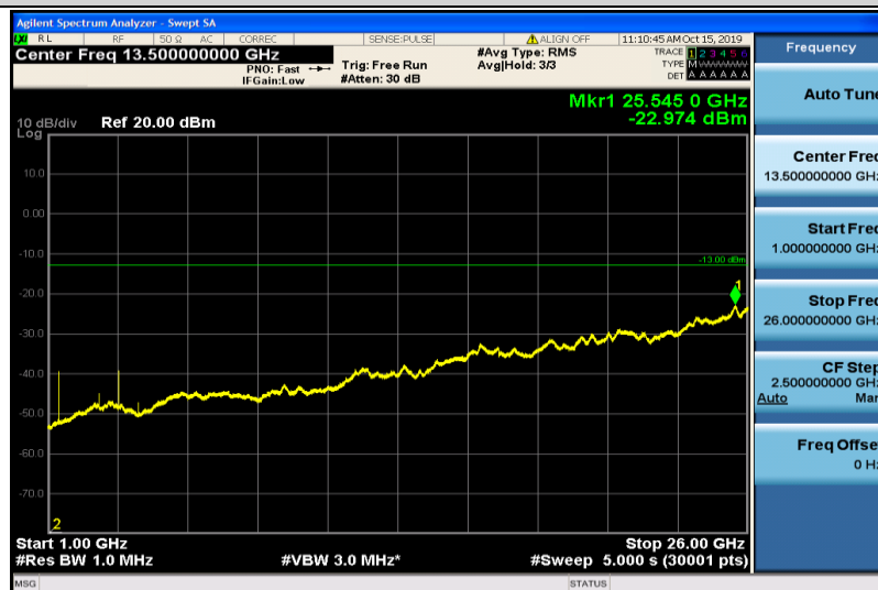
Band17-5MHz-16QAM-23755-1RB#0-1000~26000MHz
