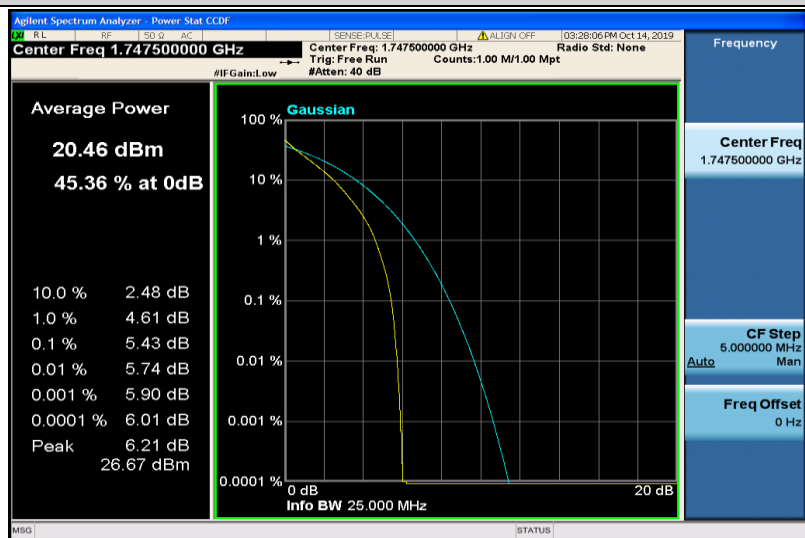
Band4-15MHz-QPSK-20325-75RB#0
