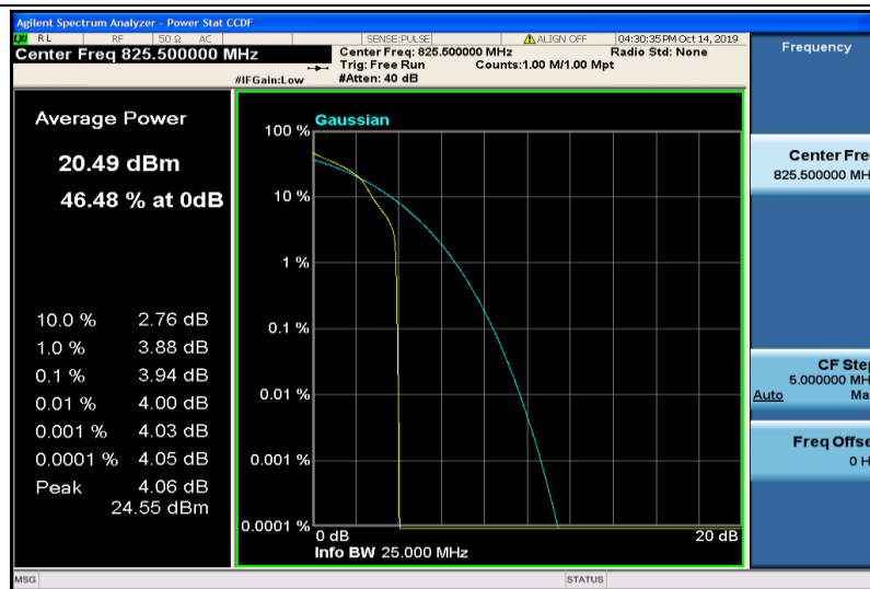
Band5-3MHz-16QAM-20415-1RB#0
