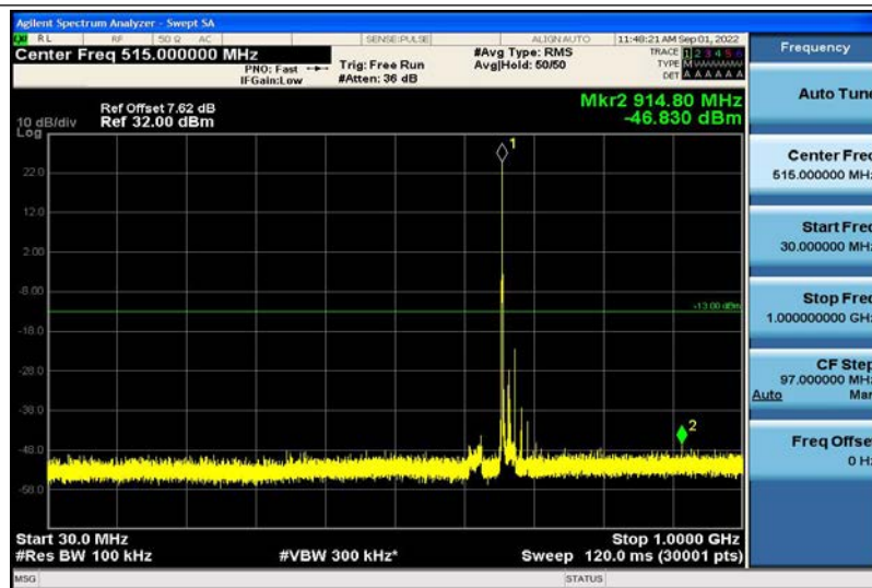
Band71-20MHz-16QAM-133222-1RB#0-30~1000MHz
