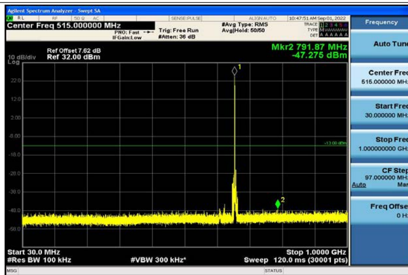
Band71-5MHz-16QAM-133147-1RB#0-30~1000MHz
