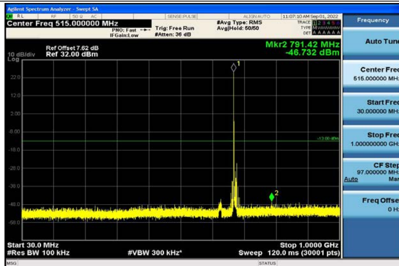
Band71-10MHz-16QAM-133297-1RB#0-30~1000MHz
