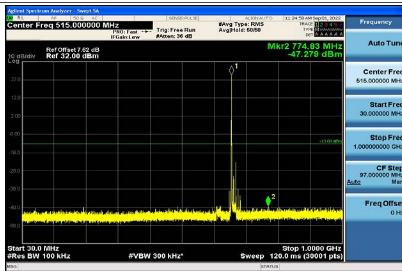
Band71-15MHz-QPSK-133197-1RB#0-30~1000MHz
