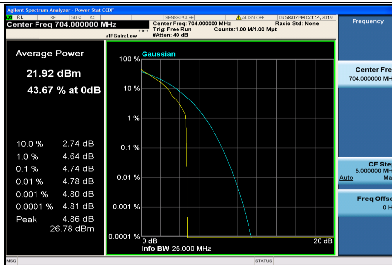
Band12-10MHz-QPSK-23060-1RB#0
