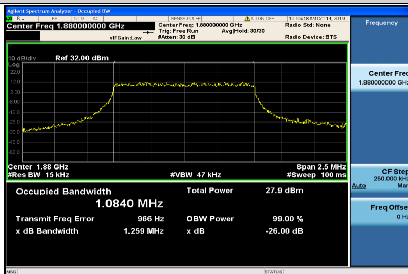
Band2-1.4MHz-QPSK-18900-6RB#0-1.0840
