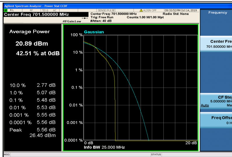
Band12-5MHz-16QAM-23035-1RB#0
