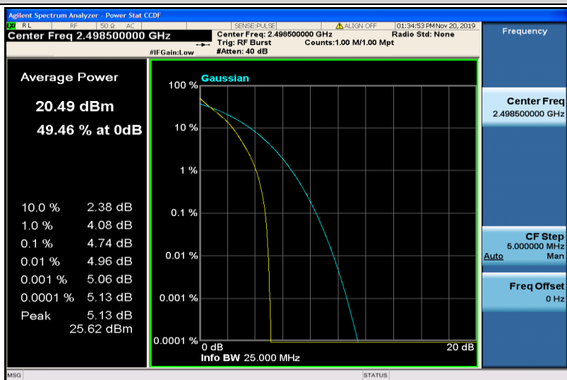
Band41-5MHz-QPSK-39675-25RB#0
