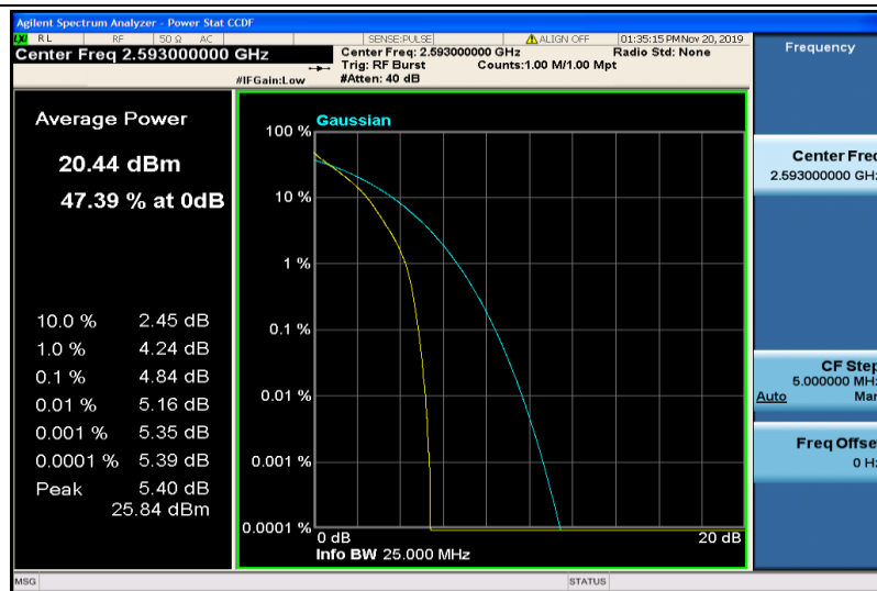
Band41-5MHz-QPSK-40620-25RB#0
