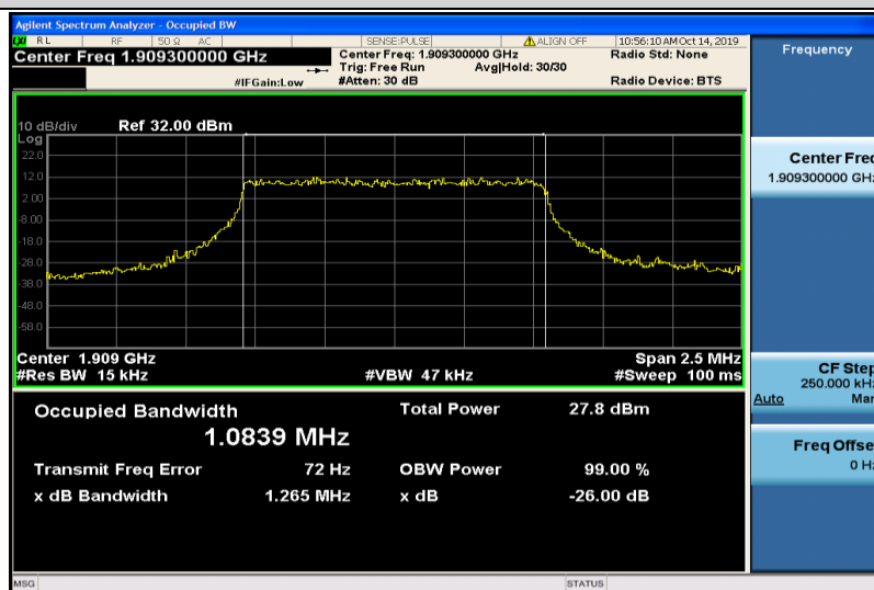
Band2-1.4MHz-QPSK-19193-6RB#0-1.0839
