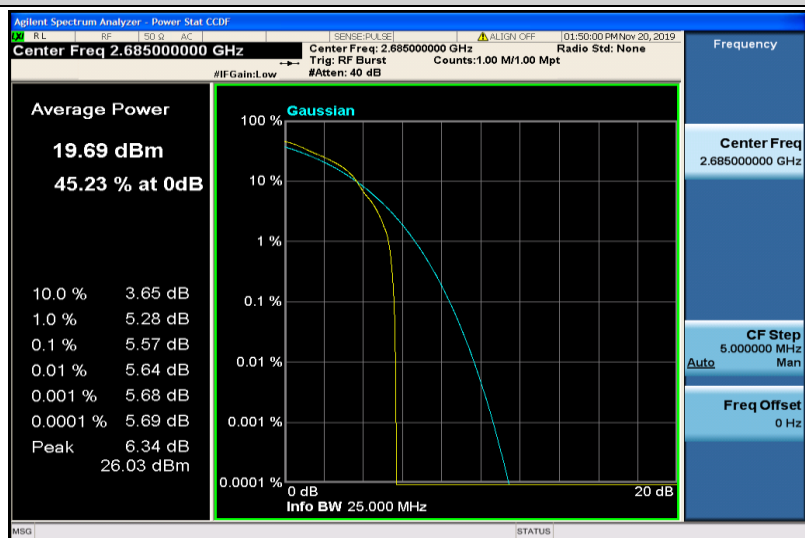
Band41-10MHz-16QAM-41540-1RB#0
