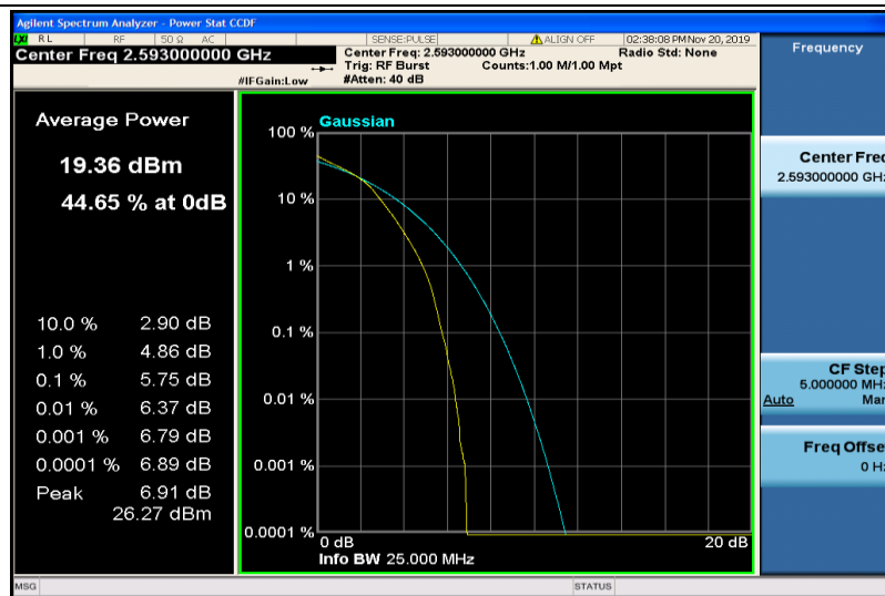
Band41-20MHz-16QAM-40620-100RB#0
