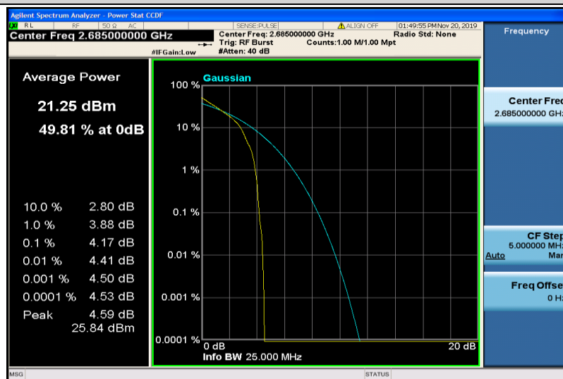
Band41-10MHz-QPSK-41540-1RB#0
