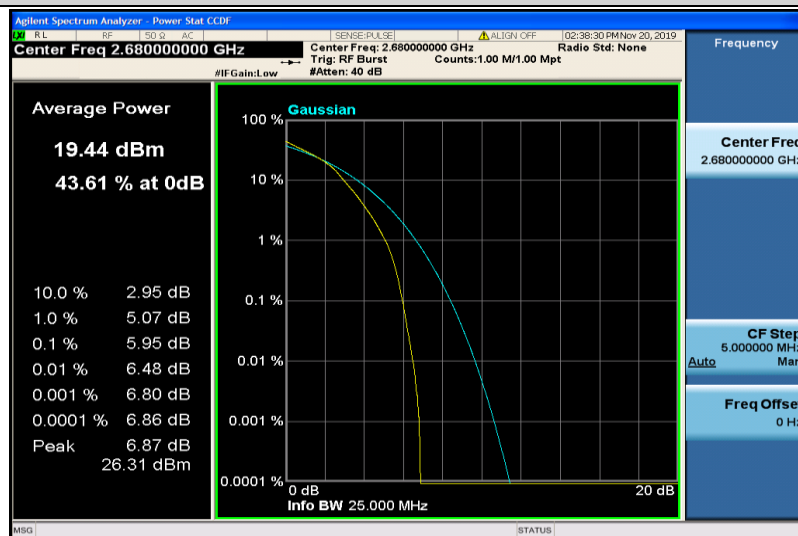
Band41-20MHz-16QAM-41490-100RB#0
