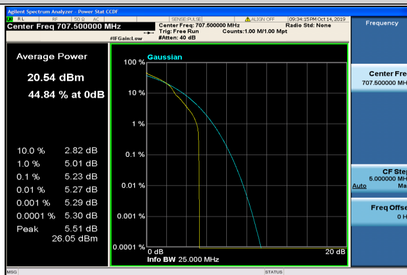
Band12-5MHz-16QAM-23095-1RB#0
