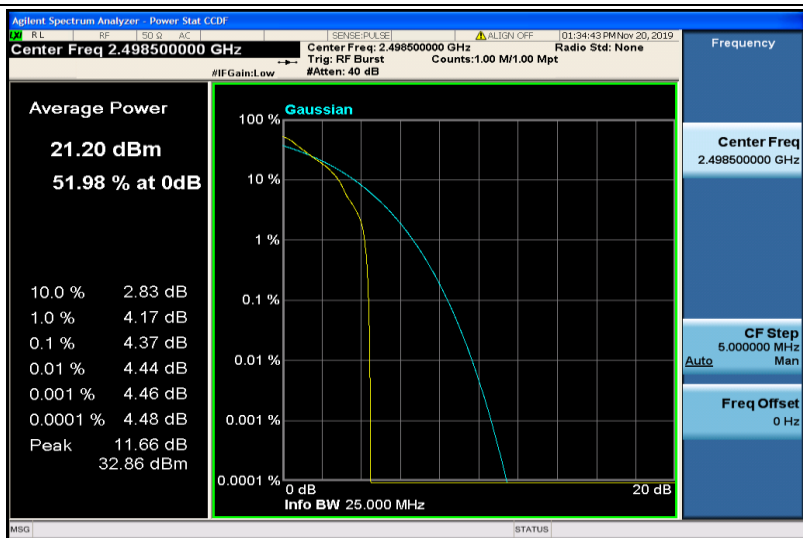
Band41-5MHz-QPSK-39675-1RB#0
