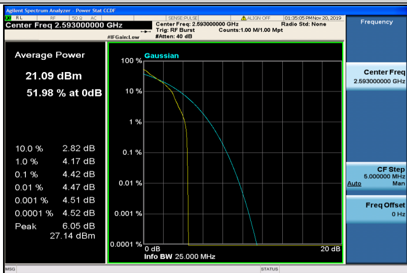
Band41-5MHz-QPSK-40620-1RB#0
