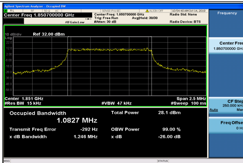
Band2-1.4MHz-QPSK-18607-6RB#0-1.0827
