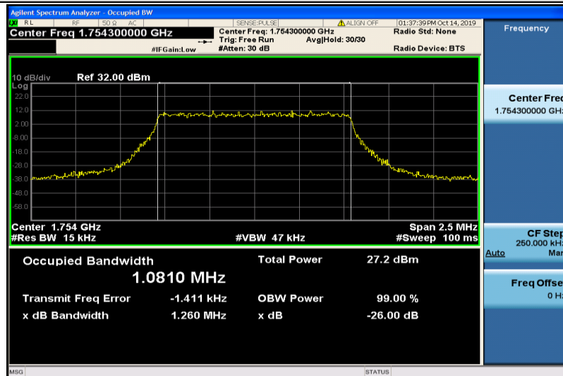
Band4-1.4MHz-16QAM-20393-6RB#0-1.0810
