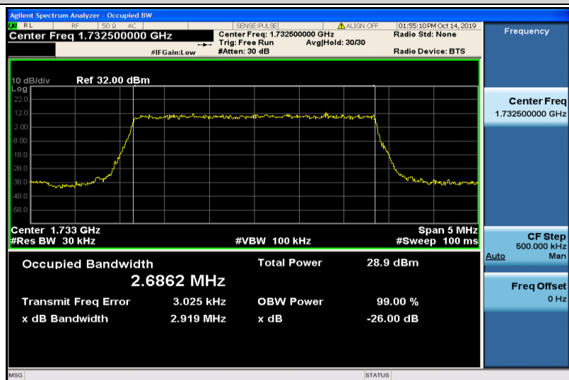
Band4-3MHz-QPSK-20175-15RB#0-2.6862
