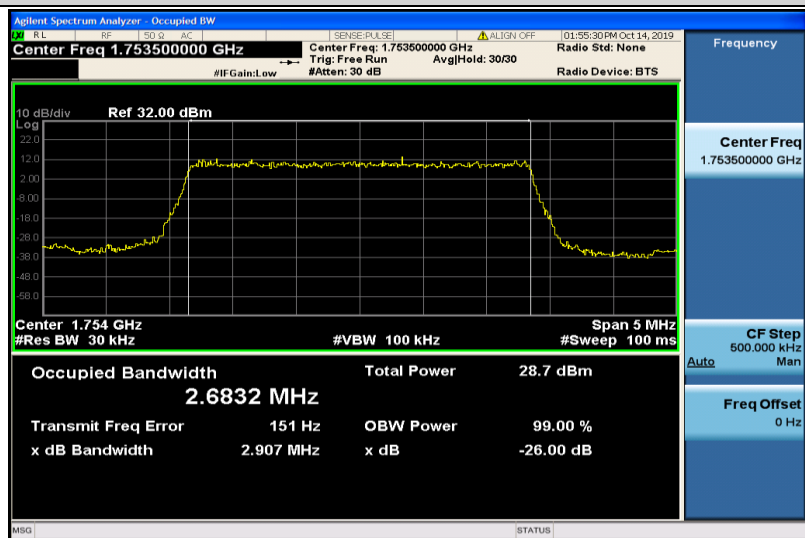
Band4-3MHz-QPSK-20385-15RB#0-2.6832
