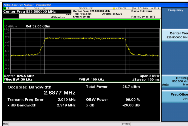
Band5-3MHz-QPSK-20415-15RB#0-2.6877
