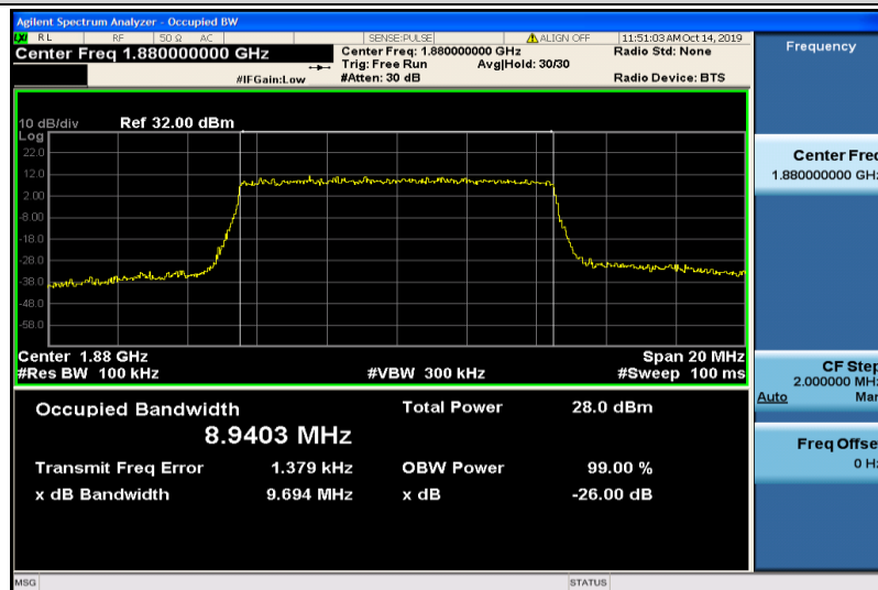
Band2-10MHz-16QAM-18900-50RB#0-8.9403
