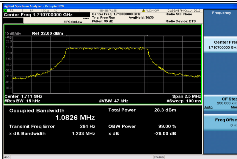
Band4-1.4MHz-QPSK-19957-6RB#0-1.0826
