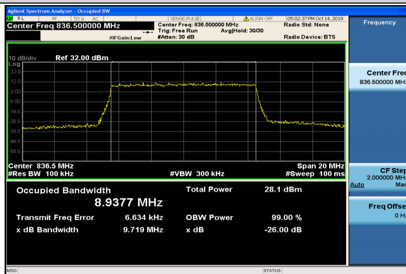
Band5-10MHz-16QAM-20525-50RB#0-8.9377
