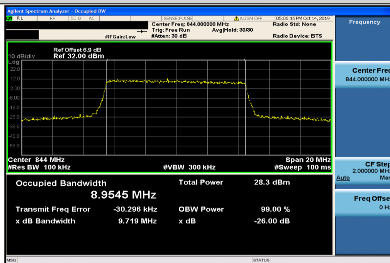
Band5-10MHz-16QAM-20600-50RB#0-8.9545
