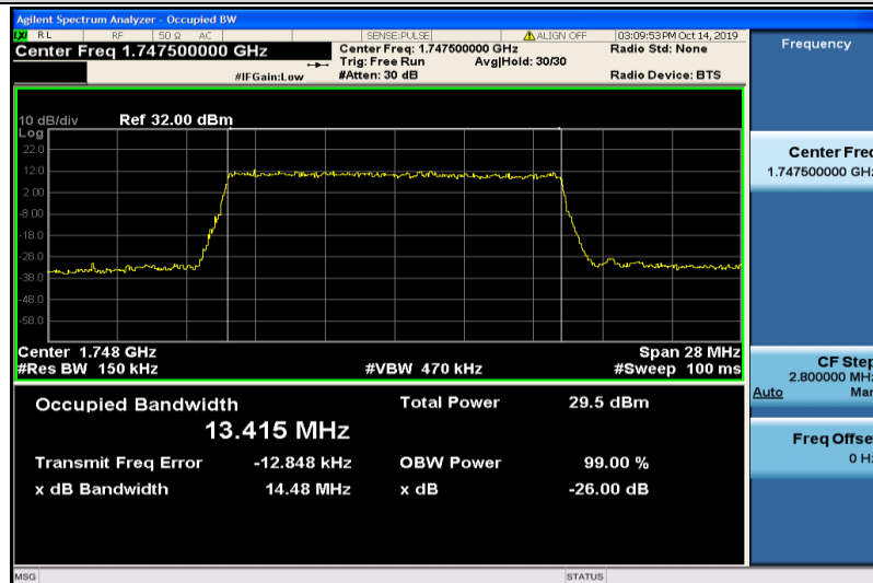
Band4-15MHz-QPSK-20325-75RB#0-13.415
