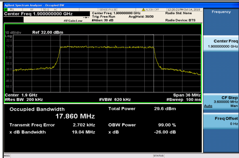
Band2-20MHz-QPSK-19100-100RB#0-17.860
