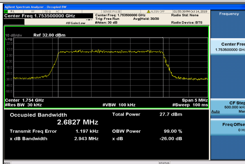
Band4-3MHz-16QAM-20385-15RB#0-2.6827
