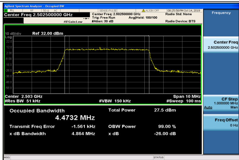
Band7-5MHz-16QAM-20775-25RB#0-4.4732
