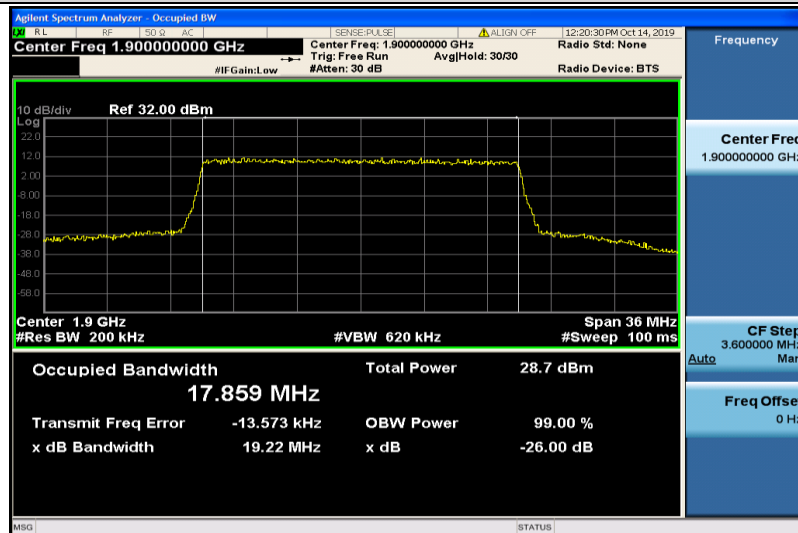
Band2-20MHz-16QAM-19100-100RB#0-17.859
