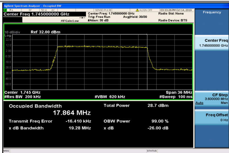
Band4-20MHz-16QAM-20300-100RB#0-17.864
