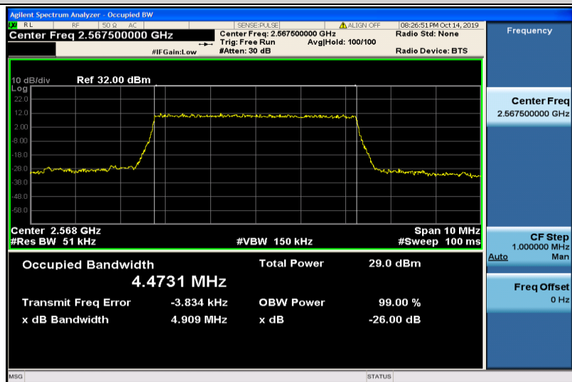
Band7-5MHz-QPSK-21425-25RB#0-4.4731
