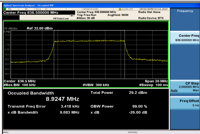
Band5-10MHz-QPSK-20525-50RB#0-8.9247
