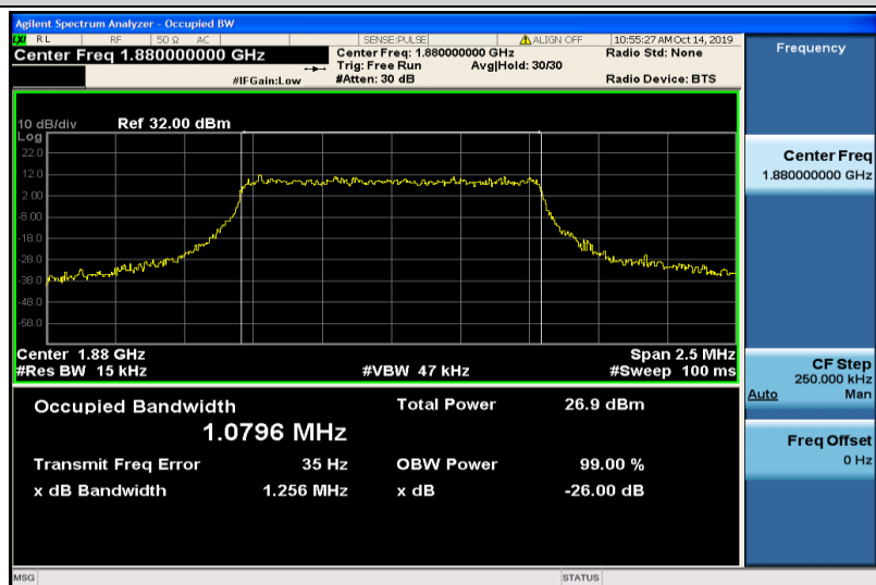
Band2-1.4MHz-16QAM-18900-6RB#0-1.0796
