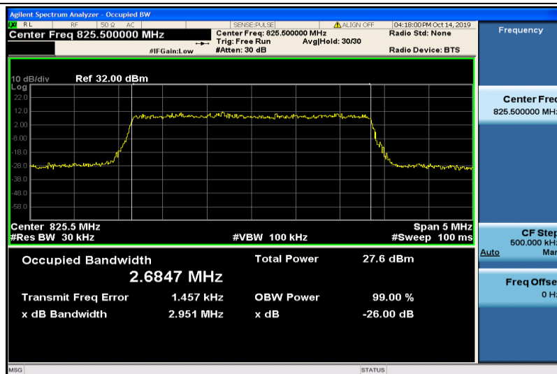
Band5-3MHz-16QAM-20415-15RB#0-2.6847
