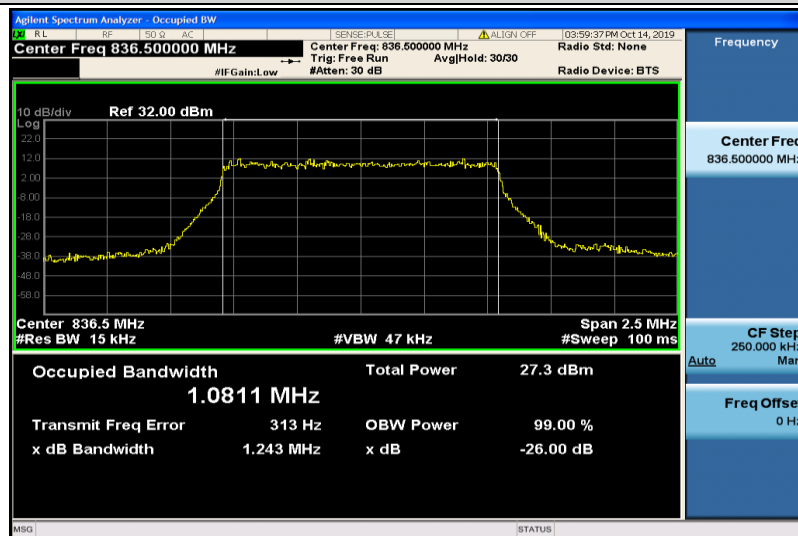
Band5-1.4MHz-16QAM-20525-6RB#0-1.0811
