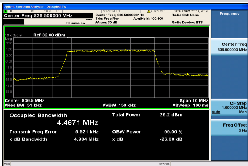
Band5-5MHz-QPSK-20525-25RB#0-4.4671
