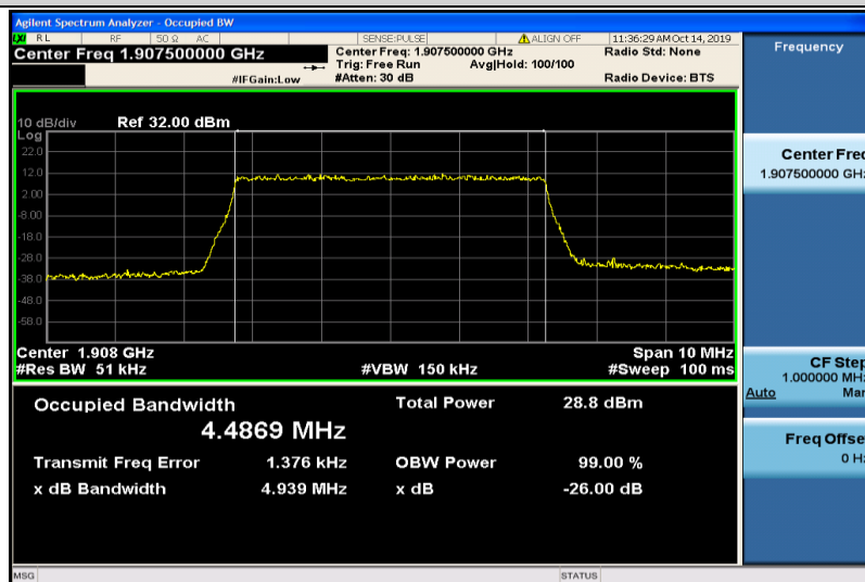
Band2-5MHz-QPSK-19175-25RB#0-4.4869
