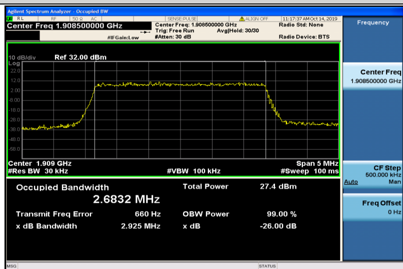
Band2-3MHz-16QAM-19185-15RB#0-2.6832
