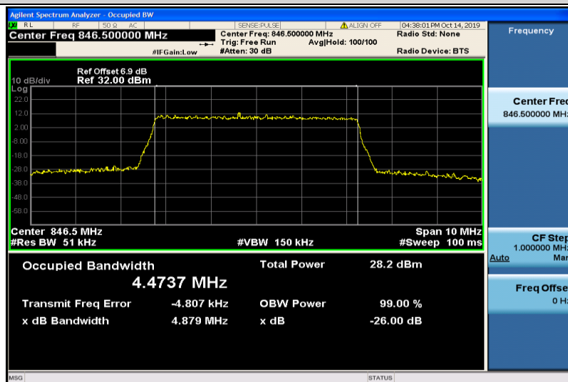
Band5-5MHz-16QAM-20625-25RB#0-4.4737
