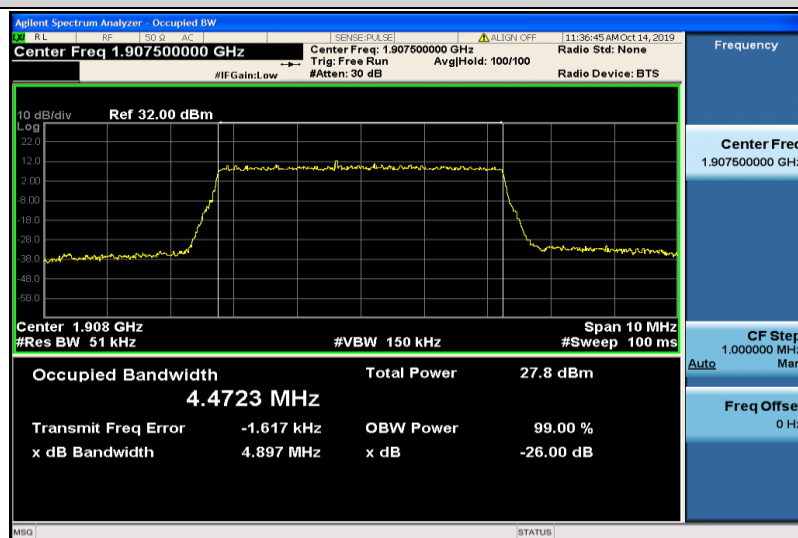
Band2-5MHz-16QAM-19175-25RB#0-4.4723
