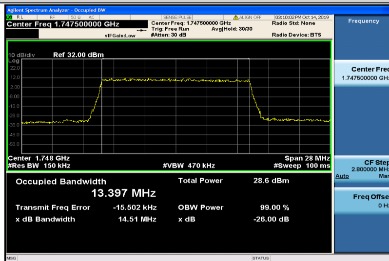
Band4-15MHz-16QAM-20325-75RB#0-13.397
