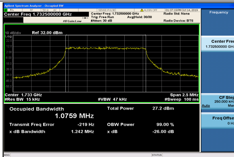
Band4-1.4MHz-16QAM-20175-6RB#0-1.0759
