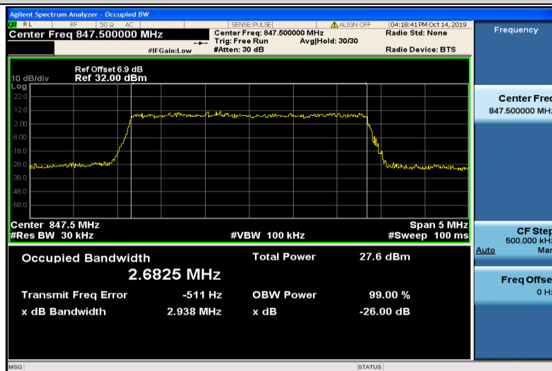
Band5-3MHz-16QAM-20635-15RB#0-2.6825
