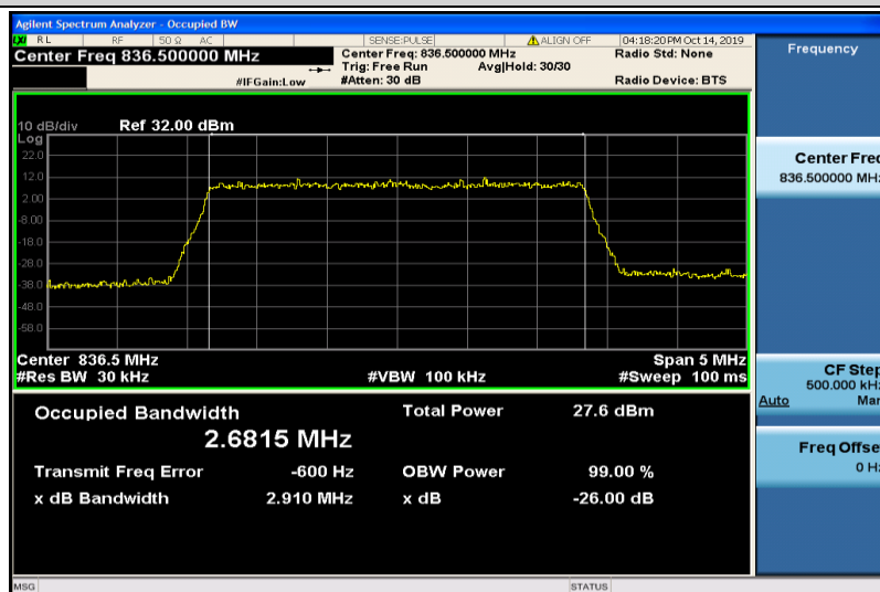
Band5-3MHz-16QAM-20525-15RB#0-2.6815
