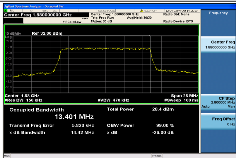
Band2-15MHz-16QAM-18900-75RB#0-13.401
