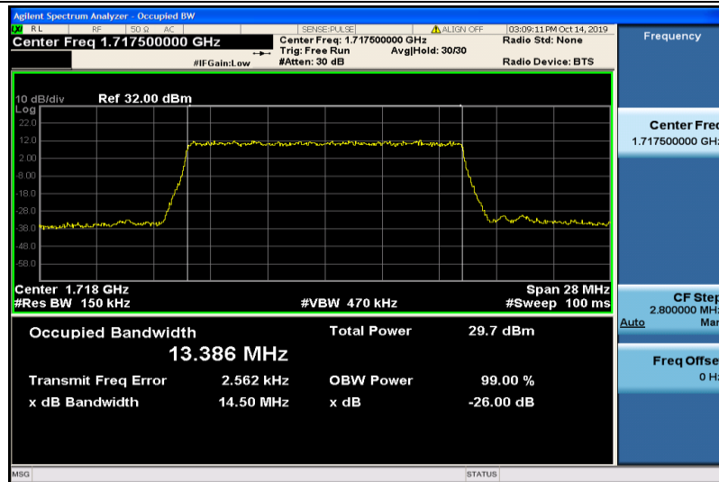
Band4-15MHz-QPSK-20025-75RB#0-13.386
