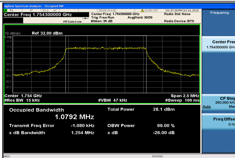
Band4-1.4MHz-QPSK-20393-6RB#0-1.0792
