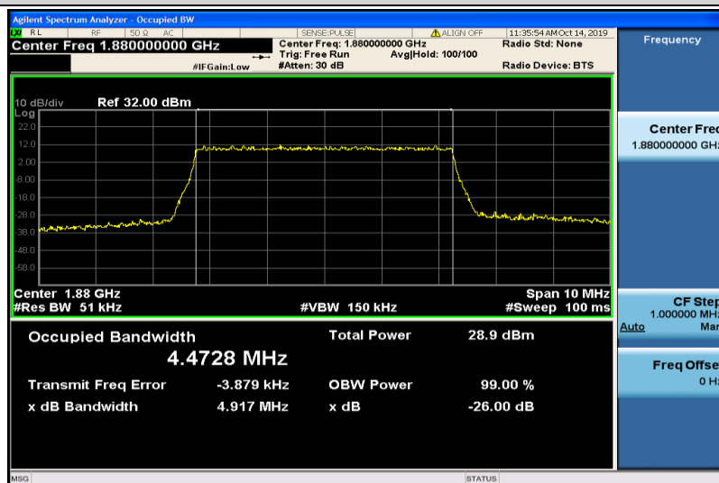
Band2-5MHz-QPSK-18900-25RB#0-4.4728
