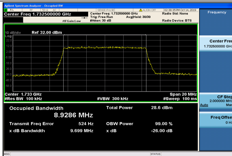
Band4-10MHz-16QAM-20175-50RB#0-8.9286
