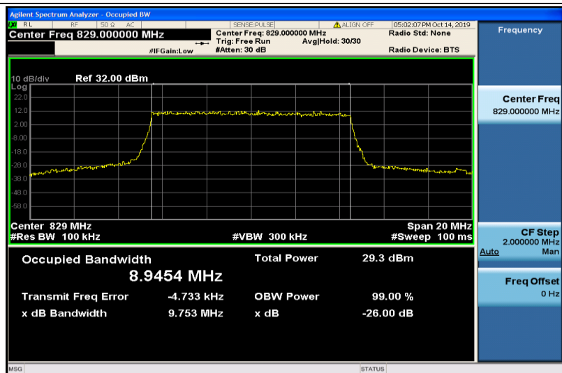
Band5-10MHz-QPSK-20450-50RB#0-8.9454
