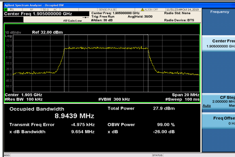
Band2-10MHz-16QAM-19150-50RB#0-8.9439
