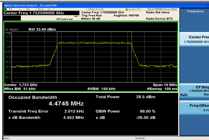
Band4-5MHz-16QAM-20375-25RB#0-4.4745
