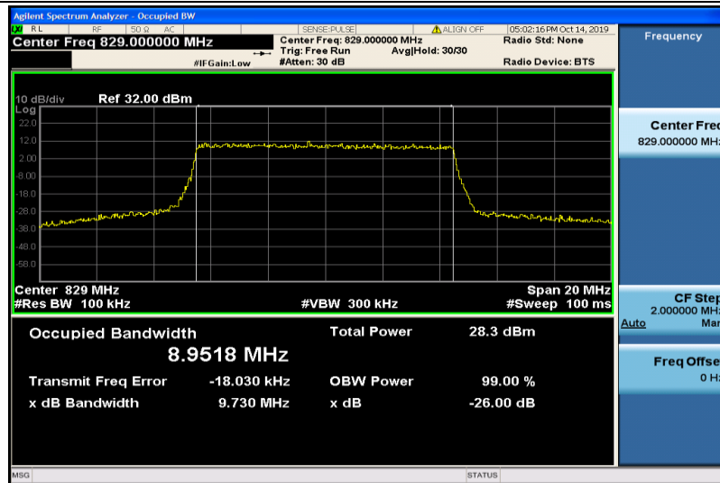
Band5-10MHz-16QAM-20450-50RB#0-8.9518
