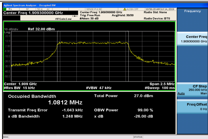
Band2-1.4MHz-16QAM-19193-6RB#0-1.0812
