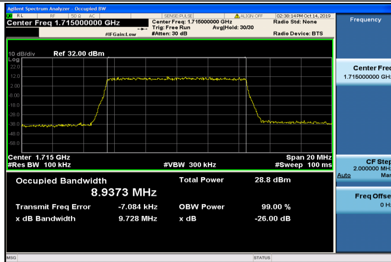
Band4-10MHz-16QAM-20000-50RB#0-8.9373
