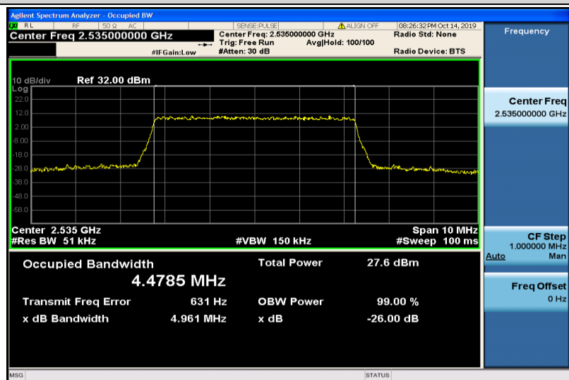
Band7-5MHz-16QAM-21100-25RB#0-4.4785
