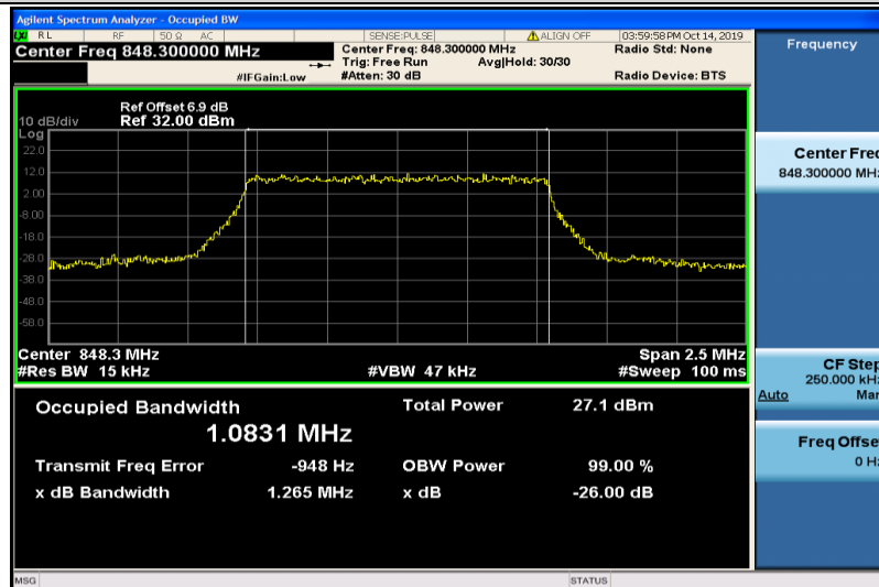
Band5-1.4MHz-16QAM-20643-6RB#0-1.0831
