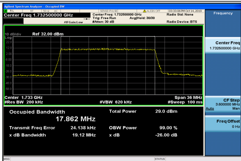
Band4-20MHz-16QAM-20175-100RB#0-17.862
