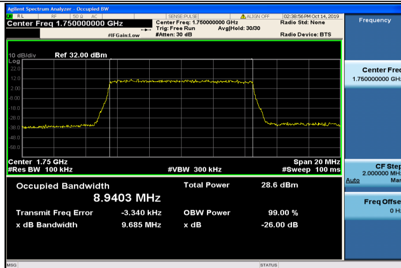
Band4-10MHz-16QAM-20350-50RB#0-8.9403
