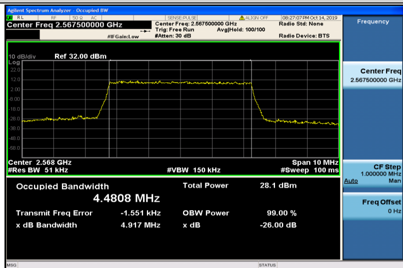
Band7-5MHz-16QAM-21425-25RB#0-4.4808
