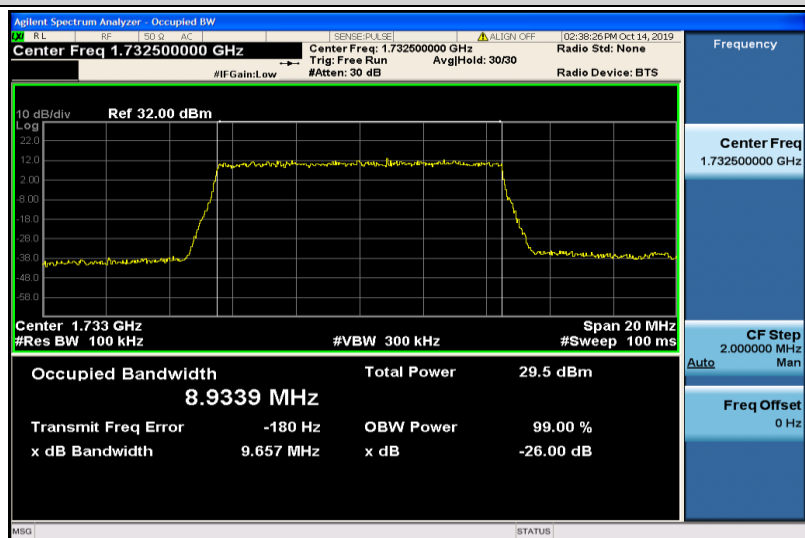
Band4-10MHz-QPSK-20175-50RB#0-8.9339
