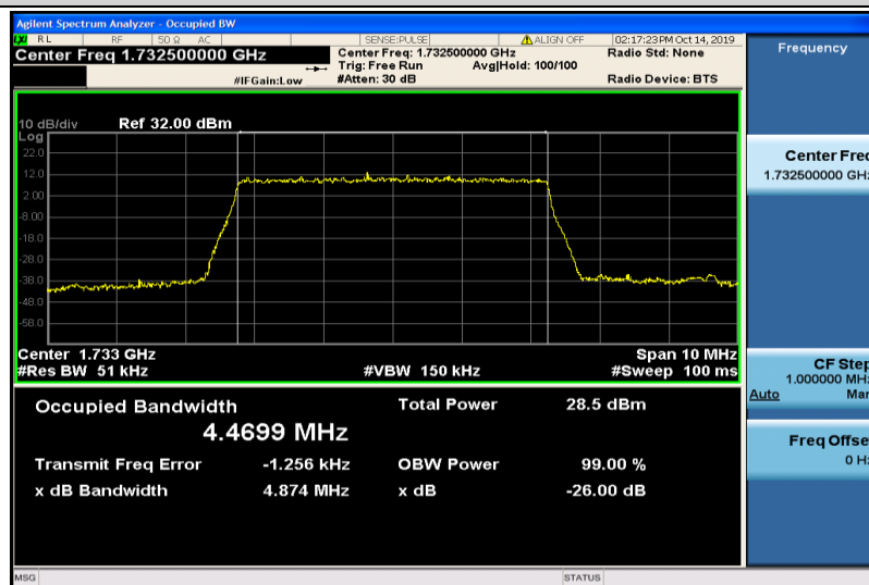
Band4-5MHz-16QAM-20175-25RB#0-4.4699
