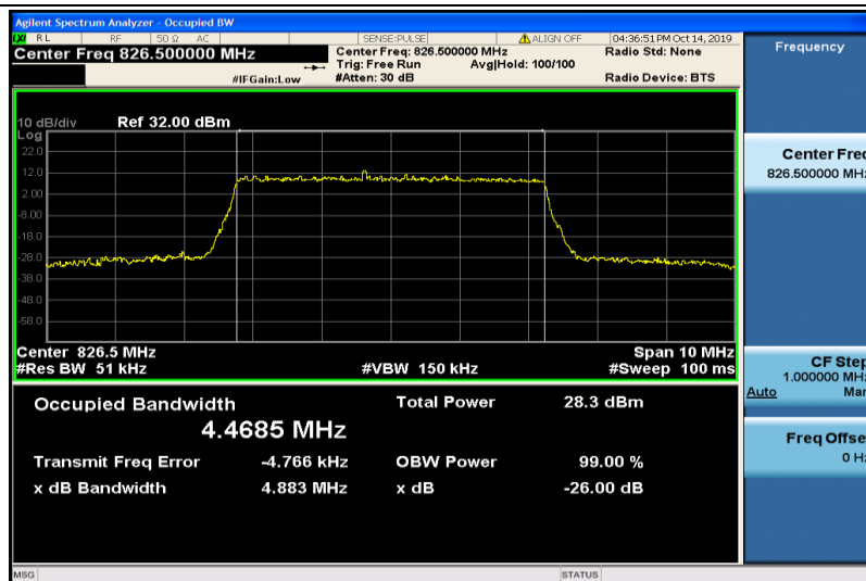
Band5-5MHz-16QAM-20425-25RB#0-4.4685
