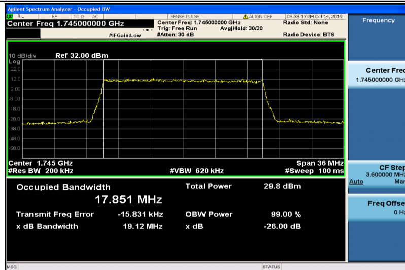
Band4-20MHz-QPSK-20300-100RB#0-17.851
