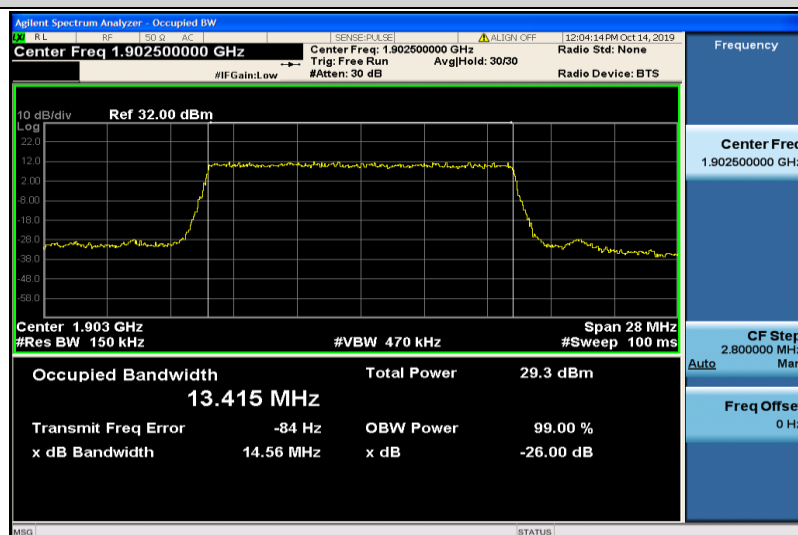
Band2-15MHz-QPSK-19125-75RB#0-13.415
