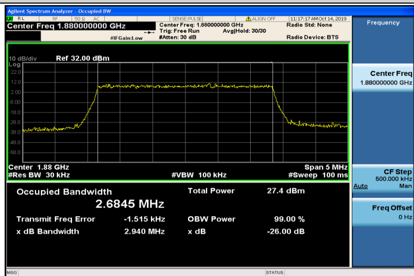
Band2-3MHz-16QAM-18900-15RB#0-2.6845
