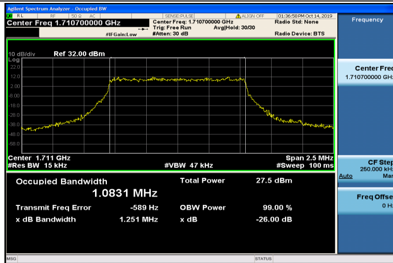
Band4-1.4MHz-16QAM-19957-6RB#0-1.0831
