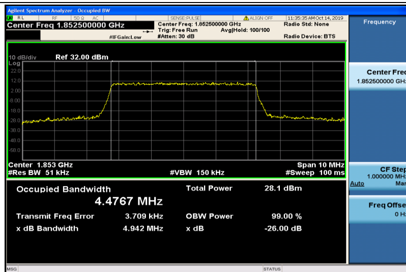
Band2-5MHz-16QAM-18625-25RB#0-4.4767
