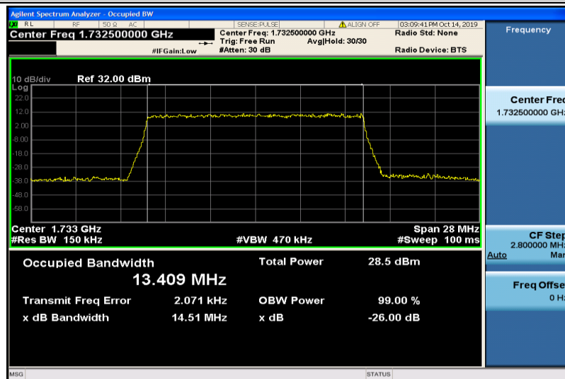
Band4-15MHz-16QAM-20175-75RB#0-13.409
