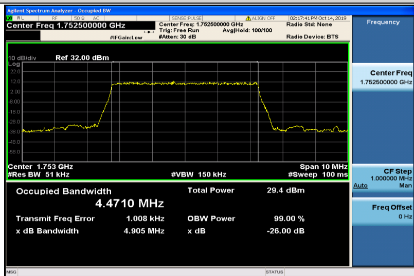
Band4-5MHz-QPSK-20375-25RB#0-4.4710
