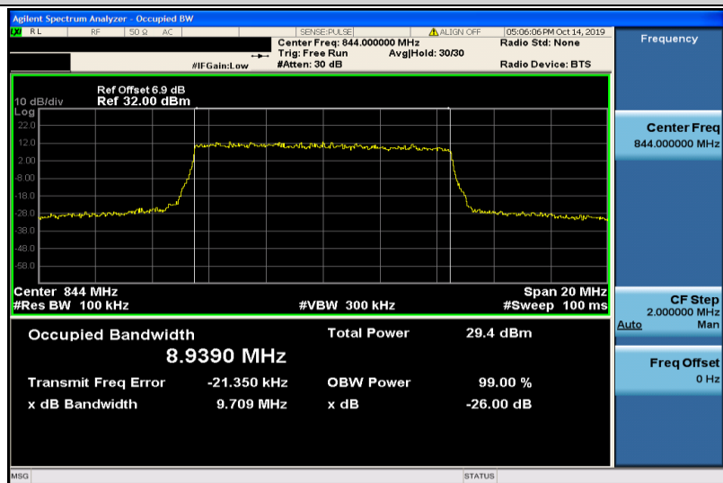
Band5-10MHz-QPSK-20600-50RB#0-8.9390
