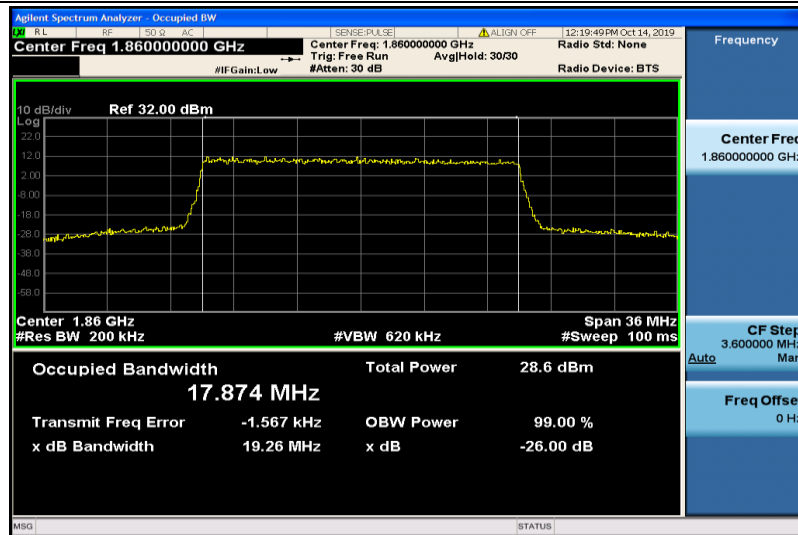
Band2-20MHz-16QAM-18700-100RB#0-17.874
