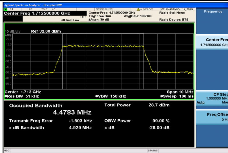
Band4-5MHz-16QAM-19975-25RB#0-4.4783
