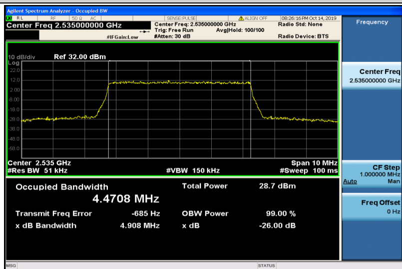
Band7-5MHz-QPSK-21100-25RB#0-4.4708
