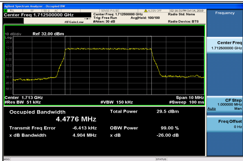
Band4-5MHz-QPSK-19975-25RB#0-4.4776
