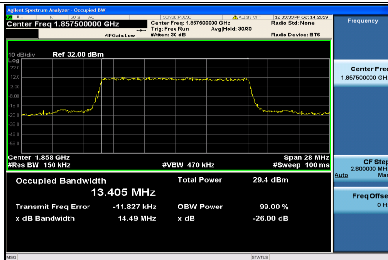
Band2-15MHz-QPSK-18675-75RB#0-13.405
