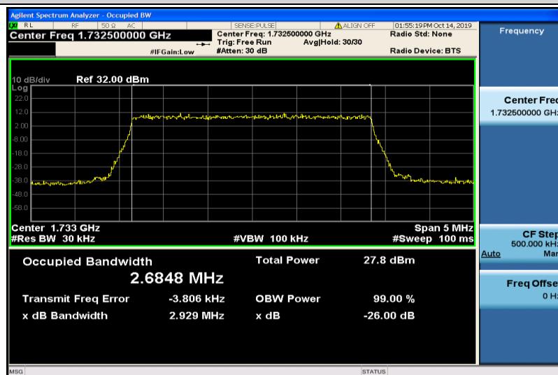
Band4-3MHz-16QAM-20175-15RB#0-2.6848
