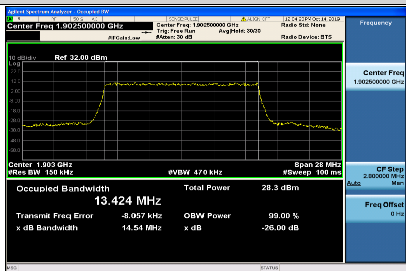
Band2-15MHz-16QAM-19125-75RB#0-13.424
