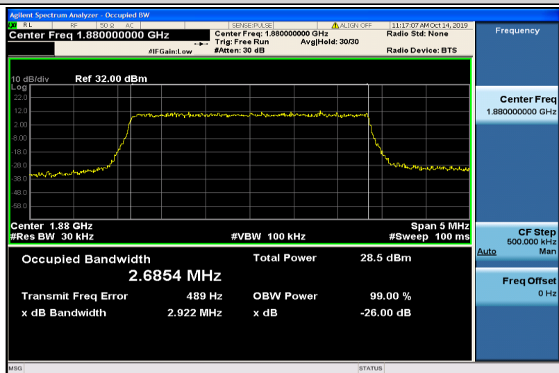
Band2-3MHz-QPSK-18900-15RB#0-2.6854
