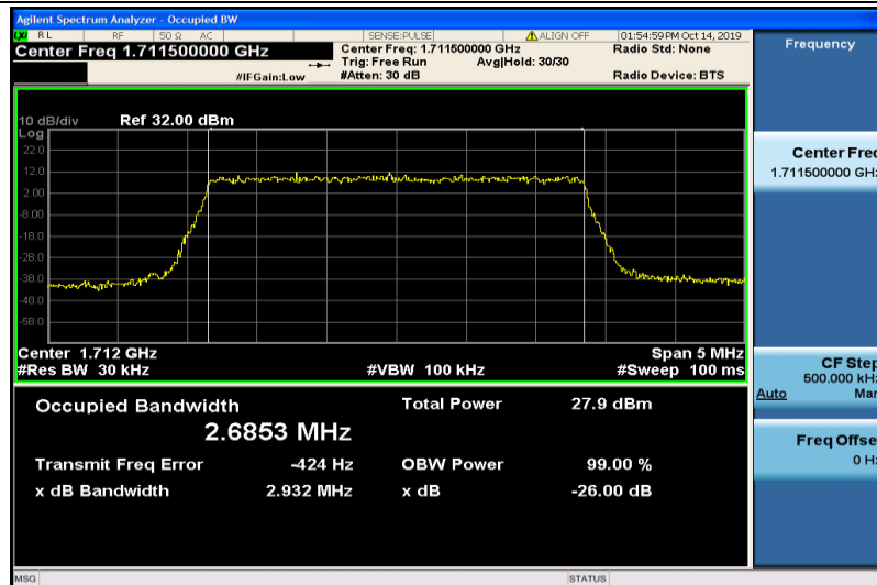
Band4-3MHz-16QAM-19965-15RB#0-2.6853
