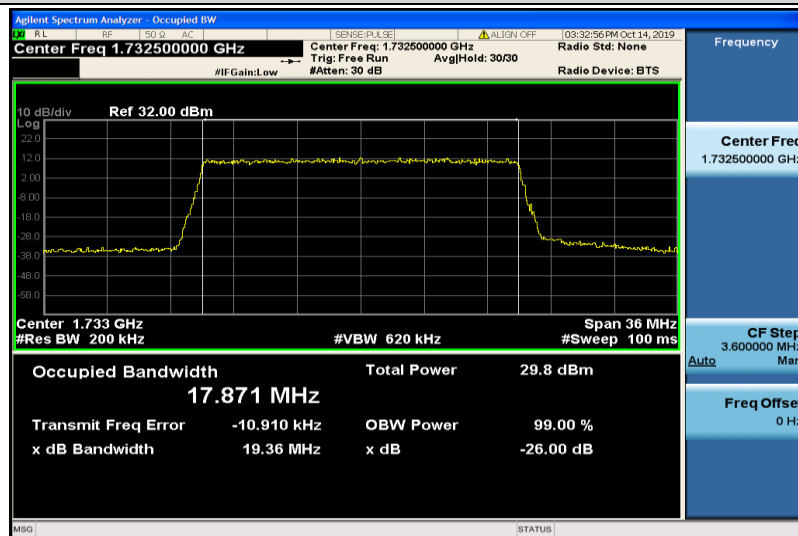
Band4-20MHz-QPSK-20175-100RB#0-17.871
