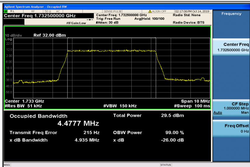
Band4-5MHz-QPSK-20175-25RB#0-4.4777
