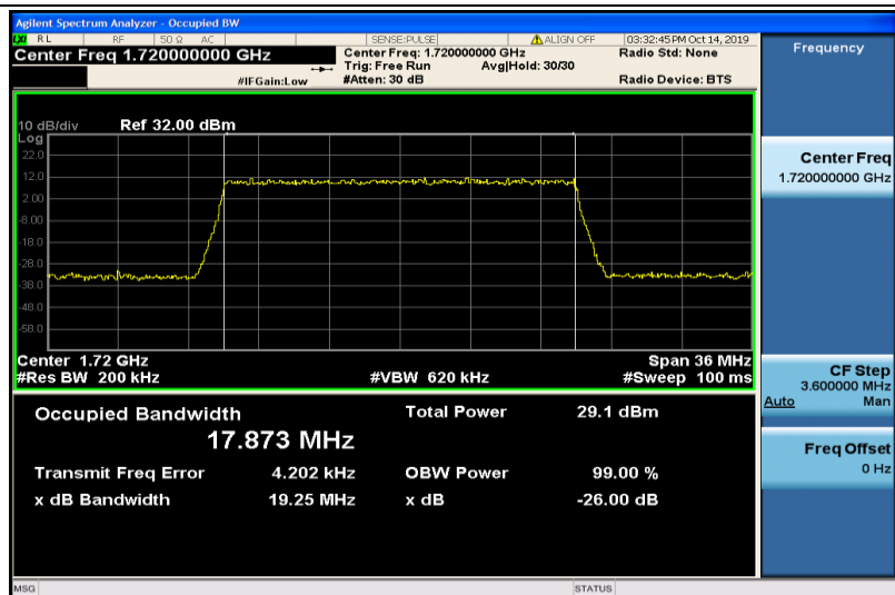
Band4-20MHz-16QAM-20050-100RB#0-17.873
