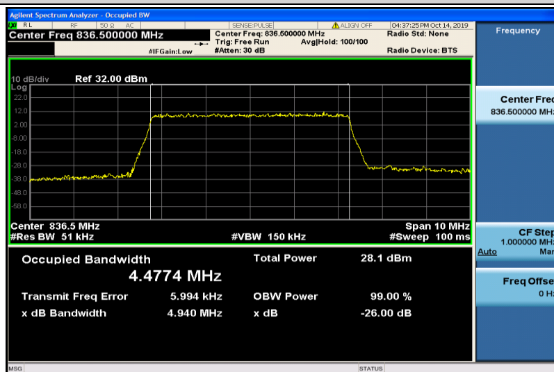
Band5-5MHz-16QAM-20525-25RB#0-4.4774
