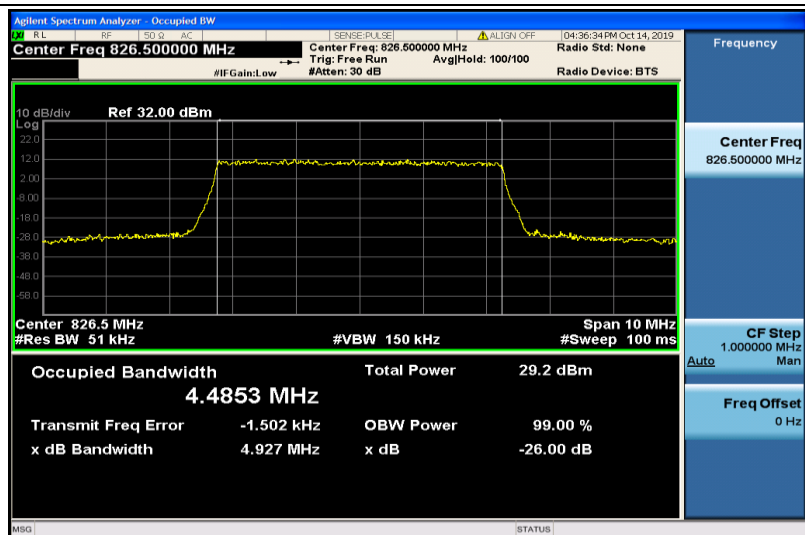
Band5-5MHz-QPSK-20425-25RB#0-4.4853
