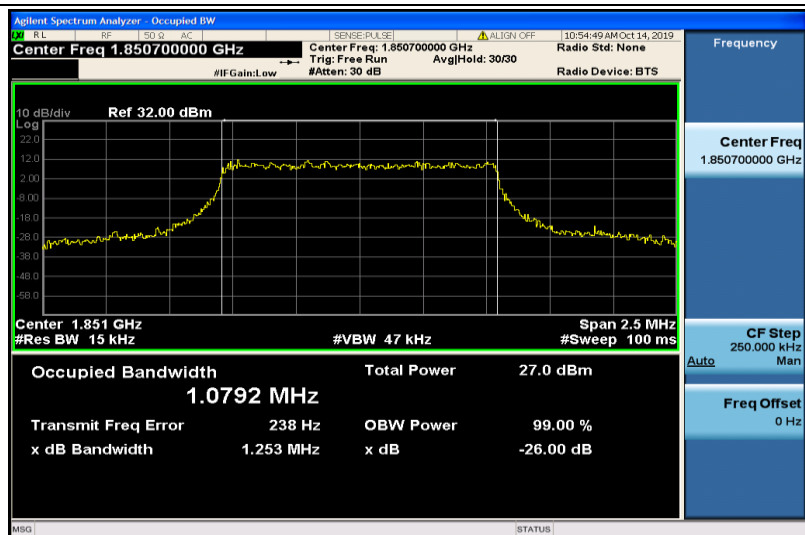
Band2-1.4MHz-16QAM-18607-6RB#0-1.0792
