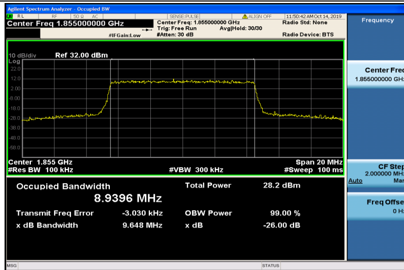
Band2-10MHz-16QAM-18650-50RB#0-8.9396
