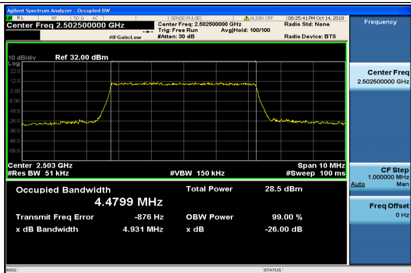
Band7-5MHz-QPSK-20775-25RB#0-4.4799
