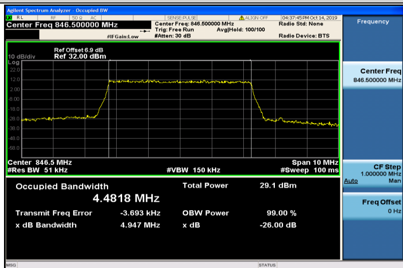
Band5-5MHz-QPSK-20625-25RB#0-4.4818
