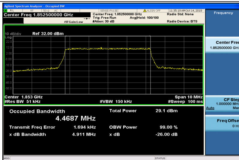
Band2-5MHz-QPSK-18625-25RB#0-4.4687
