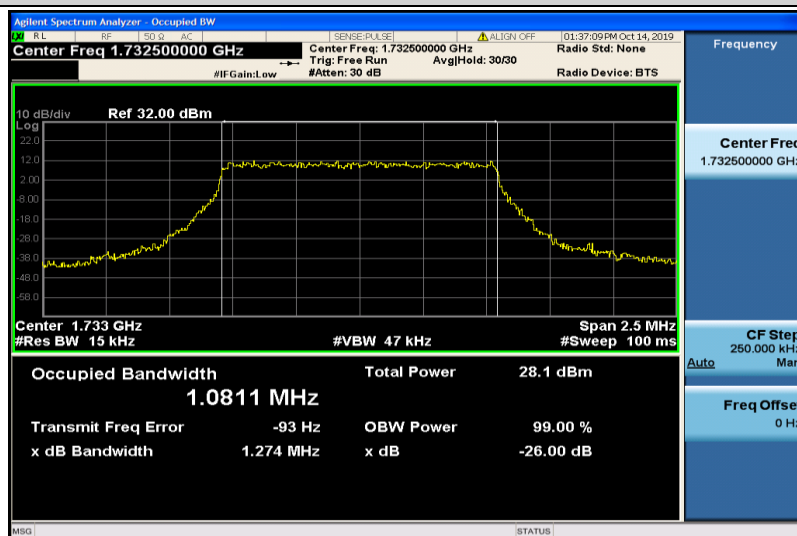
Band4-1.4MHz-QPSK-20175-6RB#0-1.0811
