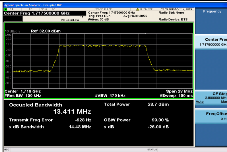
Band4-15MHz-16QAM-20025-75RB#0-13.411
