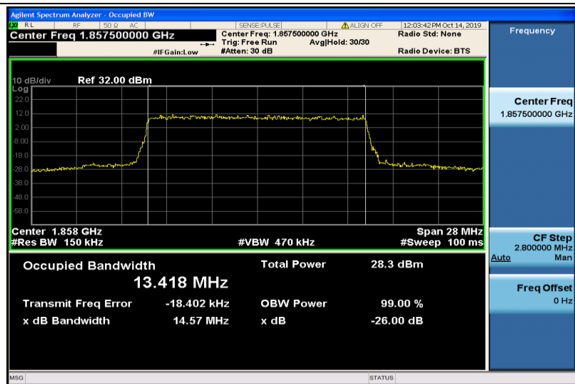
Band2-15MHz-16QAM-18675-75RB#0-13.418
