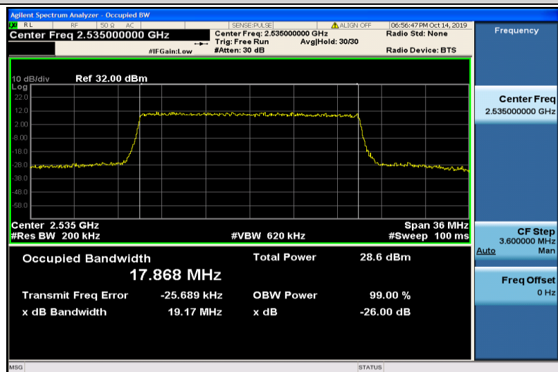
Band7-20MHz-16QAM-21100-100RB#0-17.868
