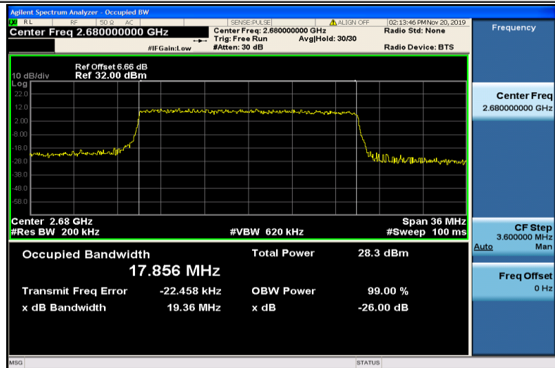
Band41-20MHz-16QAM-41490-100RB#0-17.856
