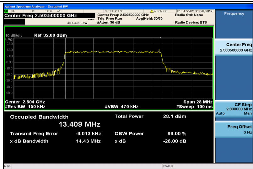
Band41-15MHz-16QAM-39725-75RB#0-13.409
