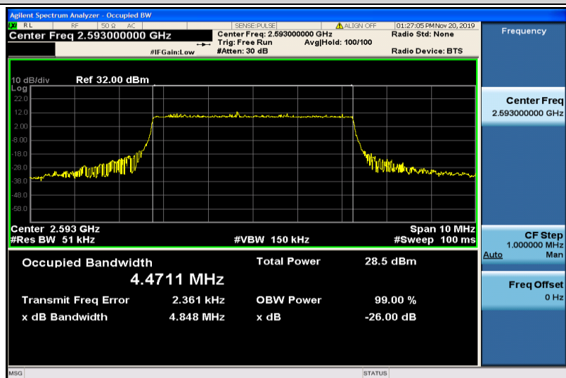
Band41-5MHz-QPSK-40620-25RB#0-4.4711
