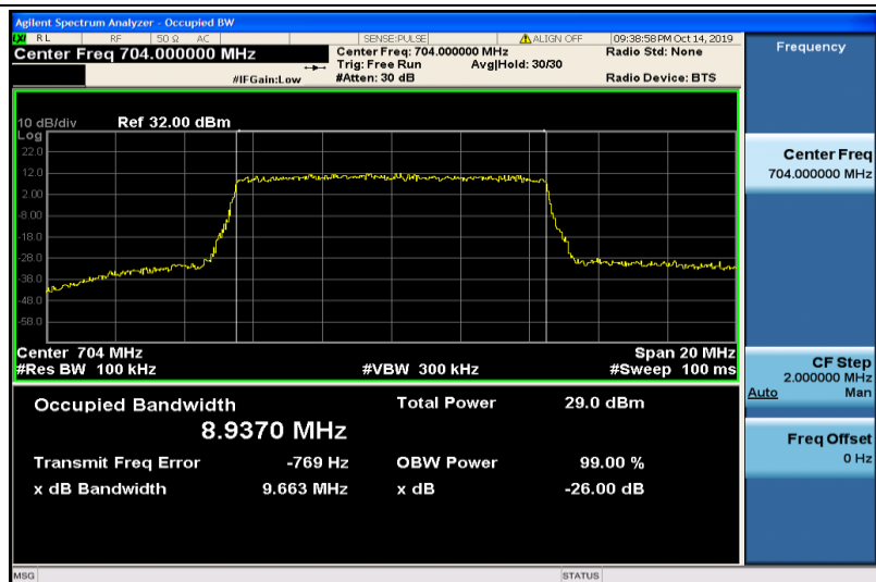
Band12-10MHz-QPSK-23060-50RB#0-8.9370
