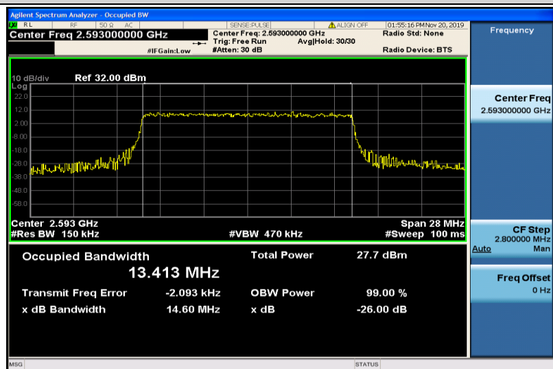
Band41-15MHz-16QAM-40620-75RB#0-13.413
