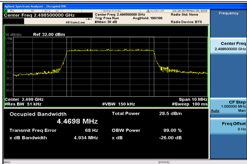
Band41-5MHz-QPSK-39675-25RB#0-4.4698
