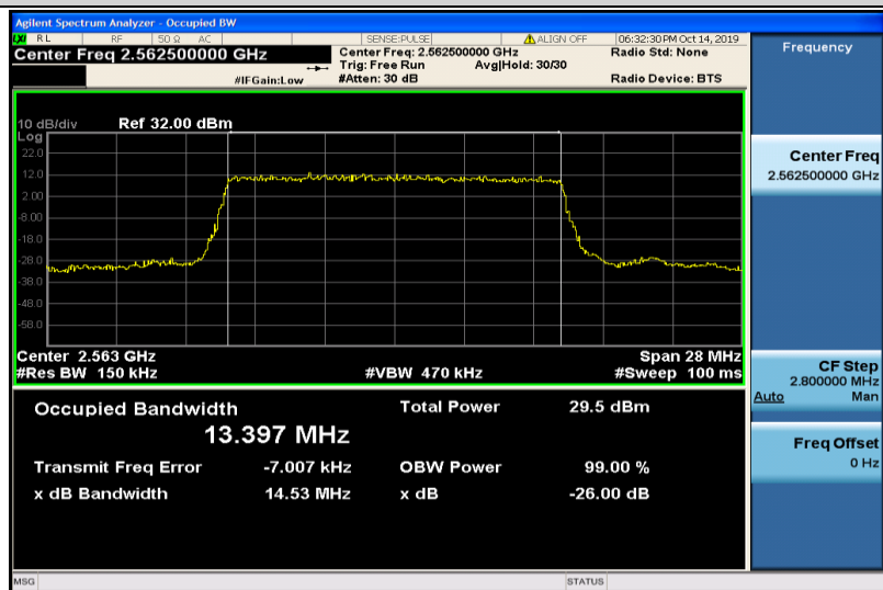
Band7-15MHz-QPSK-21375-75RB#0-13.397
