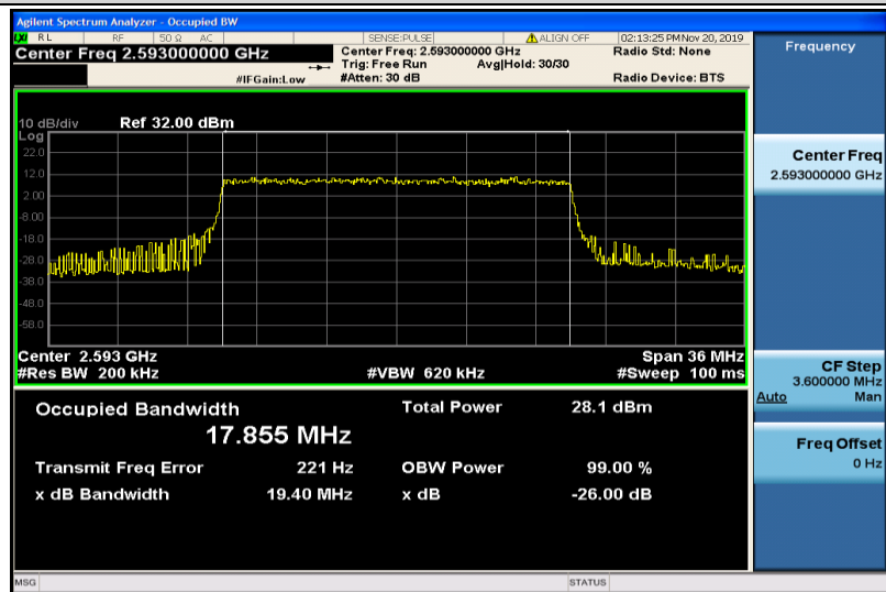
Band41-20MHz-16QAM-40620-100RB#0-17.855
