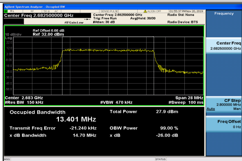
Band41-15MHz-16QAM-41515-75RB#0-13.401
