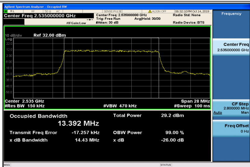
Band7-15MHz-QPSK-21100-75RB#0-13.392
