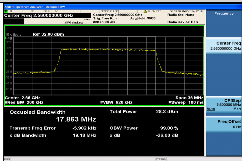
Band7-20MHz-16QAM-21350-100RB#0-17.863
