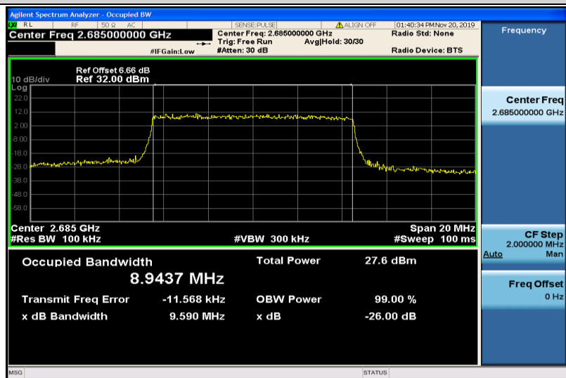
Band41-10MHz-16QAM-41540-50RB#0-8.9437
