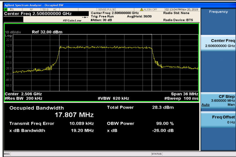
Band41-20MHz-16QAM-39750-100RB#0-17.807
