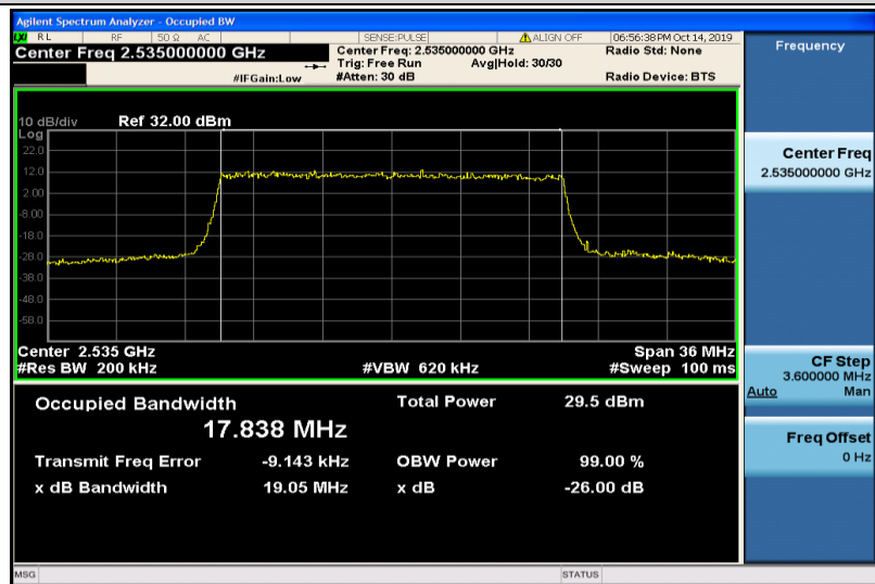
Band7-20MHz-QPSK-21100-100RB#0-17.838
