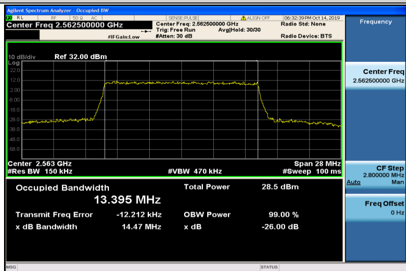
Band7-15MHz-16QAM-21375-75RB#0-13.395
