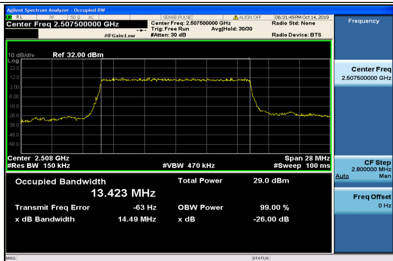
Band7-15MHz-QPSK-20825-75RB#0-13.423
