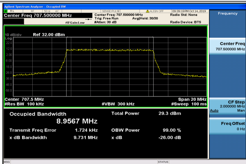
Band12-10MHz-QPSK-23095-50RB#0-8.9567
