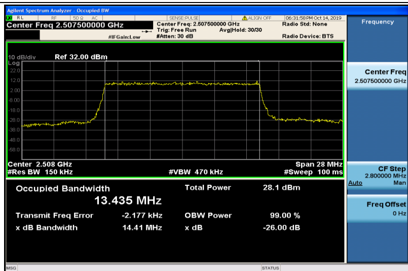
Band7-15MHz-16QAM-20825-75RB#0-13.435
