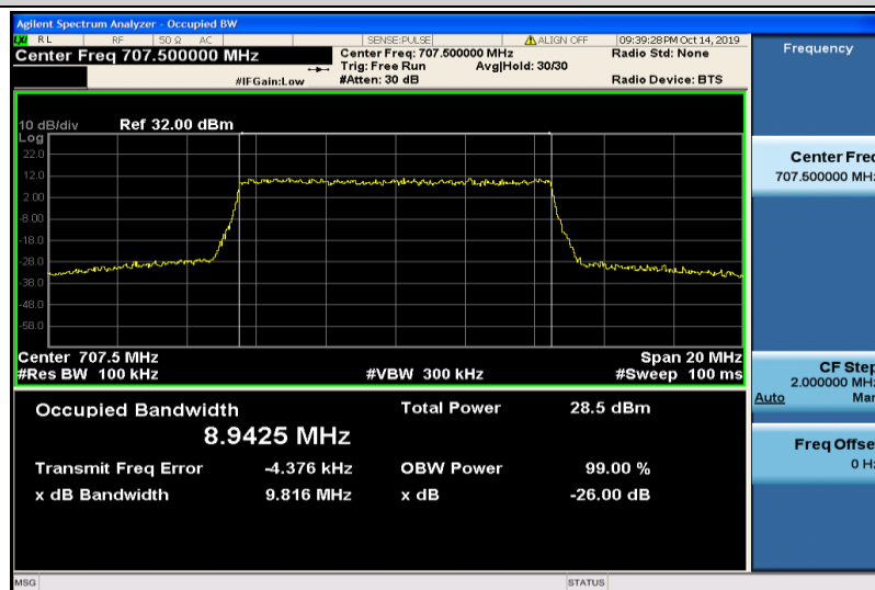
Band12-10MHz-16QAM-23095-50RB#0-8.9425
