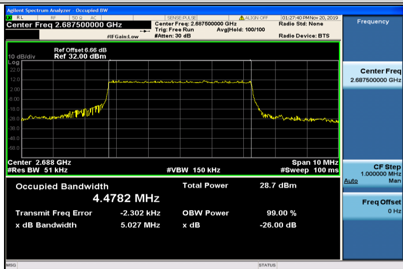
Band41-5MHz-QPSK-41565-25RB#0-4.4782
