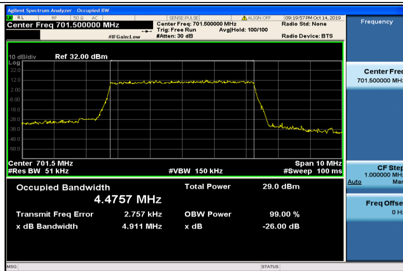
Band12-5MHz-QPSK-23035-25RB#0-4.4757
