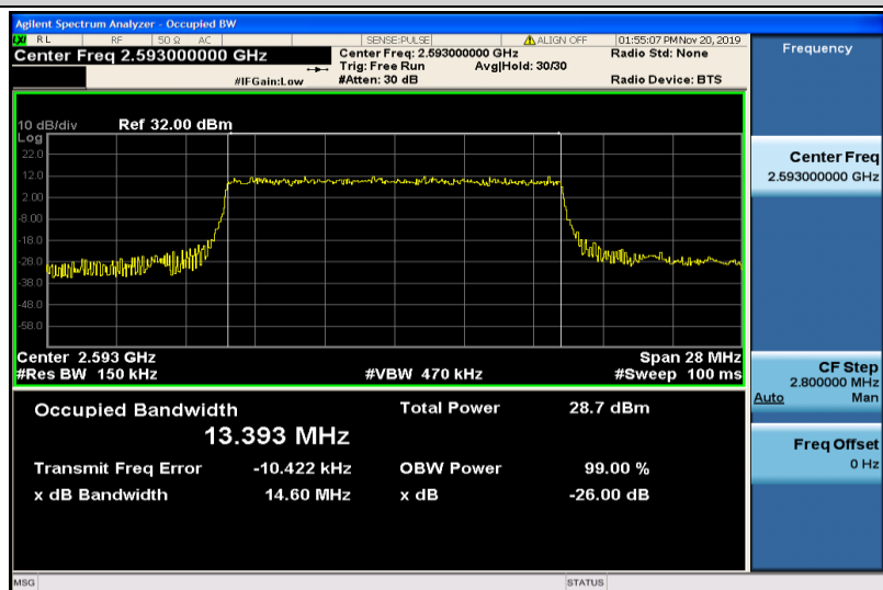
Band41-15MHz-QPSK-40620-75RB#0-13.393
