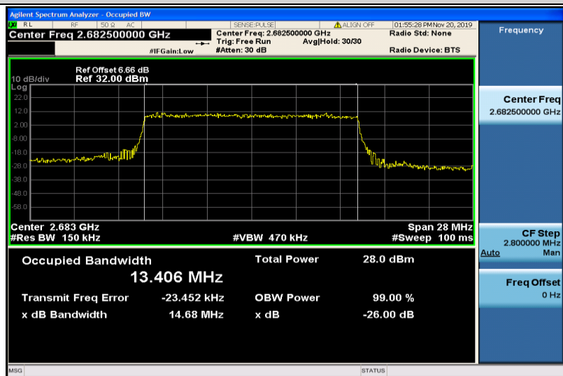
Band41-15MHz-QPSK-41515-75RB#0-13.406
