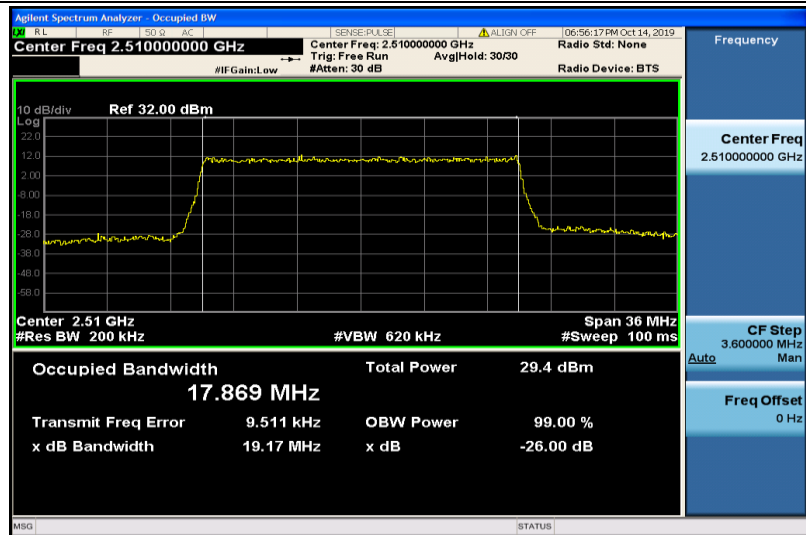
Band7-20MHz-QPSK-20850-100RB#0-17.869
