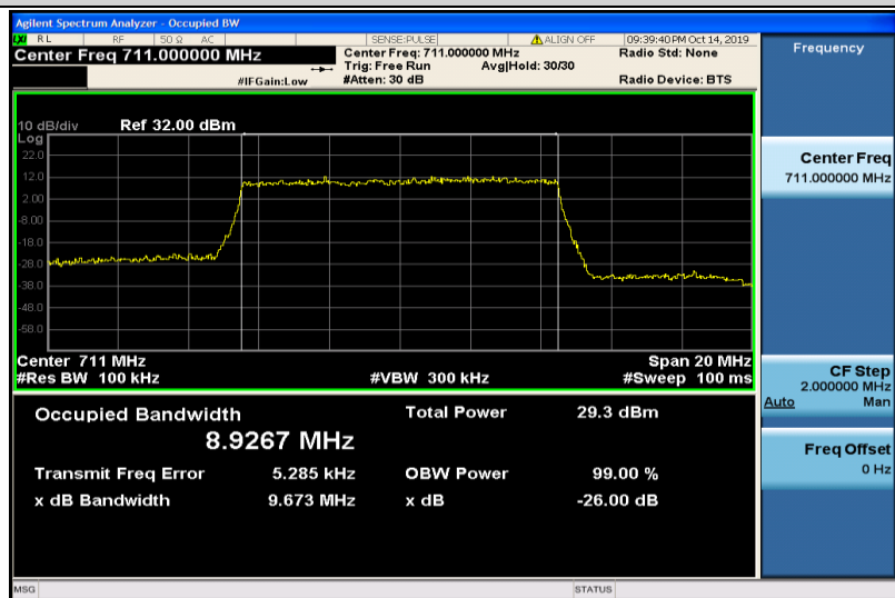
Band12-10MHz-QPSK-23130-50RB#0-8.9267
