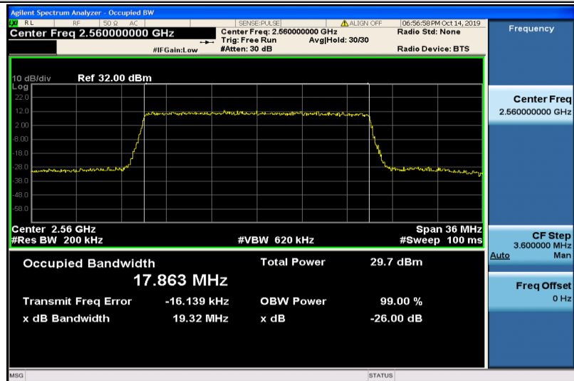
Band7-20MHz-QPSK-21350-100RB#0-17.863
