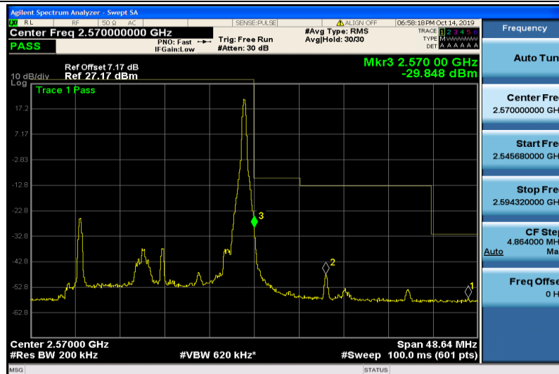
Band7-20MHz-QPSK-21350-1RB#99
