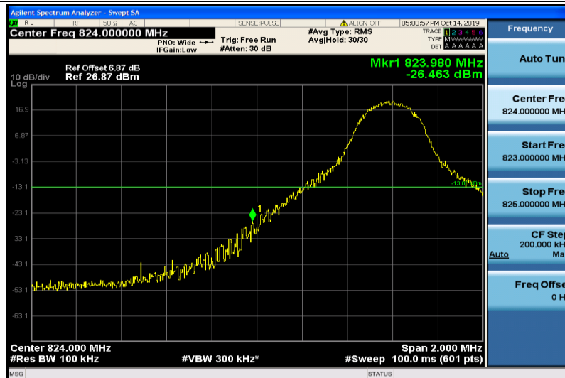
Band5-10MHz-16QAM-20450-1RB#0
