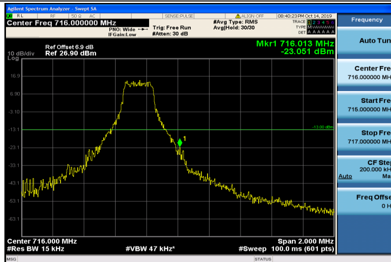
Band12-1.4MHz-16QAM-23173-1RB#5
