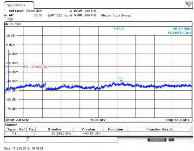
802.11n-20 MHz LOW CHANNEL, SPURIOUS 2 GHz ~ 25 GHz
