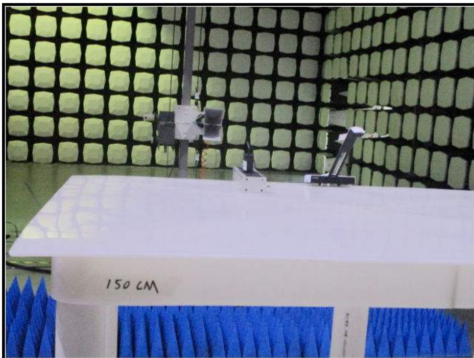
Above 1 GHz
