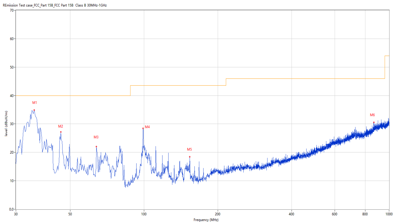
Figure 8: Test plots of Field strength of harmonics, 2403MHz, 30MHz-1GHz, Vertical polarization
