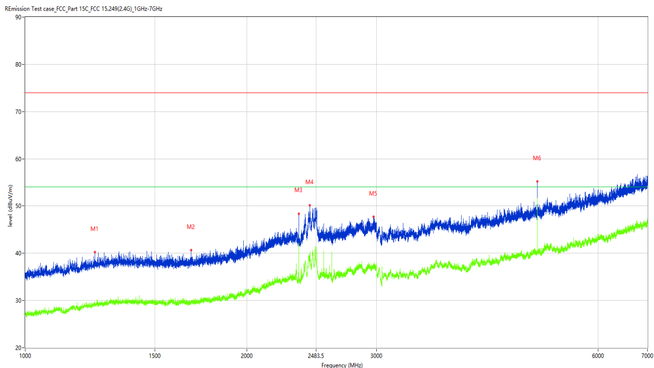
Figure 21: Test plots of Field strength of harmonics, 2480MHz, 1GHz-7GHz, Horizontal polarization
