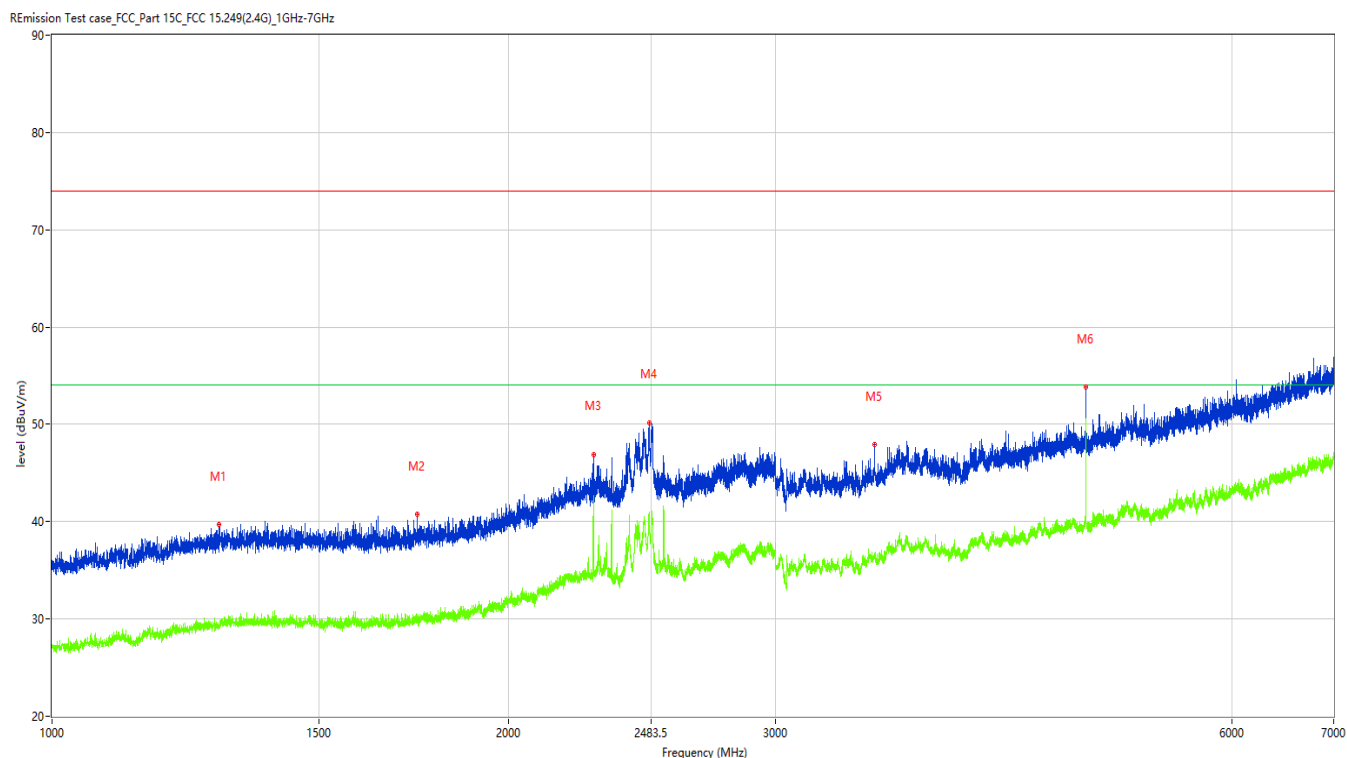
Figure 9: Test plots of Field strength of harmonics, 2403MHz, 1GHz-7GHz, Horizontal polarization
