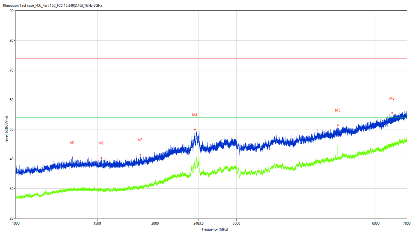
Figure 22: Test plots of Field strength of harmonics, 2480MHz, 1GHz-7GHz, Vertical polarization
