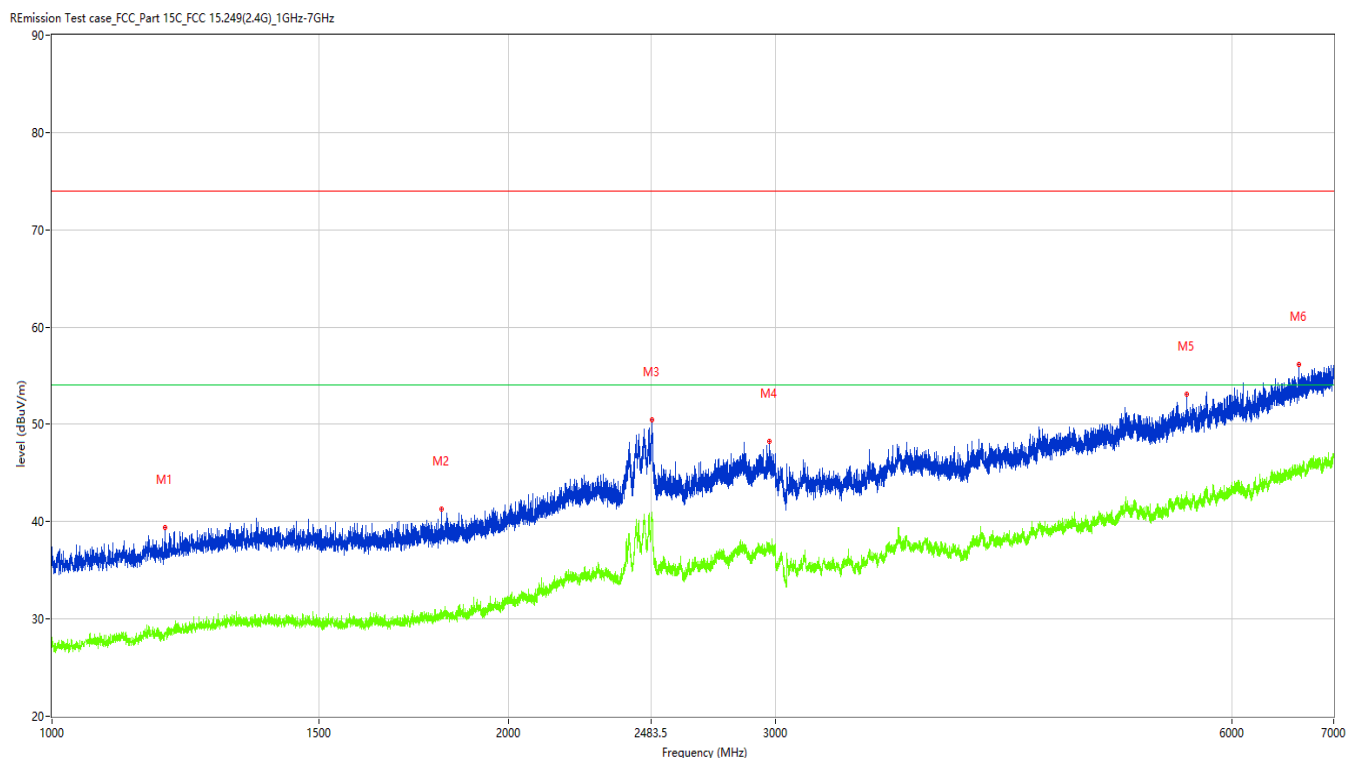
Figure 10: Test plots of Field strength of harmonics, 2403MHz, 1GHz-7GHz, Vertical polarization
