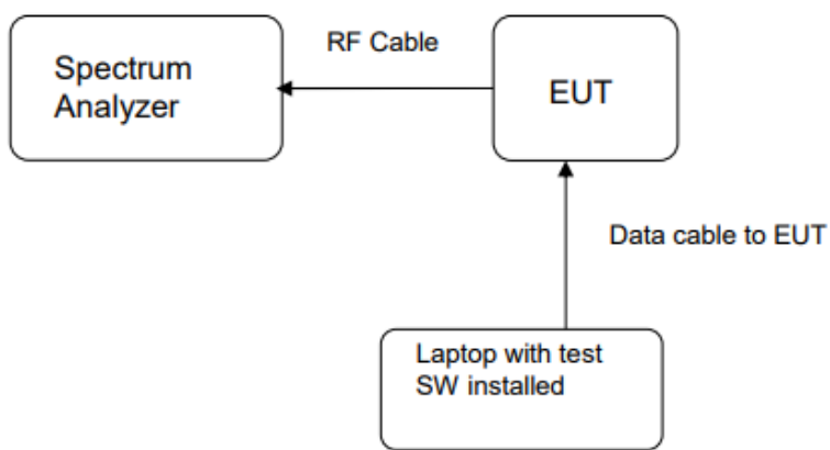
Diagram of Measurement Configuration for Transmitter Test
