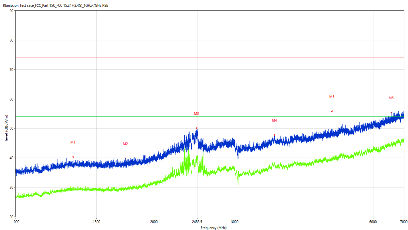
Figure 32: The plots of Radiated Emission, 2440MHz,1GHz-7GHz, Horizontal polarization
