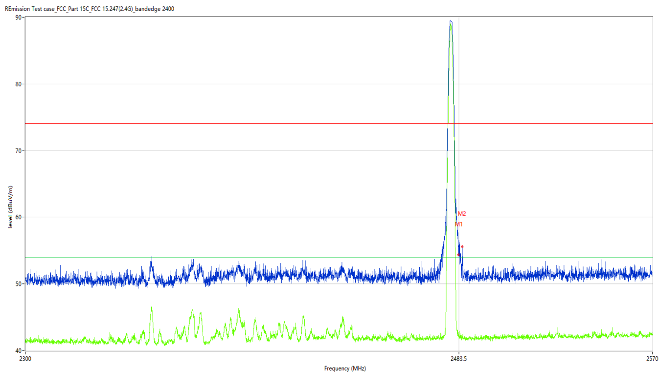
Figure 44: The plots of Band Edge, 2480MHz, Horizontal Polarization
