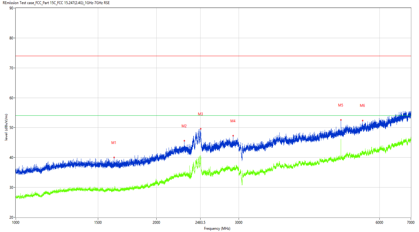
Figure 39: The plots of Radiated Emission, 2480MHz,1GHz-7GHz, Vertical polarization
