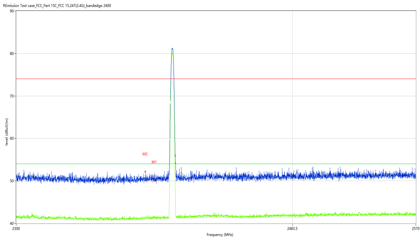
Figure 43: The plots of Band Edge, 2402MHz, Vertical Polarization
