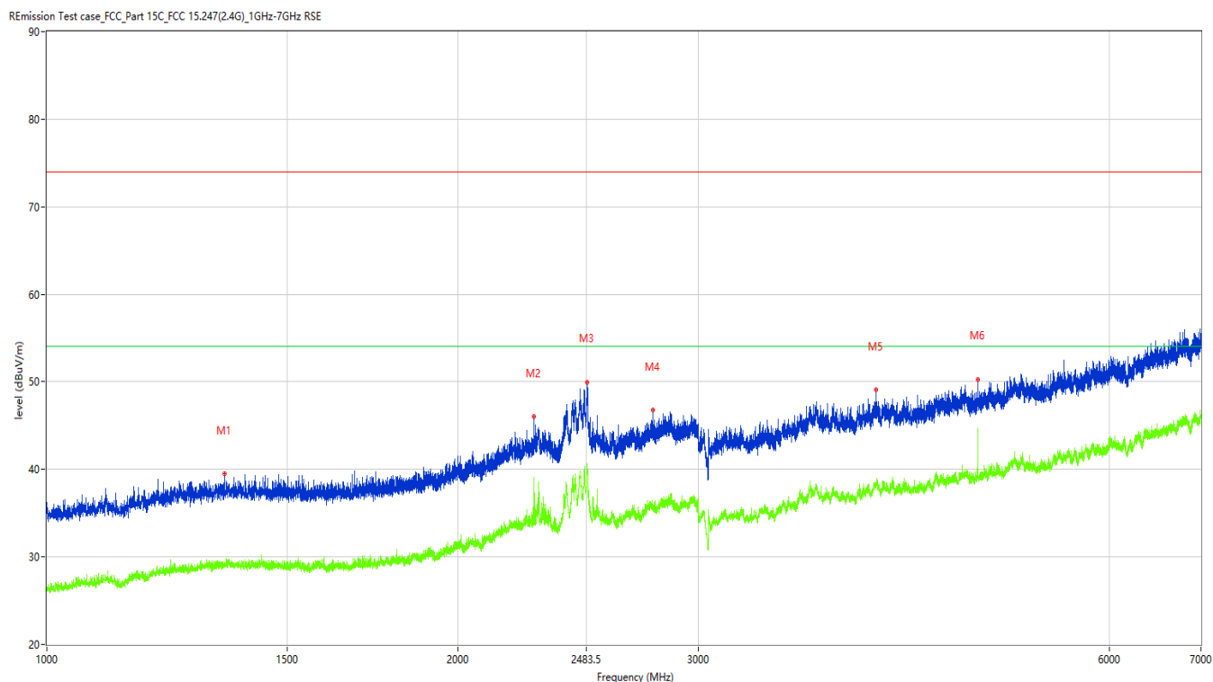
Figure 27: The plots of Radiated Emission, 2402MHz,1GHz-7GHz, Vertical polarization
