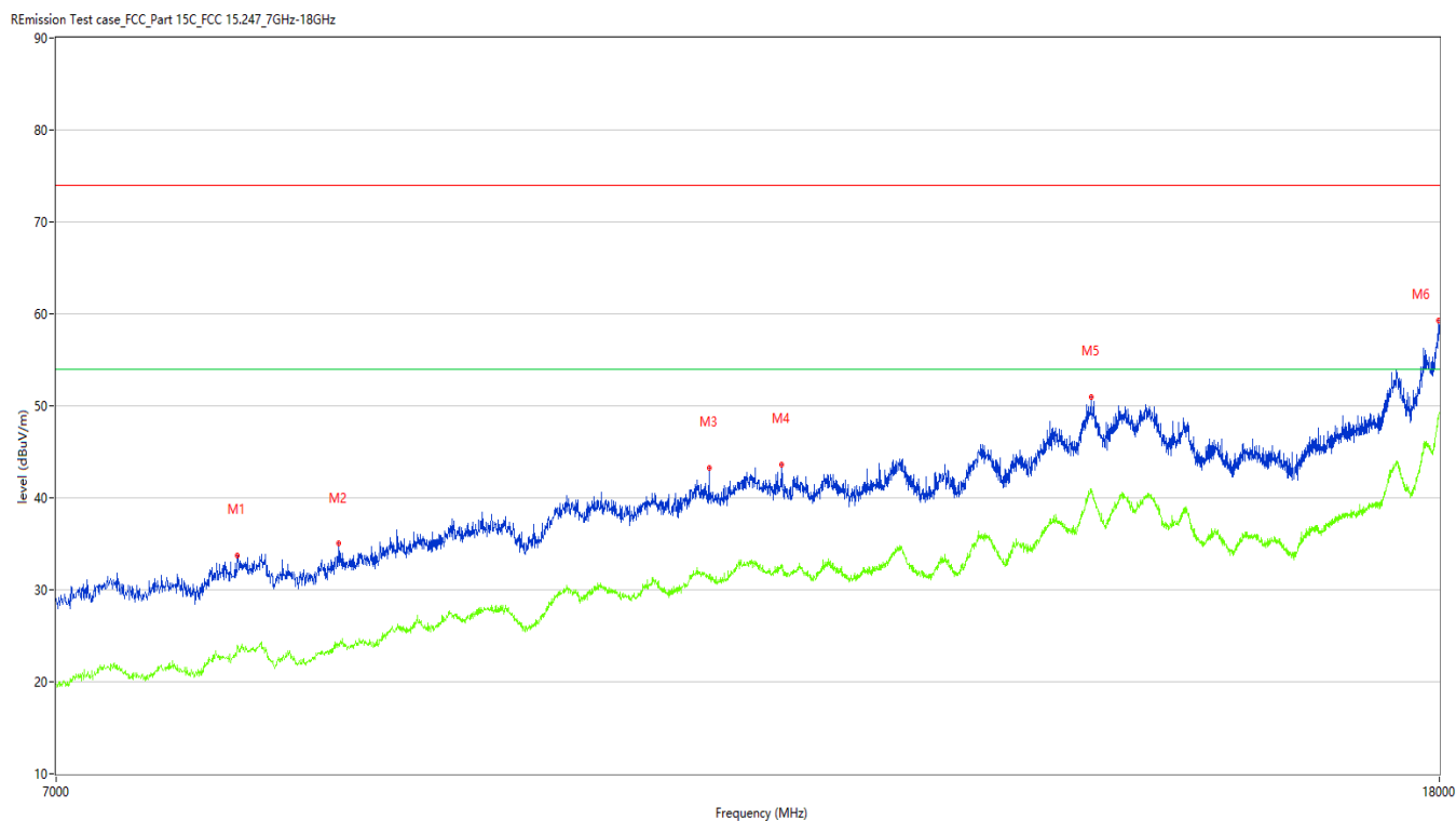
Figure 35: The plots of Radiated Emission, 2440MHz,7GHz-18GHz, Vertical polarization
