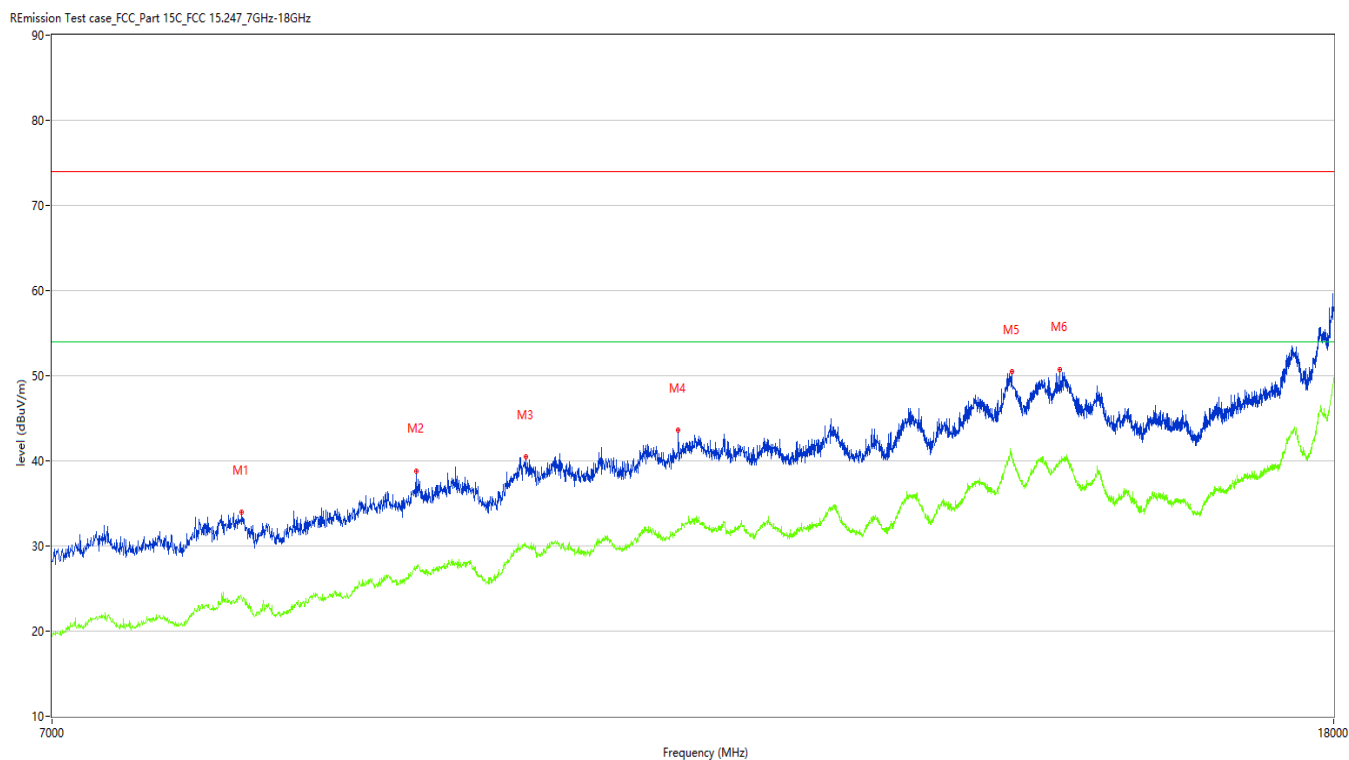
Figure 29: The plots of Radiated Emission, 2402MHz,7GHz-18GHz, Vertical polarization
