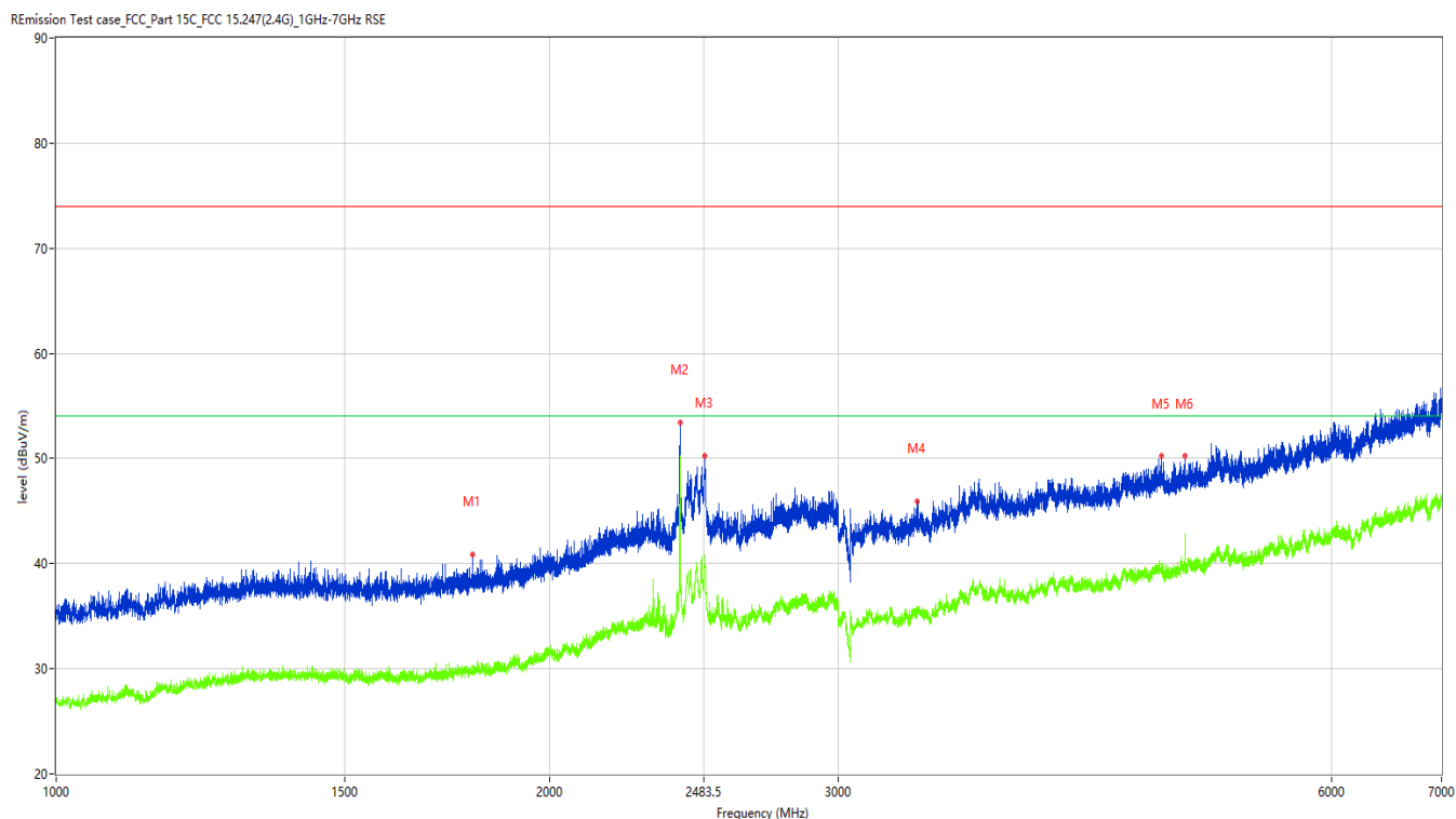
Figure 33: The plots of Radiated Emission, 2440MHz,1GHz-7GHz, Vertical polarization
