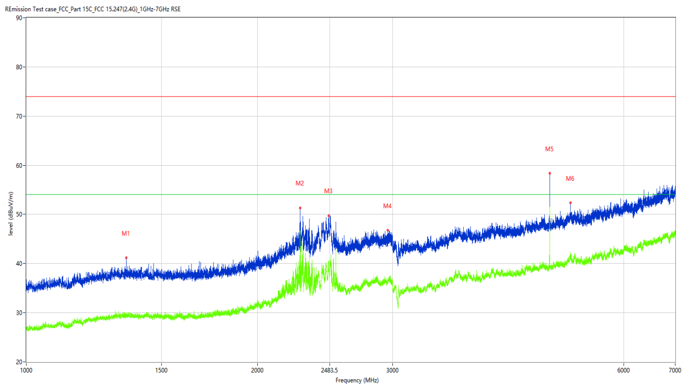
Figure 26: The plots of Radiated Emission, 2402MHz,1GHz-7GHz, Horizontal polarization
