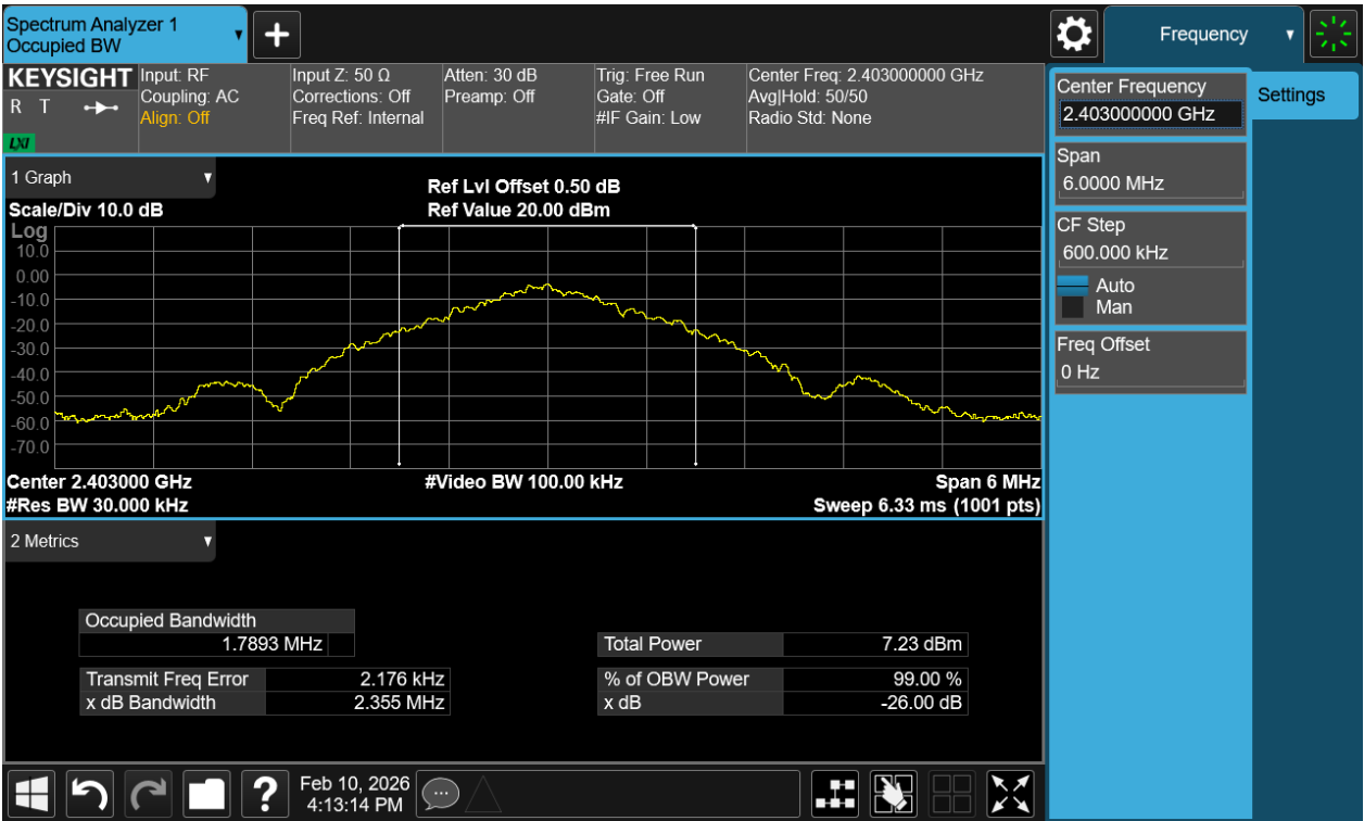
99% Bandwidth, 2403MHz
