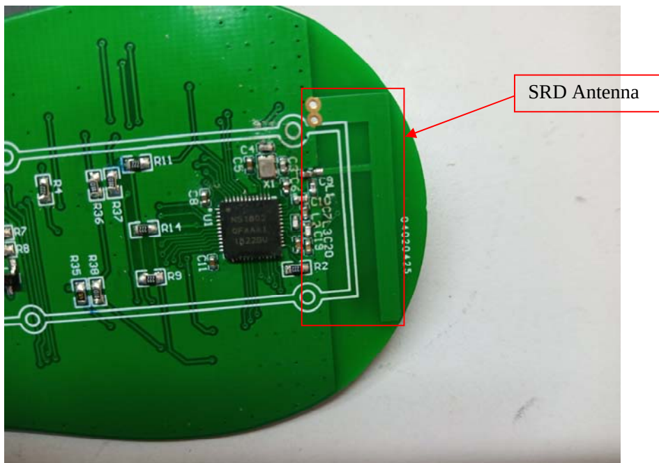
EUT –PCB Chip View-1
