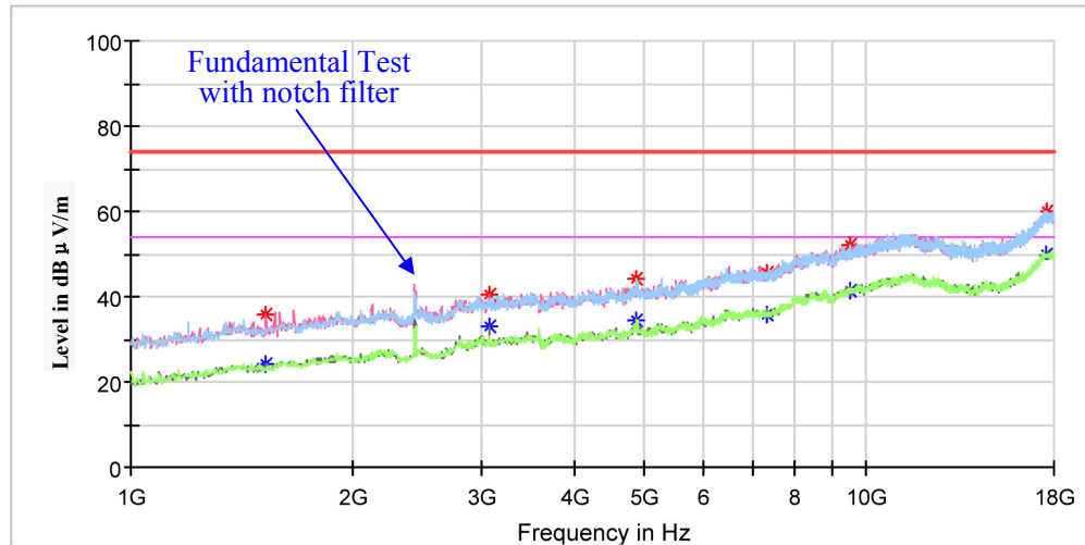
Full Spectrum
