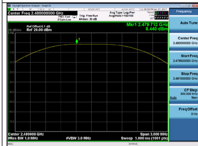
Output Power –Bluetooth LE 2480MHz
