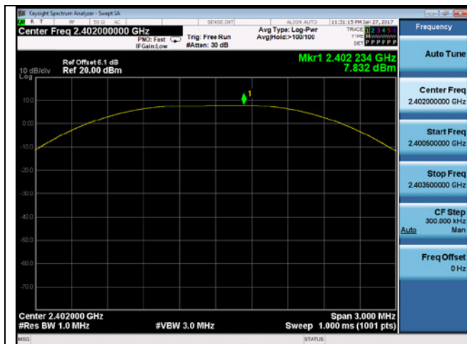
Output Power –Bluetooth LE 2402MHz
