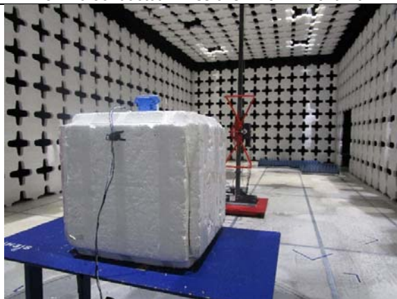
Radiated Emissions (<1GHz) – Front View
